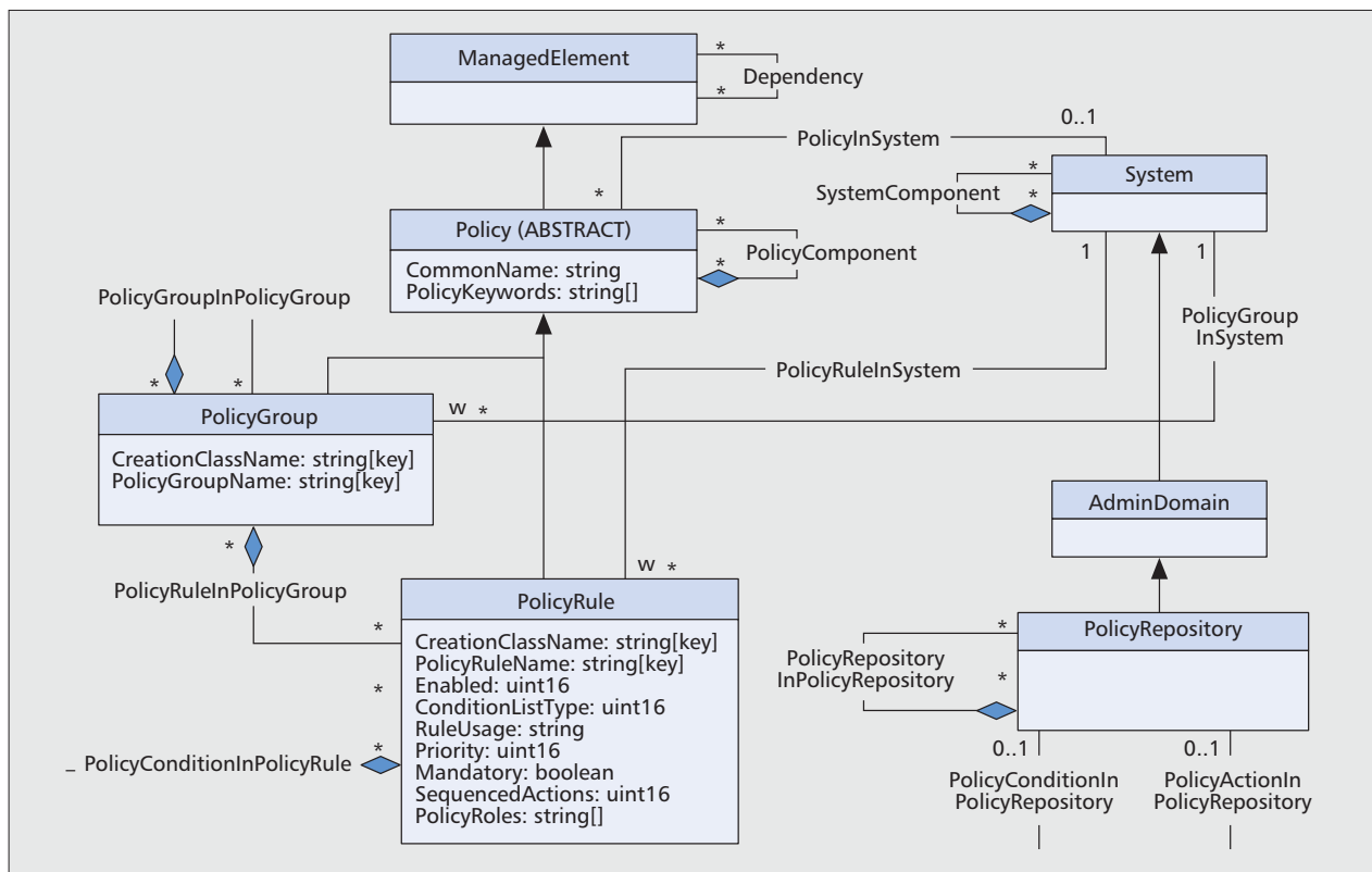
■ Figure 6. The policy core information model (PCIM)(from [22]).
