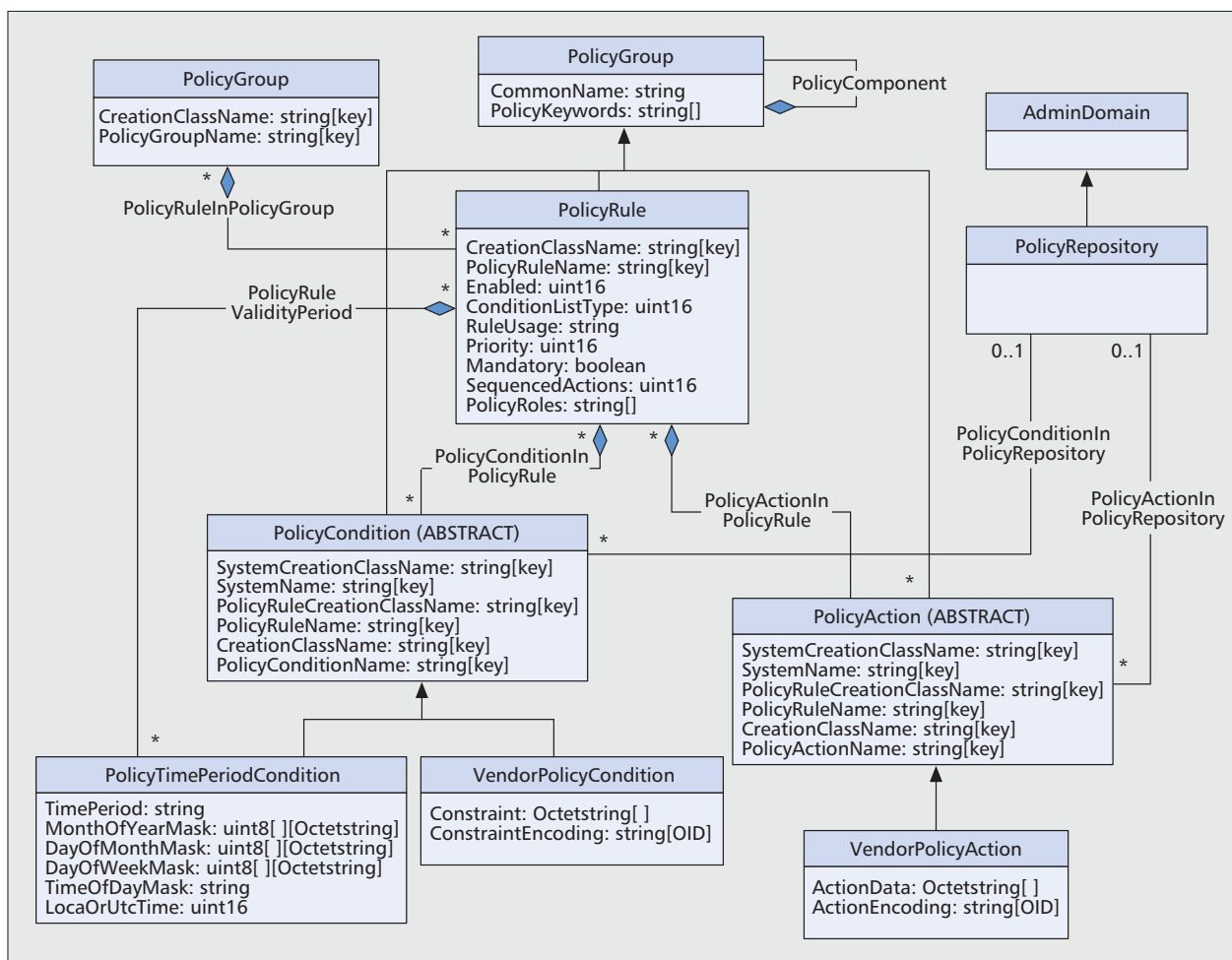
■ Figure 7. PCIM conditions and actions (from [22]).
