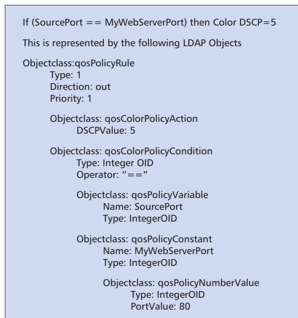
■ Figure 8. A QPIM example policy (from [22]).
