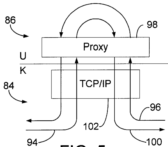
FIG. 5 (PRIOR ART)
