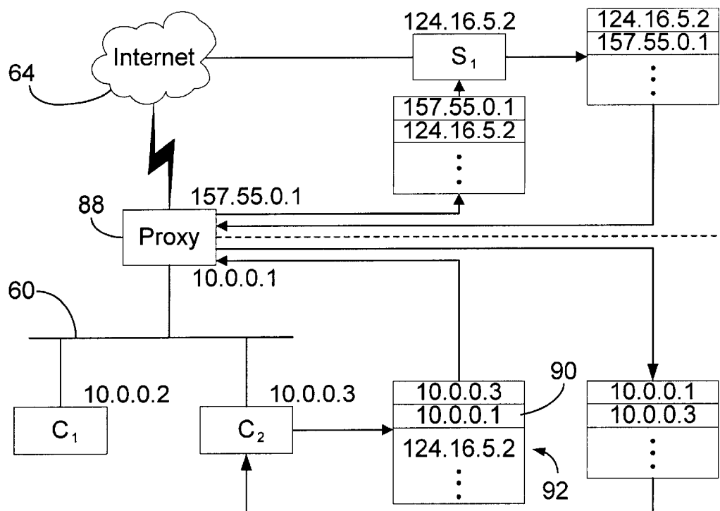
FIG. 6 (PRIOR ART)
