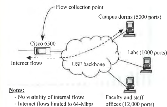
Fig. 2. USF dormitory network configuration.
