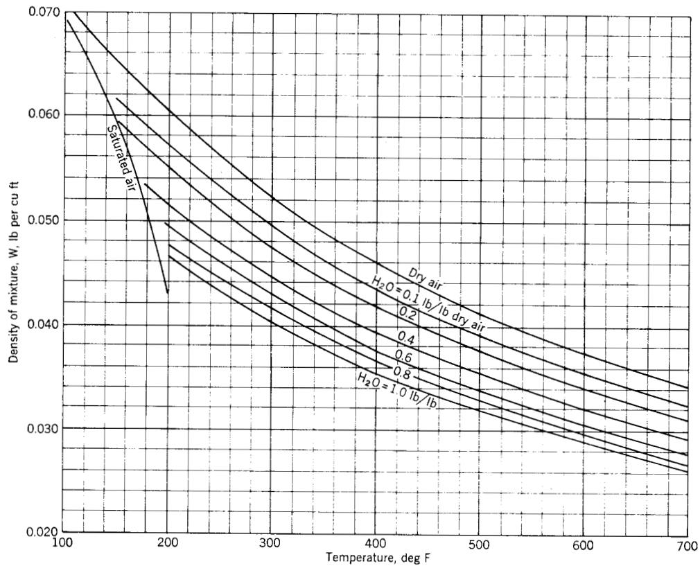
Fig 14-56. Density of air water vapor mixtures lb/ft 3 of mixture 100 to 700°F
