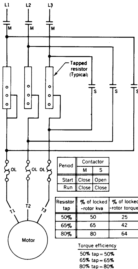
Fig 17-17. Primary resistance (two step)
