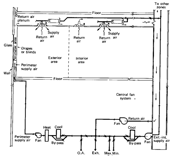
Fig 13-50. Proportionate heat distribution from ceiling arrangement using air diffusers separate from lighting fixture
