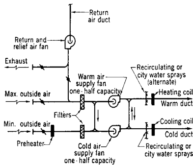
Fig 13-91. Two fan dual duct cycle with blow through dehumidifier
