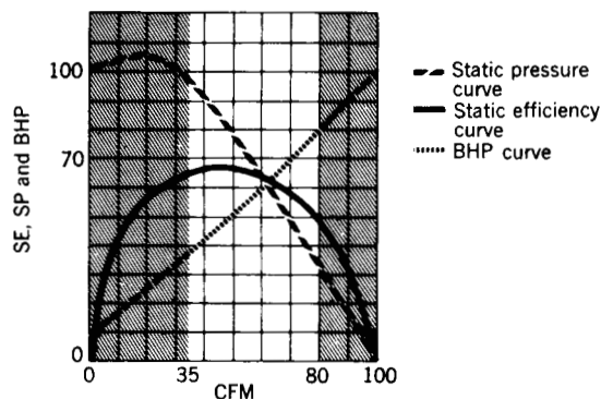
Fig 14-36. Characteristic curves for radial blade fans
