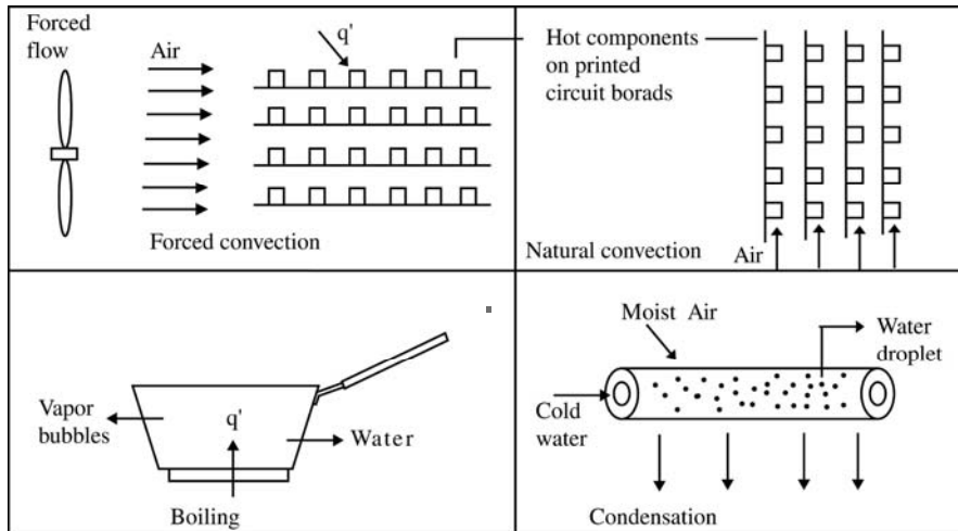
Fig 5-4. Convection heat transfer process
