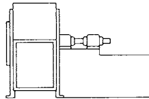
No. 8, SW, SI. For belt drive or direct connection. Arrangement No. 1 plus base for prime mover.
