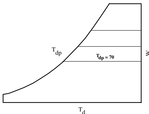
Fig 2-4g. Lines of constant dew point temperature T_{dp} on the psychrometric chart
