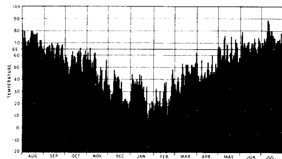
Fig 11-4. Daily mean temperatures for a given year for a specific city
