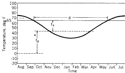
Fig 11-5. Normal daily mean temperatures plotted in a smooth curve
