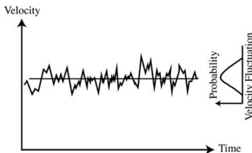
Fig 1-8. Velocity fluctuations with respect to time in turbulent flows
