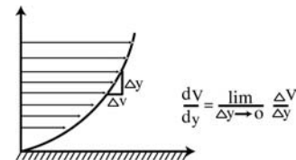
Fig 1-7. Velocity profiles and gradients in viscous flows
