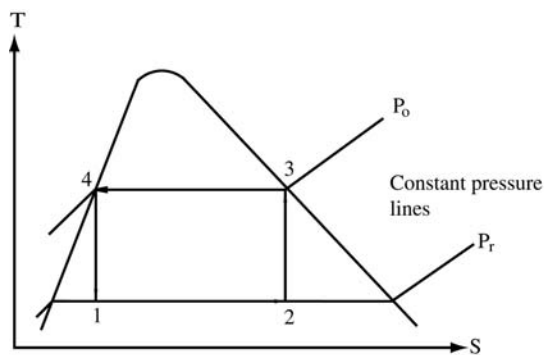
Fig 1-4. Possible thermodynamic realization of a Carnot cycle using a pure substance
