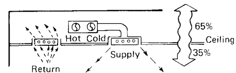
a. Separate fixtures for supply and return (35% energy enters room)
