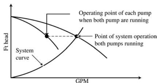
Fig 10-34. Point of system operation, parallel pumps, end point curve
