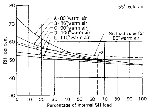
Fig 13-96. Performance over rate of internal sensible heat load; system of Figs. 13-88 and 13-89 for 55°F cold air
