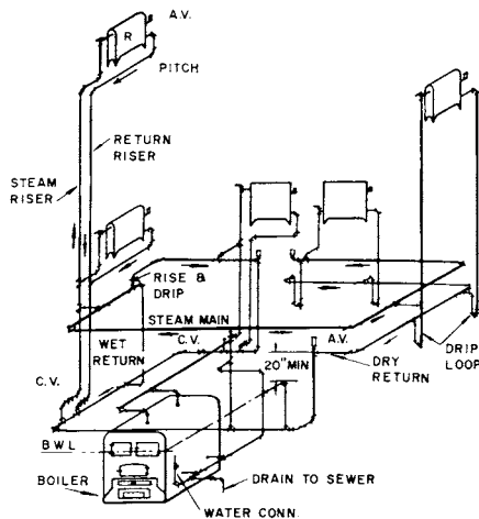
Fig 15-64. Two pipe gravity system
