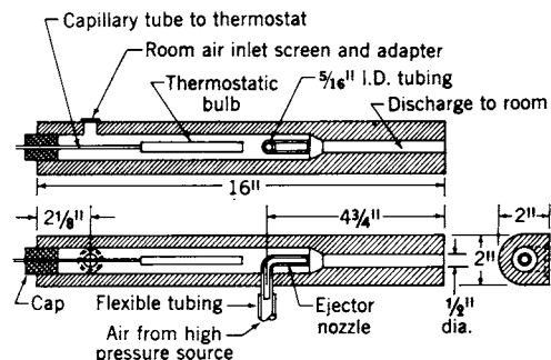
Fig 13-110. Room air sampler tube
