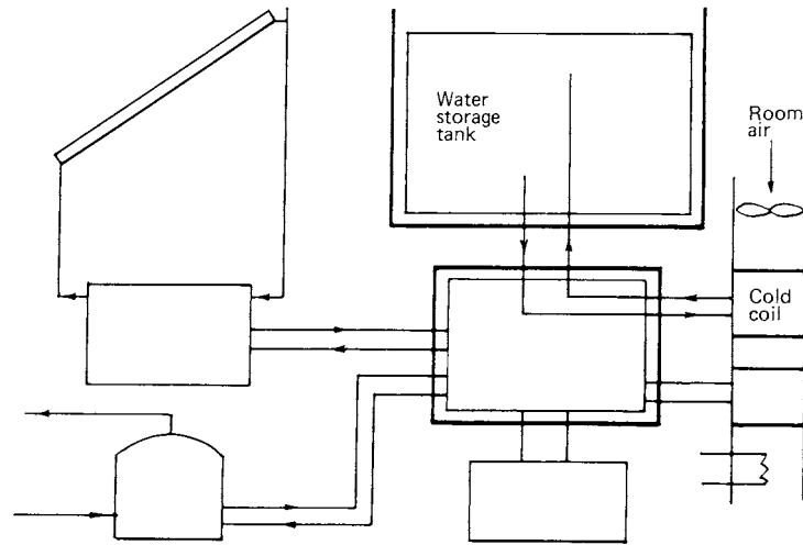
Fig 13-86. Utility off-peak space cooling
