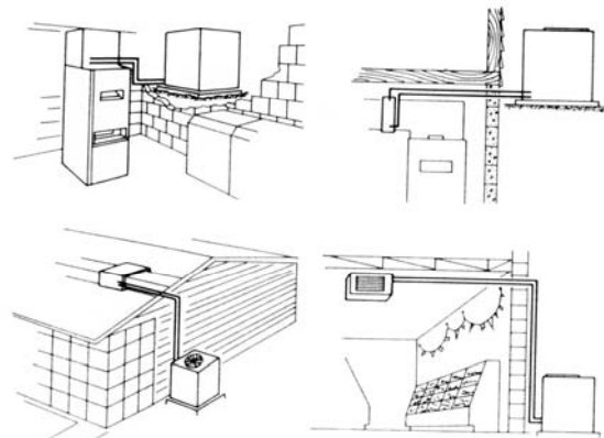
Fig 13-19. Gas fired water chiller with cooling coil
