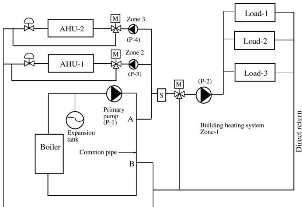
Fig 10-1. Heating system for multiple dwelling building with direct return piping system
