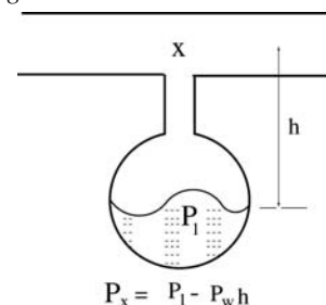
Fig 10-11. Diaphragm tank
