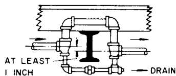
Fig 15-42. Supply main loops
