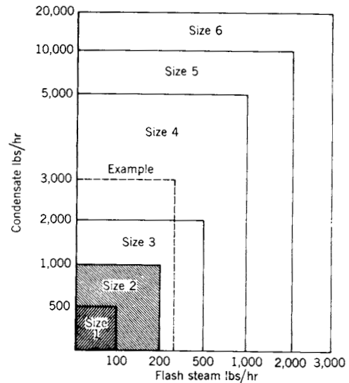
Fig 15-88. Chart for determining size number of tanks
