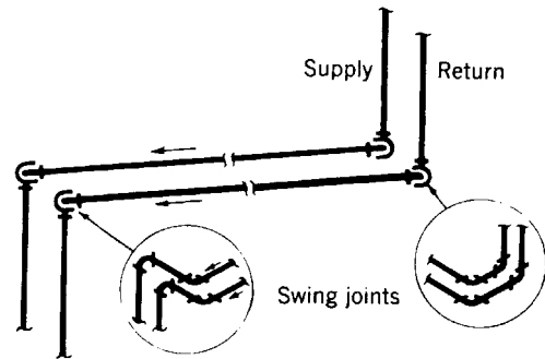
Fig 15-30. Offset connections in riser
