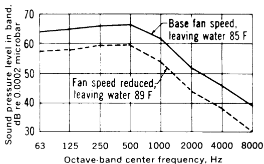
Fig 16-28. Effect of changing leaving water conditions on tower sound level
