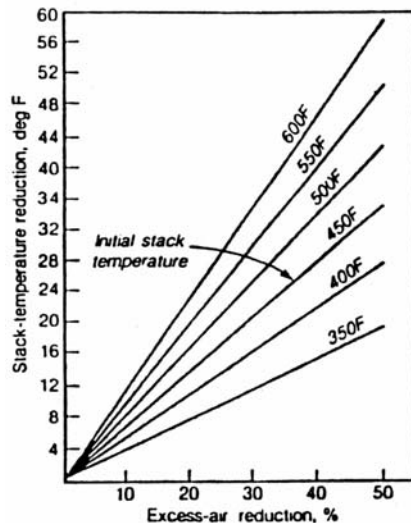
Fig 12-3a. Effect of excess air on temperatures
