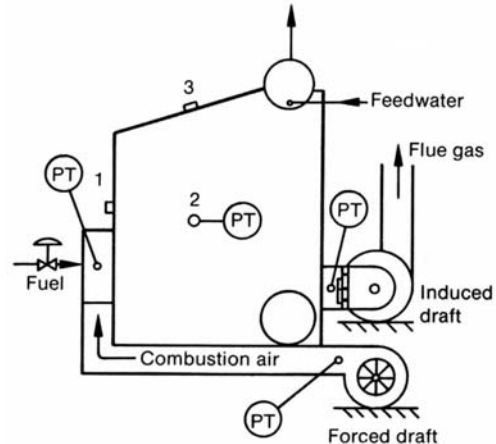
Fig 12-16. Measurement of furnace draft
