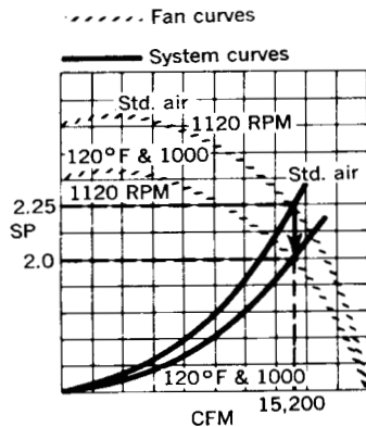
Fig 14-19. Example no. 5—Fan law no. 4 (density change)
