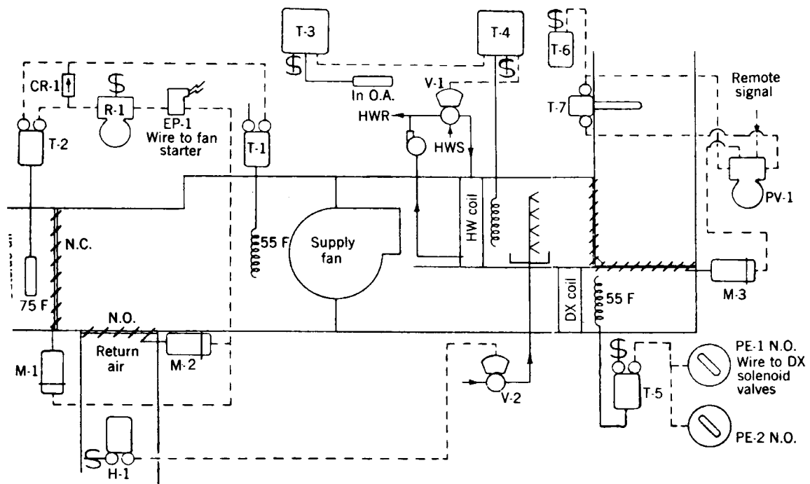
Fig 13-118. Control of typical multizone unit
