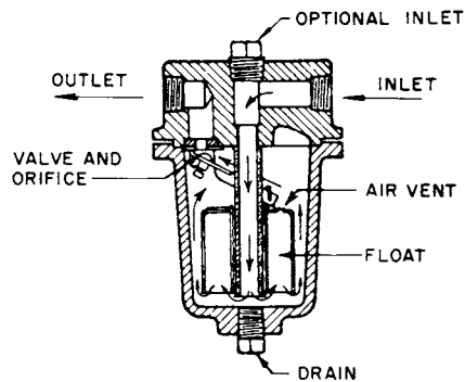
Fig 15-78. Inverted bucket trap with guide
