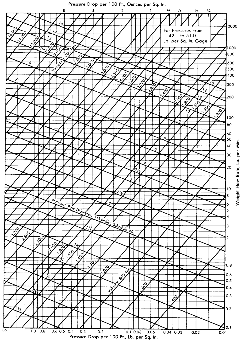
Fig 9-24. For pressure from 42.1 to 51.0 psig
