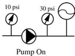
Fig 10-16. Effect of expansion tank location with respect to pump pressure
