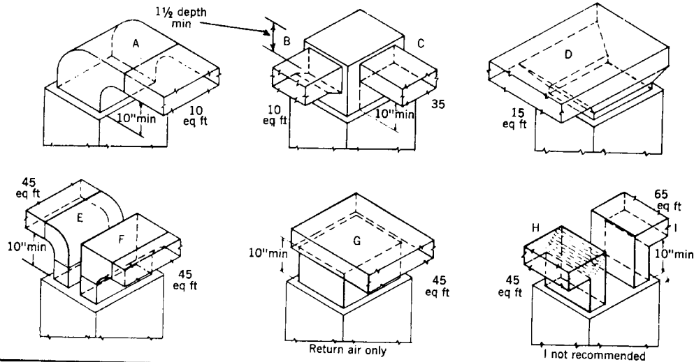
Group 2 Angles and elbows for trunk ducts equivalent lengths based on 8" depth of duct Inside radius \frac{1}{2} width of duct
