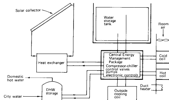
Fig 13-77. Component layout
