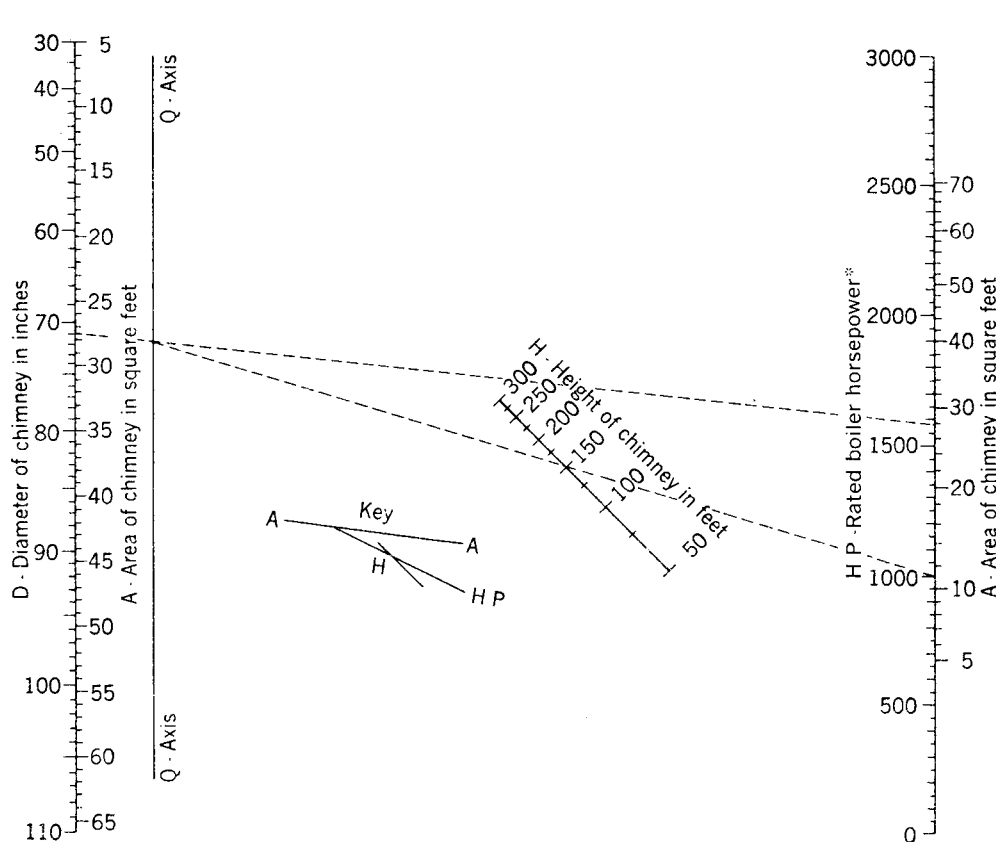
Fig 14-89. Chimney size determination
