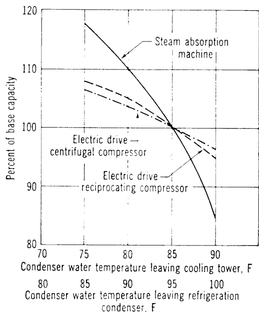
Fig 16-29. Effect of refrigeration system with changes in condensing temperatures
