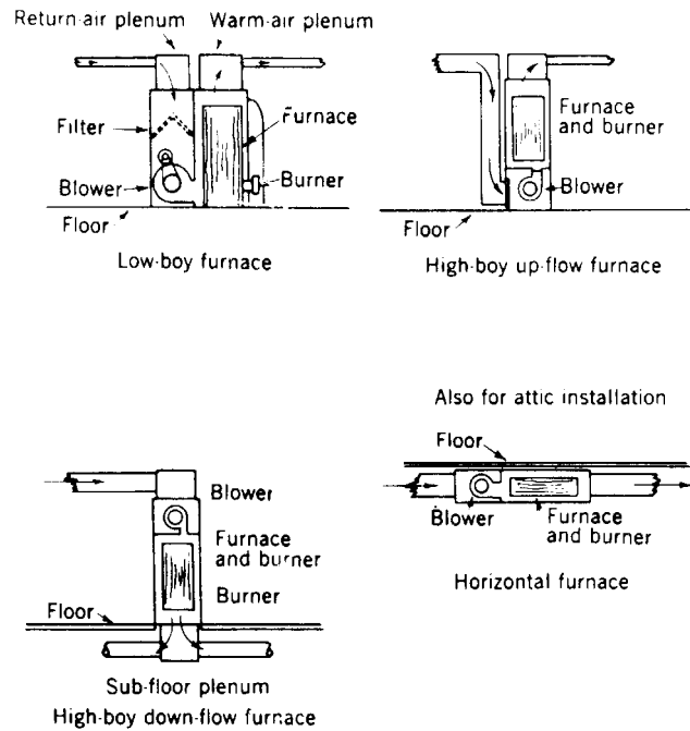
Fig 15-122. Forced air furnaces
