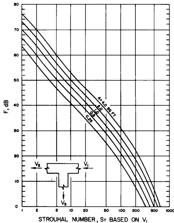
Fig 16-17. Spectrum function F for 90^\circ branch take-offs
