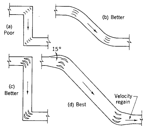
Fig 16-37. Air stream turns, good and bad
