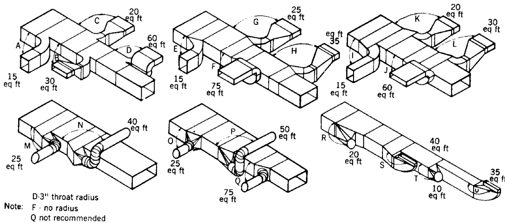
Fig 15-146. Equivalent length of duct fittings (NESCA)
