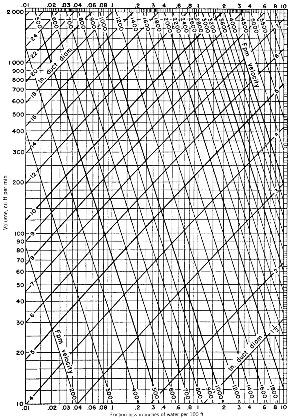
Friction of air in straight galvanized ducts, for volumes of 10 to 2000 cfm.
