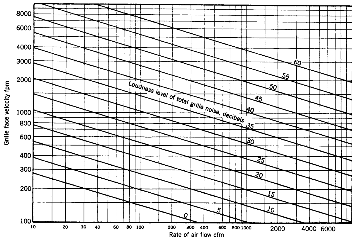
Fig 15-145. Average loudness levels for registers with vertical and horizontal fins
