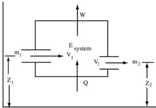
Fig 1-2. Energy flow in general thermodynamic system
