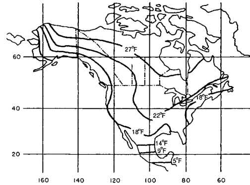
Fig 6-3. Lines of constant amplitude of ground temperature
