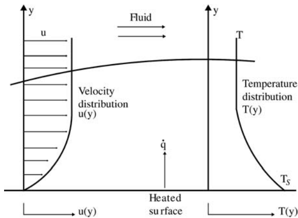
Fig 5-3. Boundary layer development in convection heat transfer
