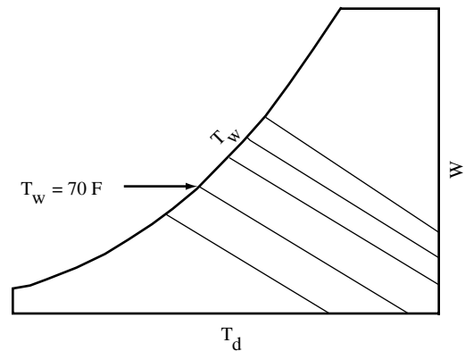
Fig 2-4d. Lines of constant wet bulb temperature T_w on the psychrometric chart
