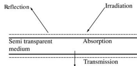
Fig 5-7. Absorption, Reflection, and Transmission processes associated with a semitransparent medium
