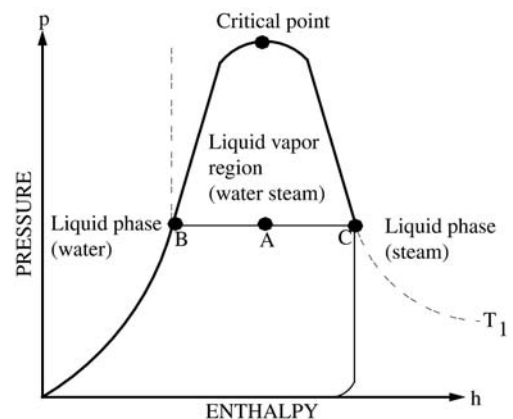
Fig 1-1a. Thermodynamic states of water in p-h coordinates
