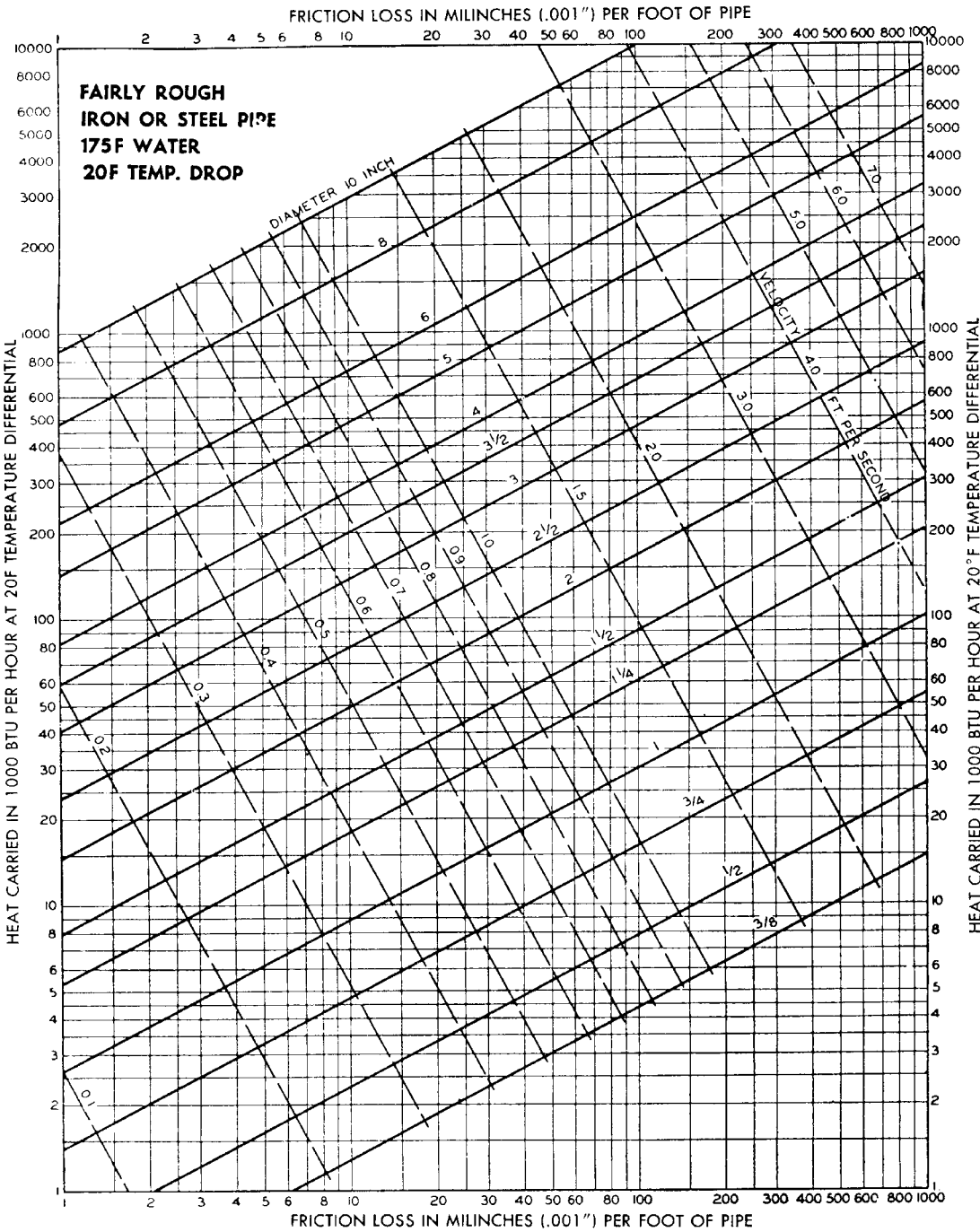
Fig 15-90. Hot water friction chart (for iron or steel tube)
