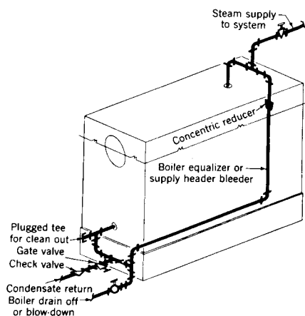
Fig 15-5. Single boiler with direct return connection
