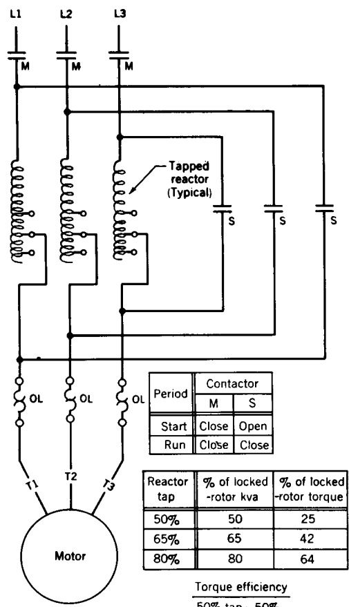
Fig 17-19. Primary reactor (two step)
