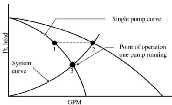
Fig 10-33. Point of system operation, single pump operation, parallel installation
