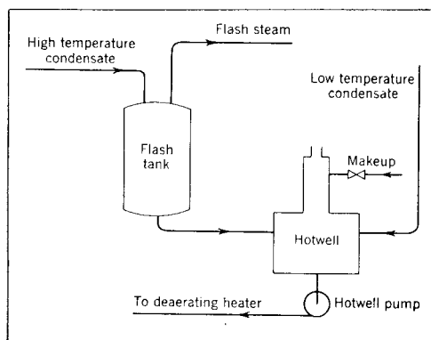
Fig 15-83. Flow diagram for generation of flash steam from high temperature condensate returns
