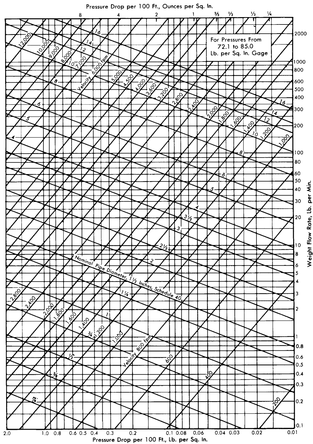
Fig 9-27. For pressure from 72.1 to 85.0 psig
