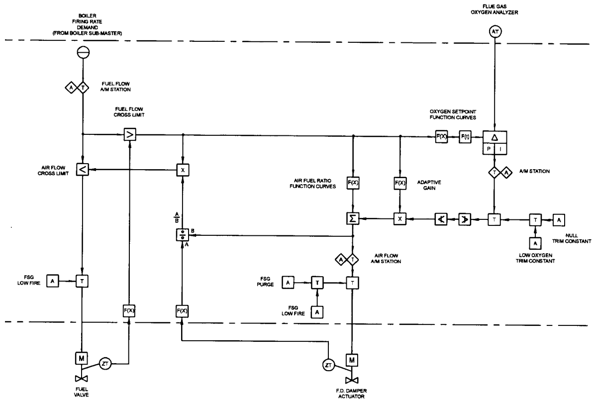
Fig 12-9. Parallel positioning control diagram shown with flue gas oxygen trim
