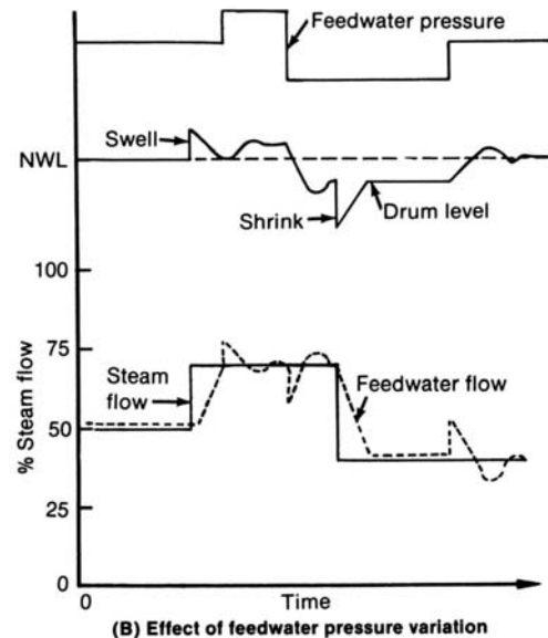
Fig 12-13. Performance of two element feedwater control (effect of feedwater pressure variations)
