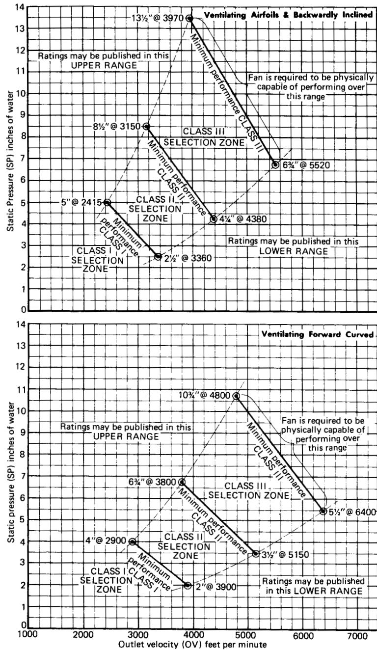
Fig 14-43. Operating limits for double width centrifugal fans
