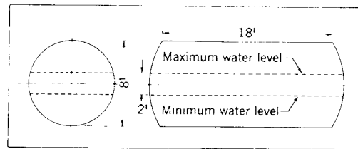
Fig 15-113. Horizontal steam pressurizing tank
