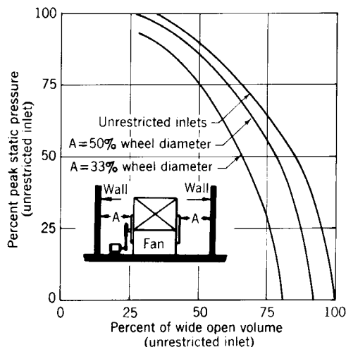
Fig 14-48. Effect of space on fan performance
