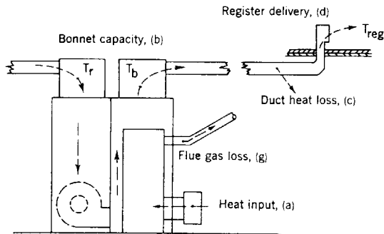
Fig 15-125. Furnace performance terminology
