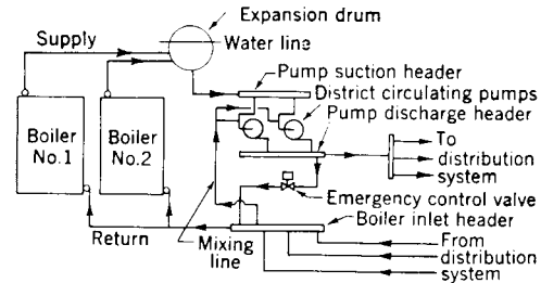
Fig 15-116. Piping arrangement for emergency control valve
