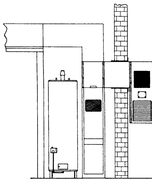
Fig 13-28. Warm air furnaces
