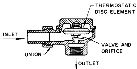
Fig 15-74. Thermostatic trap disc type
