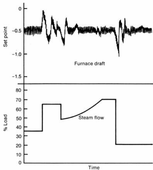
Fig 12-18. Furnace draft control (single element control of induced draft fan)
