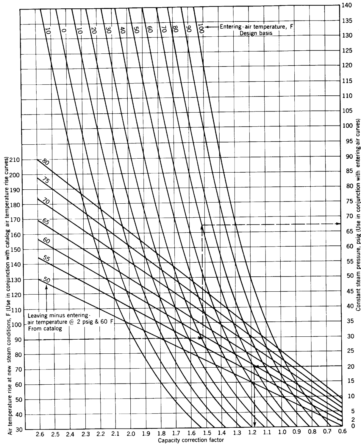
Fig 15-148. Steam supplied unit heater performance factors
