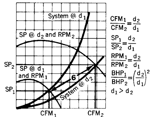
Fig 14-14. Fan law no. 6—density change (constant mass flow)
