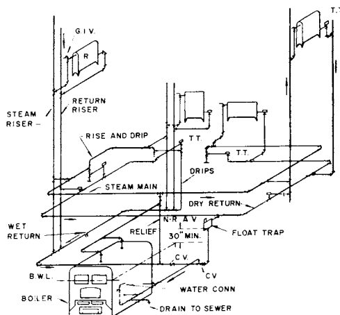
Fig 15-65. Vapor system
