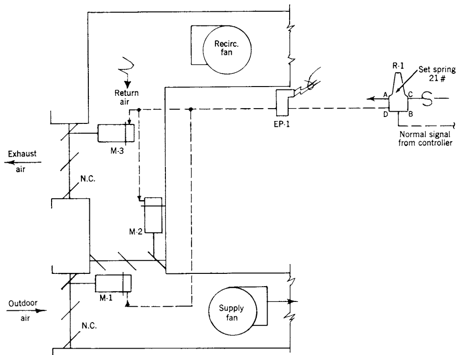
Fig 13-127. Damper operation, day cycle
