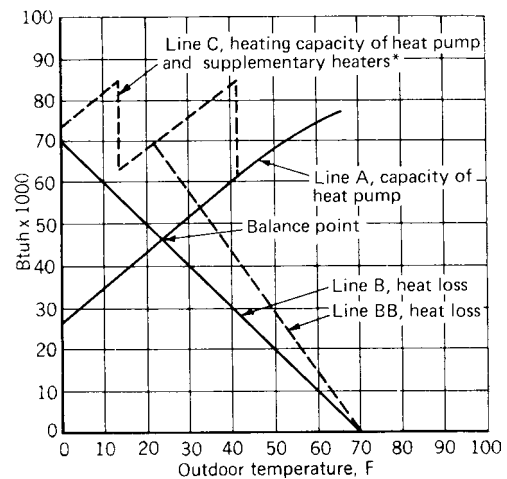
Fig 13-70. Typical air to air heat pump operation with various outdoor temperatures
