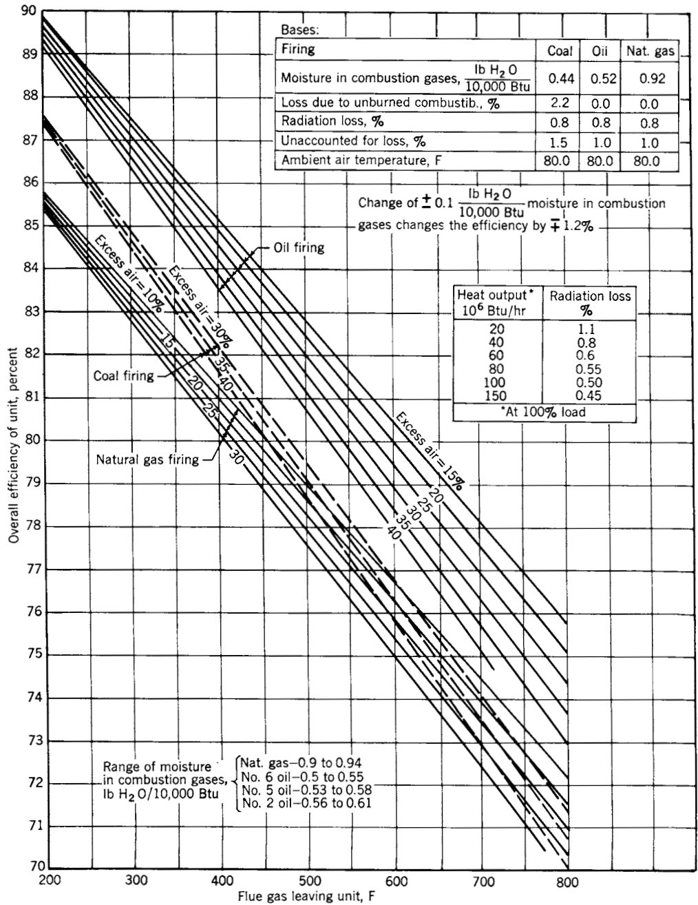
Fig 14-80. Overall efficiency of steam generating unit
