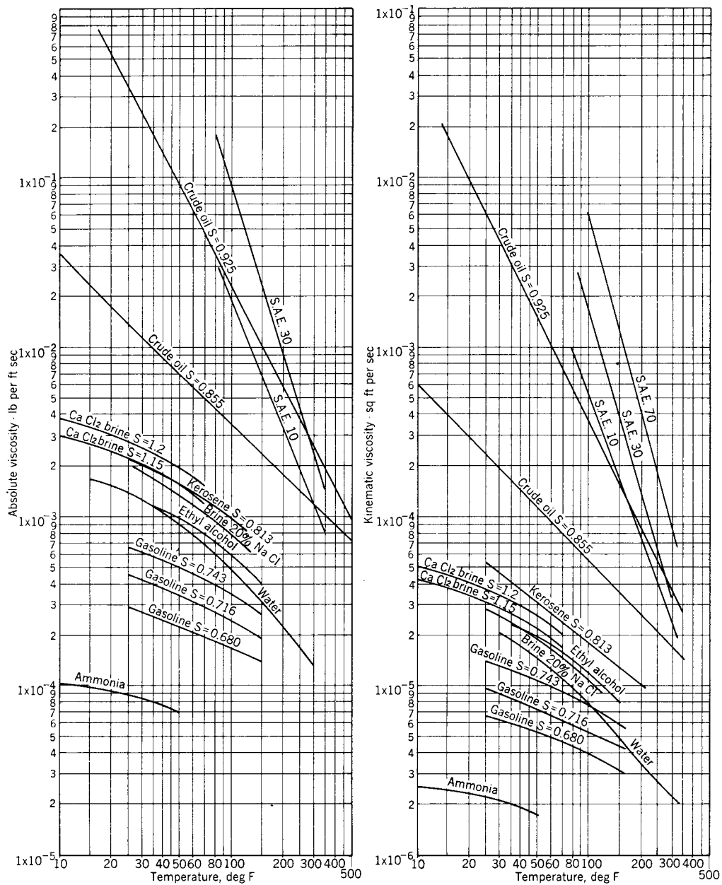
Fig 9-39. Viscosity of liquids with temperature
