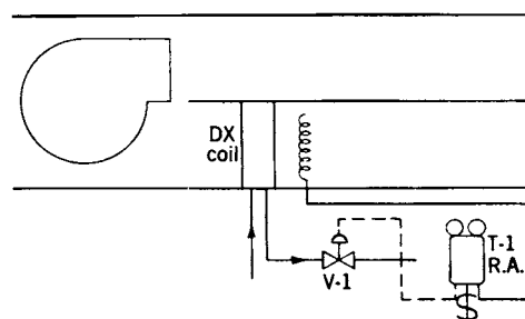
Fig 13-123. Control of cold plenum with cylinder unloader with suction pressure regulator valve
