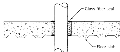
Fig 16-35. Penetration of floor slab by duct (outside of shaft)
