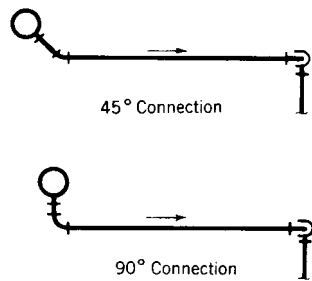
Fig 15-28. Connections from main to down feed riser
