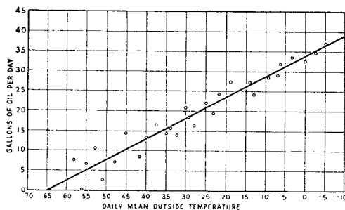
Fig 11-1. Fuel consumption per day plotted against mean daily temperature
