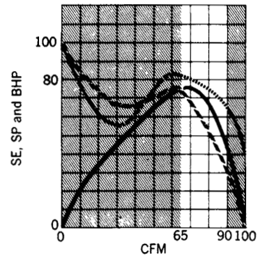
Fig 14-40. Characteristic curves for vaneaxial fans (high performance)
