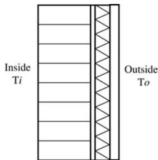
Fig 5-14. Thermal resistance network for three layers
