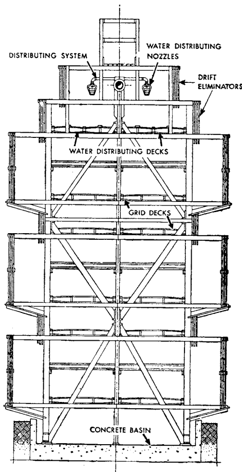
Fig 13-150. Cross section of atmospheric cooling tower
