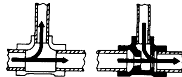
Fig 15-105. Flow through taco venture fitting and standard pipe tee
