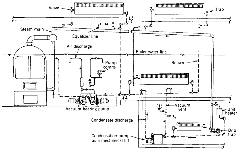
Fig 15-4. Mechanical lift should be installed to handle returns below the level of pump inlets
