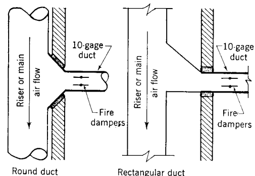
Fig 16-40. Where shaft take-off space is inadequate, use extra heavy duct
