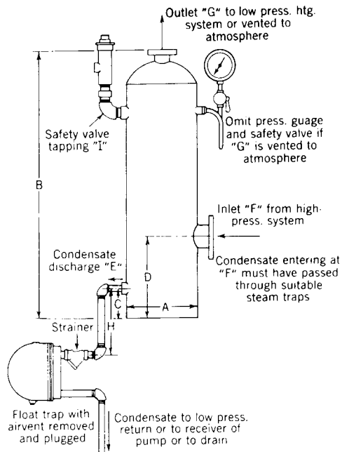
Fig 15-87. Elevation vertical flash tank
