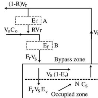
Fig 4-1. HVAC ventilation system schematic
