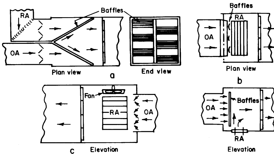
Fig 14-69. Mixing outside and return air
