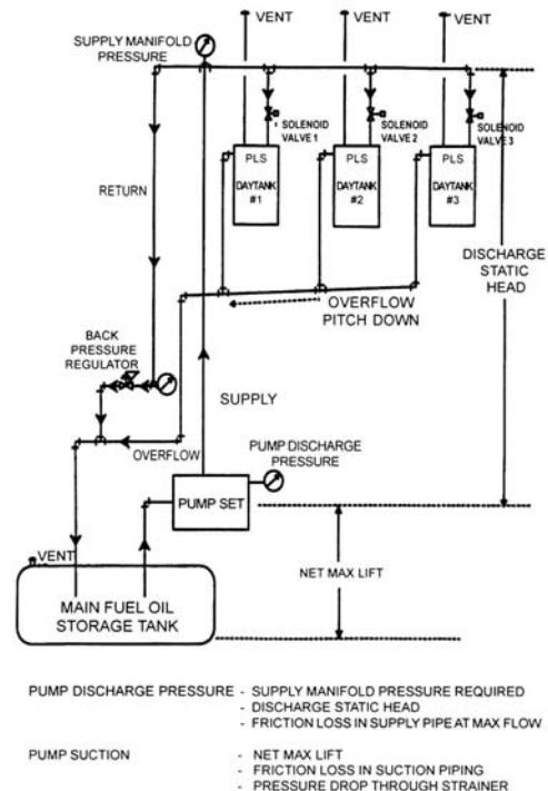
Fig 12-26. Multiple day tanks
