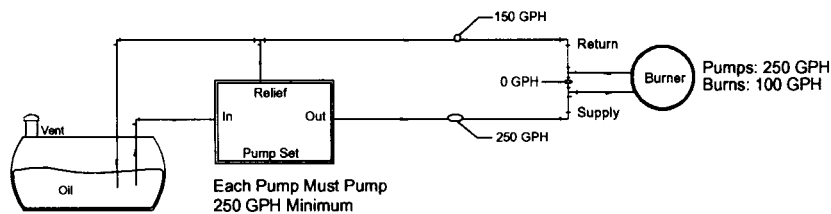
Fig 12-28. Single burner
