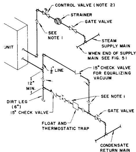
Fig 15-50. Vacuum system steam coil piping
