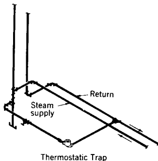
Fig 15-24. Connections for branch mains
