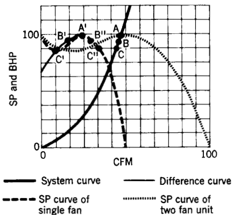
Fig 14-29. Paralleling
