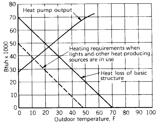
Fig 13-72. Effect of interior heat sources on the heating load and balance point
