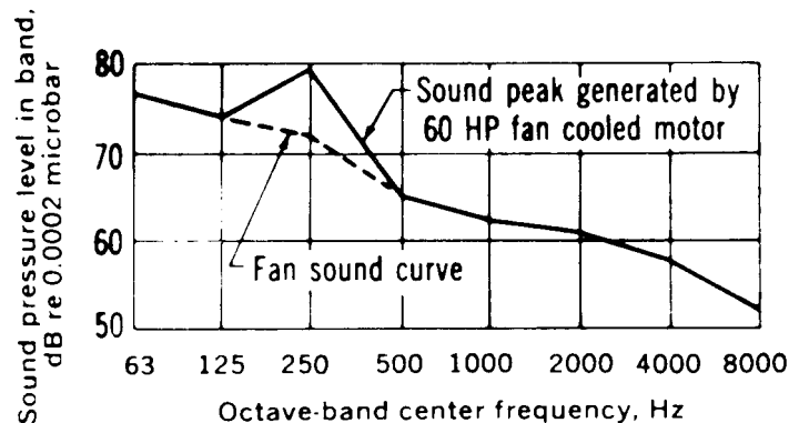
Fig 16-24. Tower water noise spectrum
