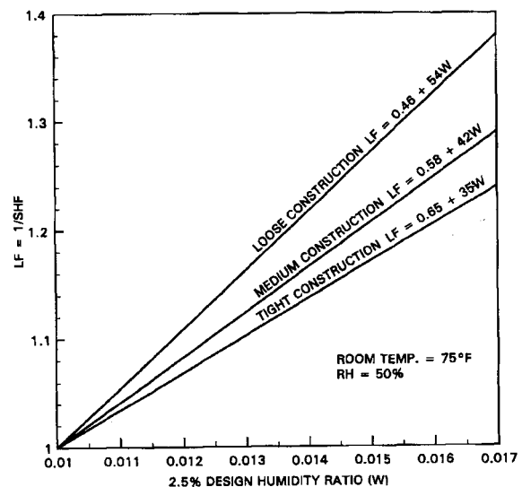
Fig 7-4. Effect of infiltration on latent load factor
