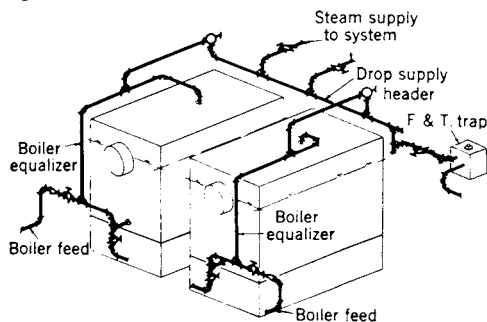
Fig 15-7. Two boilers with separate direct return connections from overhead
