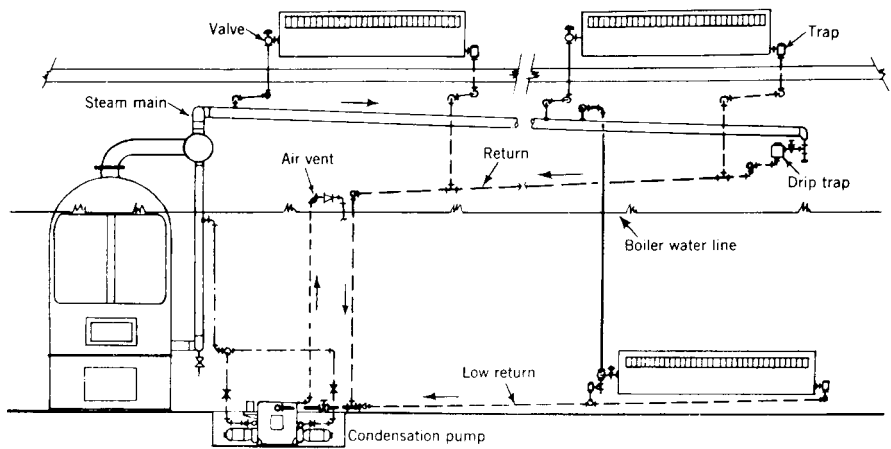
Fig 15-2. Basic components of steam heating system
