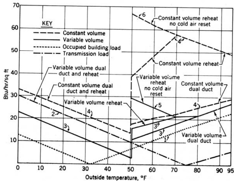
Fig 13-45. Energy requirements in Btu conditions - no sunload, southern exposure
