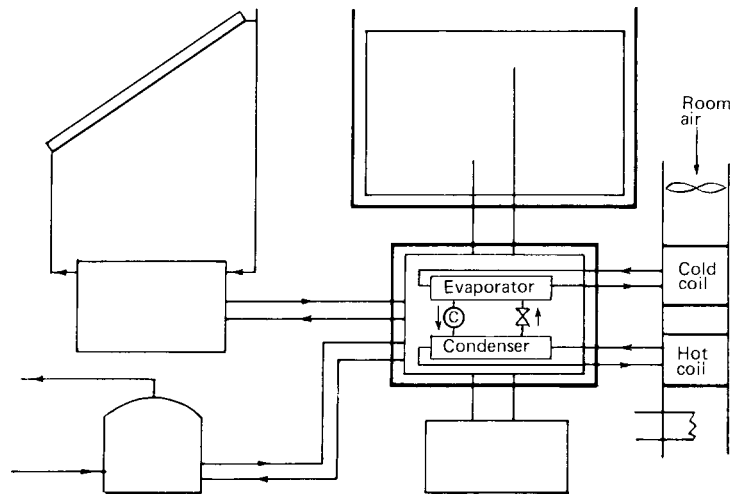
Fig 13-87. Dehumidification
