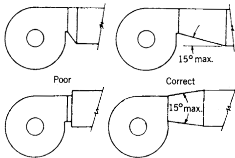
Fig 14-50. Duct transition pieces for centrifugal fan discharge. top: right and wrong transition piece with expansion all on one side of duct. bottom: right and wrong transition piece with expansion in two directions.
