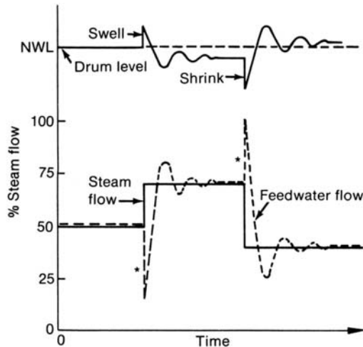
Fig 12-11. Control action of mechanical single element feedwater regulator
