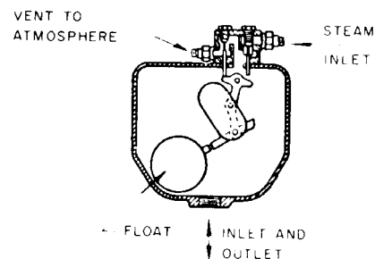
Fig 15-82. Boiler return trap or alternating receiver
