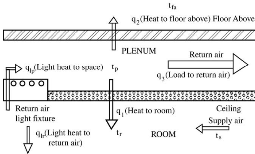
Fig 7-2. Heat balance of typical ceiling return plenum
