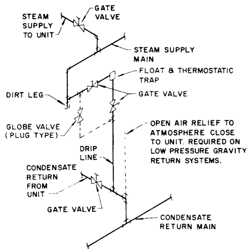
Fig 15-51. Dripping steam supply to condensate return
