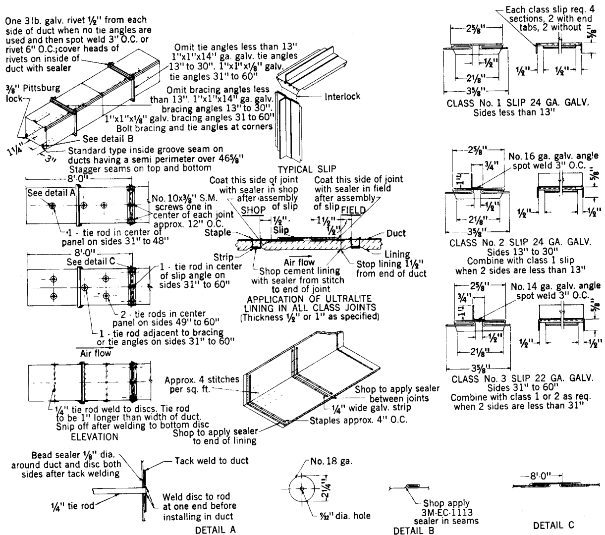
Fig 13-116. Construction of high pressure rectangular ducts
