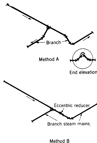
Fig 15-22. Two methods of splitting a single steam main without a drip
