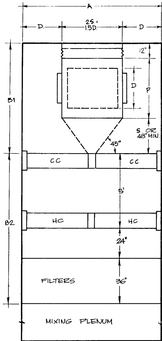
AIR HANDLING UNIT SCHEMATIC PLAN LAYOUT
