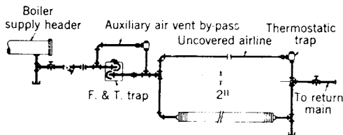
Fig 15-16. Boiler supply header drip
