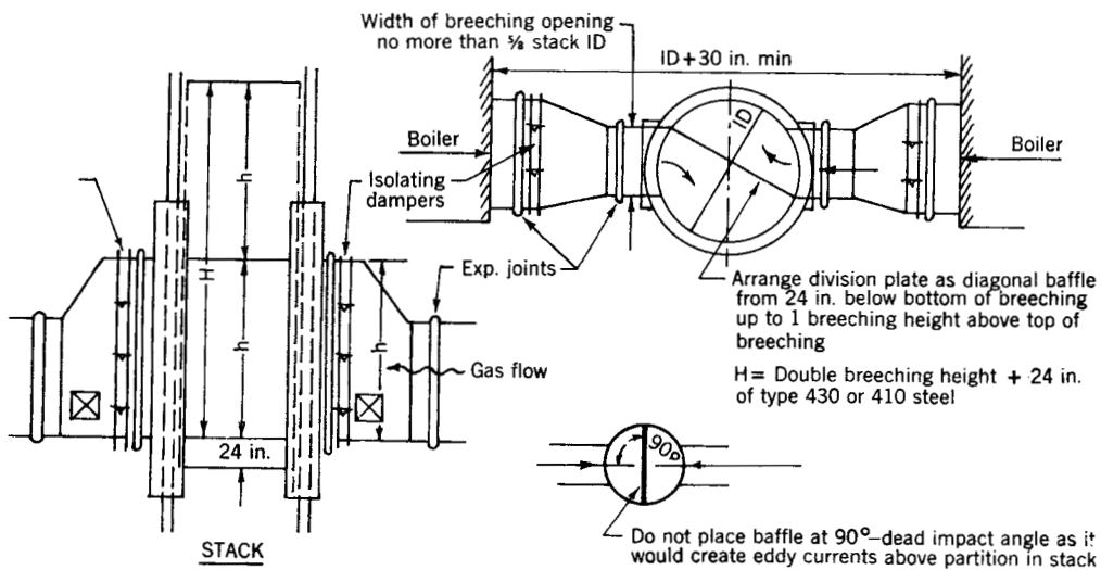
Fig 14-82. Opposite stack entry
