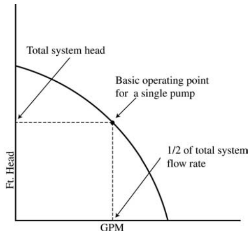
Fig 10-28. Basic pump operating point
