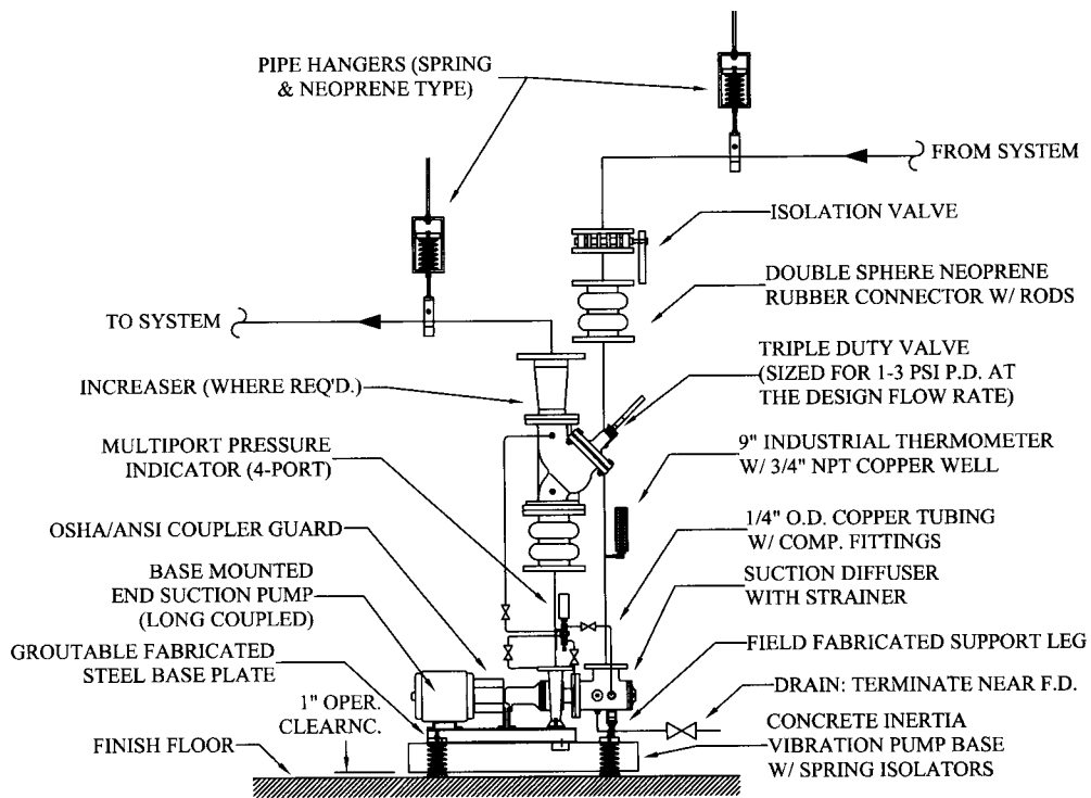
Fig 10-22. End suction pump detail
