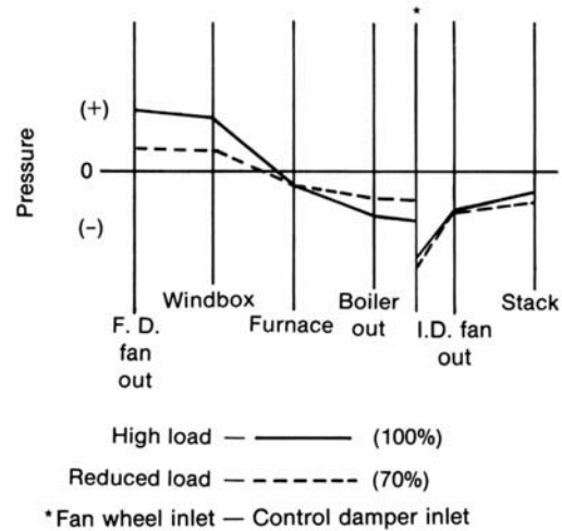
Fig 12-16. Measurement of furnace draft
