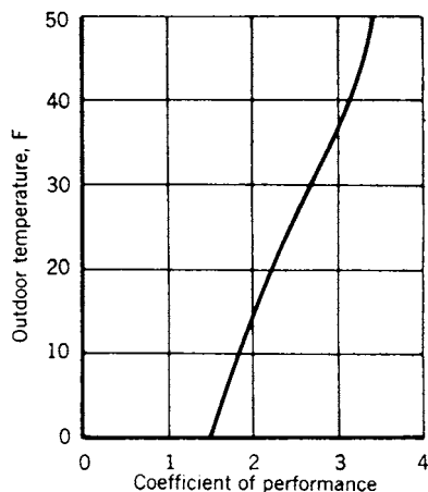
Fig 13-69. COP of air to air heat pumps for heating
