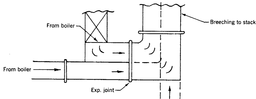
Fig 14-83. Breeching entries for joining gas flows parallel
