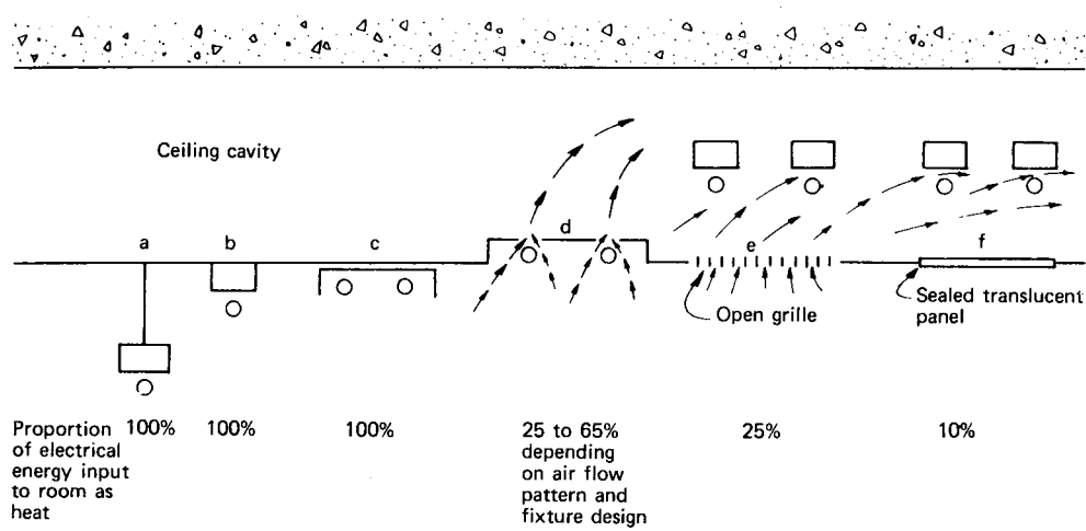
Fig 13-52. Proportionate heat distribution through luminous or louvered ceiling
