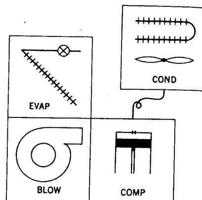
Fig 13-4. Vertical self contained air conditioned unit
