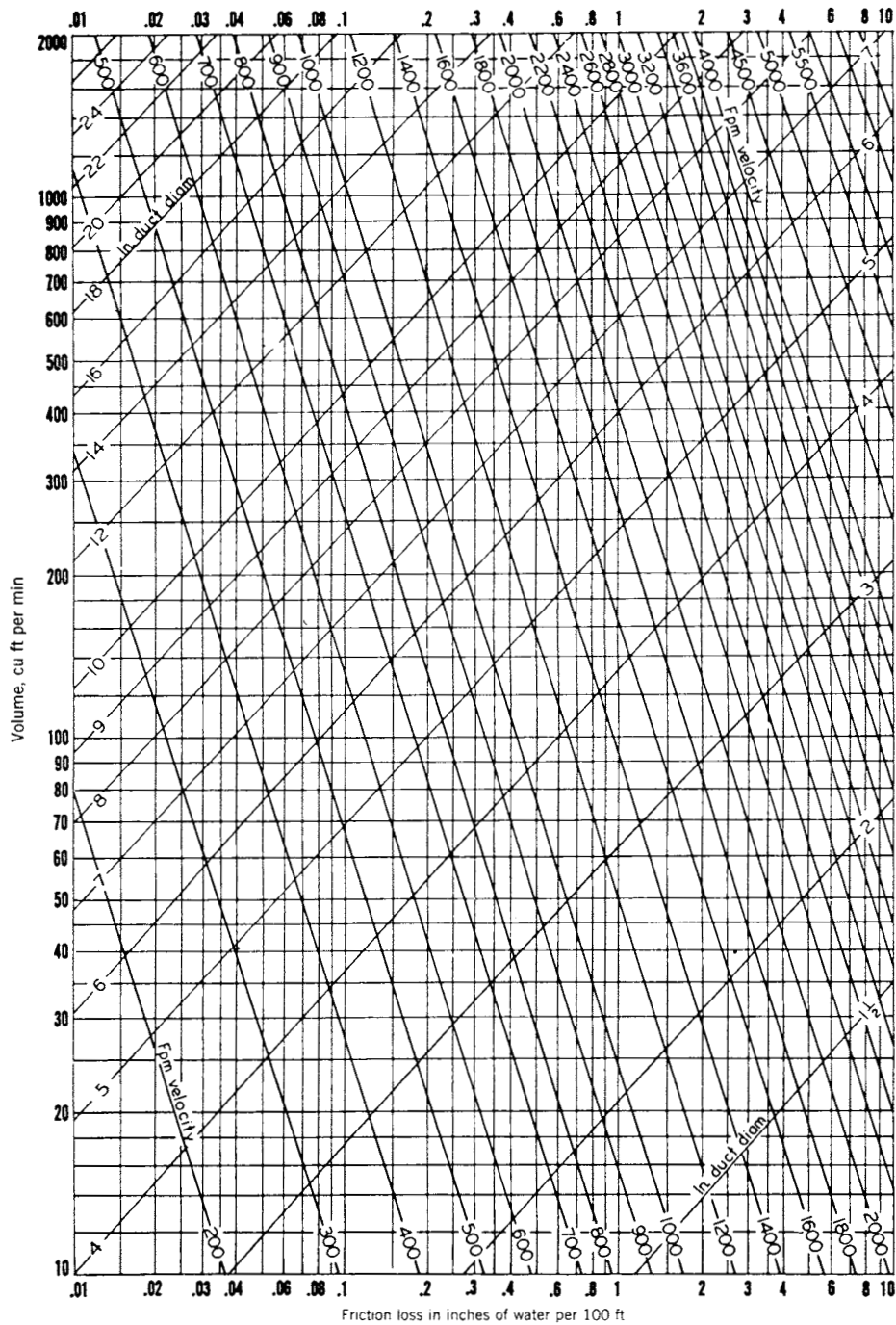
Fig 14-59a. Friction of air in straight aluminum ducts for volume of 10 to 2000 cfm (Same basis and source as Fig. 14-59b)
