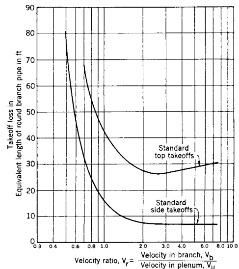
Fig 15-129. Loss of extended plenum fittings, in equivalent length of branch duct
