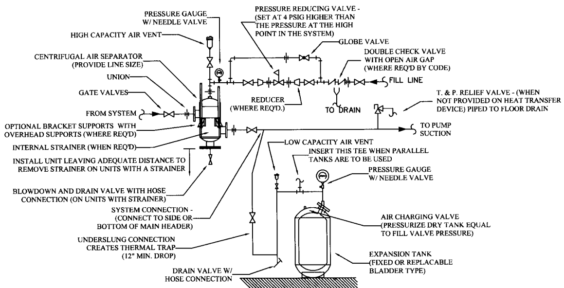
Fig 10-8. Air separator and expansion tank detail
