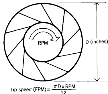
Fig 14-8. Tip speed
