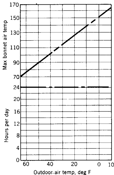
Fig 15-139. Air flow and air temperature for continuous blower operation
