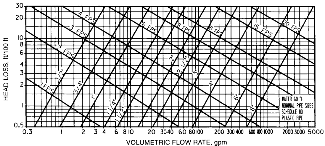
Fig 9-3. Friction loss for water in plastic pipe (Schedule 80)
