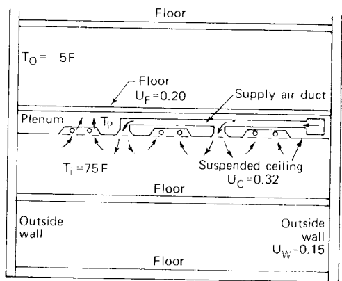
Fig 13-55. Typical plenum arrangement
