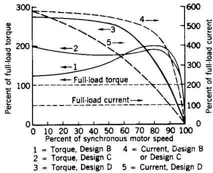
Fig 17-2. Torque current relationships for 100 hp, 1800 rpm motor; locked rotor kva/hp = 5.52; Code letter F
