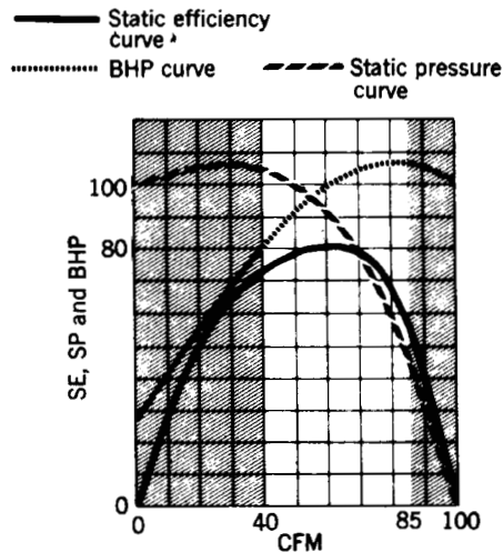
Fig 14-34. Characteristic curve for radial blade fans
