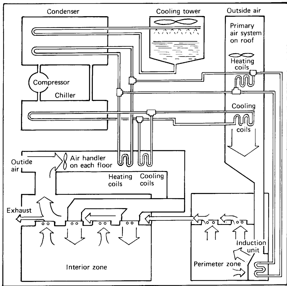
Fig 13-62. Schematic diagram of heat recovery system using split condenser as installed in an office building
