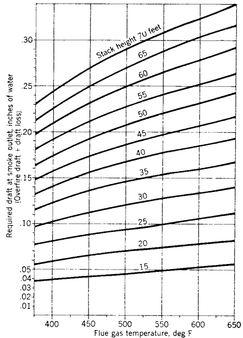
Fig 14-90. Chimney draft versus flue gas temperature for various height chimneys
