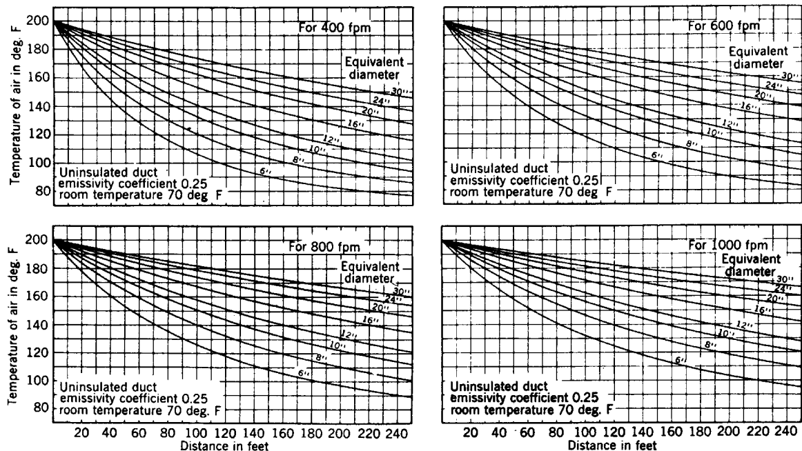
Fig 15-141. Temperature drop in ducts for different air velocity
