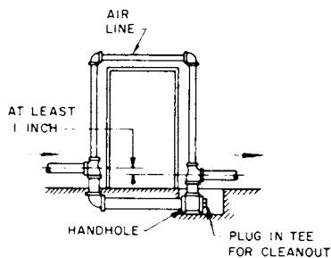
Fig 15-43. Return main loop
