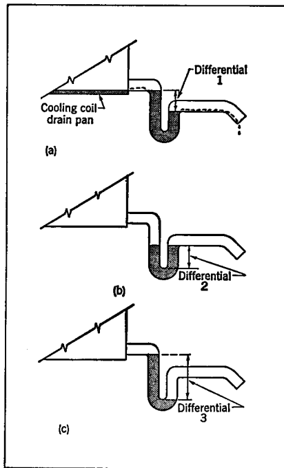
Fig 14-78. Properly designed trap, shown, here does not lose its seal under various fan conditions. (a) Fan running and condensate draining; (b) Fan off; (c) Trap solves the problem)
