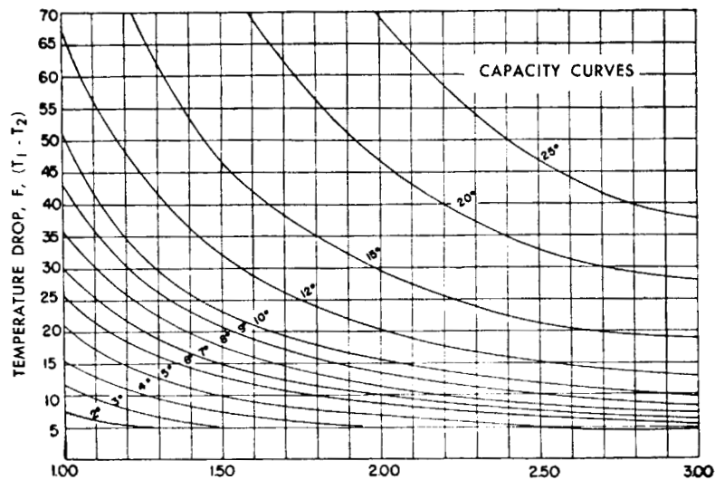
Fig 13-149. Capacity curves for atmospheric cooling towers
