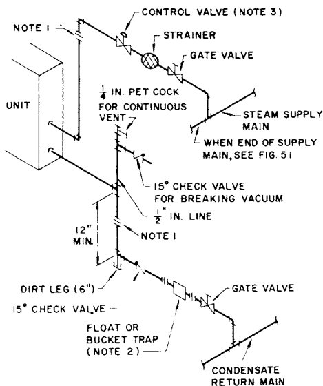
Fig 15-48. High or medium pressure coil piping
