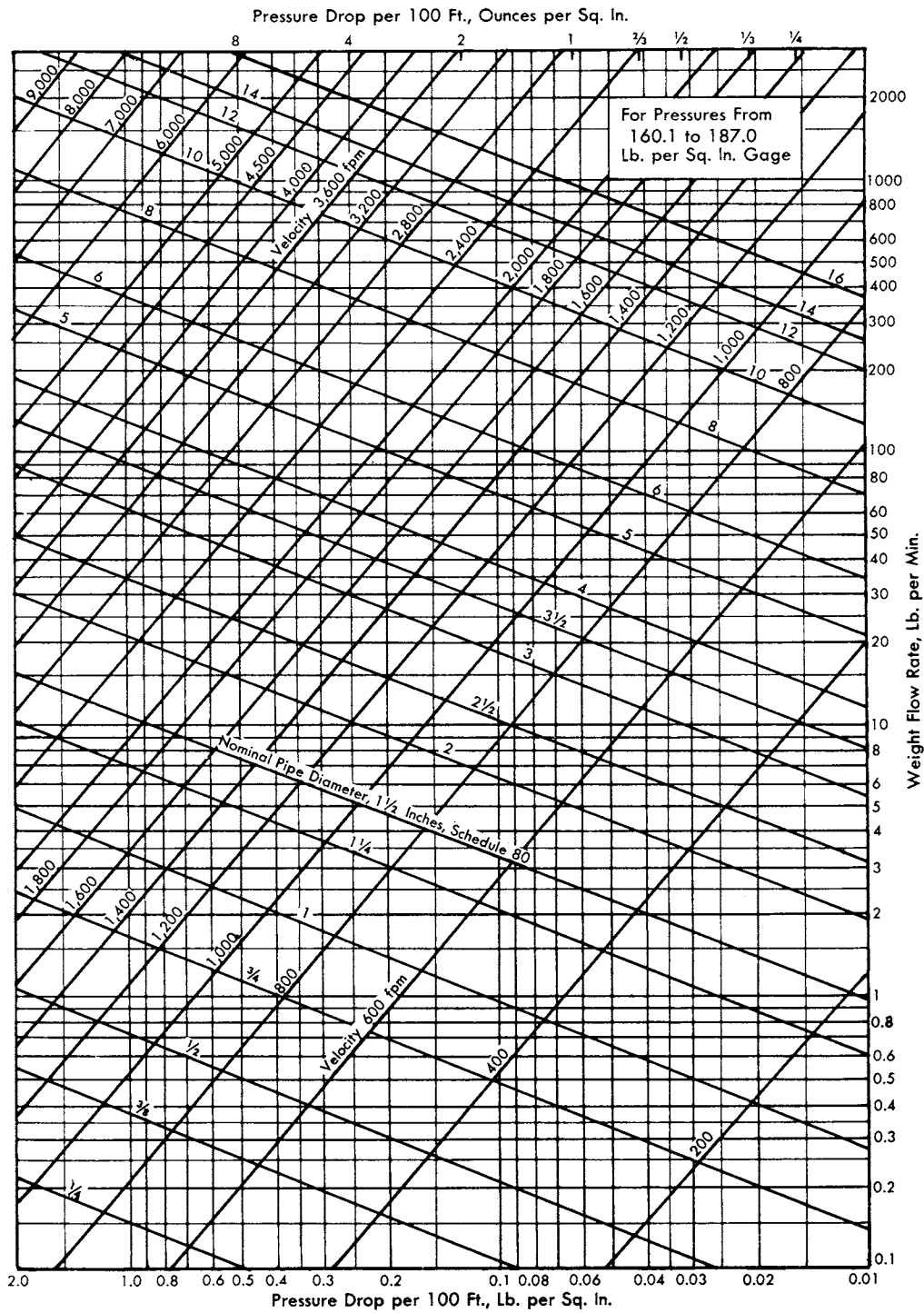
Fig 9-32. For pressure from 160.1 to 187.0 psig
