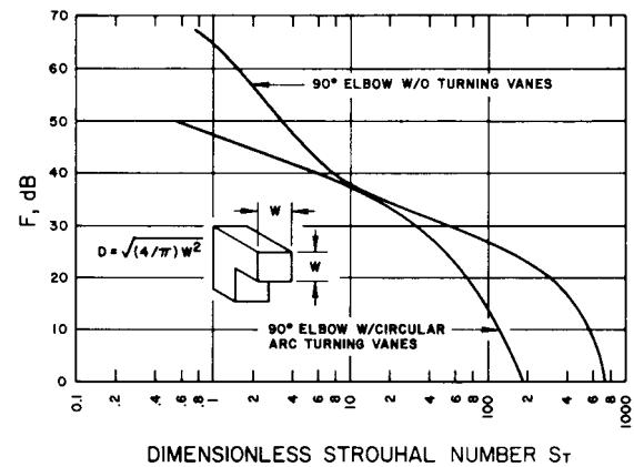
Fig 16-15. Spectrum function F for square cross section 90° elbow
