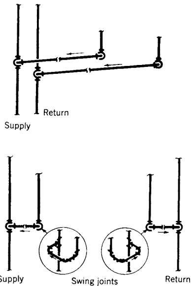
Fig 15-29. Runout connections from main to heating units
