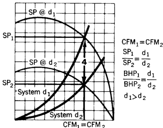
Fig 14-12. Fan law no. 4—effect of density change (constant volume)
