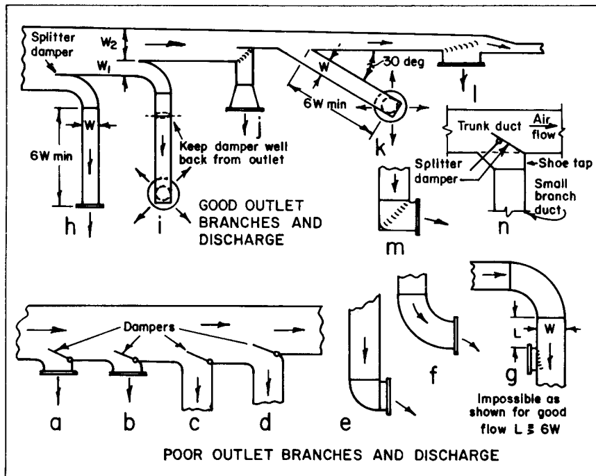
Fig 14-63. Outlet branches and discharge
