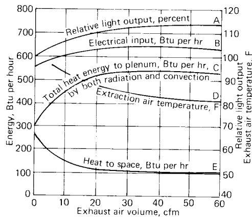
Fig 13-54. Manufacturer's data on heat distribution for a typical four lamp troffer
