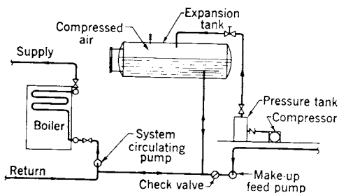
Fig 15-110. Method of pressurizing HTW system by air
