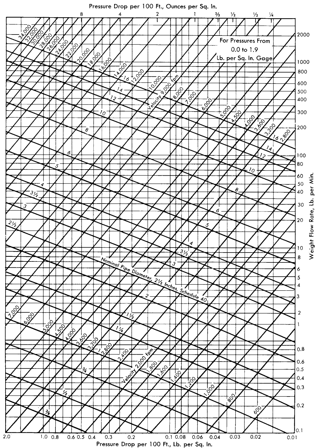
Fig 9-15. For pressure from 0.0 to 1.99 lb/inch 2 gage
