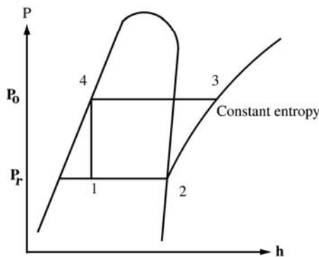
Fig 1-5b. Practical refrigeration cycle in P-h coordinates
