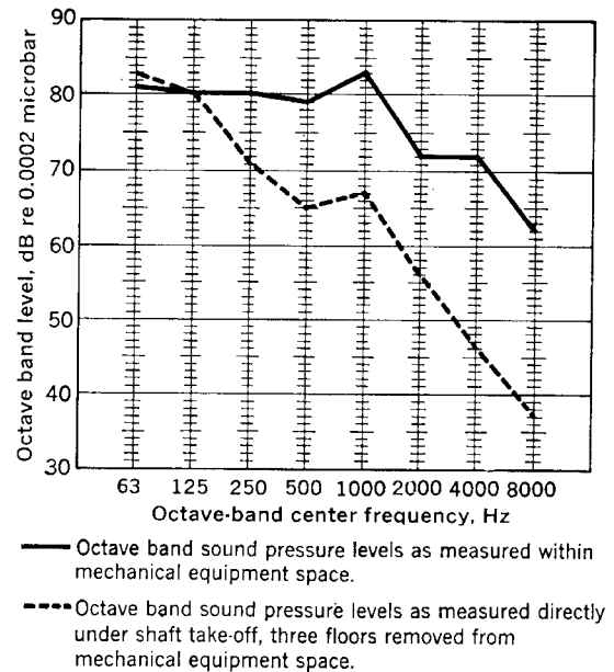
Fig 16-31. Noise band in first octave band is greater in tenant space
