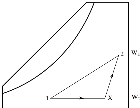
Fig 3-9. Psychrometric diagram of heating with humidification process
