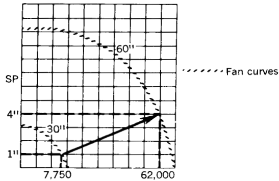
Fig 14-17. Example no. 3—Fan law no. 3 (diameter change)
