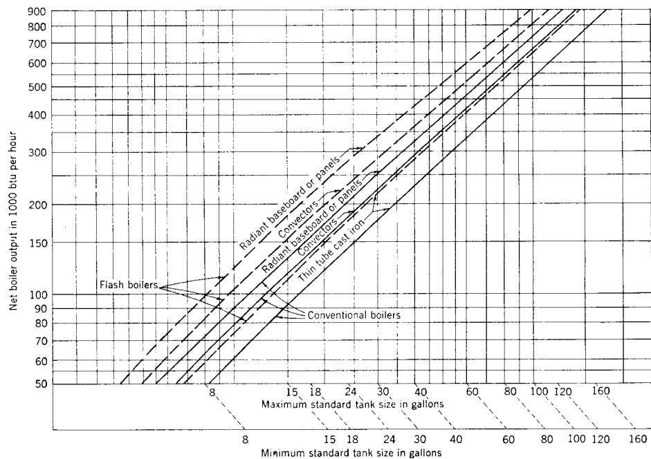
Fig 15-108. Minimum standard tank size in gallons
