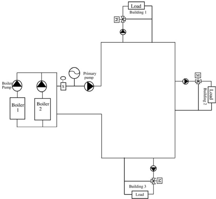
Fig 10-3. Primary system with constant speed heating system pump for multiple buildings
