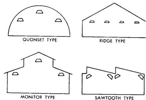
Fig 15-150. Building construction determines mounting arrangement
