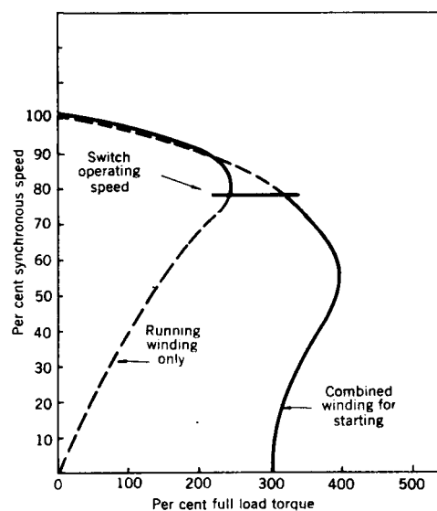
Fig 17-5a. Speed torque curve for a capacitor start motor
