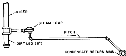
Fig 15-45. Riser dripped to dry return
