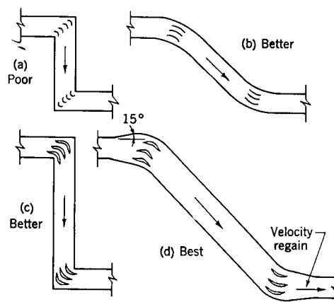
Fig 14-71. Air stream turns between successive fittings
