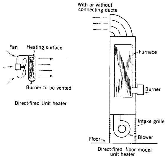
Fig 15-124. Allied version of forced air furnaces
