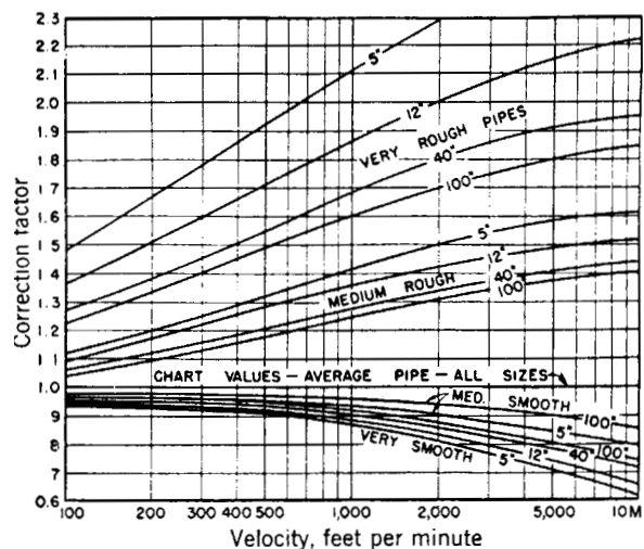
Fig 14-57. Correction factors for pipe roughness, to be applied to values read from Figs. 14-58a, and 14-58b.
