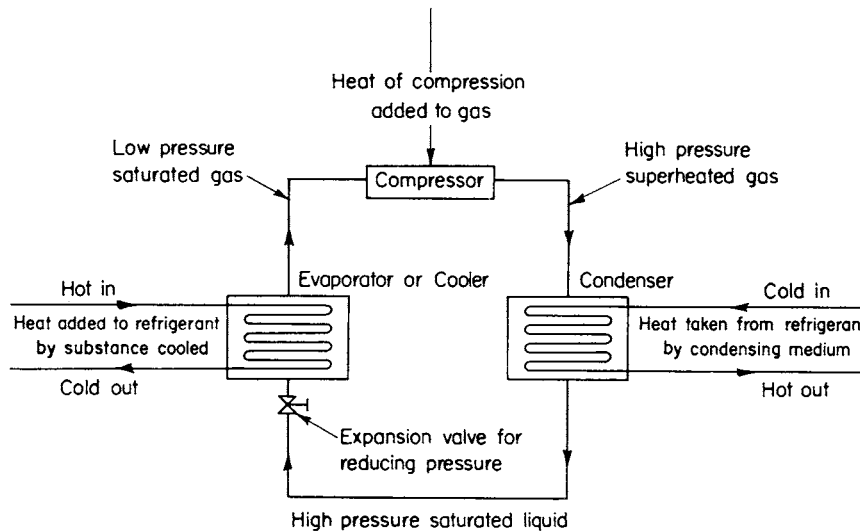
Fig 13-68. Schematic of refrigerant flow in a heat pump system for heating and cooling
