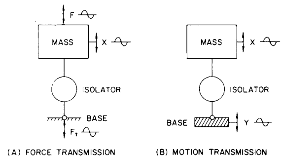
Fig 16-5. Single degree freedom vibration isolation system
