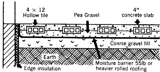
Fig 15-135d. One form of warm air floor panel heating
