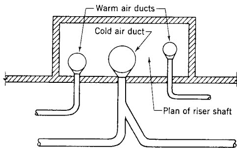
Fig 16-42. Typical duct connections to risers to avoid crossovers
