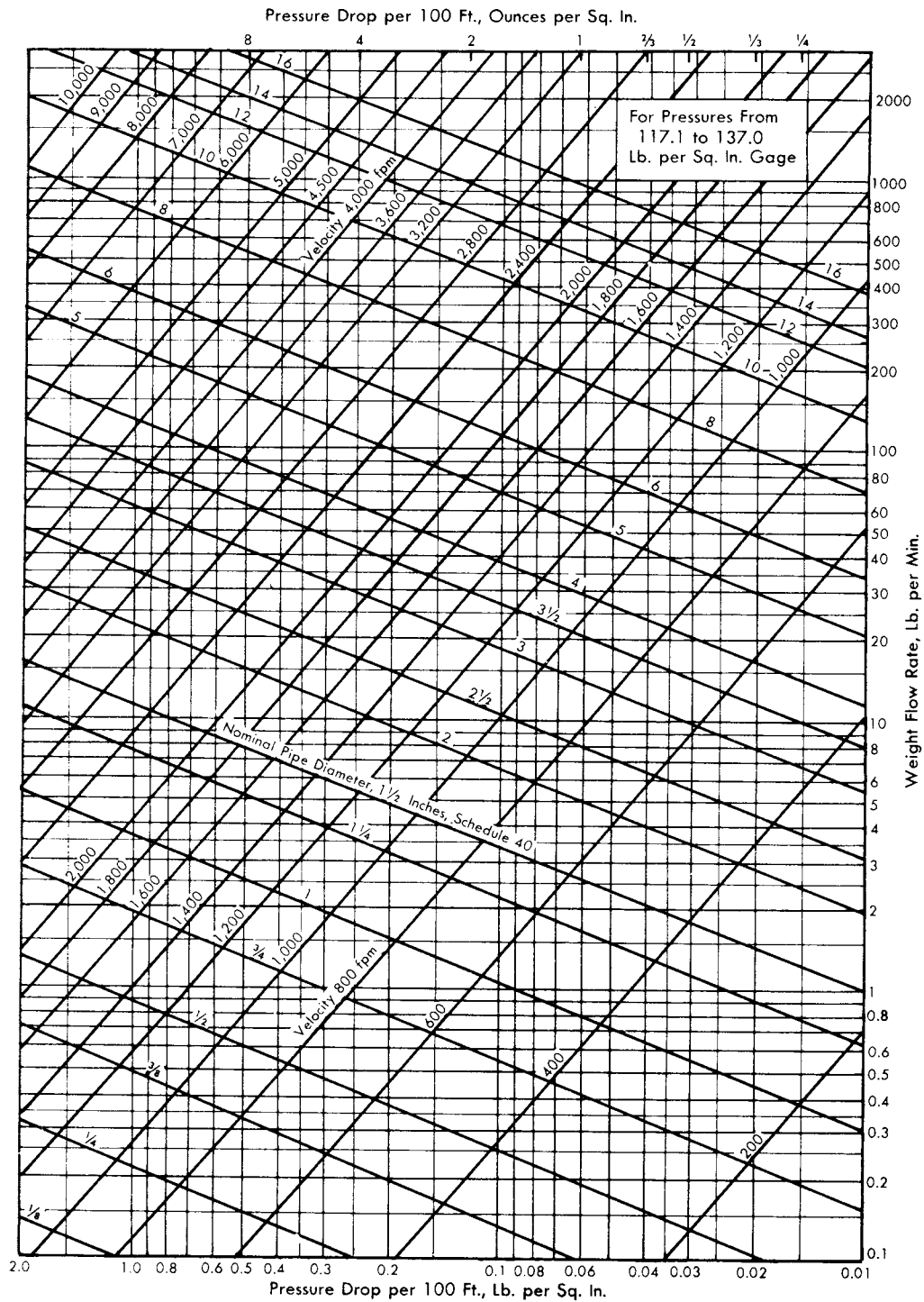
Fig 9-30. For pressure from 117.1 to 137.0 psig
