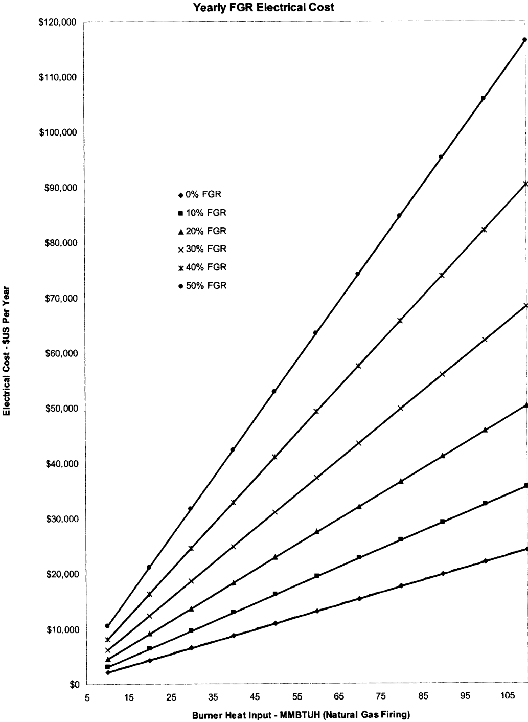
Fig 12-25. Induced combustion Air/FGR mixture electrical cost
