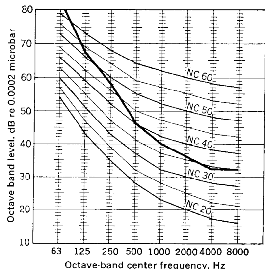
Fig 16-32. Typical curve of high velocity air distribution system generated noise
