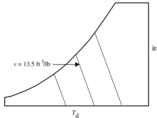
Fig 2-4c. Lines of constant specific volume v on the psychrometric chart
