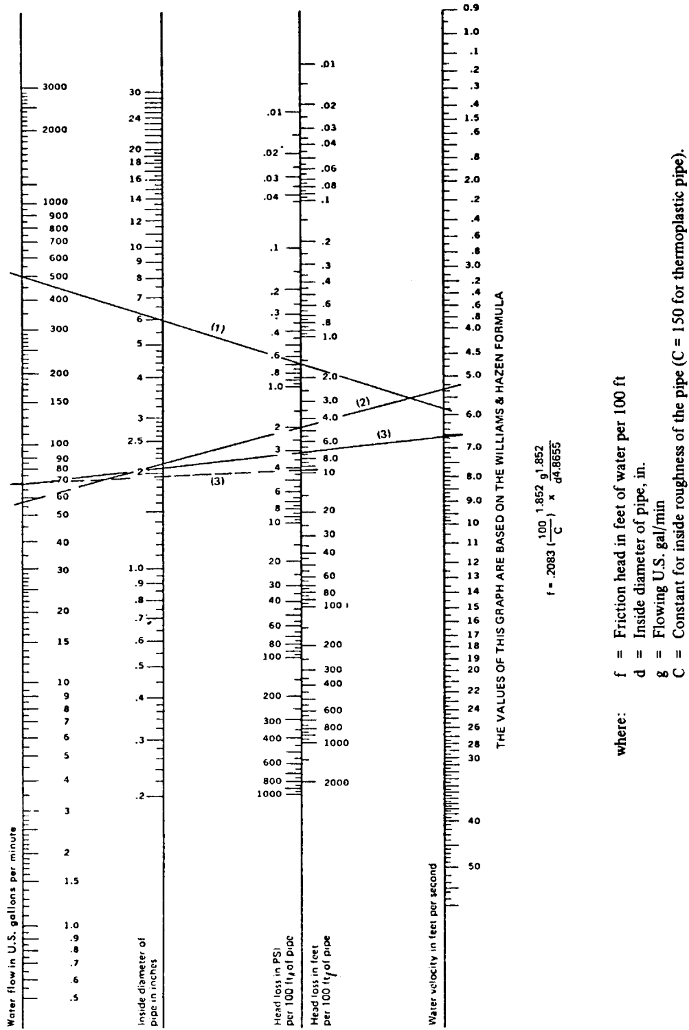
Fig 9-40. Flow loss characteristics of water flow through rigid plastic pipe
