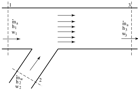
Fig 3-10. Adiabatic mixing of two streams process
