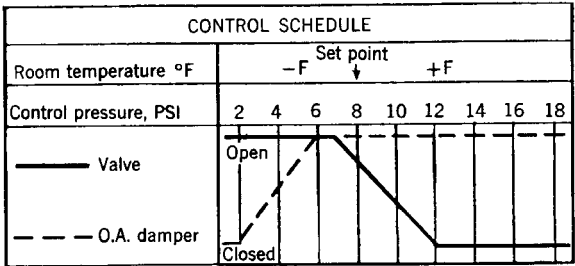
Fig 13-131. Unit ventilator using hot water
