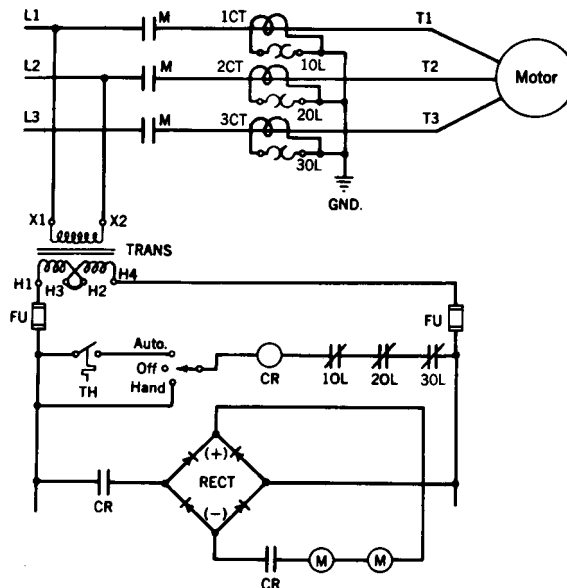
Fig 17-13. Full voltage, size 6, 3-phase, magnetic starter; 2-wire control (low voltage release)
