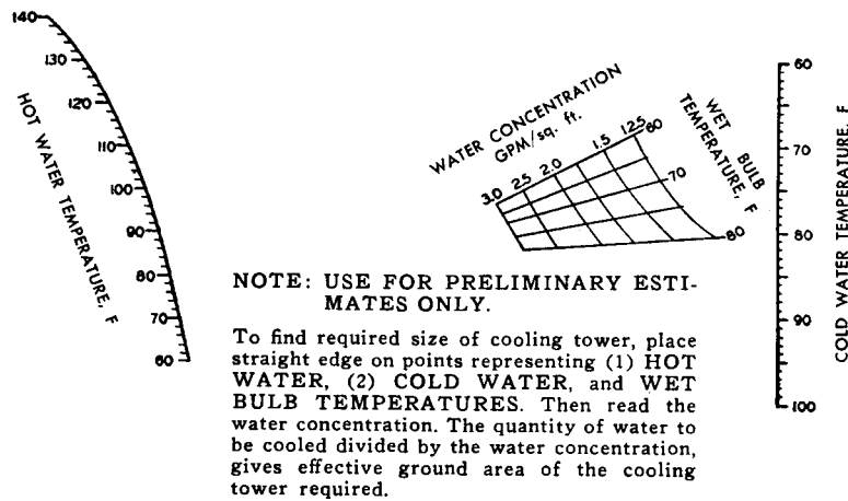
Fig 13-147. Sizing chart for mechanical draft cooling towers
