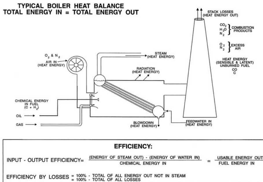
Fig 12-4. Typical boiler heat balance
