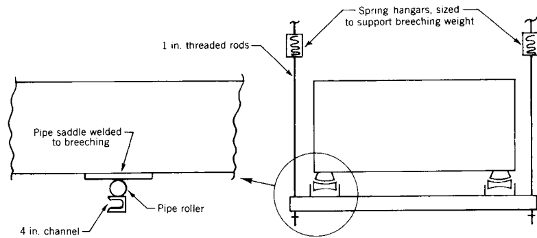
Fig 14-86. Breaching hanger supports
