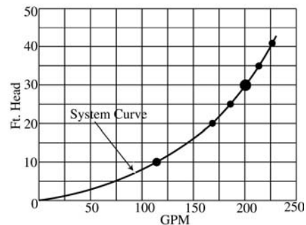
Fig 10-31. Paralleled pump system curve
