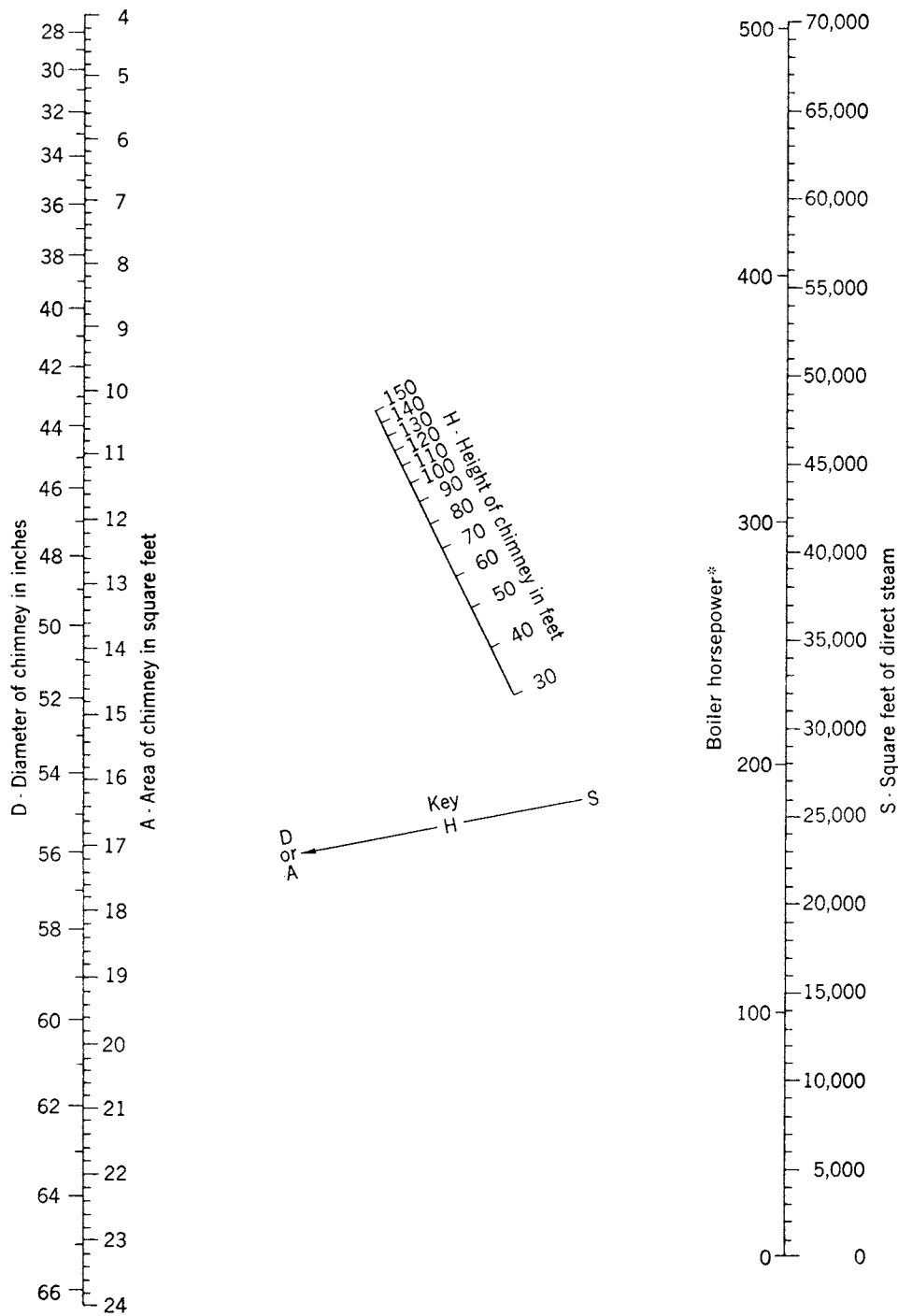
Fig 14-88. Breeching design selection
