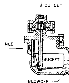
Fig 15-76. Upright bucket trap
