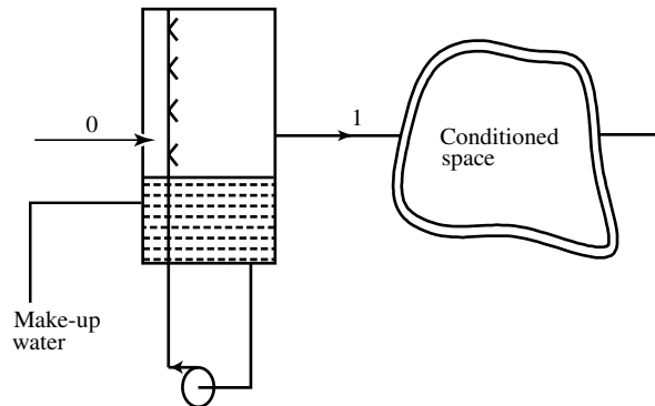
Fig 3-12. Evaporative cooling system
