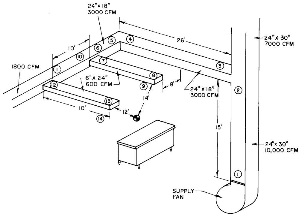
Fig 16-20. Ducted air supply system
