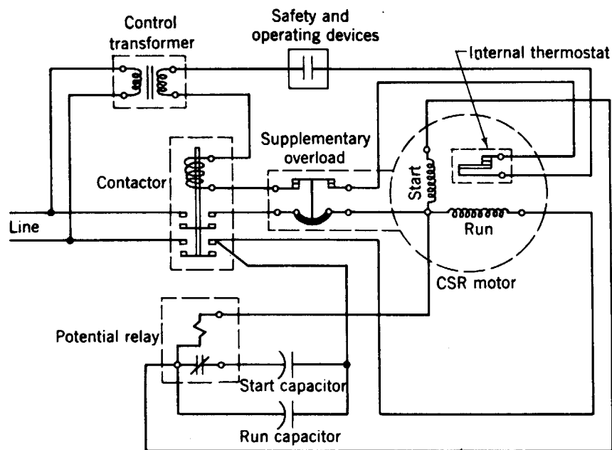
Fig 17-10. Capacitor start capacitor run motor with internal protection and potential relay
