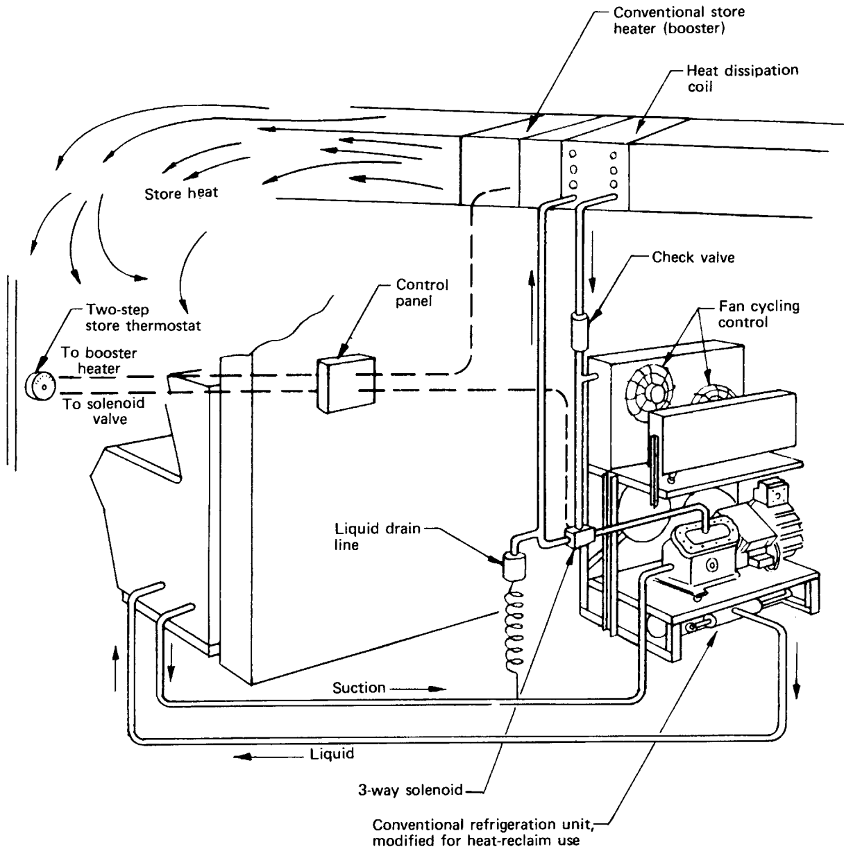
Fig 13-67. Diagram of heat recovery system using rotary heat exchanger
