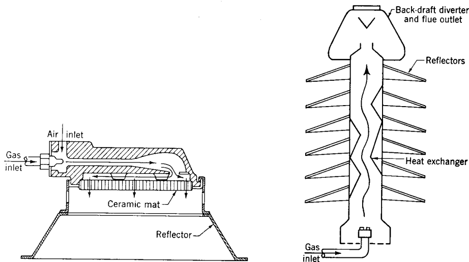
Fig 15-149. Two types of gas fired radiant (infrared) heaters
