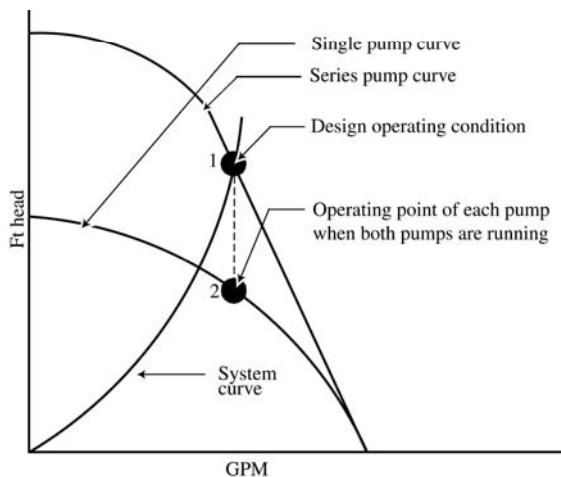
Fig 10-39. Series pump system operation
