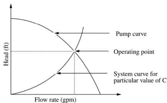
Fig 10-24. System characteristic curves
