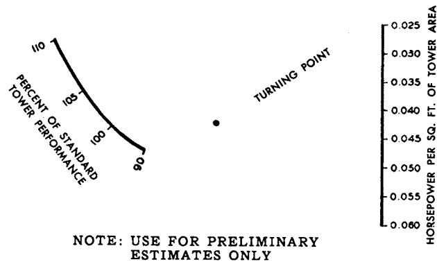
Fig 13-147. Sizing chart for mechanical draft cooling towers
