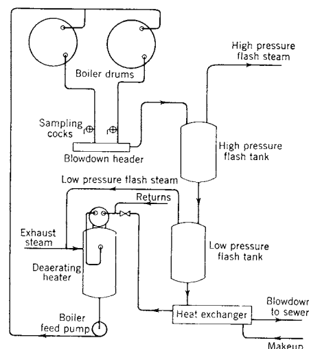
Fig 15-84. Flow diagram for two-stage flash system based on heat in continuous boiler blowdown
