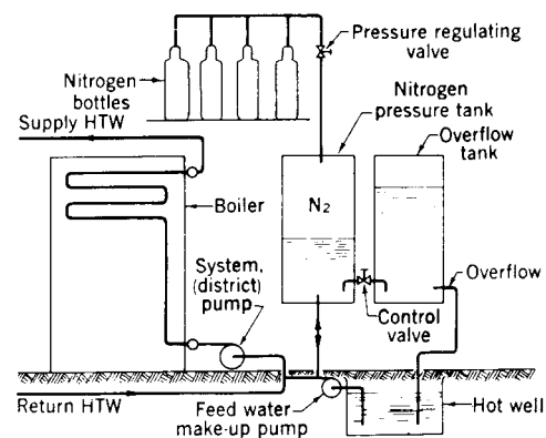
Fig 15-112. Nitrogen pressurization HTW system without overhead tank
