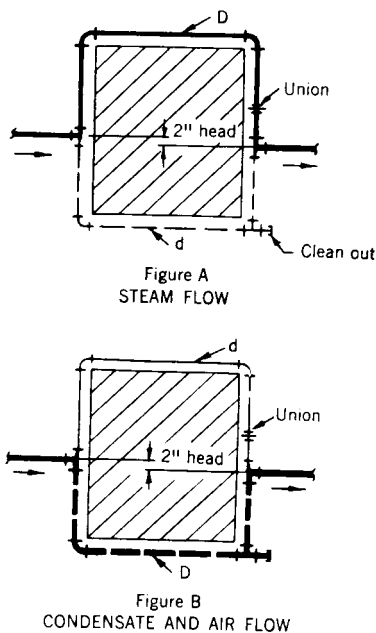
Fig 15-33. Detail of piping around obstacle
