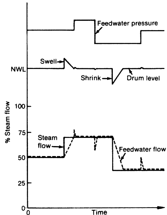
Fig 12-14. Performance of three element feedwater control (effect of feedwater pressure variations)
