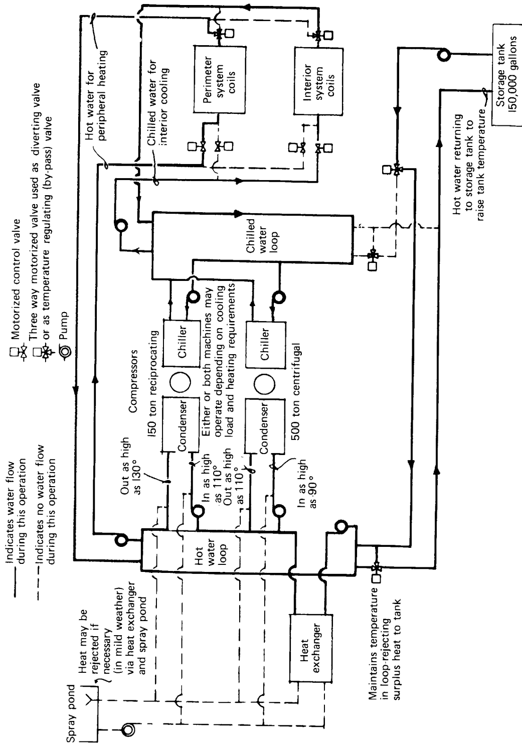
Fig 13-64. Piping system for heat recovery and storage system
