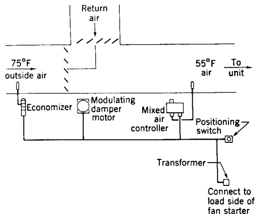
Fig 13-36. Outside air controlled from mixed air temperature
