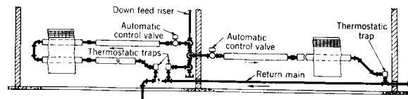
Fig 15-10. Fin tube heater piping connections
