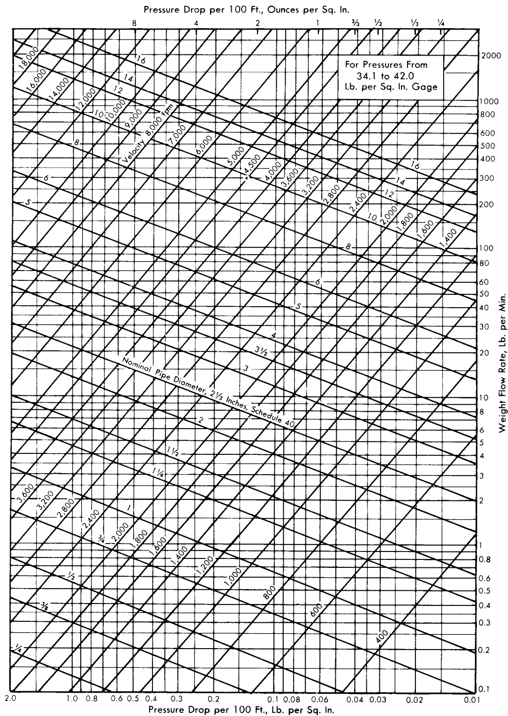
Fig 9-23. For pressure from 34.1 to 42.0 psig
