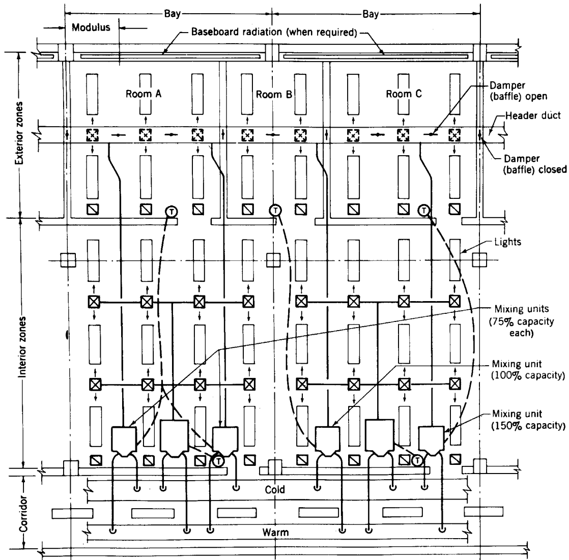
Fig 13-111. Modular arrangement for overhead dual duct system, Scheme C
