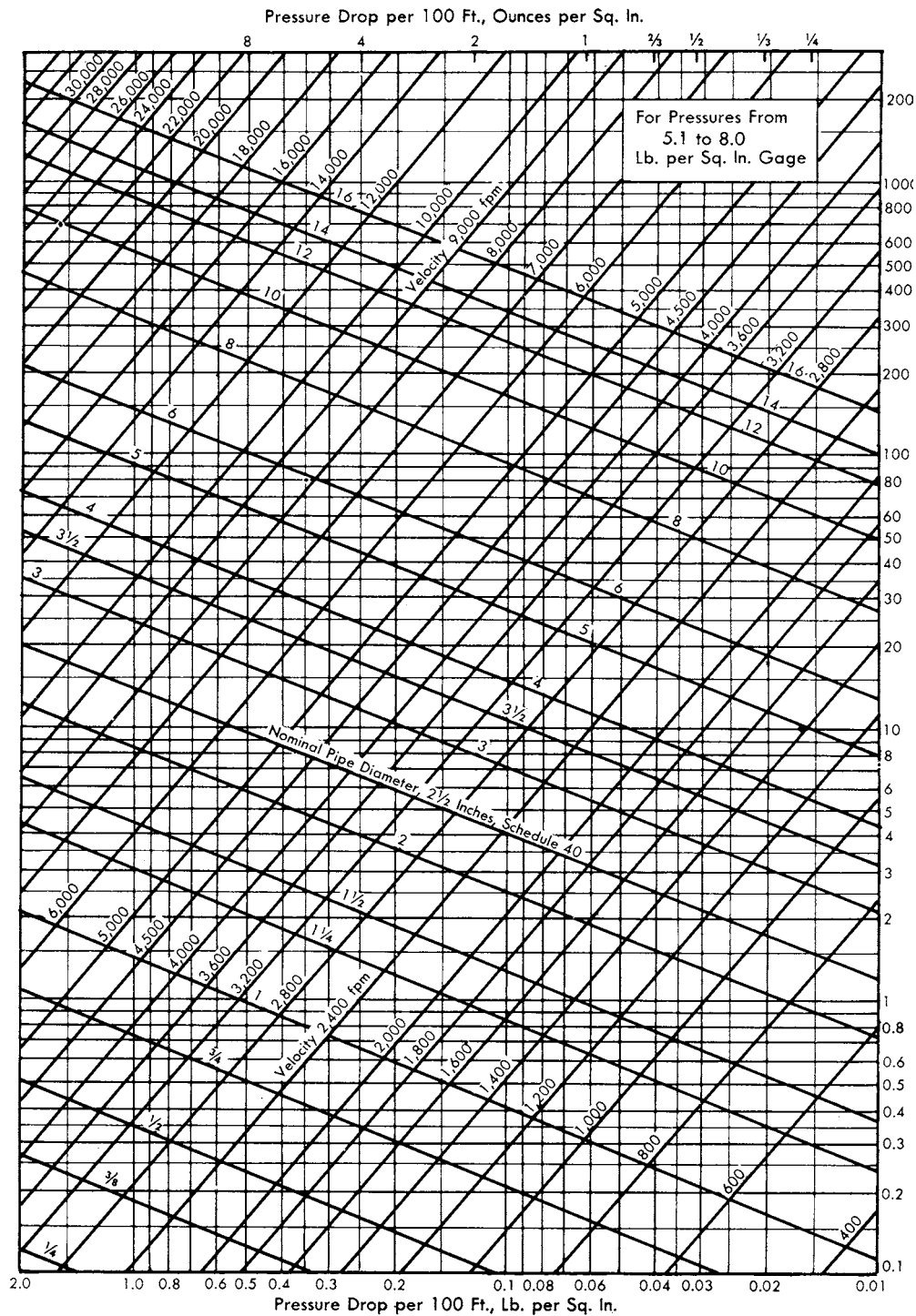
Fig 9-17. For pressure from 5.1 to 8.0 psig
