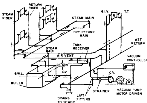
Fig 15-66. Mechanical vacuum system
