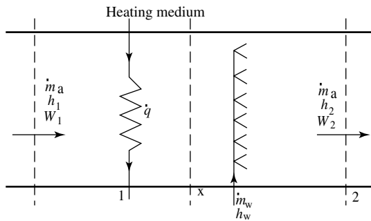
Fig 3-8. Schematic of heating with humidification process
