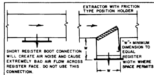
Fig 14-65. Top register connection to trunk duct
