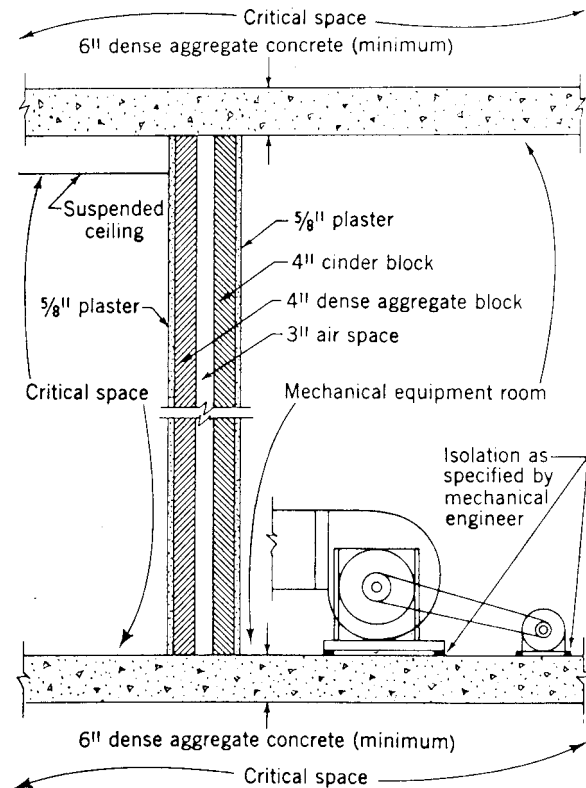
Fig 16-4. Suggested Partition Construction Between Mechanical Equipment Room and Critical Spaces
