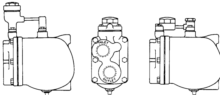
Fig 15-152. Heavy duty double ported float thermostatic steam traps
