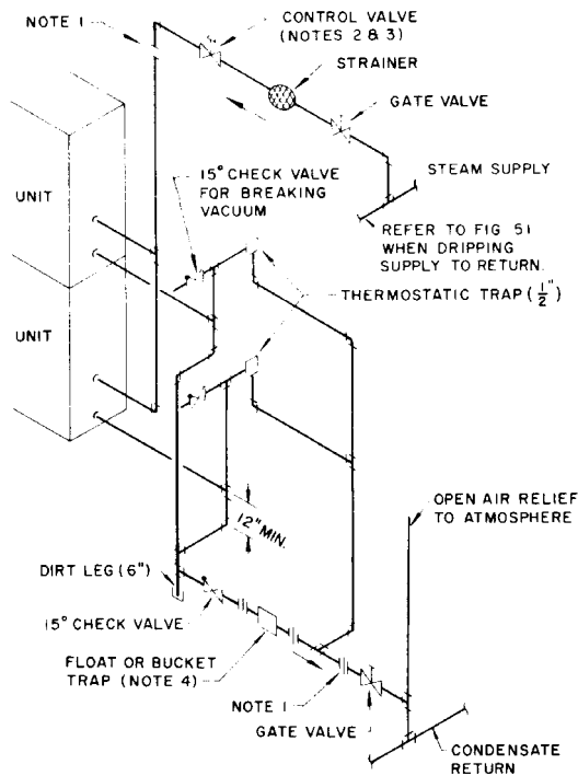
Fig 15-55. Multiple coil low pressure piping gravity return
