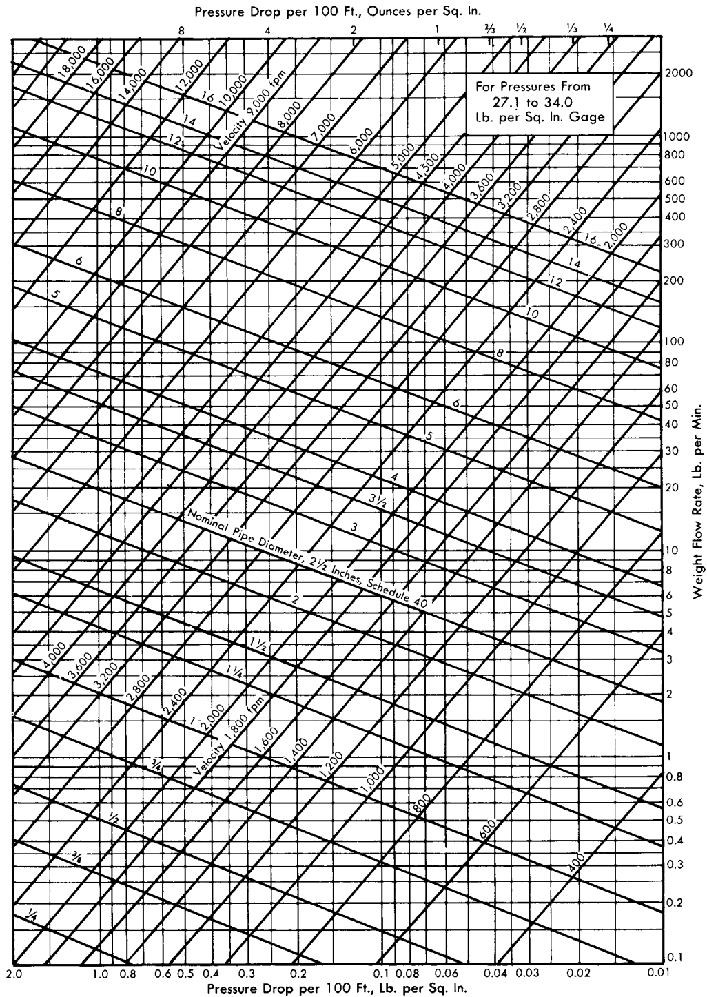
Fig 9-22. For pressure from 27.1 to 34.0 psig
