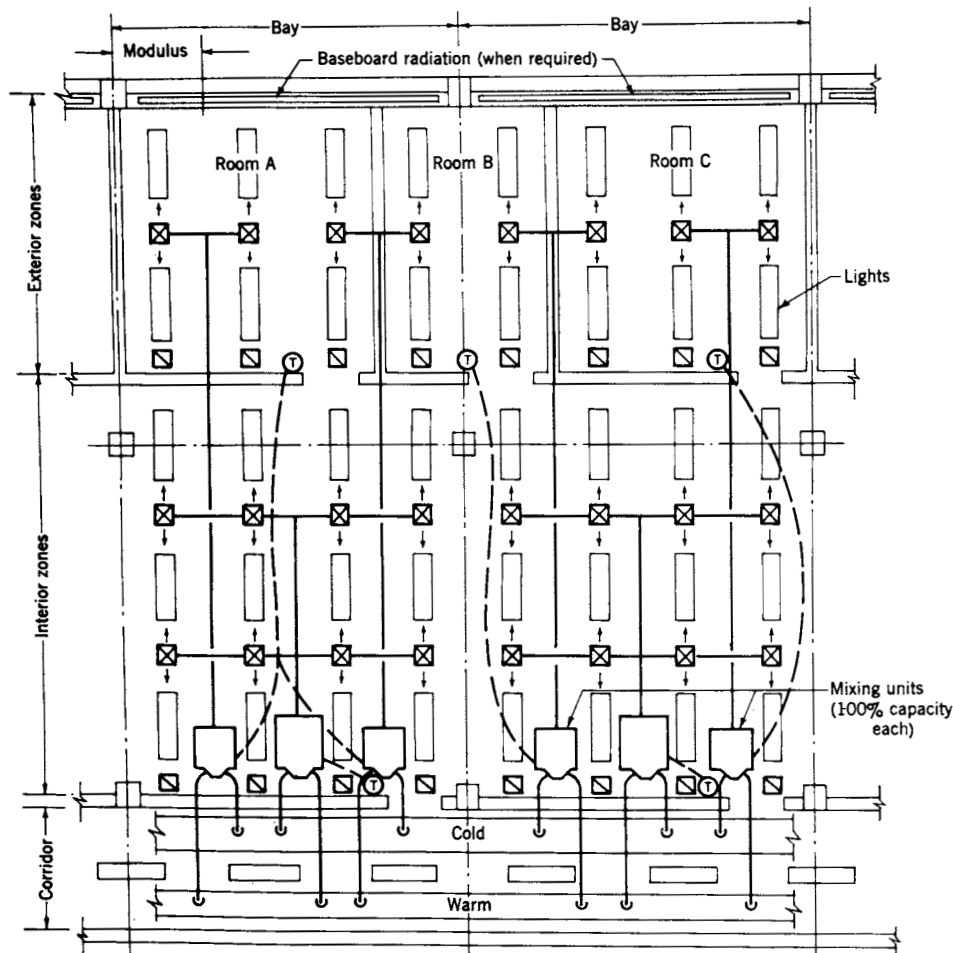
Fig 13-112. Modular arrangement for overhead dual duct system, Scheme D
