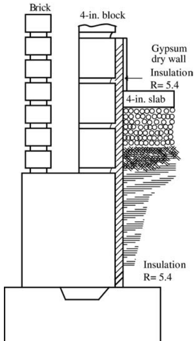
Fig 6-5. 8-inch block wall slab on grade foundation insulation
