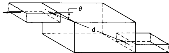
Fig 16-14. Diagram of a sound absorbing plenum
