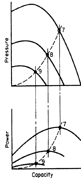
Fig 12-24. Speed control
