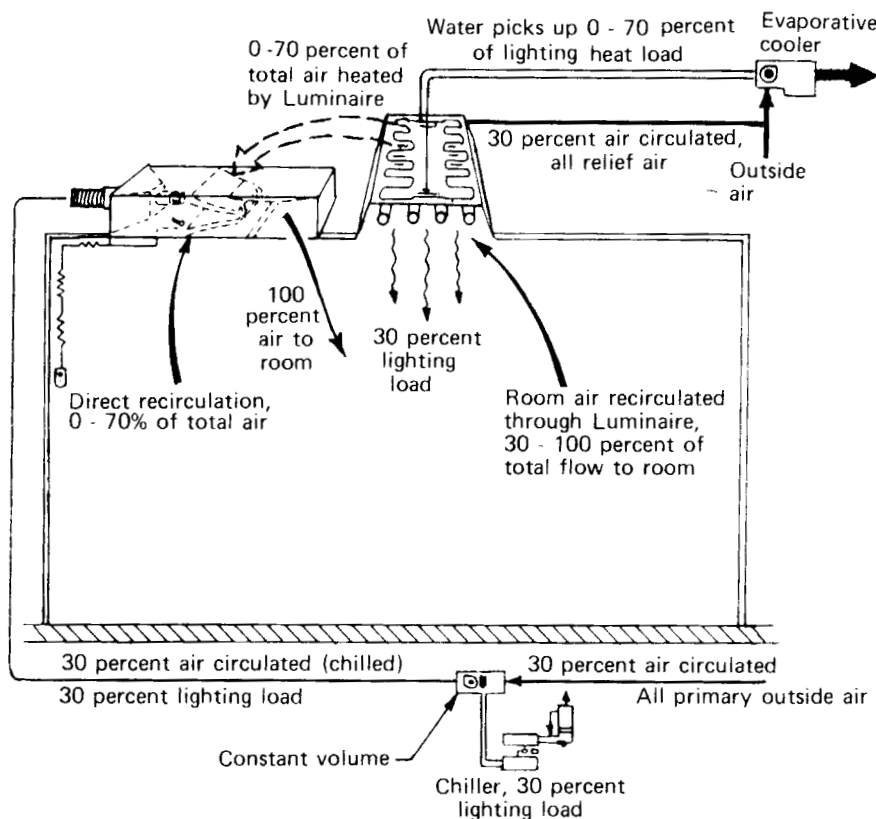
Fig 13-57. Patterns of heat flow and water flow for system
