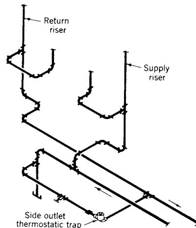
Fig 15-26. End of branch main drip with thermostatic trap
