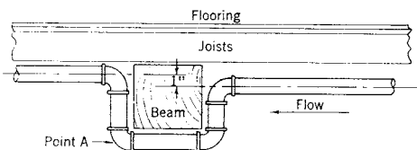
Fig 15-100. Method of crossing a beam
