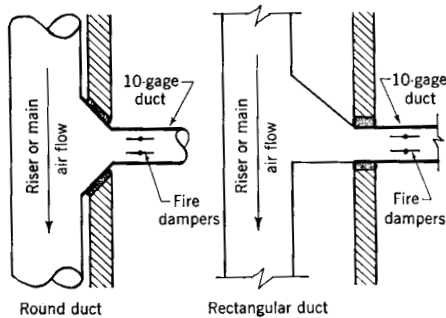
Fig 14-73. Shaft take-off space is inadequate; use extra heavy duct
