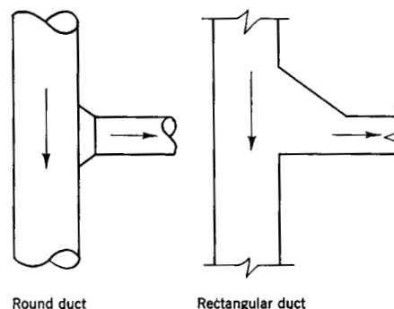
Fig 14-72. Tap off from riser
