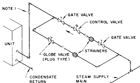
Fig 15-52. Bypass with manual control
