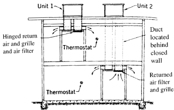
Fig 13-22. Unitary packages on roof ducted to first and second floor
