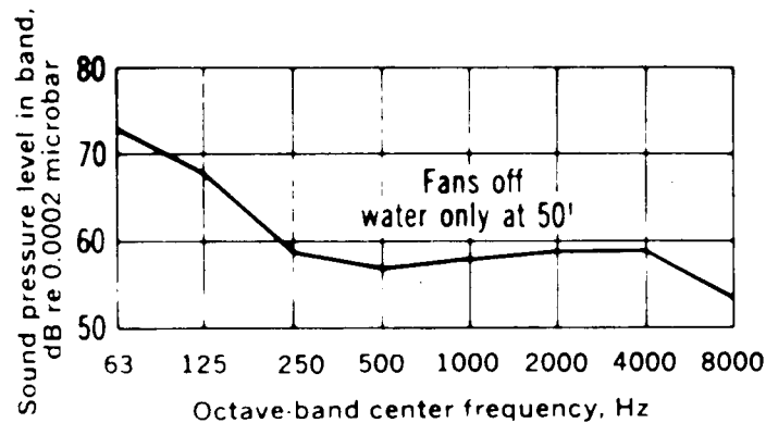
Fig 16-23. Tower water noise spectrum
