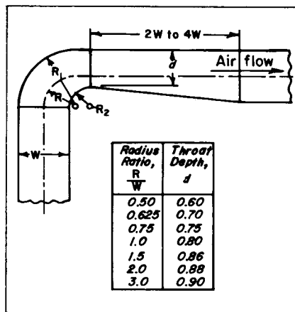
Fig 14-64. Venturi elbow
