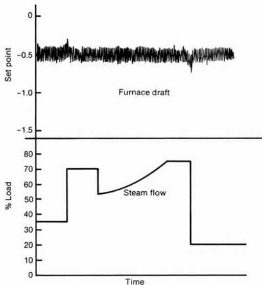
Fig 12-19. Furnace draft control (feed forward and feedback control of induced draft fan)
