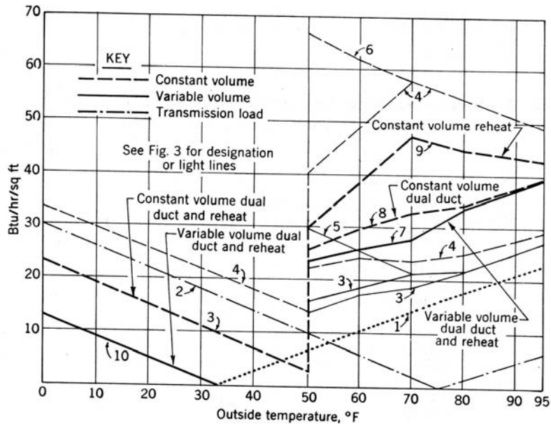
Fig 13-46. Energy requirement in Btu conditions-full sun load southern exposure
