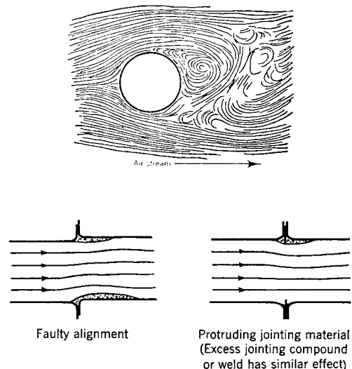
Fig 16-36. Turbulence due to round obstruction, duct misalignment and protruding edge in air stream
