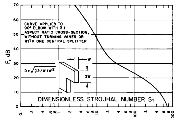
Fig 16-16. Spectrum function F for regular cross section 90° elbow
