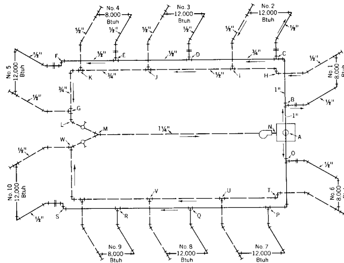
Fig 15-104. Layout for Two-pipe reversed return hot water heating system with forced circulation (For Example 8)
