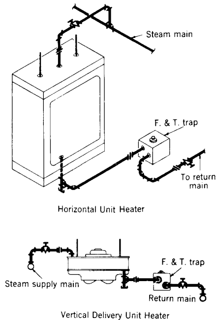
Fig 15-11. Unit heater piping details
