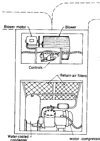
Fig 13-2. Vertical self contained air conditioned unit
