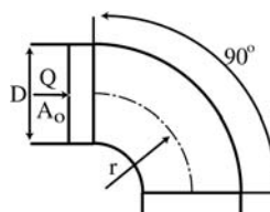
Die stamped 90° elbows
