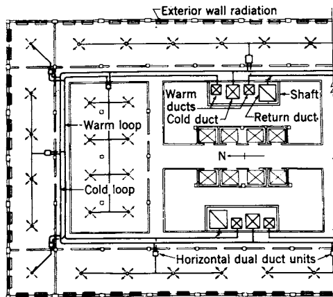
Fig 13-100. Typical office building dual duct layout with supplementary radiation at exterior wall with minimum number of zones
