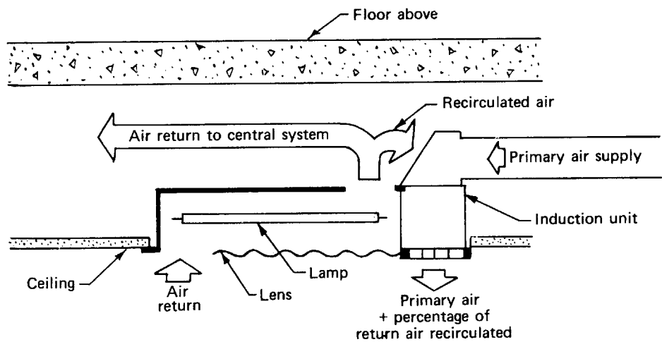
Fig 13-59. Air cooled luminaire application
