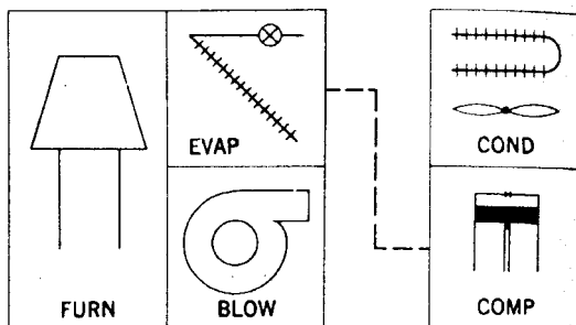
Fig 13-11. Split system year round air conditioner
