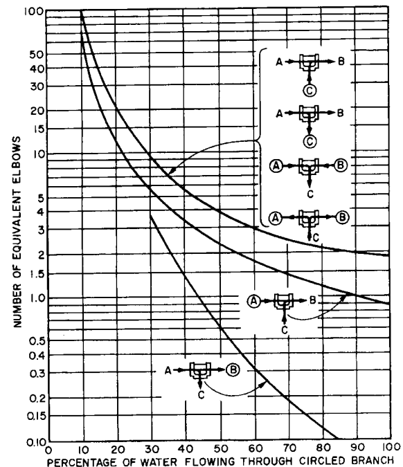
Fig 9-4. Elbow equivalents of tees at various flow conditions
