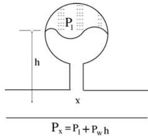
Fig 10-12. Closed tank air water interact
