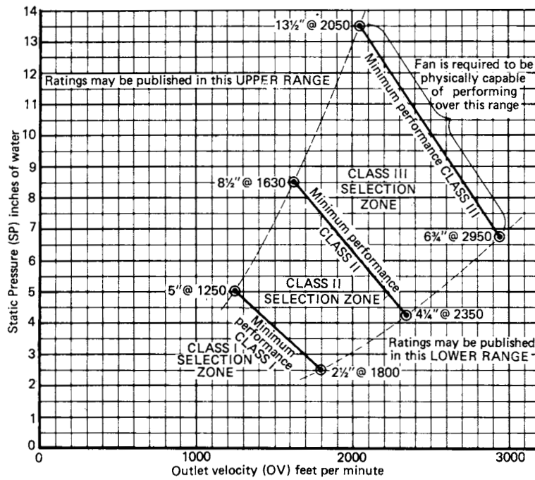
Fig 14-41. Operating limits for centrifugal fans tubular
