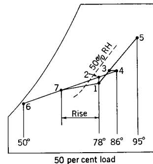
Fig 13-94. Psychrometric chart for dual duct system for Fig. 13-88 50% load
