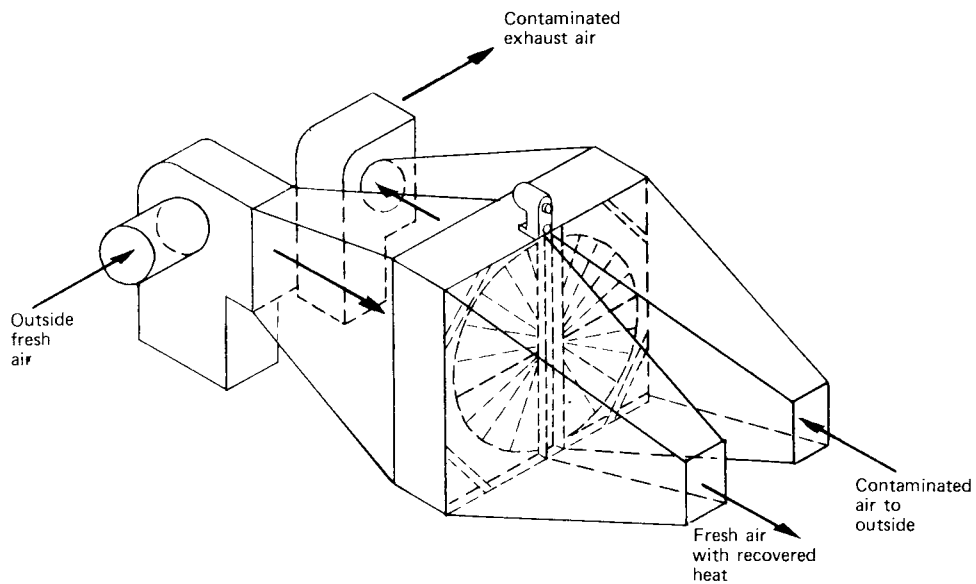
Fig 13-63. Diagram of regenerative heat recovery system
