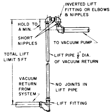
Fig 15-46. One step condensate lift
