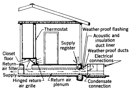
Fig 13-26. Ducts run through crawl space
