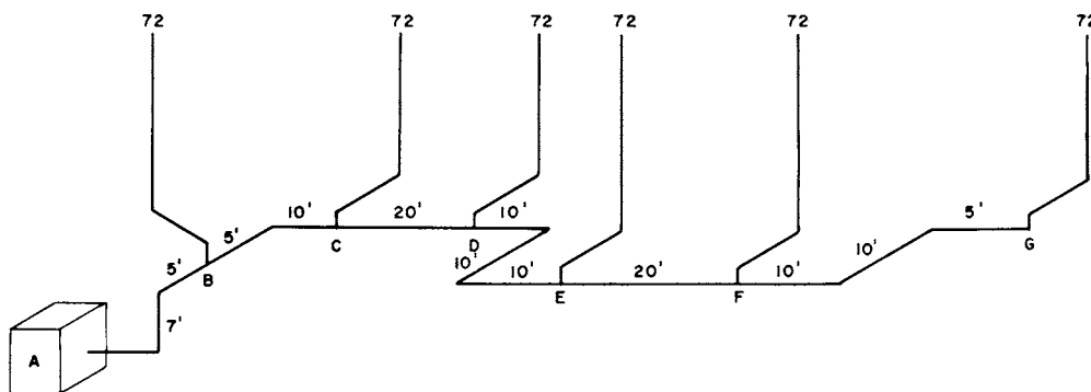
Fig 15-71. Low pressure vacuum return
