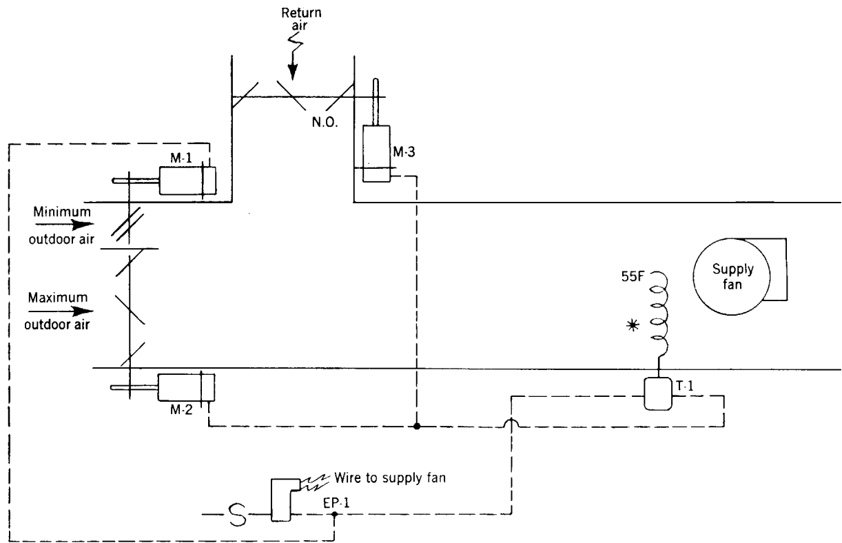
Fig 13-126. Mixed air control with minimum outside air
