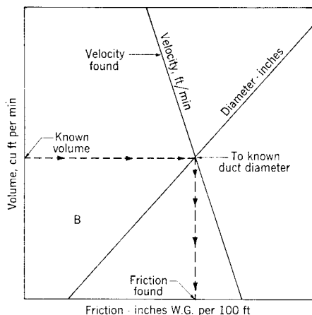
Fig 14-60b. Finding velocity and friction from known volume and diameter
