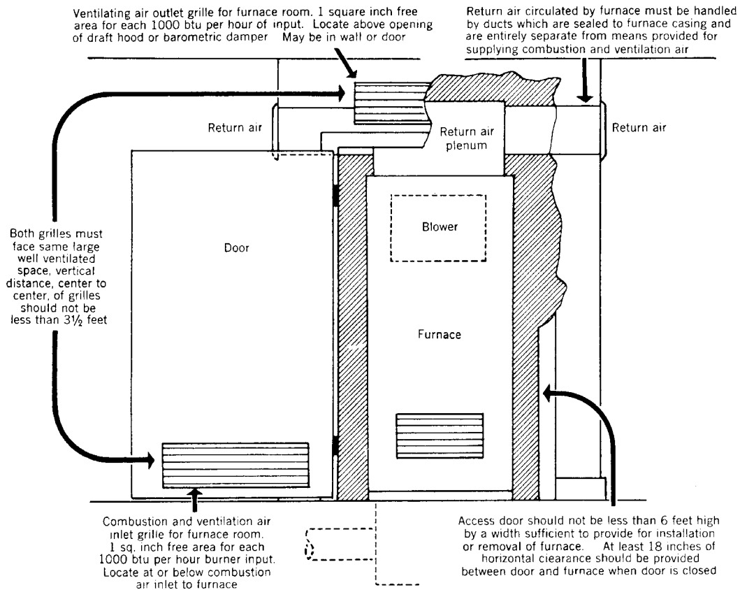
Fig 15-136b. Provisions for combustion and ventilation air for furnace closet
