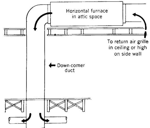
Fig 15-135f. Attic furnace installation leading to duct system in crawl space
