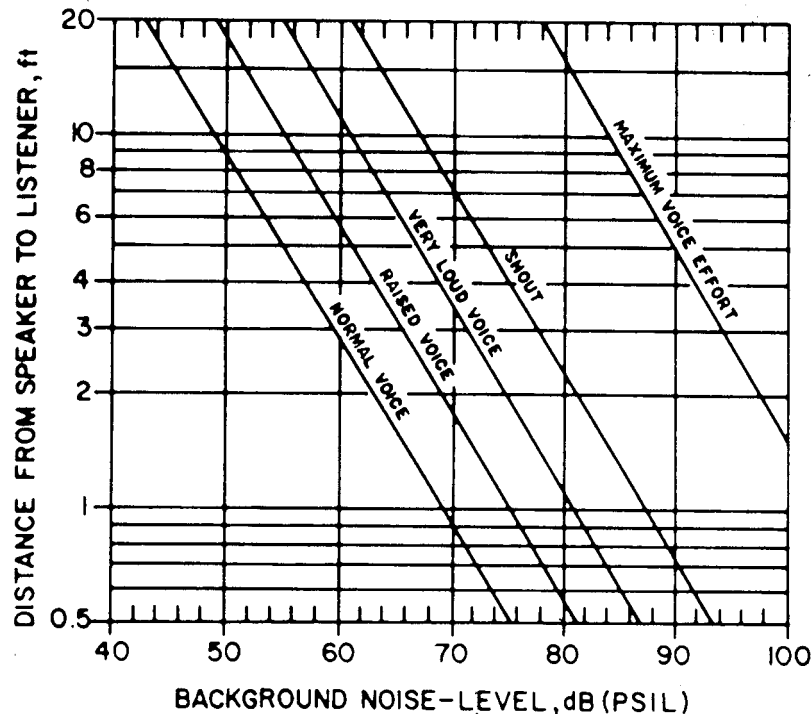
Fig 16-2. Relation of required Voice Effort for Communication in terms of PSIL and distance between Speaker and Listener
