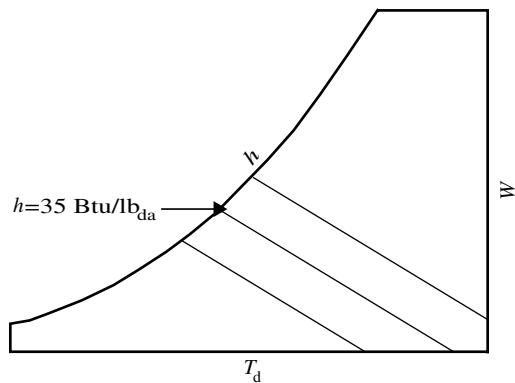
Fig 2-4f. Lines of constant enthalpy h on the psychrometric chart
