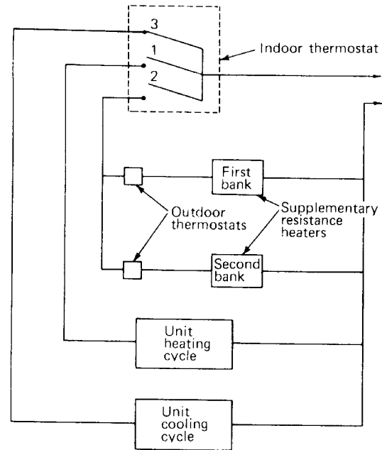
Fig 13-73. Control circuit for residential heat pump
