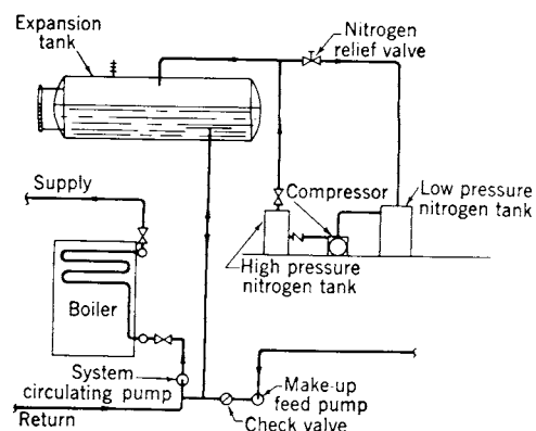
Fig 15-111. Insert gas pressurized htw system using nitrogen
