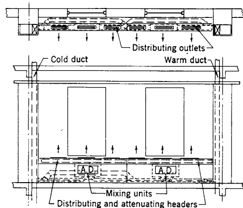
Fig 13-107. Arrangement for vertical under window dual duct units to units per riser
