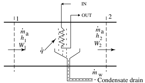
Fig 3-6. Schematic of cooling with dehumidifying process
