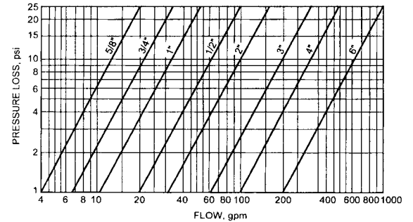
Fig 9-8. Pressure loss in disk type water meters
