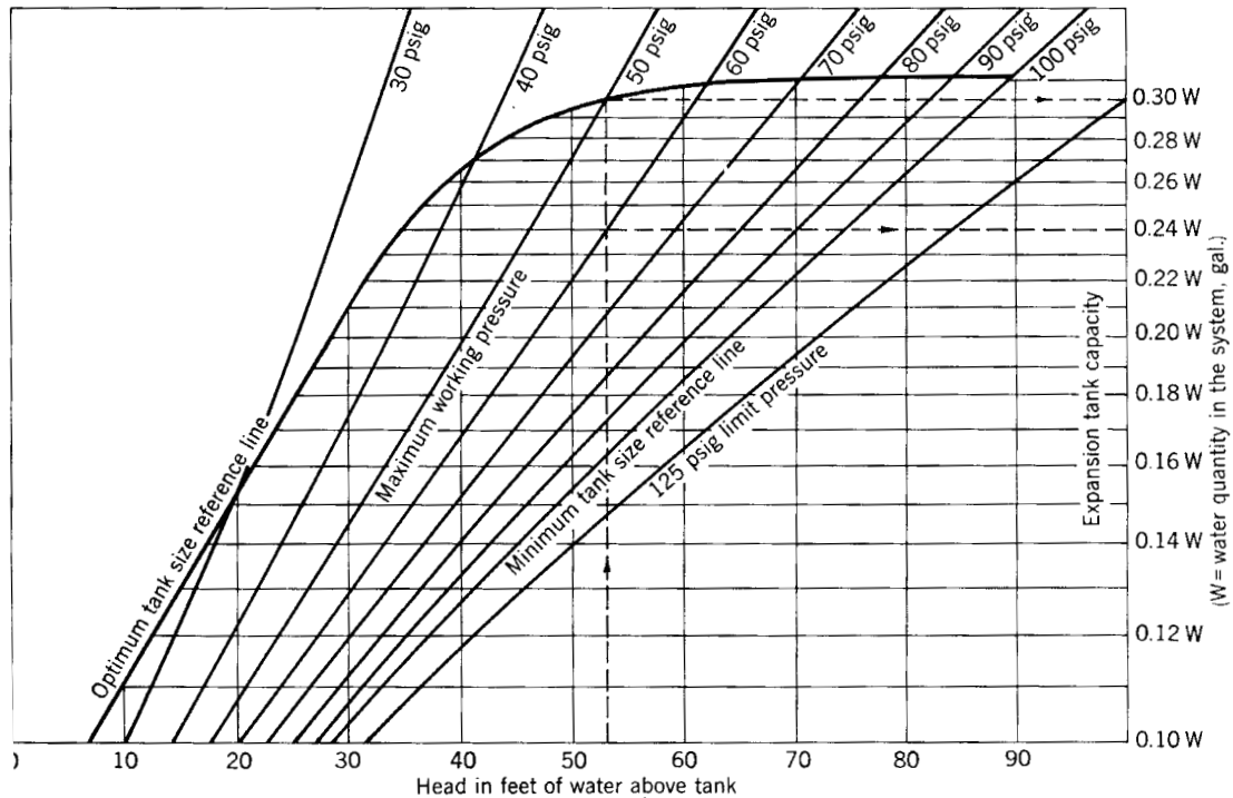
Fig 15-107. Head in feet of water above tank
