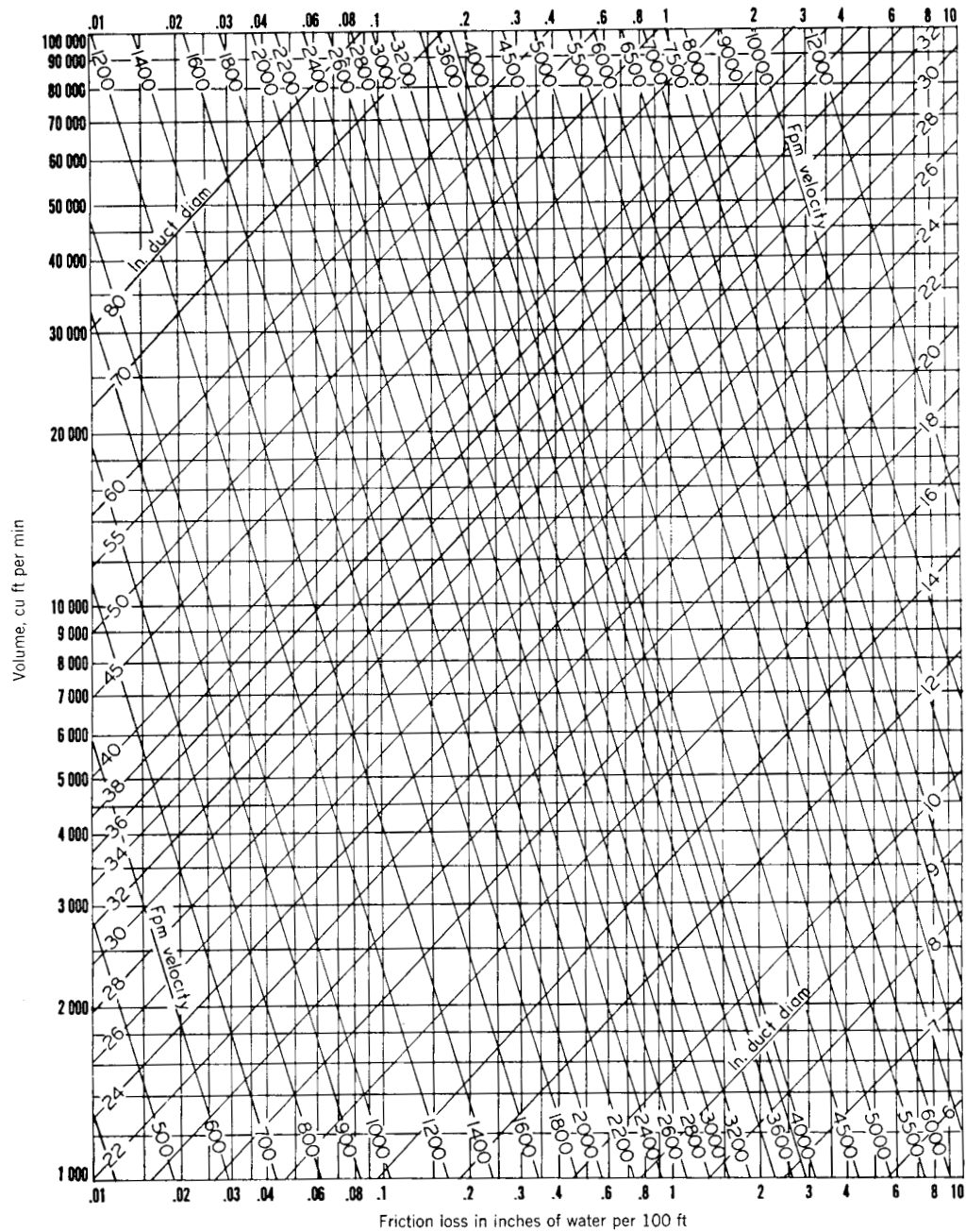
Fig 14-59b. Friction of air in straight aluminum ducts for volume of 1,000 to 100,000 cfm (Based on standard air of 0.075 lb/ft 3 density flowing through clean round galvanized ducts having approximately 40 joints per 100 ft)
