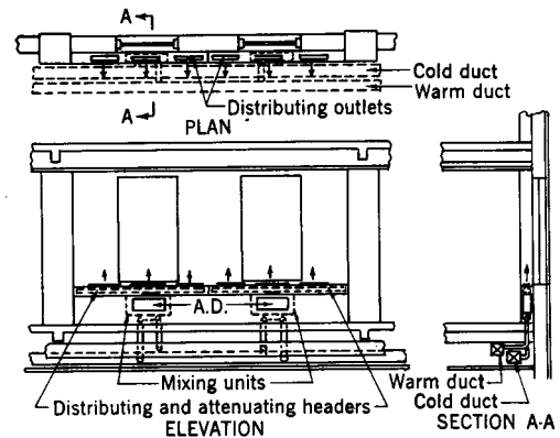
Fig 13-105. Arrangement for vertical under window dual duct units two units per riser
