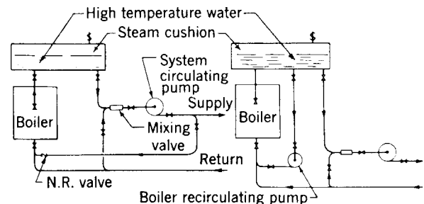
Fig 15-118. HTW system with boiler recirculating
