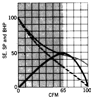
Fig 14-39. Characteristic curves for propeller fans
