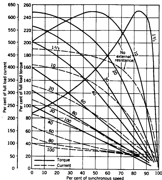
Fig 17-6. Family of speed torque curves and speed current curves for a single wound rotor induction motor
