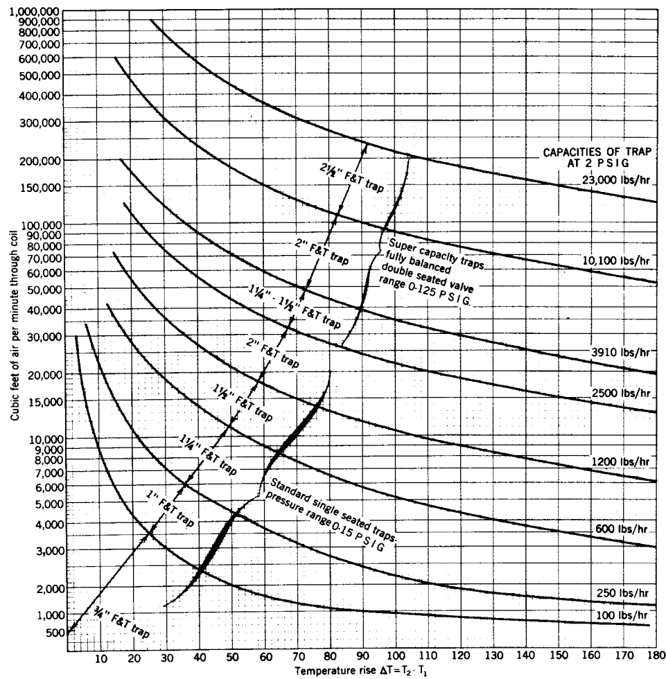
Fig 15-155. Sizing of steam traps
