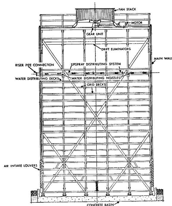
Fig 13-146. Cross section of mechanical draft cooling tower
