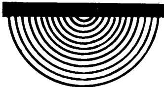
Fig 16-9b. Uniform hemispherical radiation, Q = 2 single reflecting surfaces
