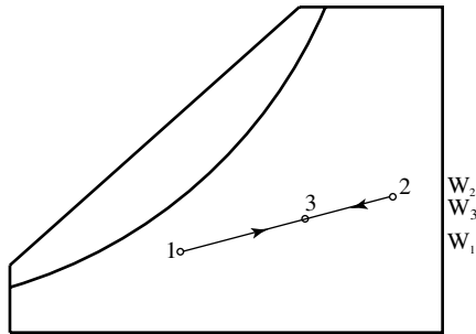
Fig 3-11. Psychrometric diagram of adiabatic mixing process
