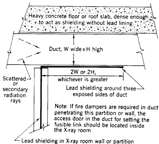
Fig 16-43. Elevation of section through X-ray room
