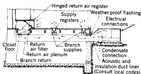
Fig 13-27. Unit in slab where building has basement
