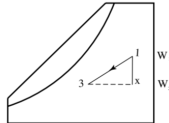
Fig 3-7. Psychrometric diagram of cooling with dehumidifying process
