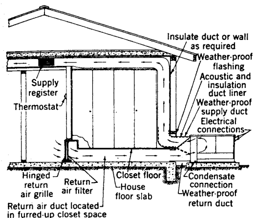
Fig 13-25. Self-contained unit mounted on slab
