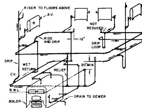
Fig 15-62. One pipe gravity system with dripped risers
