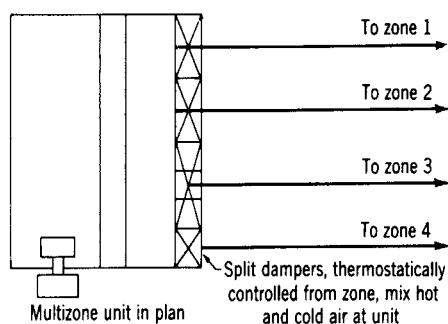
Fig 13-32. Multizone package can serve multiple zones
