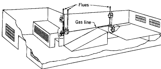
Fig 15-156. Typical installation of suspended propeller type heaters
