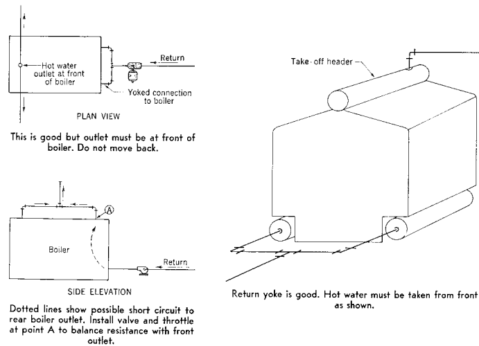
Fig 15-103. Connecting a return line to boiler
