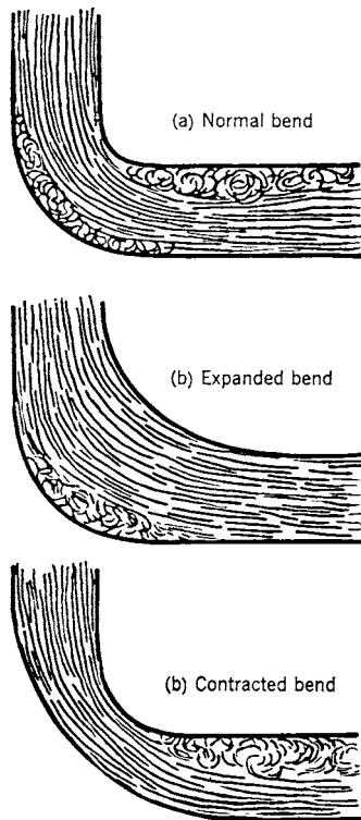
Fig 16-38. Air pattern in bends of various patterns
