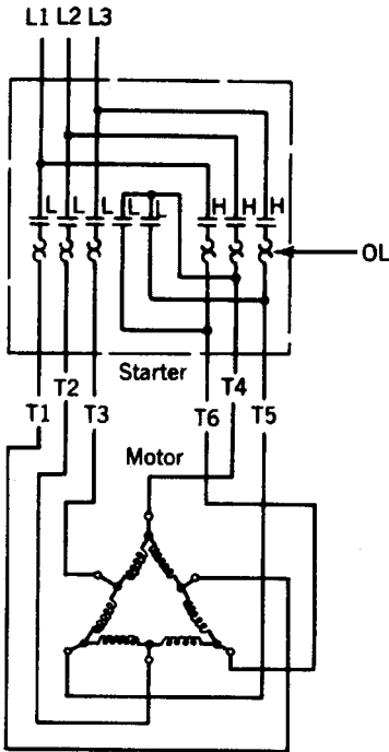
Two speed, single winding (consequent pole) constant horsepower
