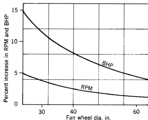
Fig 14-49. Inlet guide vane restriction
