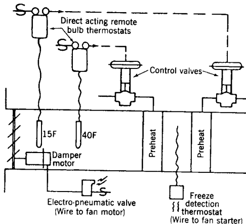
Fig 13-133. Hot water preheat coil control
