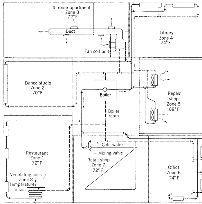
Fig 15-91. Application of hot water system for production of different space requirements: zone 1 convectors, 1 pipe series loop; zone 2 baseboard, single pipe; zone 3 fan coil duct system; zone 4 fan coil room units; zone 5 unit heaters; zone 6 convectors, 2 pipe direct return; zone 7 panel ceiling; zone 8 fan coil, for heating outdoor air for restaurant
