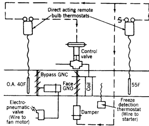
Fig 13-134. Face and bypass control
