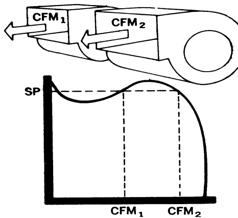
Fig 14-28. Unbalanced parallel operation
