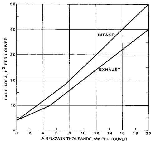
Fig 8-5. Criteria for louver sizing
