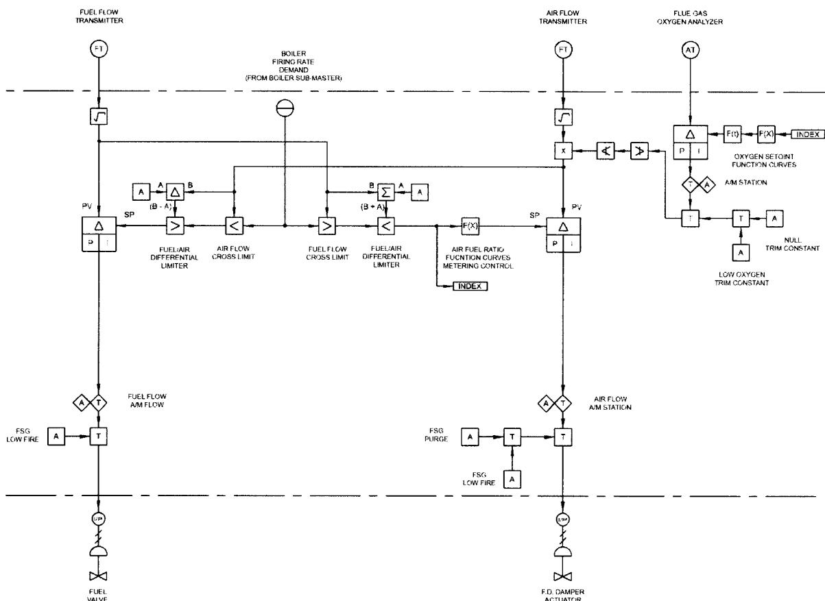
Fig 12-10. Fully metered control diagram shown with flue gas oxygen trim
