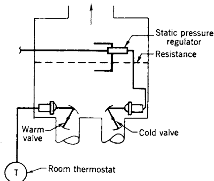
Fig 13-114. Type B duct constant volume unit
