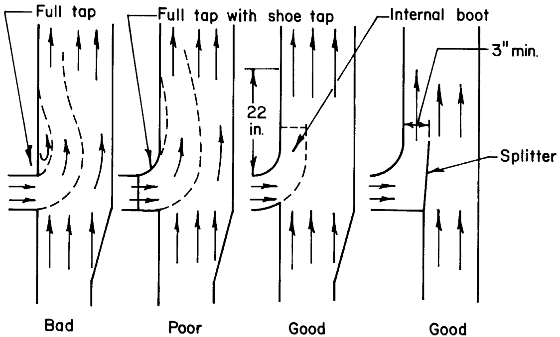
Fig 14-67. Four types of arrangements of return or exhaust air duct branch fittings
