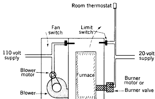
Fig 15-137. Basic arrangement of controls
