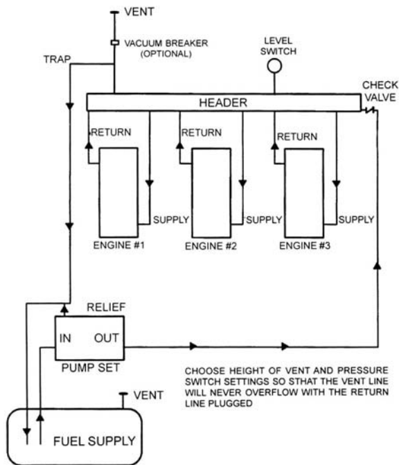
Fig 12-27. Emergency generator "Loop System"
