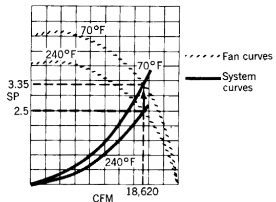
Fig 14-18. Example no. 4—Fan law no. 4 (density change)
