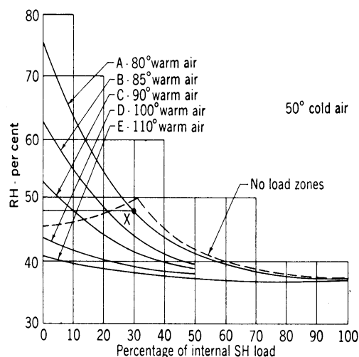
Fig 13-97. Performance over whole range of internal sensible heat load; system of Fig. 13-91 for 50°F cold air
