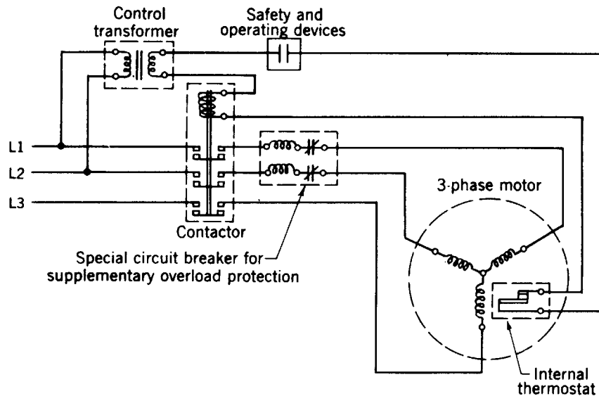
Fig 17-11. Three phase motor with internal protection
