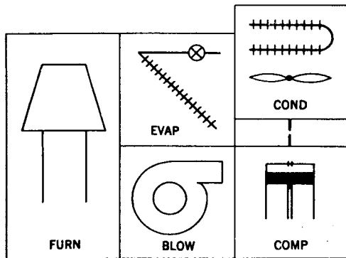
Fig 13-10. Year round air conditioner with remote air cooled condensers
