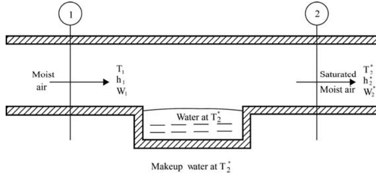
Fig 2-3. Adiabatic saturation of air
