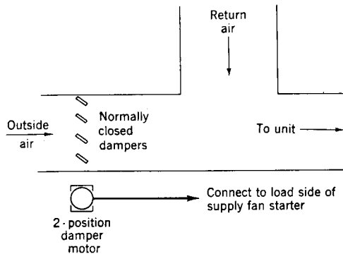
Fig 13-34. Simplest ventilation system
