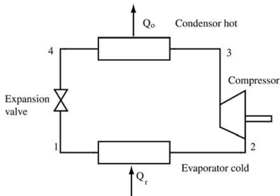
Fig 1-6. Components of the refrigerator or air conditioner
