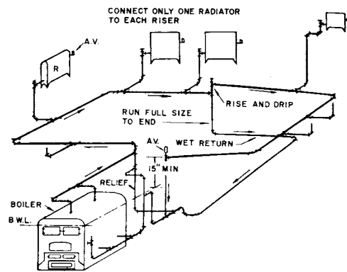
Fig 15-61. One pipe upfeed gravity system
