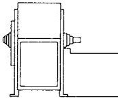
No. 7, SW, SI. For belt drive on direct connection. Arrangement No. 3 plus base for prime mover. Not recommended in sizes 27" diameter and smaller.
