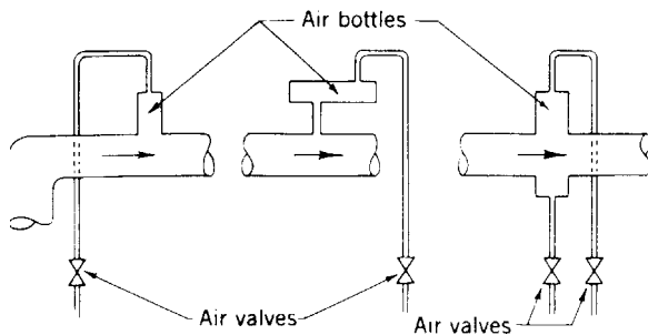
Fig 15-117. Collecting chambers for venting of air
