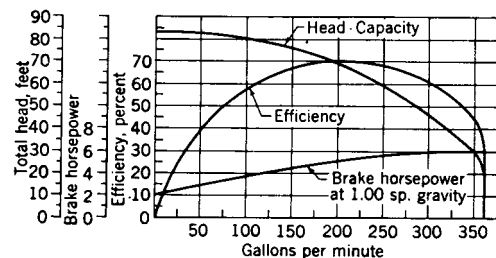
Fig 10-17. Performance curves for a typical centrifugal pump one with 9.5 in. impeller diameter and 1750 rpm constant speed
