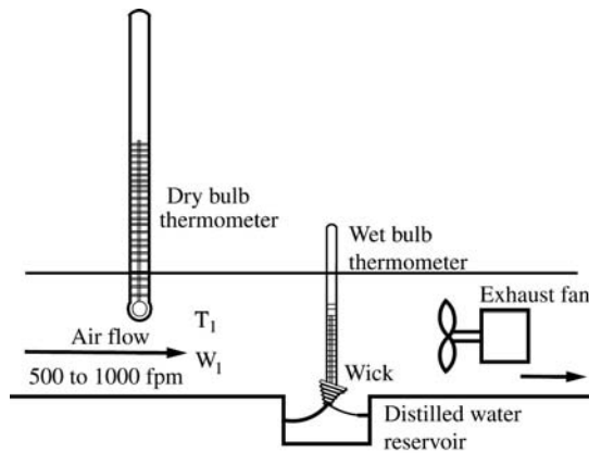
Fig 2-1. Psychrometry apparatus for measuring wet and dry- bulb temperatures
