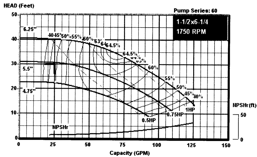
Fig 10-18. Pump curve for Series 60 B&G inline pump
