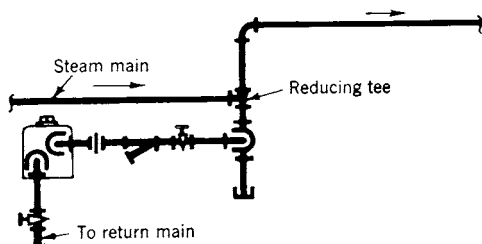
Fig 15-18. Steam main rise and drip connection
