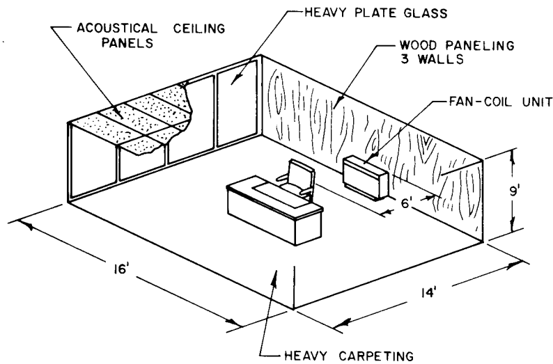
Fig 16-10. An office for which NC level is to be computed
