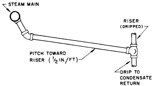
Fig 15-37. Connection to dripped risers
