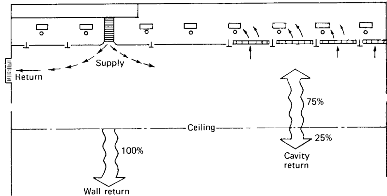
Fig 13-53. Proportionate heat distribution through luminous or louvered ceiling
