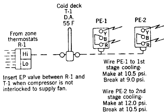
Fig 13-120. Cold deck control
