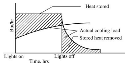
Fig 7-3. Thermal storage effect in cooling load from lights
