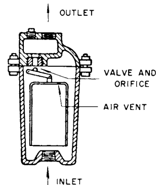
Fig 15-77. Inverted bucket trap
