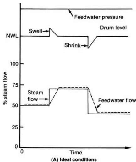
Fig 12-12. Performance of two element feedwater control (ideal conditions)
