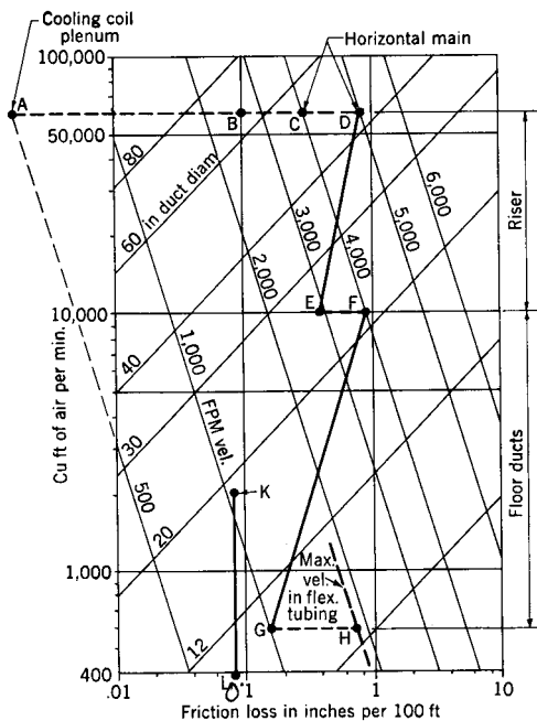
Fig 13-99. Air friction chart
