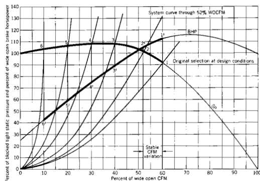
Fig 14-53. Discharge damper performance for air foil fan
