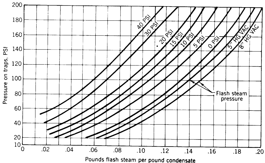
Fig 15-86. Lbs flash steam per lb condensate
