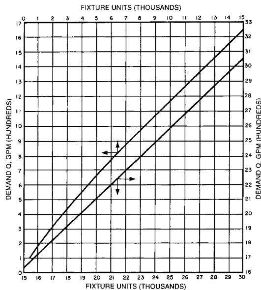
Fig 9-5. Demand versus fixture units
