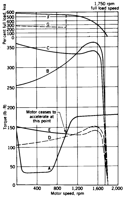
Fig 17-14. Torque speed and KVA speed curves for 60 hp motor and compressor
