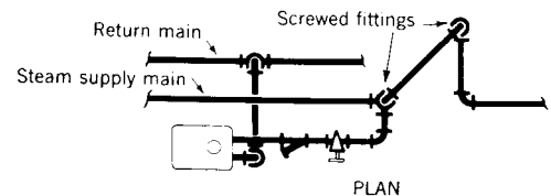
Fig 15-32. Swing type expansion loop combined with main rise and drip
