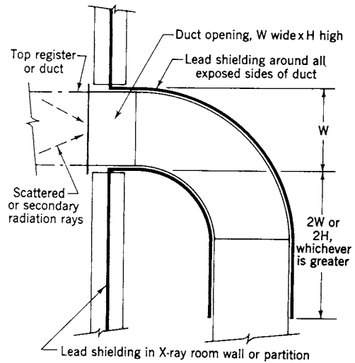
Fig 16-44. Elevation of Section Through X-ray Room
