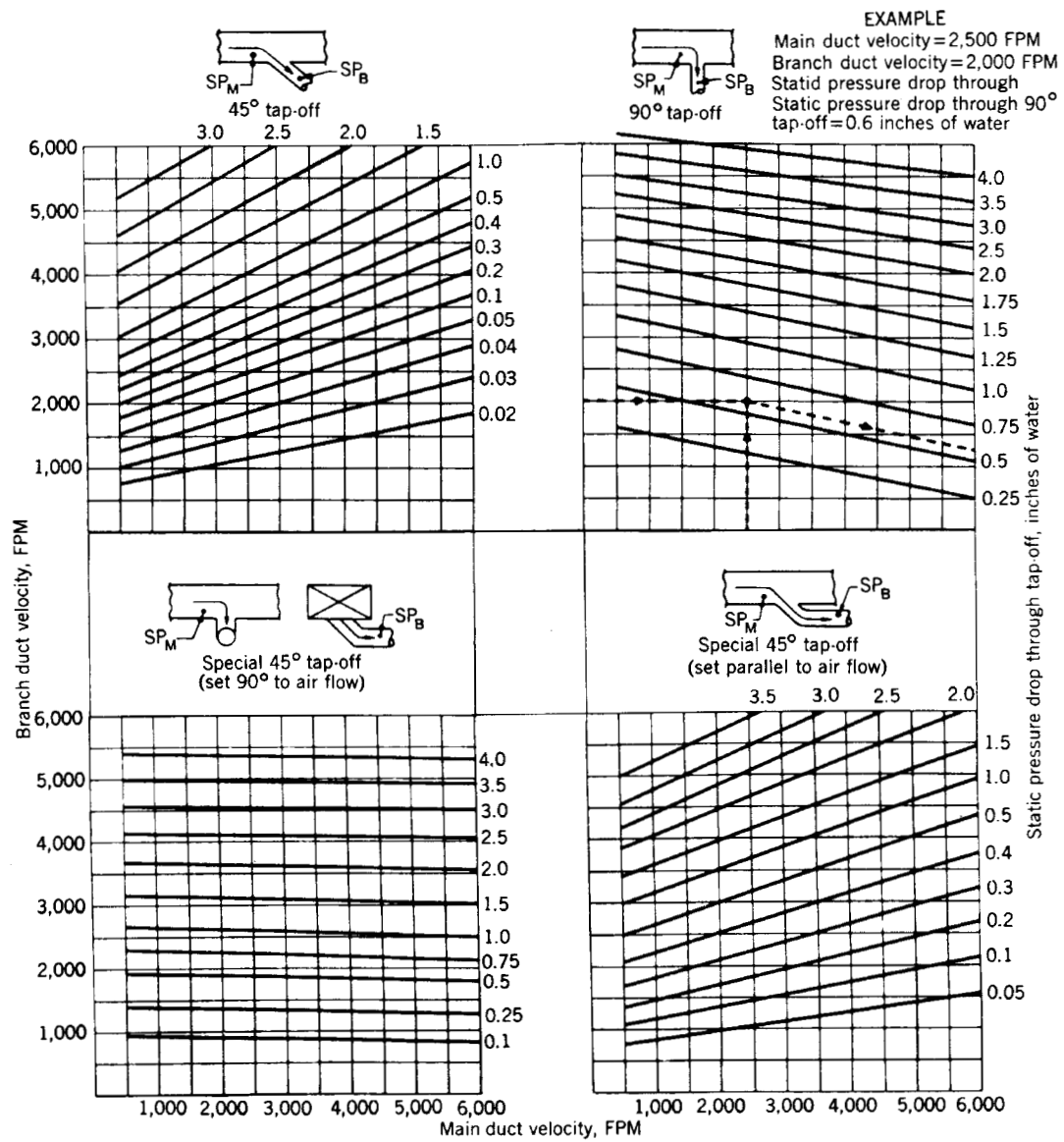
Fig 14-74. Static pressure losses through 4 types of tap off connections in high velocity duct systems
