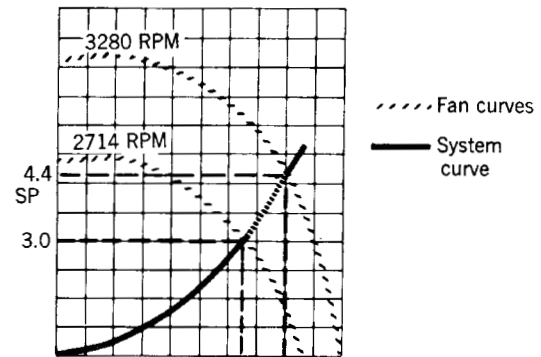
Fig 14-16. Example no. 2—Fan law no. 1 (RPM Change)
