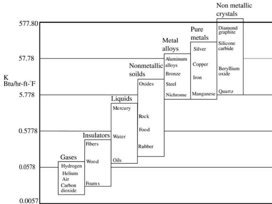
Fig 5-2. Range of thermal conductivity of various materials at different temperatures
