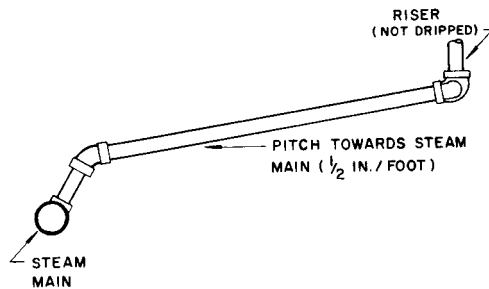
Fig 15-38. Connection to risers
