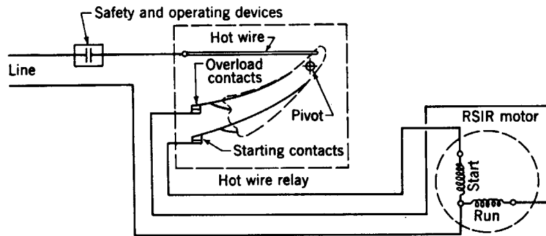
Fig 17-7. Hot wire relay with resistance start, induction run motor
