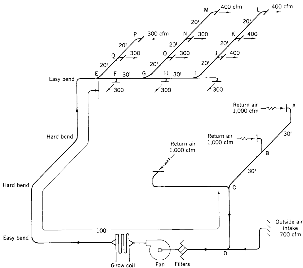
Fig 14-70. Layout of system employing constant pressure drop method
