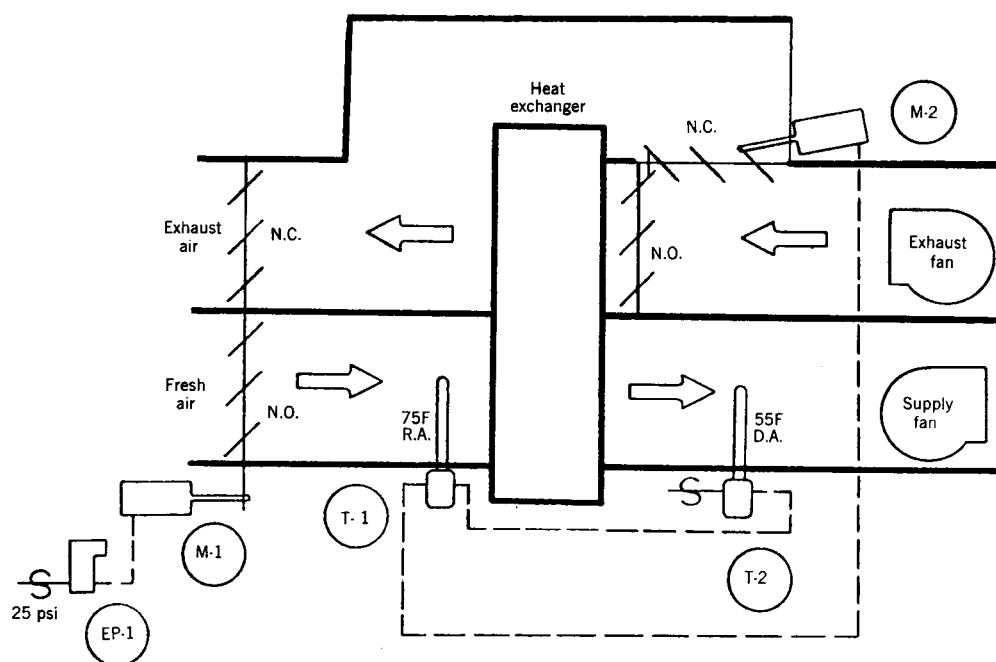
Fig 13-143b. Rotary air-to-air heat exchanger control, variable speed
