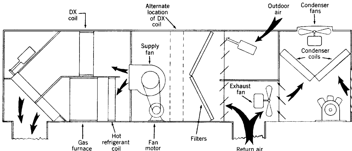
Fig 13-117. Multizone rooftop control
