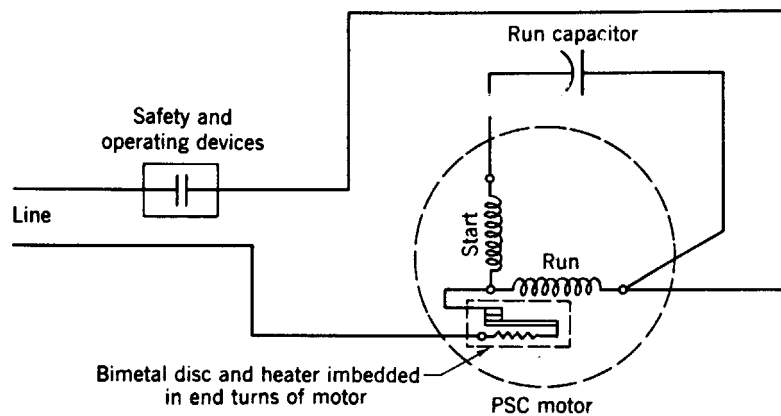
Fig 17-9. Permanent split capacitor motor with internal line break overload protection
