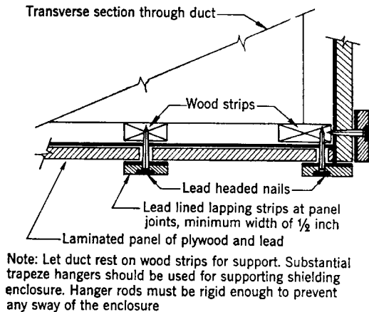
Fig 16-45. Elevation of section through X-ray room
