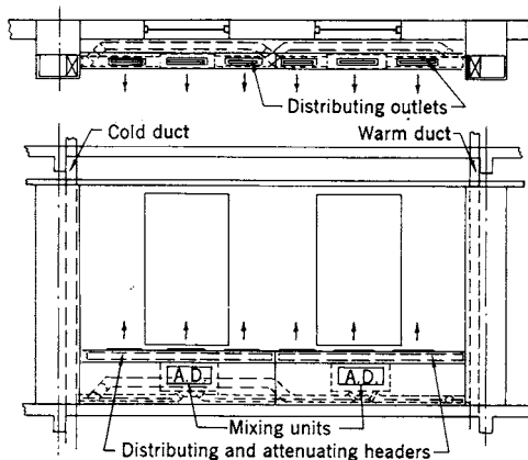
Fig 13-104. Arrangement for vertical under window dual duct units two units per riser
