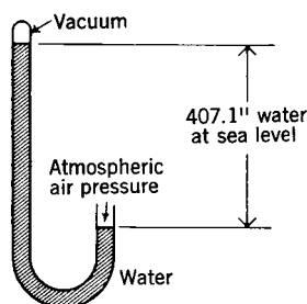
Fig 14-1. Atmospheric pressure
