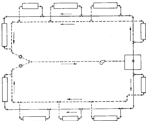
Fig 15-96. Two pipe reversed return system
