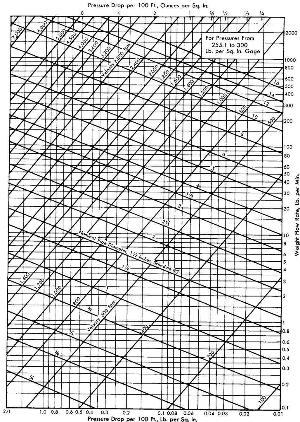
Fig 9-35. For pressure from 255.1 to 300.0 psig
