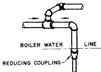
Fig 15-44. Dripping steam main
