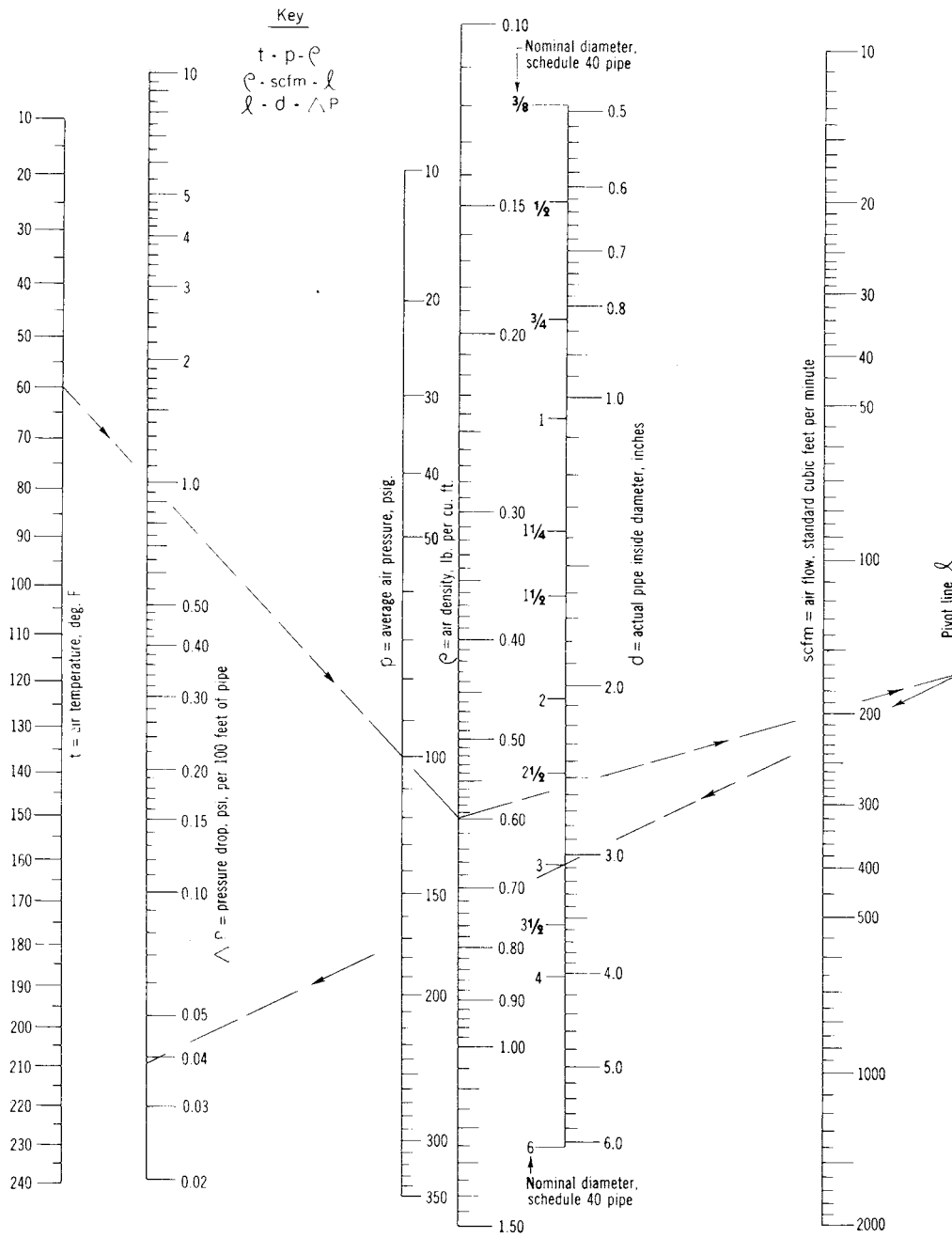
Fig 9-38. Nomograph for calculating pressure drops in steel pipe and sizing of air in pipes
