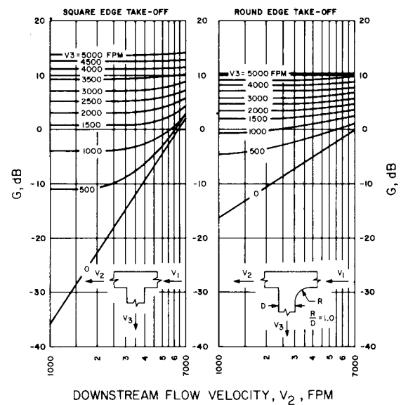
Fig 16-19. Velocity function G for 90^\circ branch take-offs
