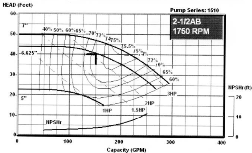
Fig 10-21. Pump curve for Series 1510 B&G end suction pump
