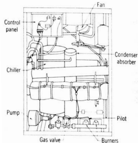
Fig 13-18. Gas fired water chiller
