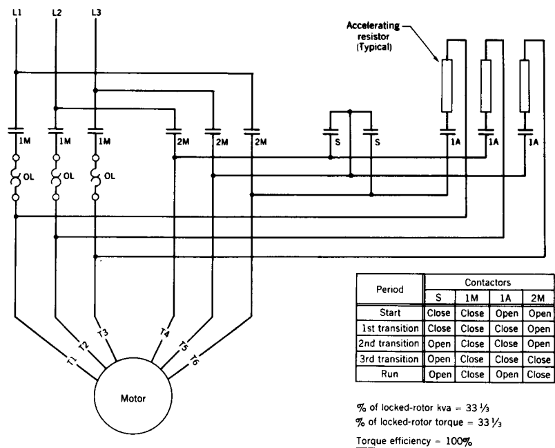
Fig 17-23. Star delta (closed circuit transition)
