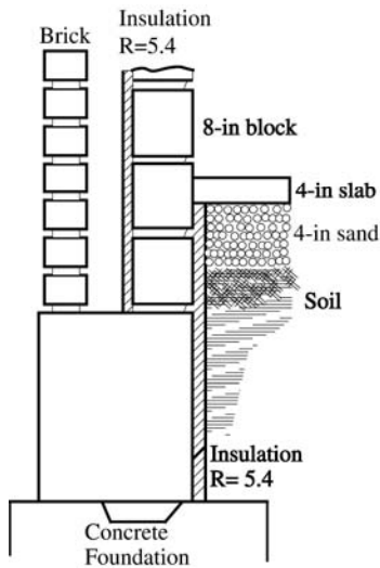
Fig 6-4. Concrete wall slab on grade foundation insulation
