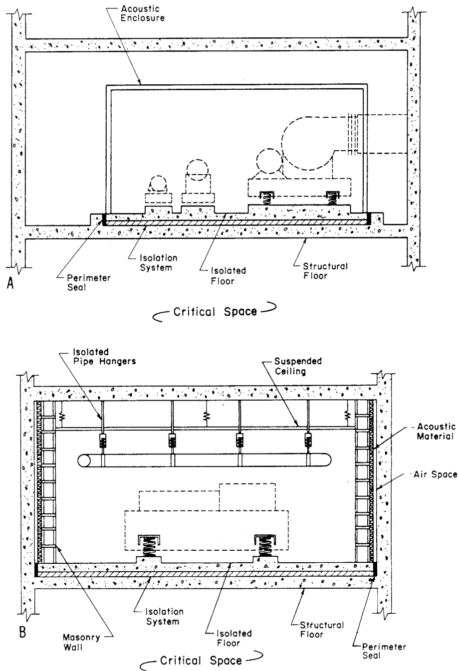
Fig 16-6. Two Structural Methods for Isolating Mechanical Equipment Noise
