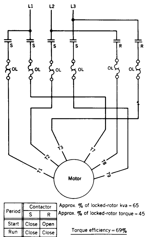
Fig 17-16. Part winding (two-thirds winding start)
