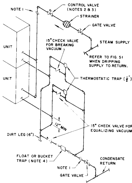
Fig 15-56. Multiple coil low pressure vacuum system piping
