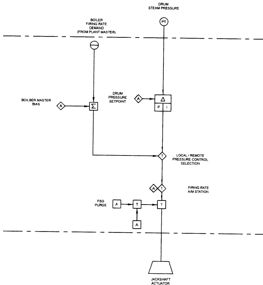
Fig 12-8. Single point positioning shown with local pressure control
