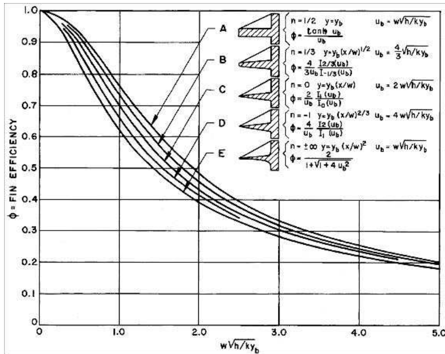
Fig 1-12. Efficiency of straight fins
