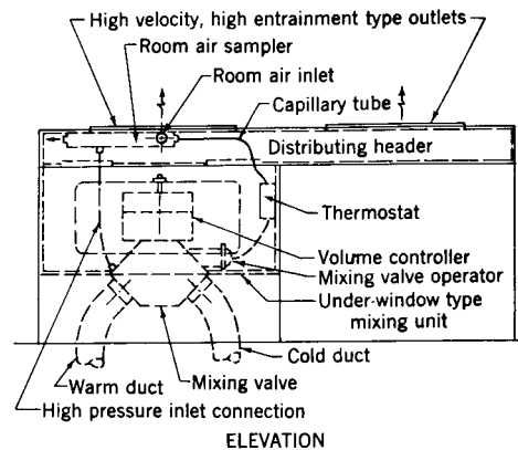
Fig 13-109. Method of mounting air sampler in mixing unit
