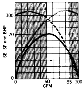
Fig 14-38. Characteristic curves for tubular centrifugal fans
