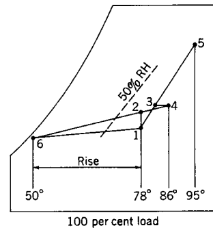
Fig 13-93. Psychrometric chart for dual duct system for Fig. 13-88 full load
