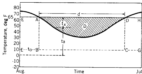
Fig 11-6. Normal daily mean temperature curve showing graphically the number of degree-days
