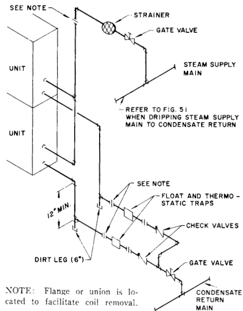
Fig 15-57. Low pressure or vacuum system steam traps
