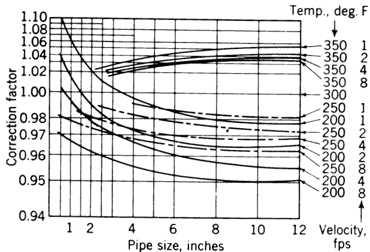
Fig 15-120. Correction factors for friction loss from Fig. 15-121
