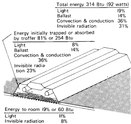
Fig 13-49. Theoretical dissipation of heat with two 40-watt fluorescent lamps and ballast (assumed 60% luminaire efficiency)
