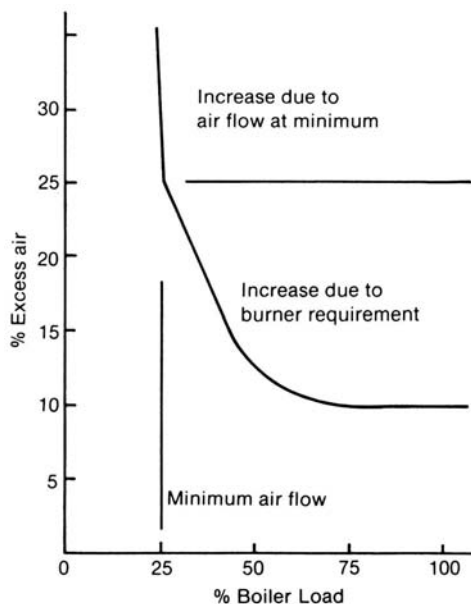
Fig 12-1. Typical curve for excess air versus boiler load
