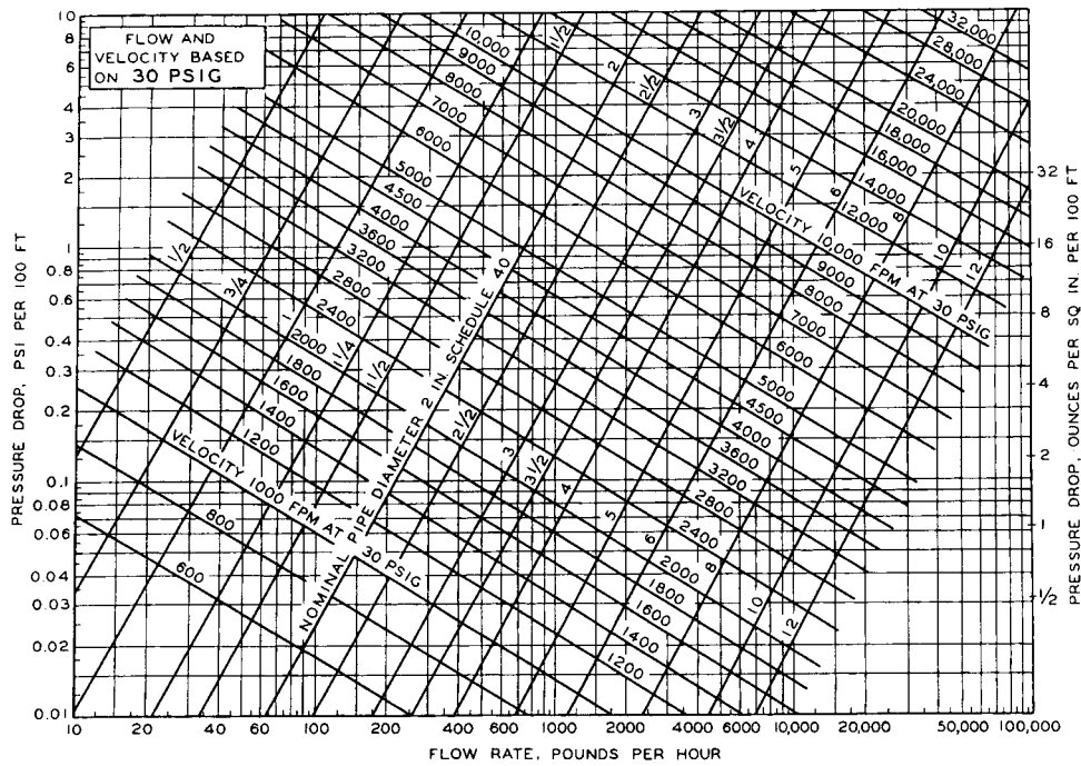
Fig 9-11. Flow rate and velocity of steam in Schedule 40 pipe at saturation pressure of 30 psig
