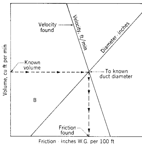
Fig 14-60c. Finding volume and friction from known velocity and diameter
