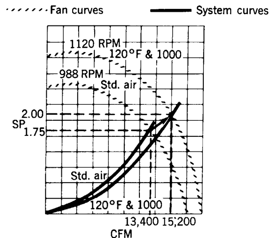
Fig 14-20. Example no. 5—Fan law no. 6 (density change)
