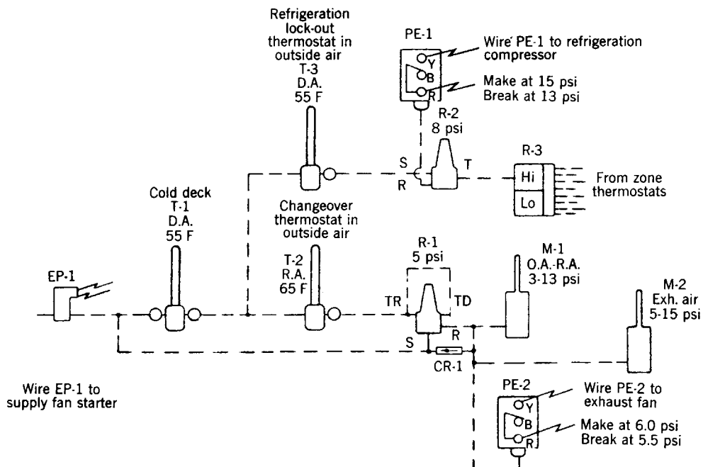
Fig 13-119. Mixed air control
