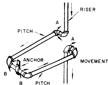
Fig 15-41. Riser anchor
