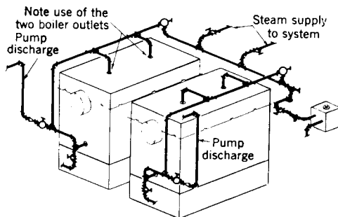
Fig 15-8. Two boilers with separate direct return connections from overhead
