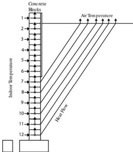
Fig 6-2. Heat flow path for partially insulated basement wall
