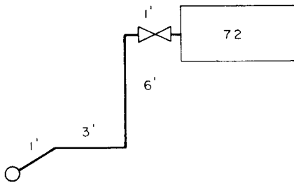
Fig 15-70. Low pressure run out and riser
