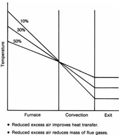
Fig 12-3b. Effect of excess air on temperatures
