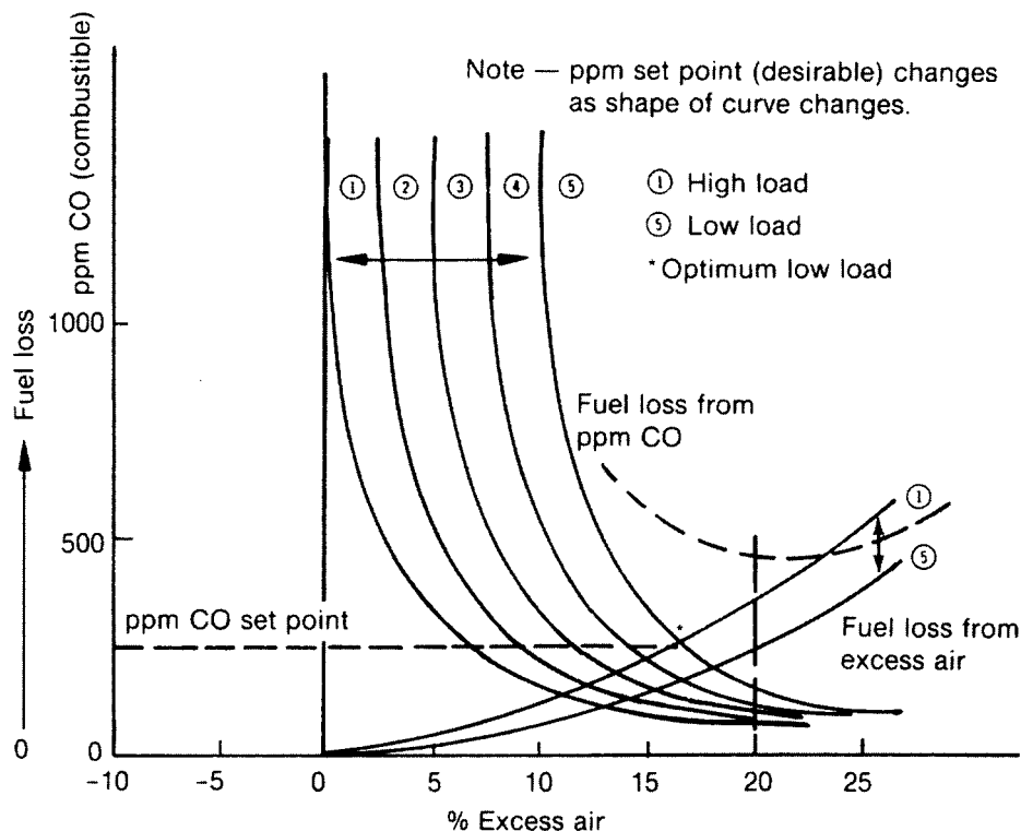
Fig 12-2. Excess air combustible gas relationship
