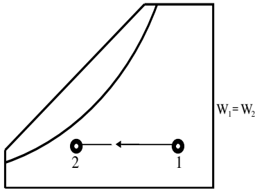
Fig 3-3. Psychrometric diagram of simple cooling process
