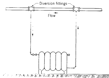
Fig 15-102. Preferred connection when radiation is below supply and return
