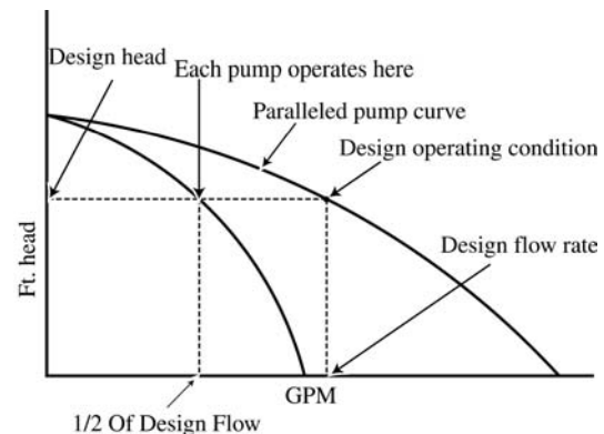
Fig 10-30. Actual point of system operation and the constructed combined parallel curve
