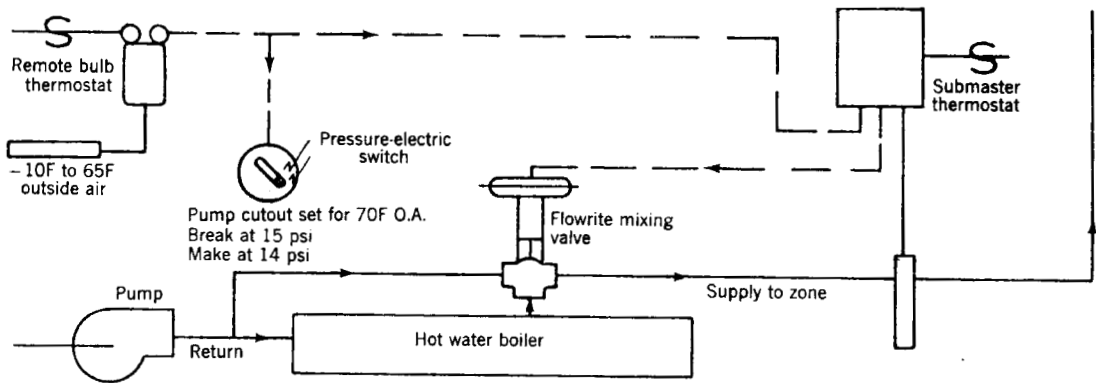
Fig 13-132. Scheduled hot water control
