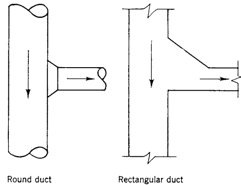
Fig 16-39. Tap-off from main or riser
