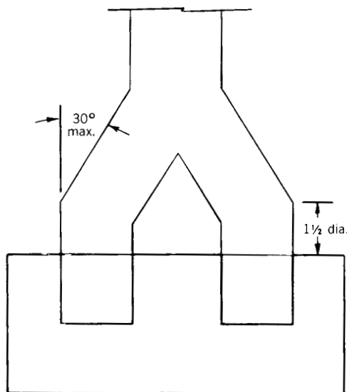
Fig 14-52. Proper construction of a pants connection on a two-fan unit
