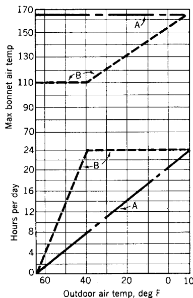
Fig 15-140. Air flow and air temperature for intermittent blower operation
