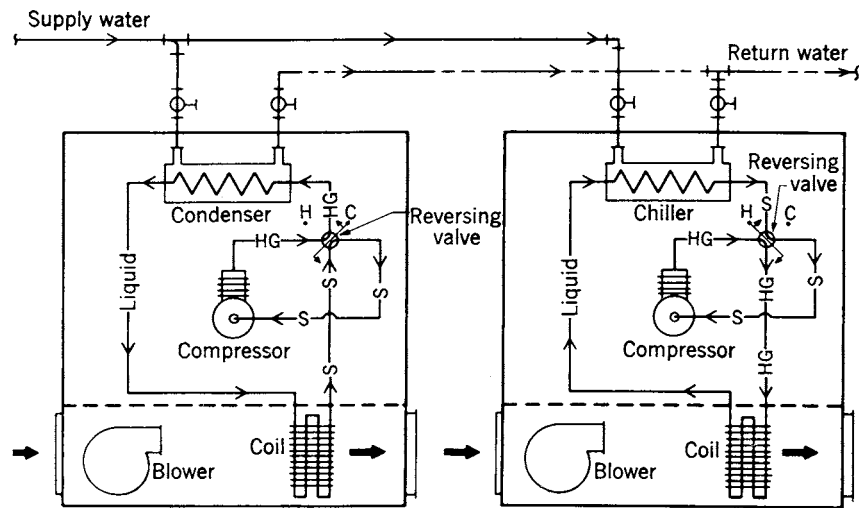
Fig 13-74. Water is recirculated in a loop as a heat reservoir
