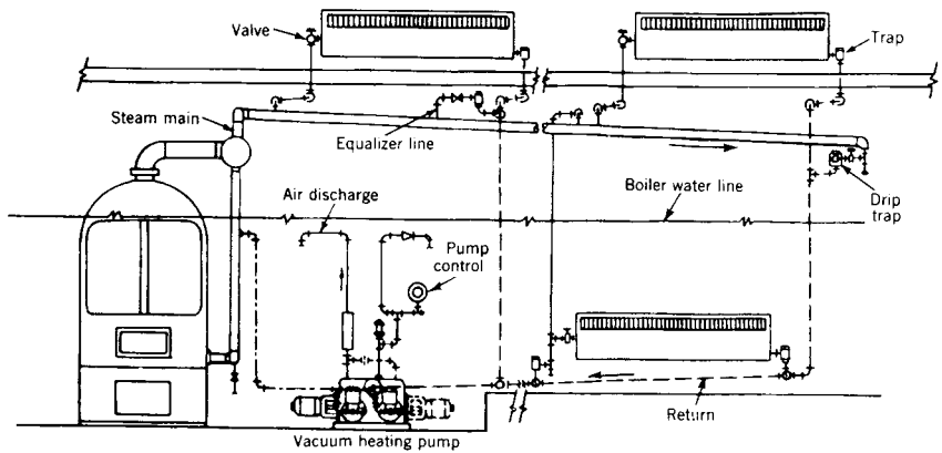
Fig 15-3. Vacuum heating pump maintains a vacuum in the return piping under all operating conditions
