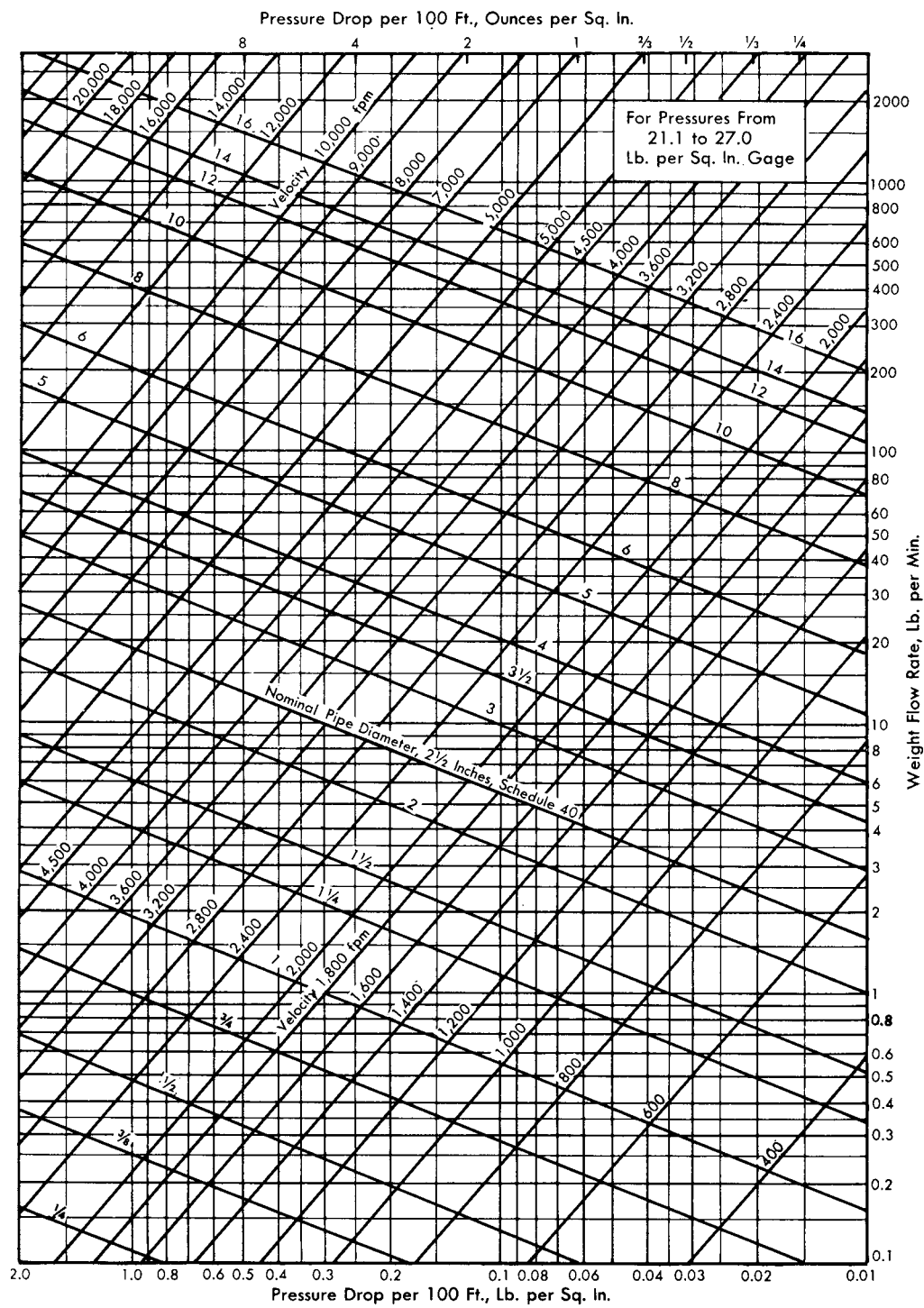
Fig 9-21. For pressure from 21.1 to 27.0 psig
