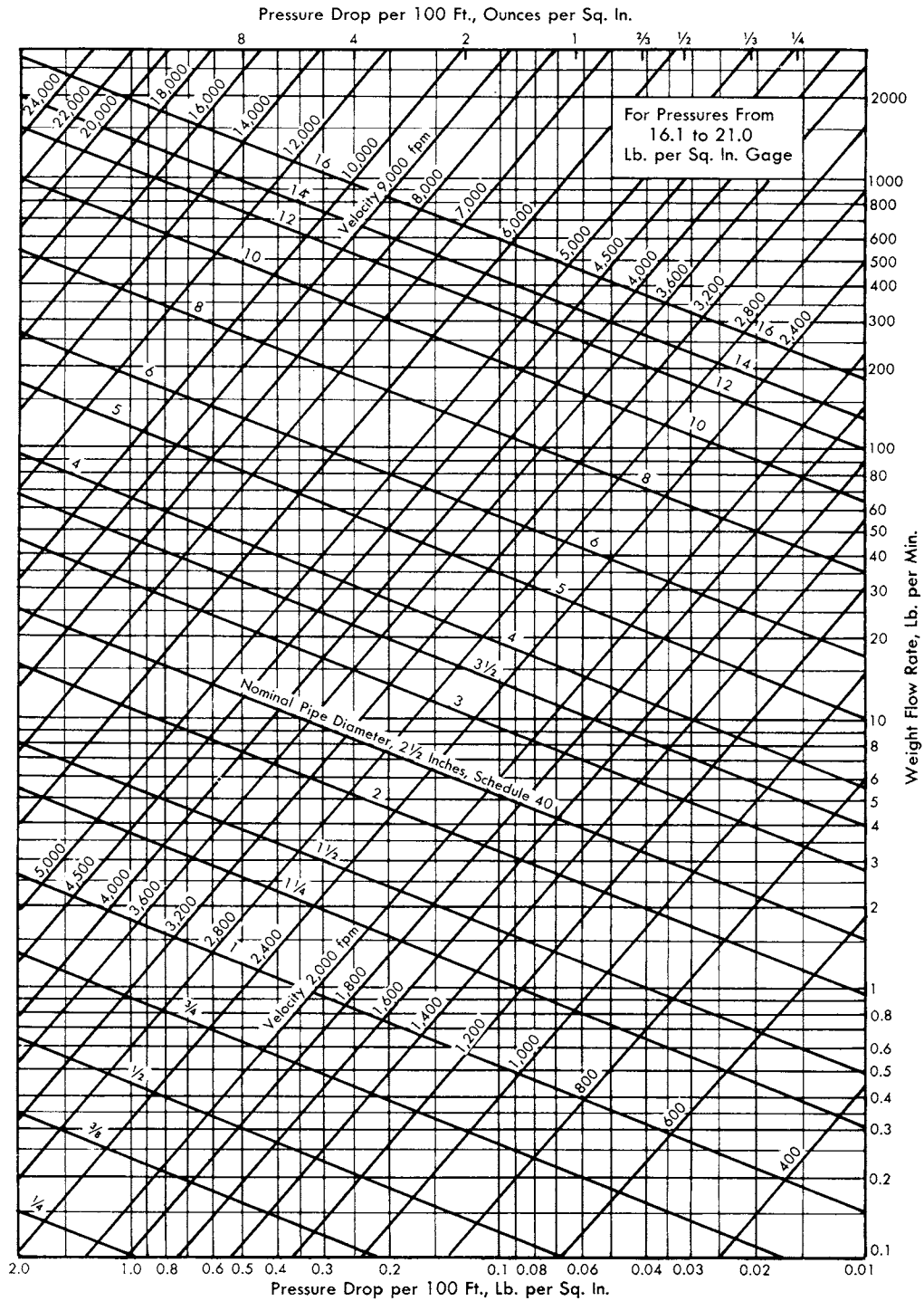
Fig 9-20. For pressure from 16.1 to 21.0 psig
