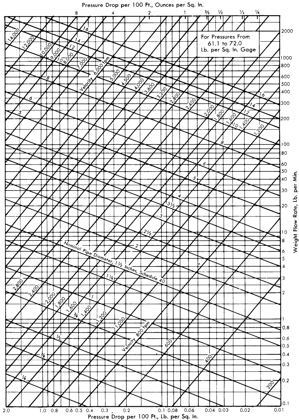
Fig 9-26. For pressure from 61.1 to 72.0 psig
