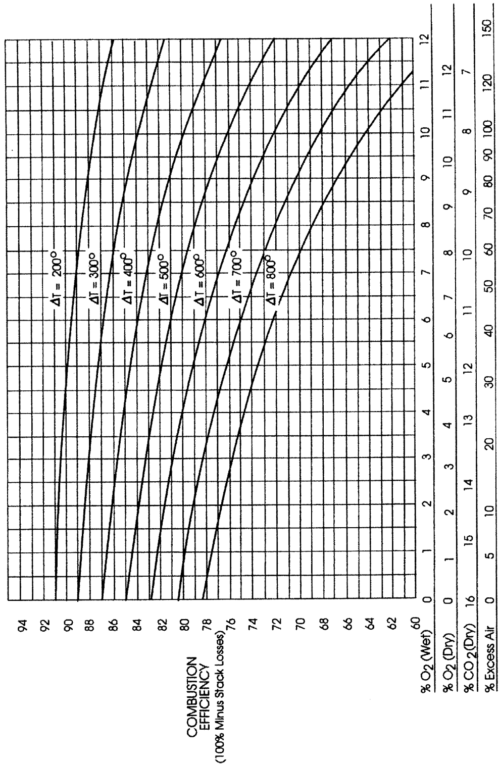
Fig 12-7. Combustion efficiency of No. 6 oil
