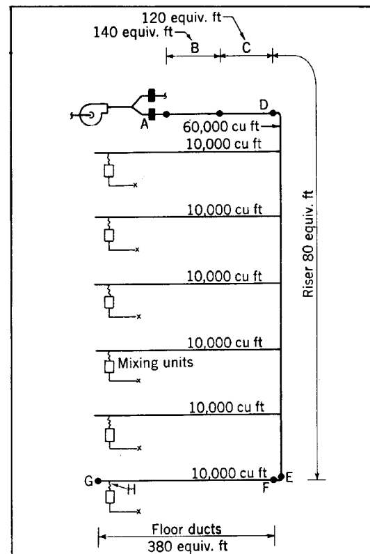
Fig 13-98. Dual duct system showing cold air duct only
