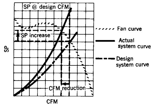
Fig 14-24. Variations from design—air shortage
