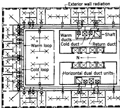
Fig 13-101. Typical office building dual duct layout with supplementary radiation at exterior wall zoned to provide selective temperature control for each enclosure
