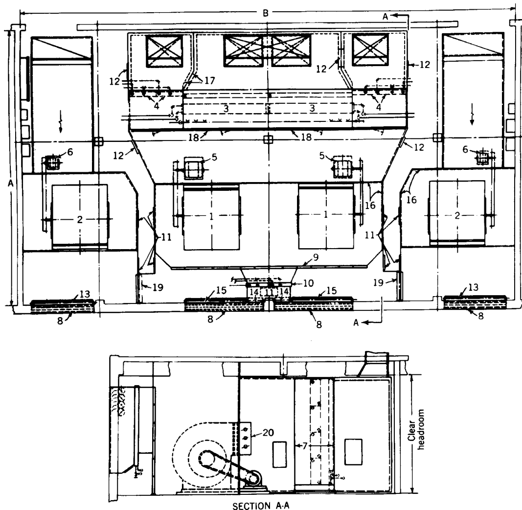
Fig 13-115. Type large capacity dual duct system
