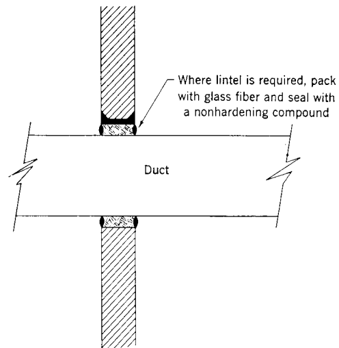
Fig 16-34. Ductwork through partition from mechanical to occupied space
