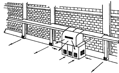
Fig 15-158. Details of gas fired heater installation
