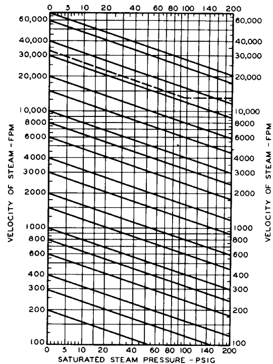
Fig 15-67. Velocity conversion
