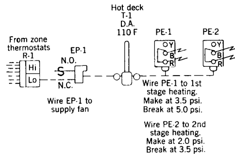
Fig 13-121. Hot deck control
