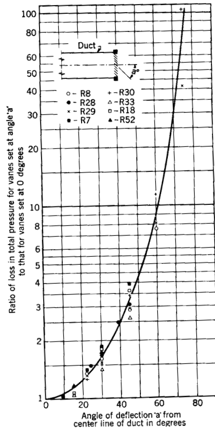
Fig 15-143. Increase in pressure loss with different angles of deflection. symbols represent different experimental use
