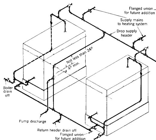
Fig 15-6. Two boilers with common return header and Hartford connection
