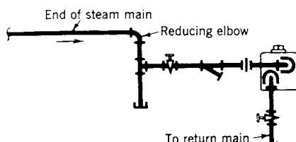
Fig 15-19. Details of end of main drip
