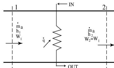
Fig 3-2. Schematic of simple cooling process (sensible cooling)
