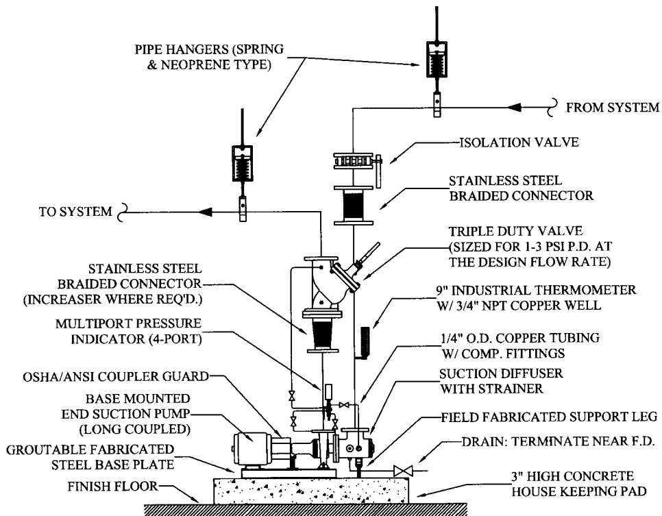
Fig 10-23. End suction pump detail
