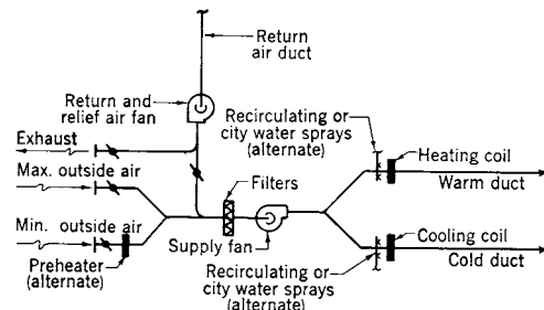
Fig 13-88. Single fan dual duct cycle with blow through dehumidifier
