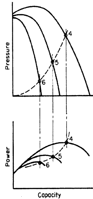
Fig 12-23. Vortex Damper
