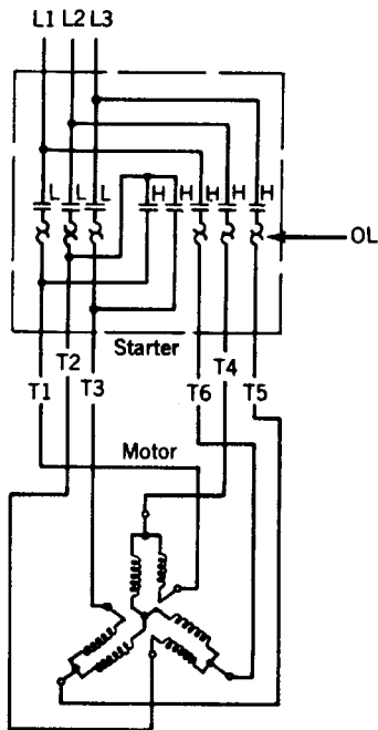
Two speed, single winding (consequent pole) variable torque
