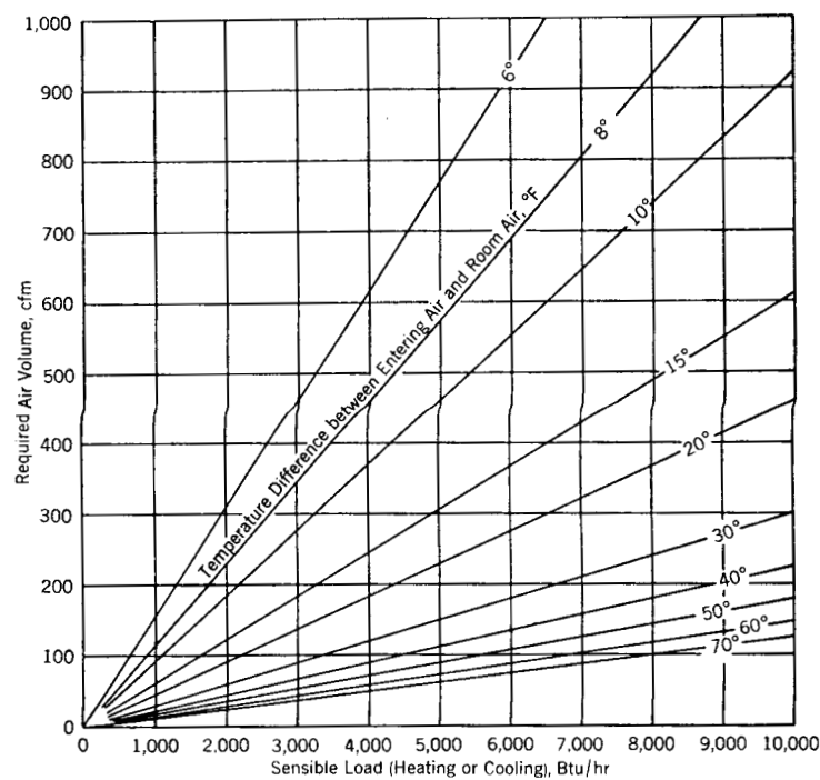
Fig 14-76. Air volume required to handle sensible heating or cooling loads
