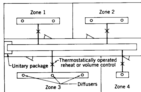
Fig 13-31. Single unit serves in multizone
