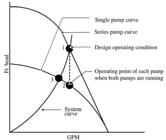
Fig 10-40. Single pump operation series installation
