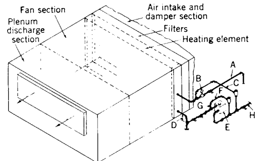
Fig 15-14. Auditorium ventilator piping connections
