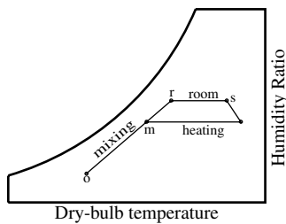
Fig 3-15. Psychrometric diagram of heating/humidifying process
