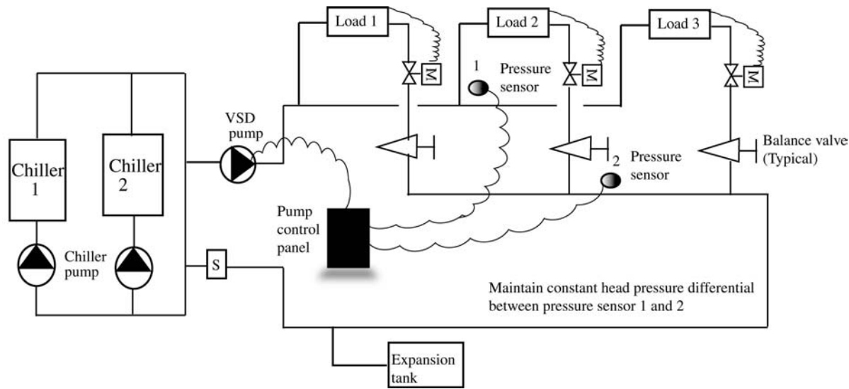
Fig 10-5. Closed chilled water system with variable speed chilled water supply pump
