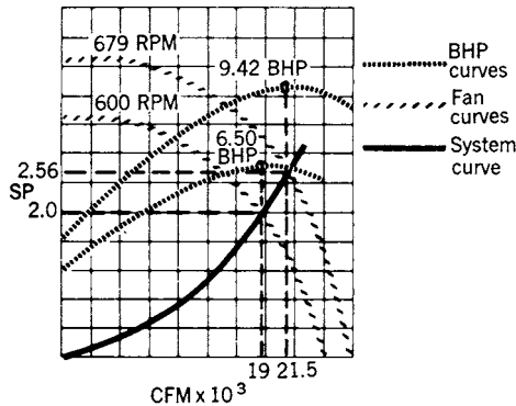
Fig 14-15. Example no. 1—Fan law no. 1 (RPM change)
