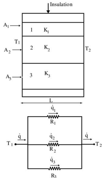
Fig 5-11. Thermal resistance network for three layers, parallel arrangements
