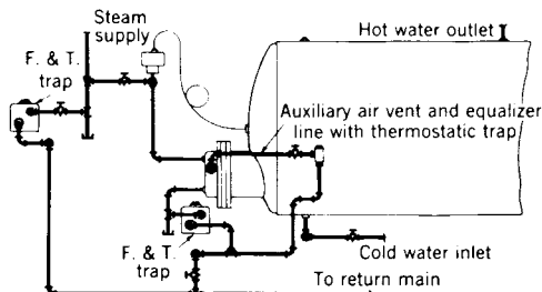
Fig 15-15. Piping connections to hot water generator
