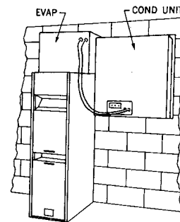
Fig 13-13. Split system, flush wall condensing unit
