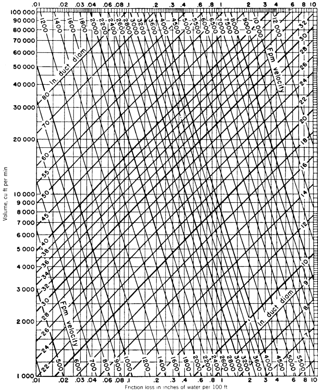
Fig 14-58a. Friction of air in straight galvanized ducts, for volumes 1000 to 100,000 cfm . (Same basis and source as Fig. 14-58b)
