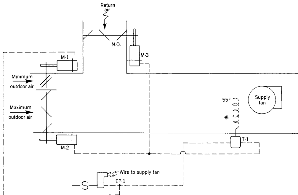
Fig 13-128. Changeover control
