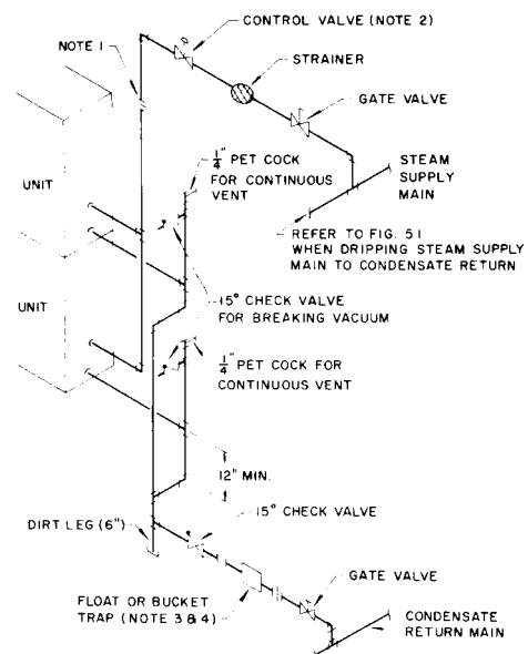
Fig 15-54. Multiple coil high pressure piping
