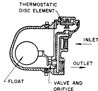
Fig 15-75. Typical float and thermostatic trap
