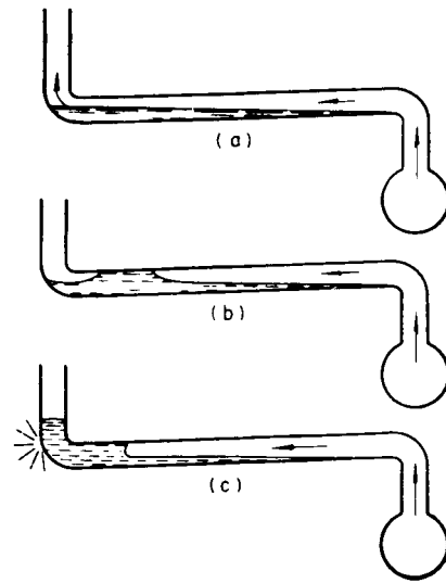
Fig 15-39. Water hammer
