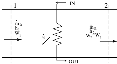
Fig 3-4. Schematic of simple heating process
