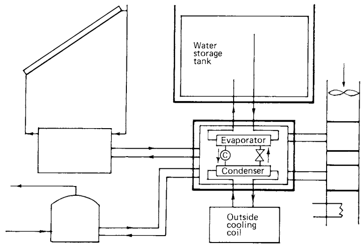
Fig 13-85. Cold storage
