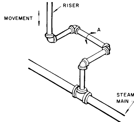
Fig 15-40. Riser connected to allow for expansion
