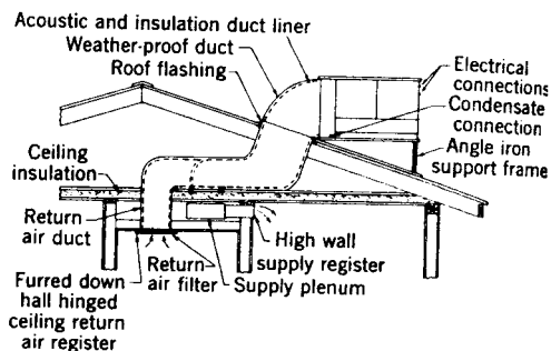
Fig 13-23. Self-contained unit mounted on gabled roof may not be visible from front
