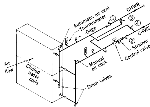
Fig 13-145. Isometric view of chilled water coil for both counterflow and parallel flow
