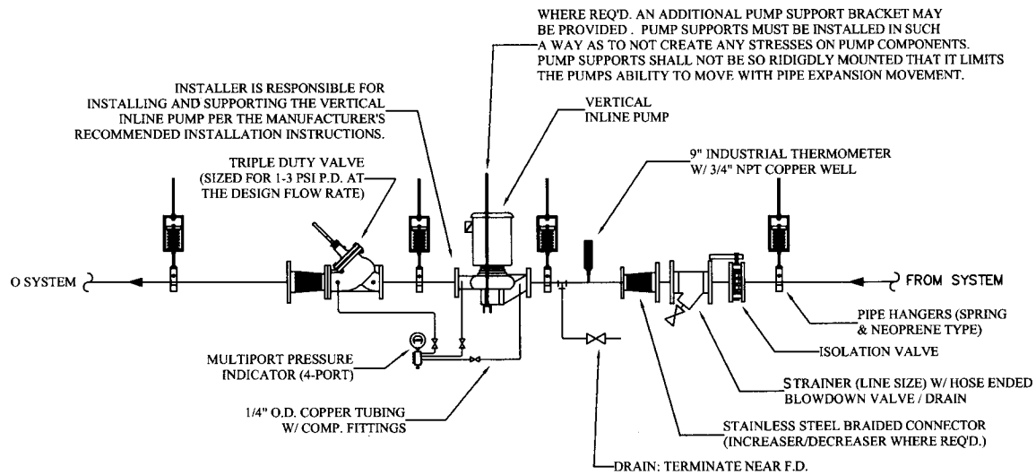
Fig 10-20. Vertical inline pump detail
