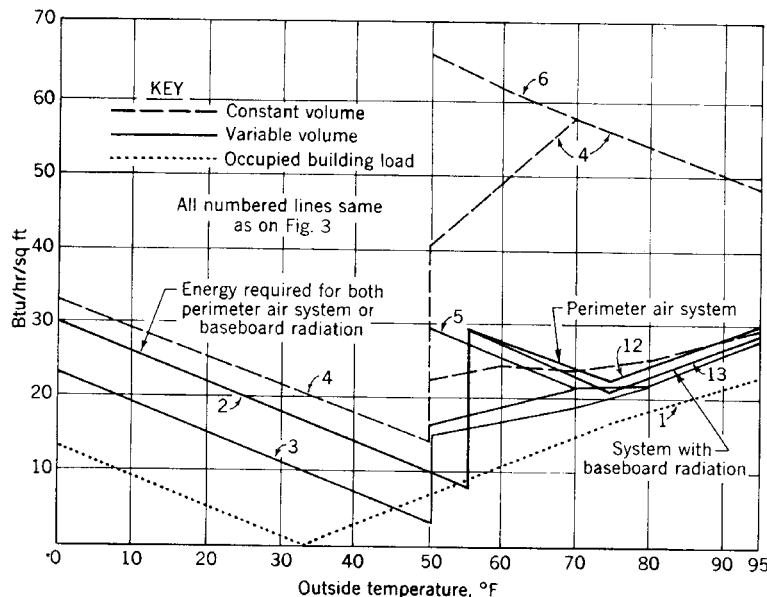
Fig 13-47. Energy requirement in Btu conditions-no sun load southern exposure
