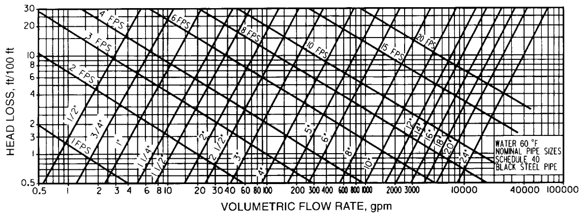
Fig 9-1. Friction loss for water in commercial steel pipe
