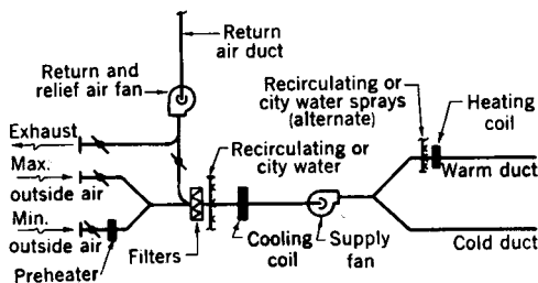
Fig 13-92. Single fan dual duct cycle with push through dehumidifier
