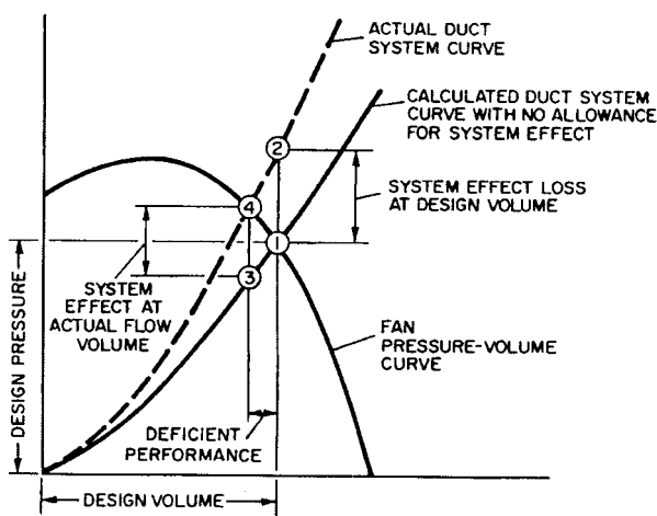
Fig 8-2. Deficient system performance with system effect ignored
