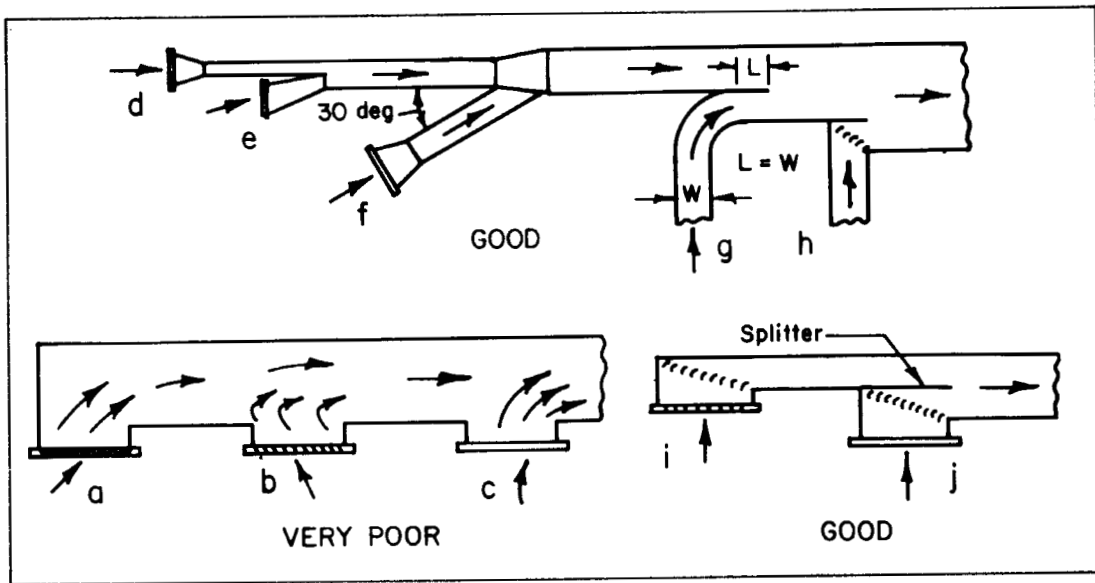
Fig 14-66. Air flow into ducts
