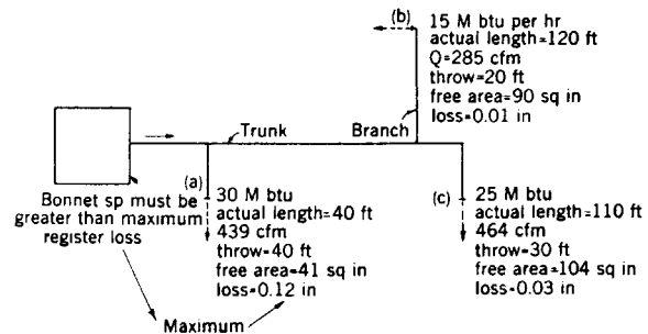
Fig 15-144. Maximum register loss and its relation to duct loss and bonnet static pressure
