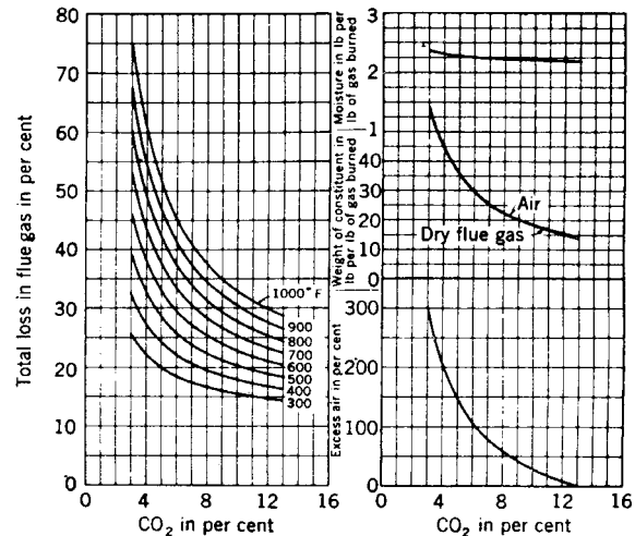
Fig 15-126. Flue gas losses with natural gas as fuel
