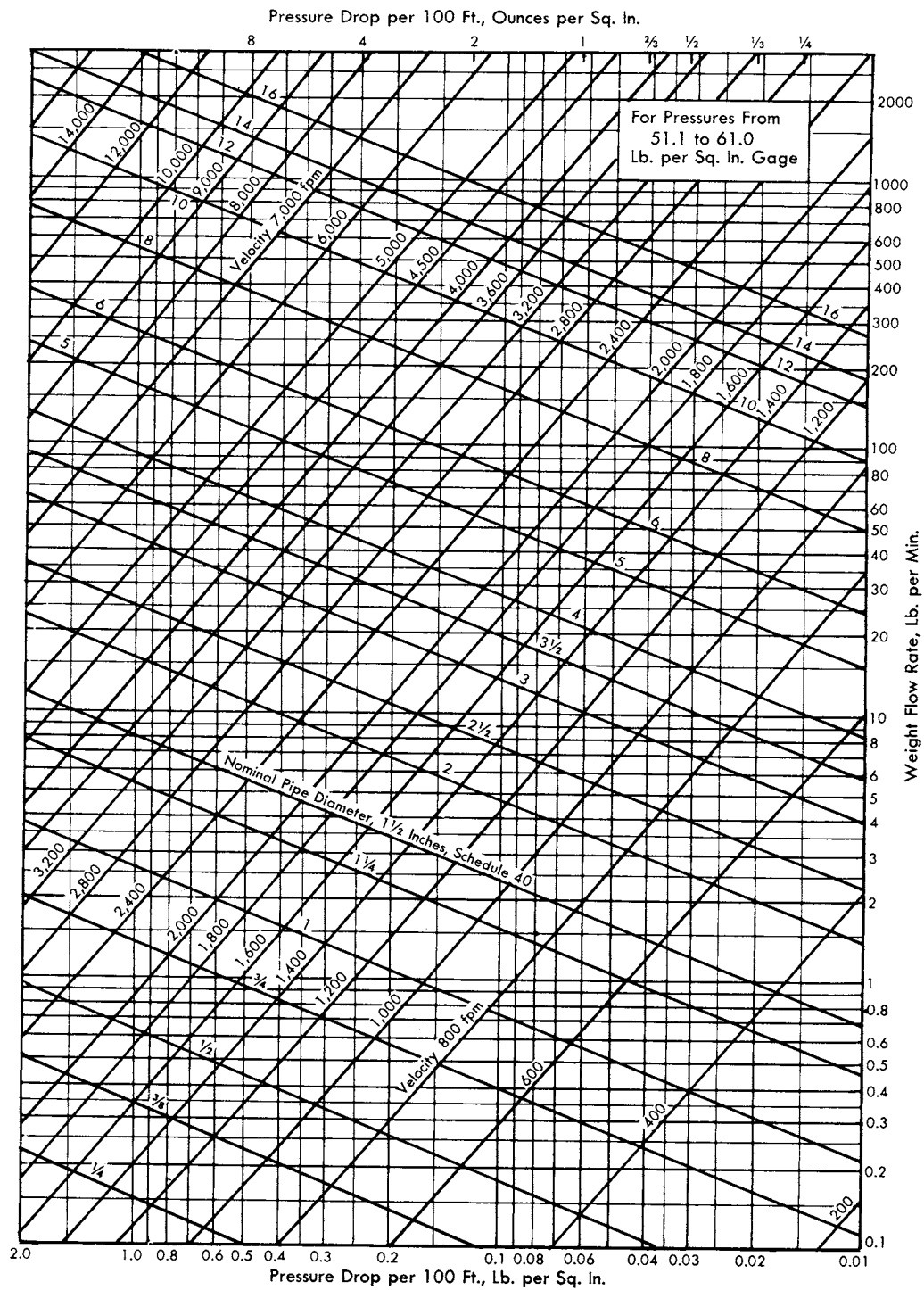
Fig 9-25. For pressure from 51.1 to 61.0 psig
