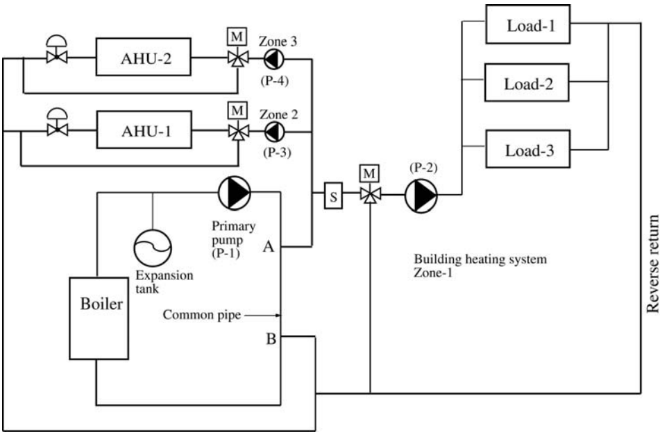
Fig 10-2. Heating system for multiple dwelling building with reverse return system
