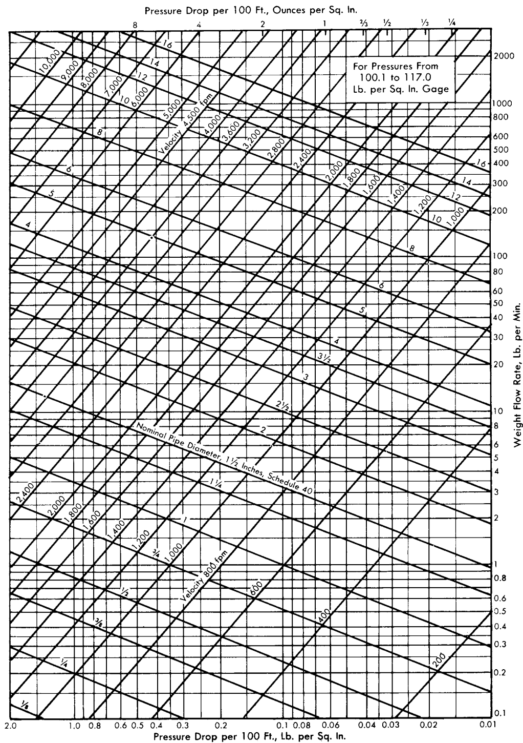
Fig 9-29. For pressure from 101.1 to 117.0 psig
