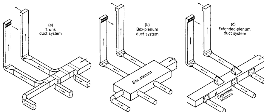
Fig 15-130. Three types of air duct system
