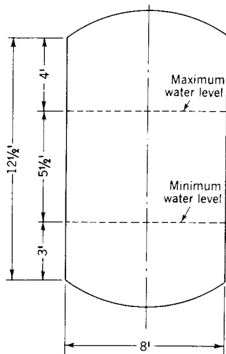
Fig 15-114. Vertical nitrogen pressurizing tank
