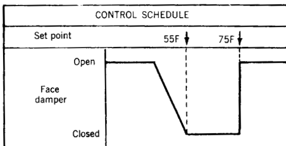
Fig 13-141a. Rotary air to air heat exchanger control, face-bypass
