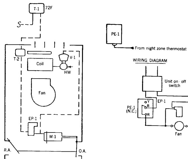
Fig 13-129. Unit ventilator control large unit
