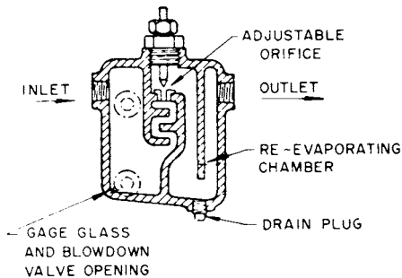
Fig 15-79. Flash type
