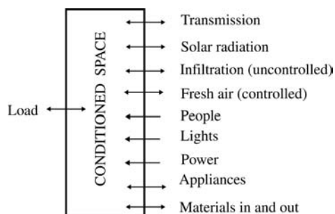
Fig 5-17. Components of heating and cooling loads
