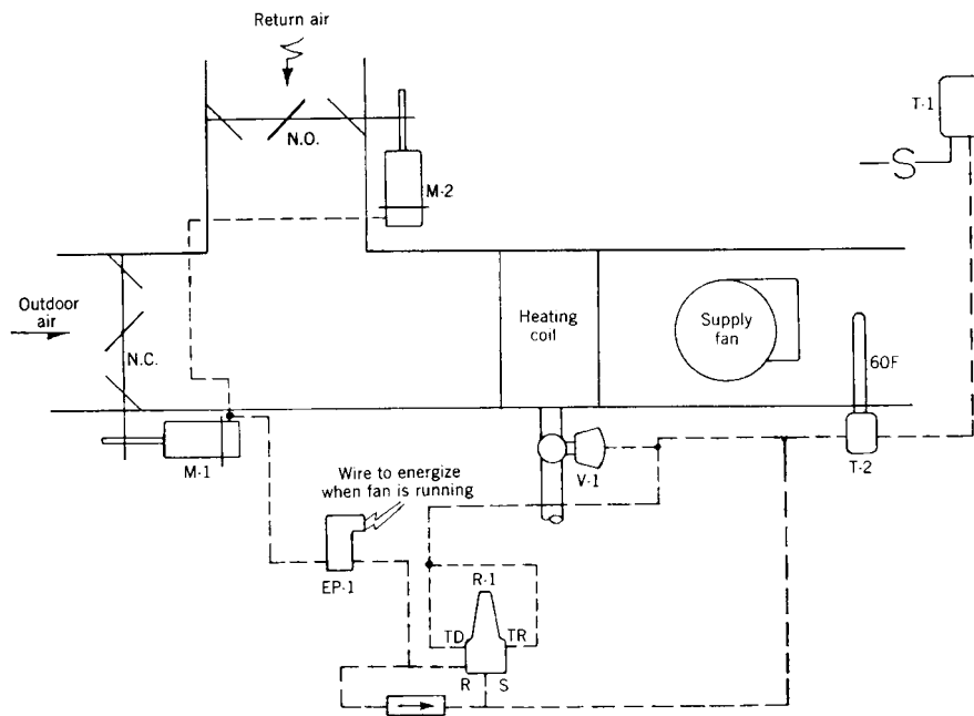
Fig 13-129. Unit ventilator control large unit
