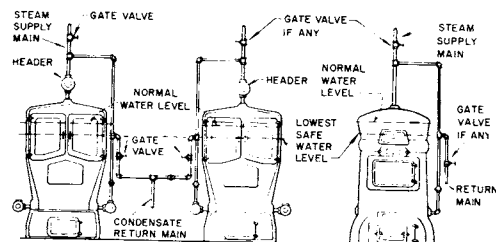
Fig 15-58. Hartford return loop
