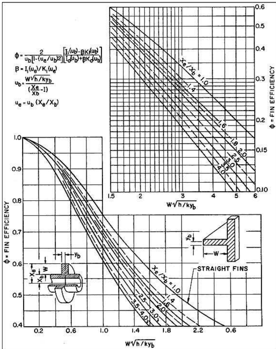
Fig 1-13. Fin efficiency for annular fins of constant thickness
