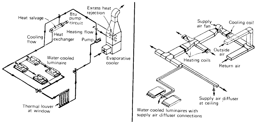
Fig 13-60. Integrated system operation
