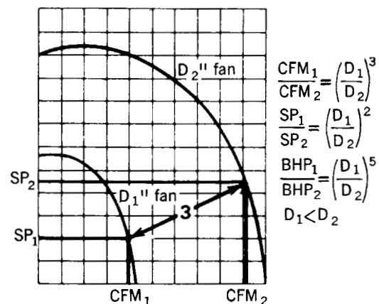
Fig 14-11. Fan law no. 3—change in wheel diameter (constant RPM)
