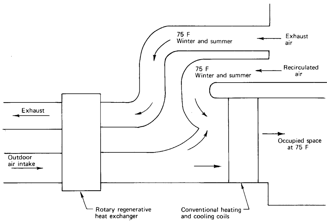
Fig 13-65. Diagram of heat recovery system using rotary heat exchanger
