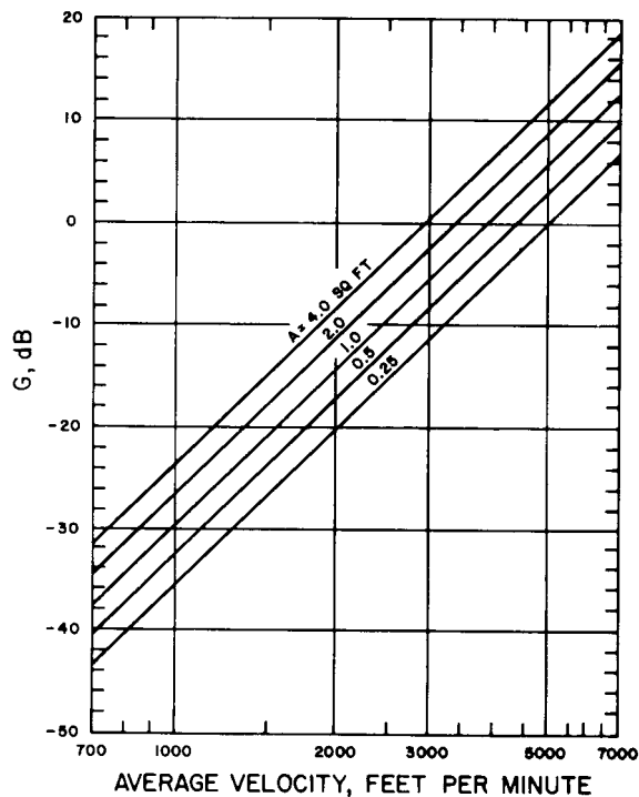
Fig 16-18. Velocity function G for 90^\circ elbows
