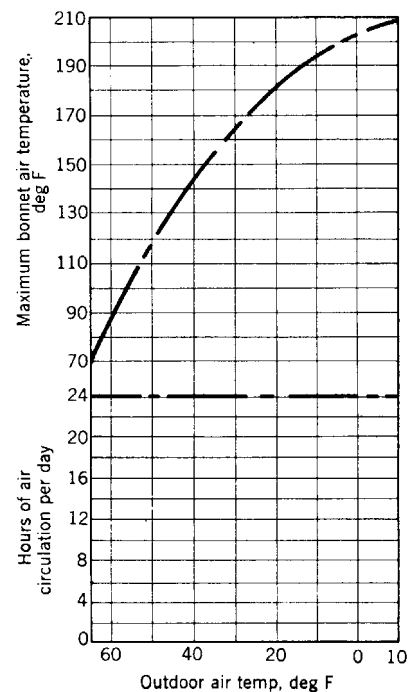
Fig 15-138. Air flow and air temperature for gravity warm air system
