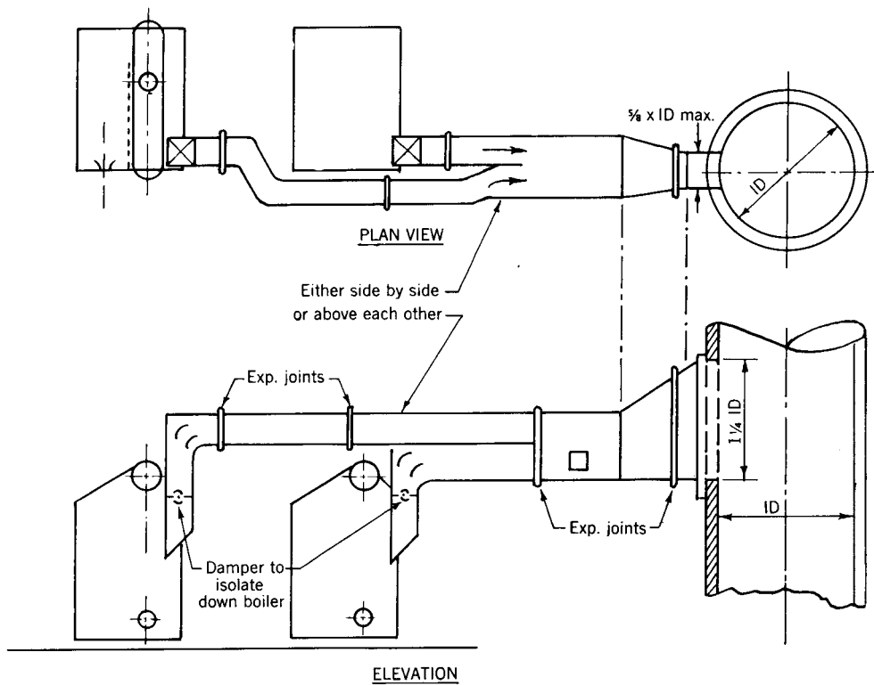
Fig 14-81. Typical breaching flow arrangements and stack entry
