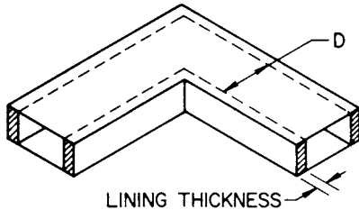
Fig 16-13. Illustration of duct width D for Table 16-19
