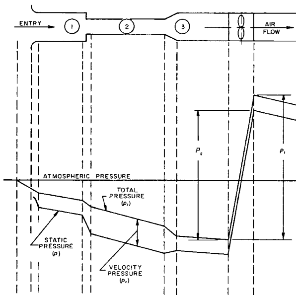
Fig 8-3a. Pressure changes in system
