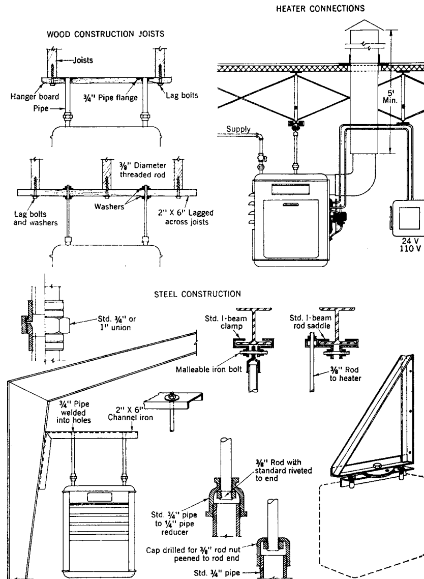
Fig 15-159. Details of gas fired heater installation
