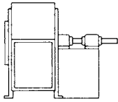
No. 1, SW, SI. For belt drive or direct connection. Wheel overhung. Two bearings on base.
