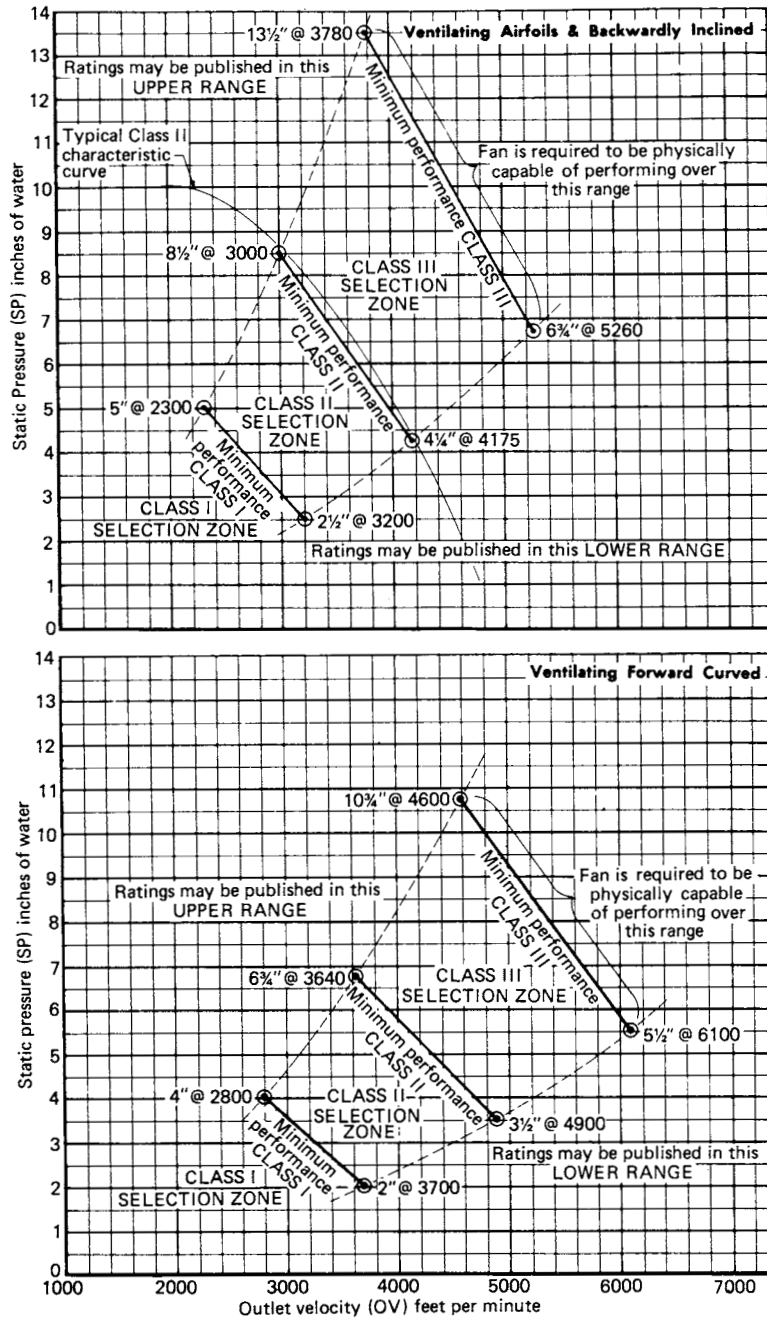
Fig 14-42. Operating limits for single width centrifugal fans
