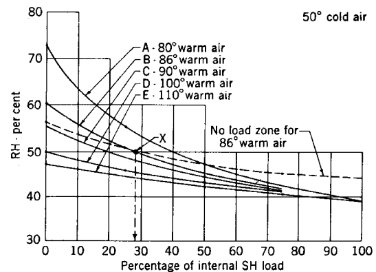
Fig 13-95. Performance over rate of internal sensible heat load; system of Fig. 13-88 and 13-89 for 50°F cold air
