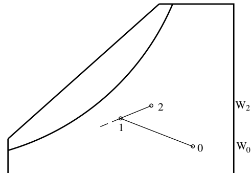
Fig 3-13. Psychrometric diagram for evaporative cooling system
