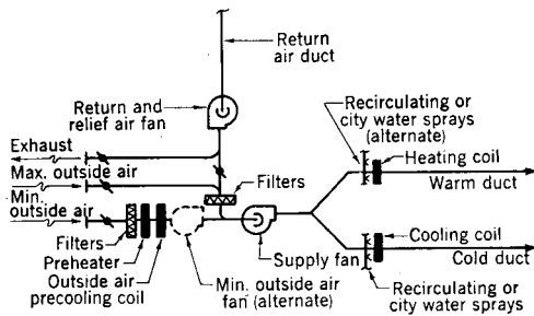
Fig 13-90. Single fan dual duct cycle with additional minimum outside air dehumidifier
