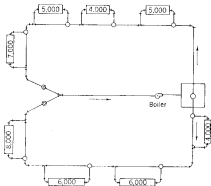
Fig 15-93. One pipe diversion loop system
