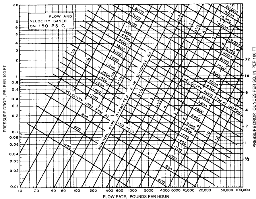
Fig 9-14. Flow rate and velocity of steam in Schedule 40 pipe at saturation pressure of 150 psig
