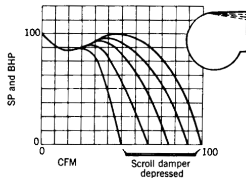
Fig 14-30. Effect of scroll dampers
