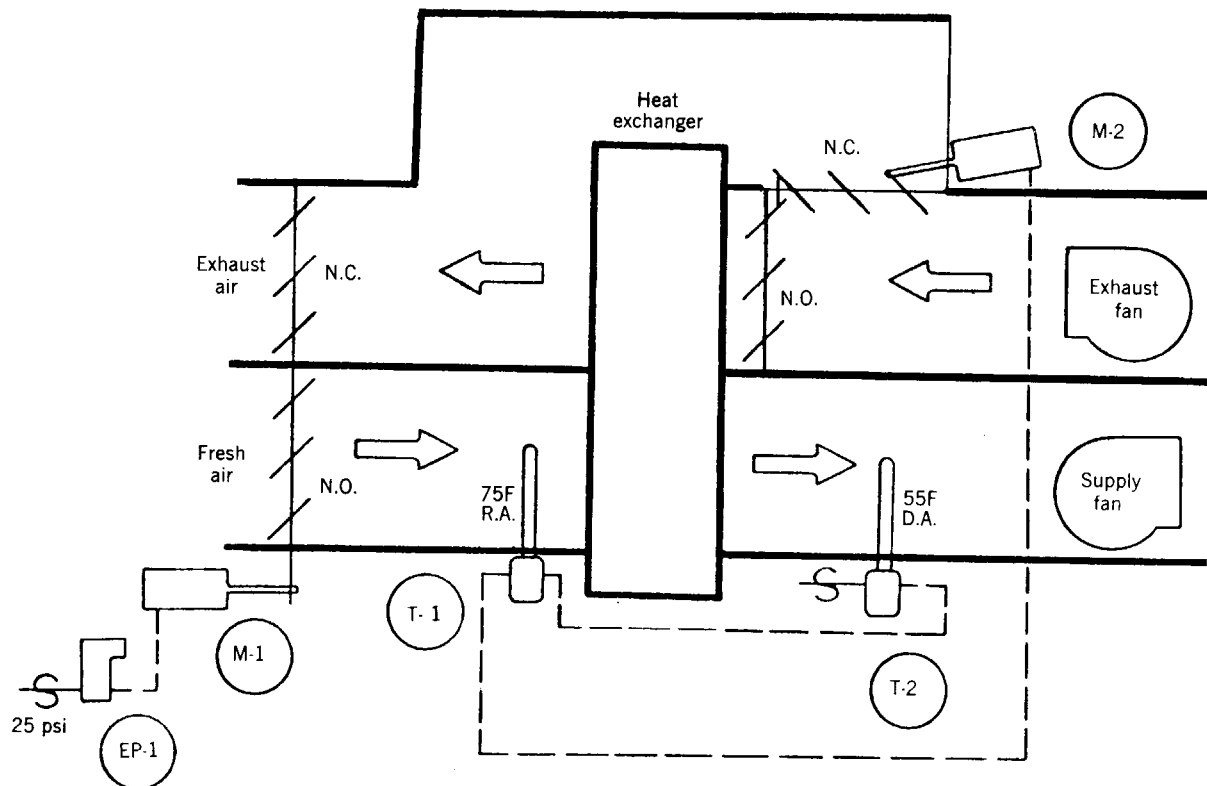
Fig 13-143a. Rotary air-to-air heat exchanger control, face bypass
