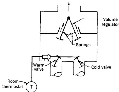
Fig 13-113. Type a duct constant volume unit
