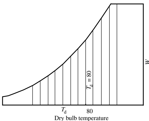
Fig 2-4a. Lines of constant dry bulb temperature t_d on the psychrometric chart
