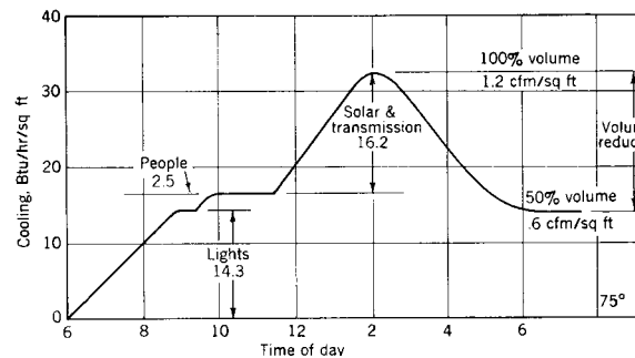
Fig 13-43. Load profile
