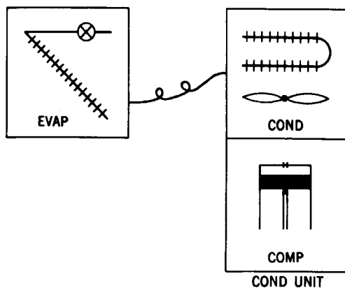
Fig 13-6. Split condenser and evaporator unit
