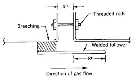
Fig 14-85. Expansion joint
