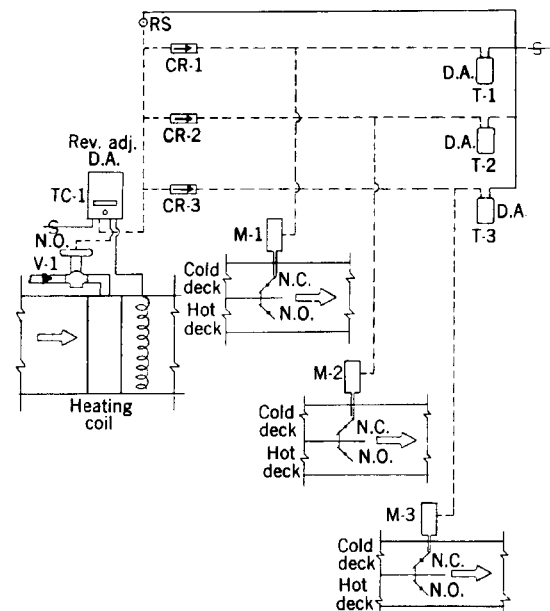
Fig 13-124. Zone mixing damper
