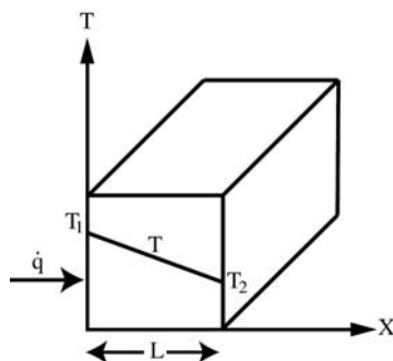
Fig 5-1. One-dimensional heat transfer by conduction
