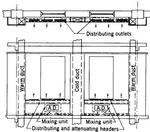
Fig 13-103. Arrangement of vertical, under window, dual duct units connected to risers, one unit per riser
