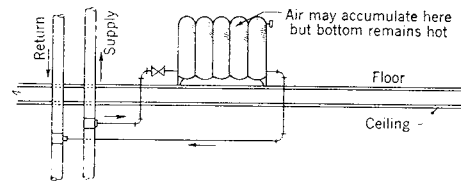
Fig 15-101. Preferred connection when radiation is above supply and return
