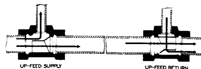
Fig 15-106. Flow through Bell & Gossett monoflow fitting upfeed supply and upfeed return
