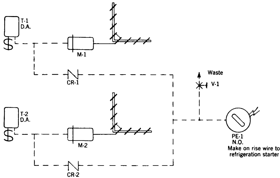
Fig 13-125. Refrigeration starting
