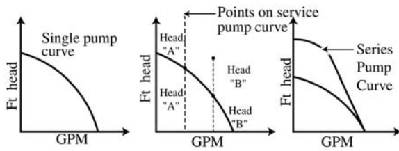
Fig 10-38. Series pump curve construction
