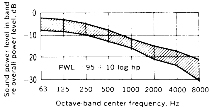
Fig 16-21. Sound spectrum for axial flow tower fans
