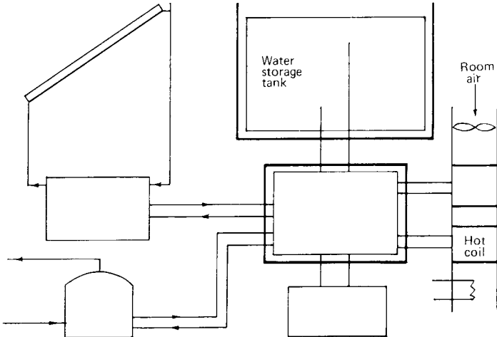
Fig 13-81. Direct solar heating
