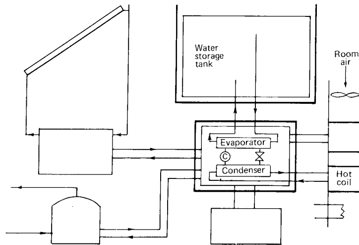
Fig 13-82. Solar augmented heat pump heating
