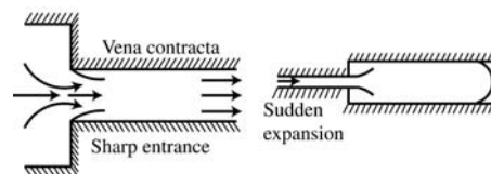
Fig 1-11b. Flow through sudden contraction or expansion
