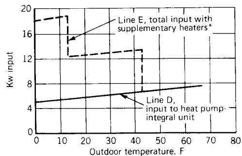
Fig 13-71. Electrical input for various outdoor temperatures
