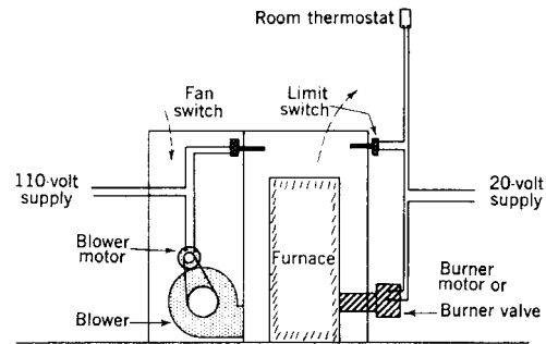
Fig 15-135a. Air velocity front of intake
