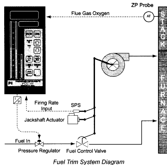
Fig 12-20. Fuel trim system diagram
