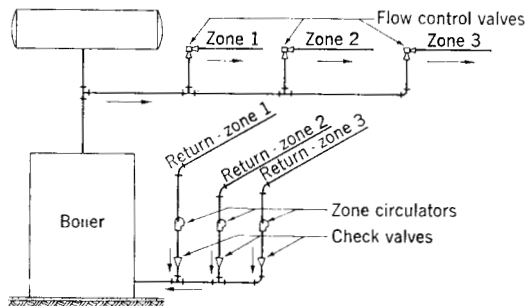
Fig 15-99. Schematic diagram shows proper use of both check valves and flow control valves
