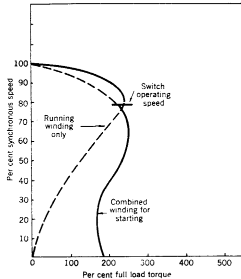
Fig 17-5d. Speed torque curve for a permanent split phase motor having a high starting current
