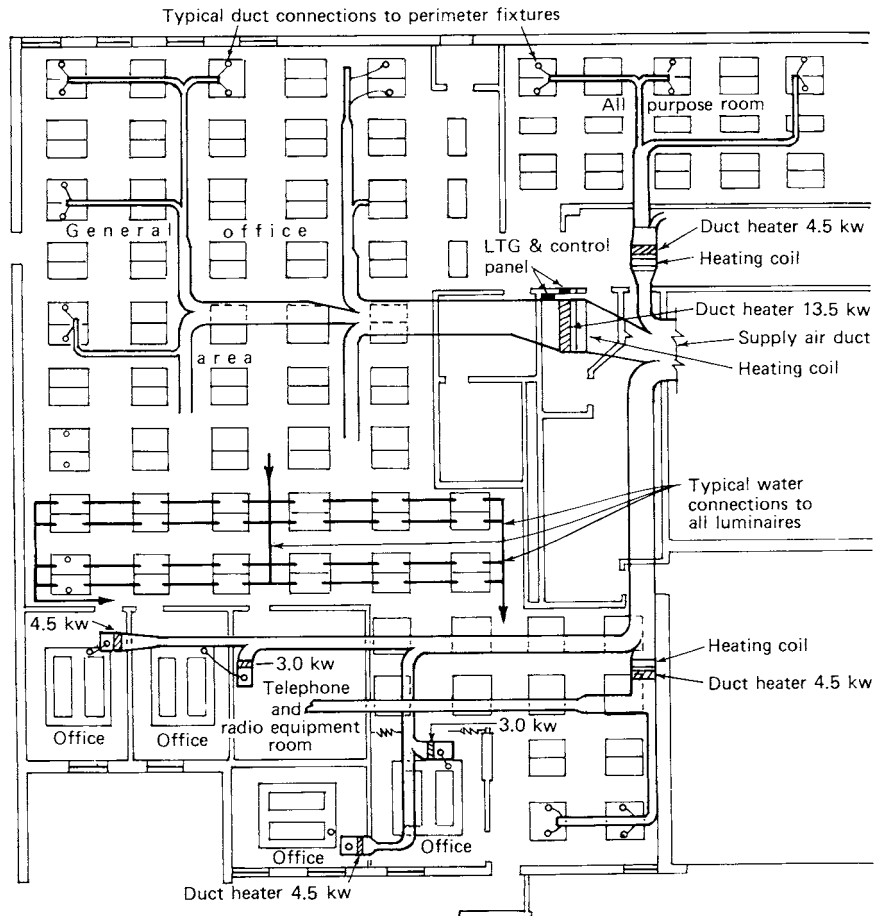
Fig 13-61. Integrated heat by light application
