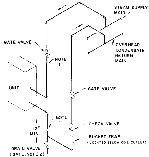
Fig 15-53. Condensate lift to overhead return
