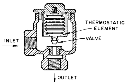
Fig 15-73. Thermostatic trap bellows type
