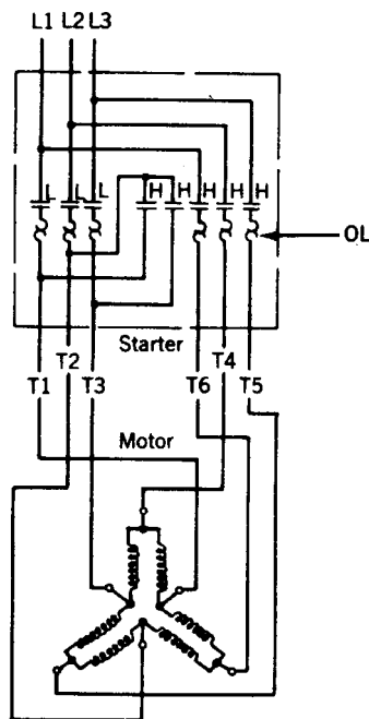
Two speed, single winding (consequent pole) consequent torque
