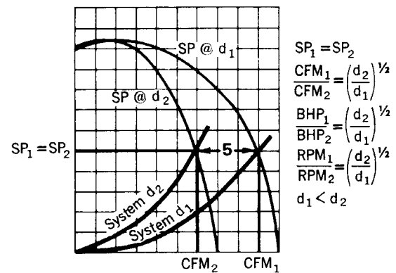
Fig 14-13. Fan law no. 5—density change (constant static pressure)
