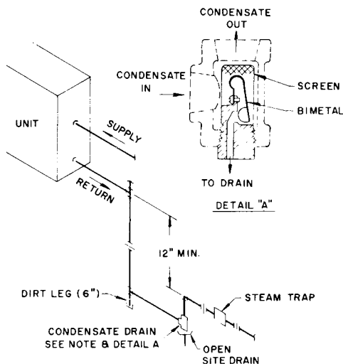
Fig 15-60. Freeze up protection for low pressure and vacuum systems
