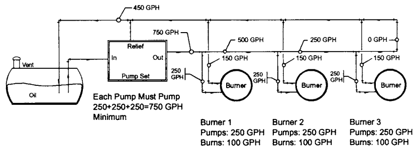
Fig 12-29. Burners piped in parallel
