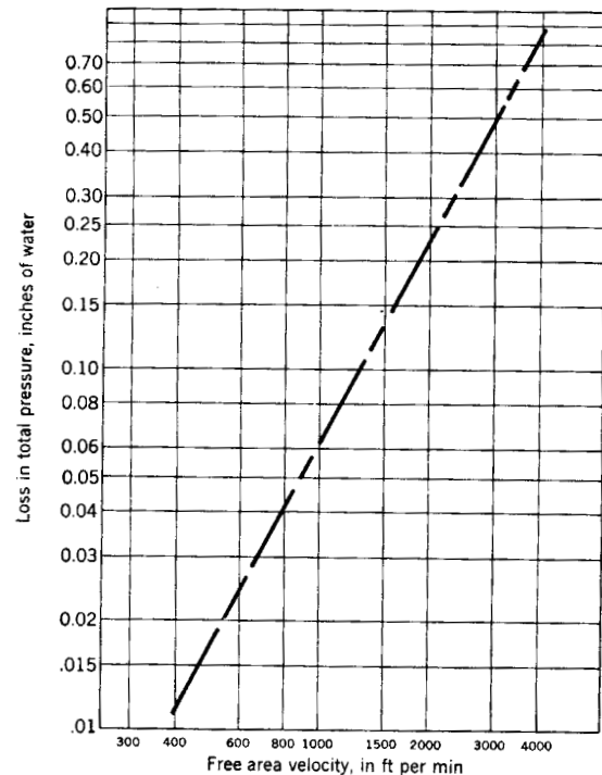
Fig 15-142. Total pressure loss of register as affected by free area velocity
