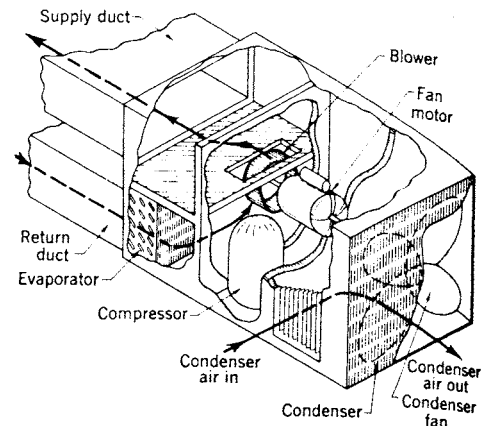
Fig 13-3. Horizontal self contained air conditioned unit
