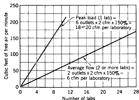
Fig 9-36. Compressed air charts
