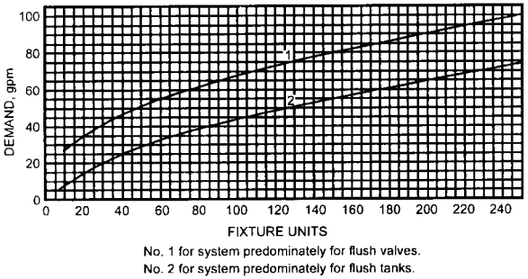
Fig 9-7. Estimate curves for demand load on enlarged scale
