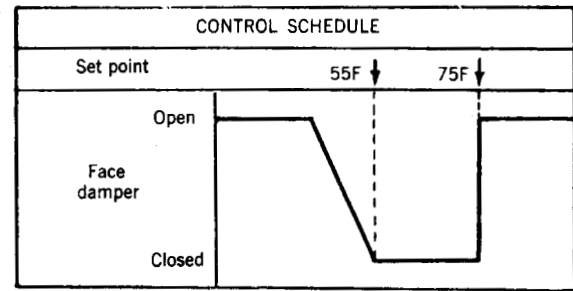
Fig 13-142a. Rotary air to air heat exchanger control, variable speed
