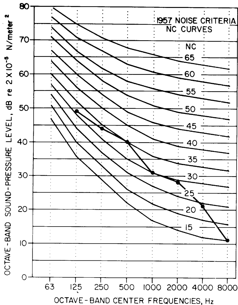
Fig 16-11. Determination of noise criteria for Example 1
