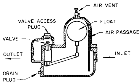
Fig 15-72. Float trap
