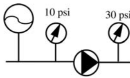
Fig 10-14. Effect of expansion tank location with respect to pump pressure
