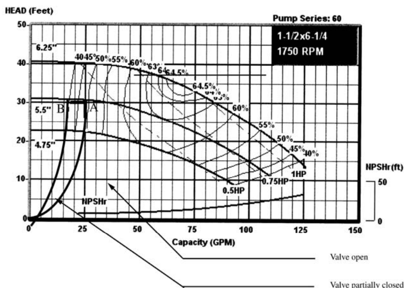
Fig 10-26. Pump curve for Series 60 B&amp;G inline pump
