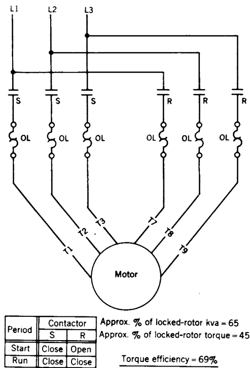
Fig 17-15. Part winding (one half winding start)
