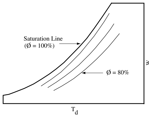
Fig 2-4e. Lines of constant relative humidity \phi on the psychrometric chart
