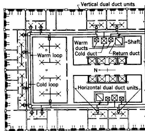
Fig 13-102. Typical office building dual duct layout 100% air stream zoned to provide selective temperature control for each enclosure with vertical duct units at exterior walls
