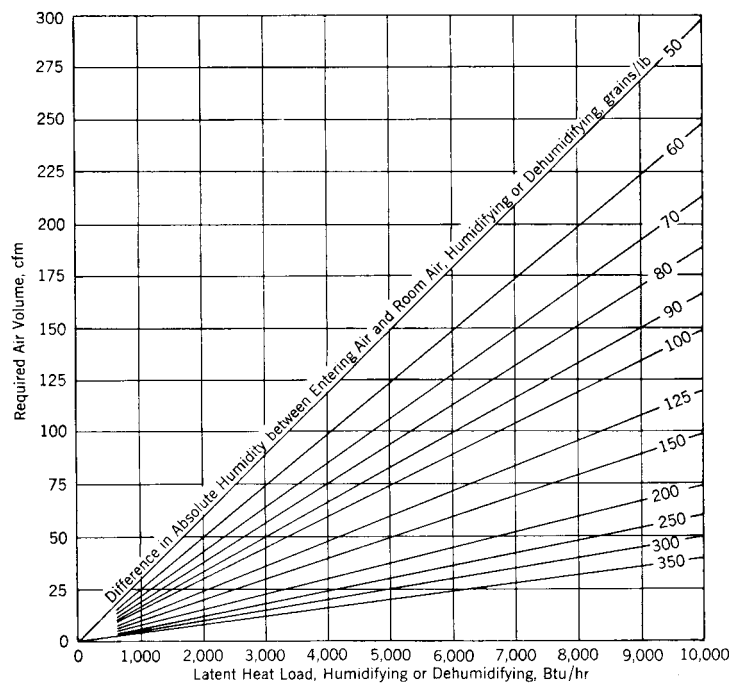
Fig 14-77. Air volume required to handle humidifying or dehumidifying loads
