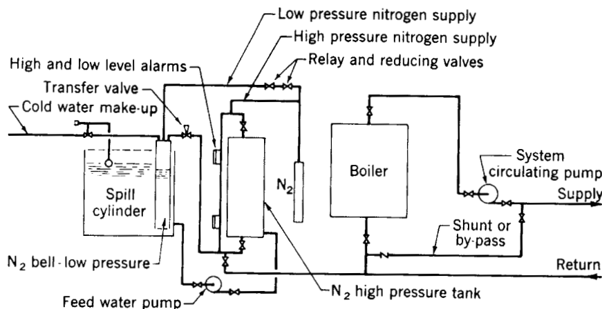
Fig 15-119. HTW system with bypass for light load condition
