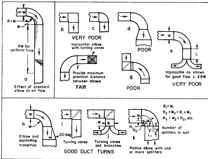
Fig 14-62. Duct turns
