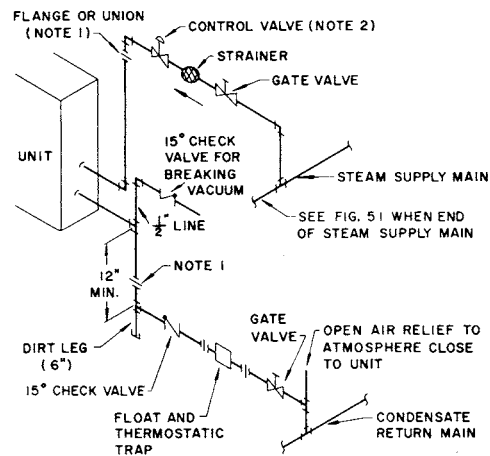
Fig 15-49. Single coil low pressure piping gravity return
