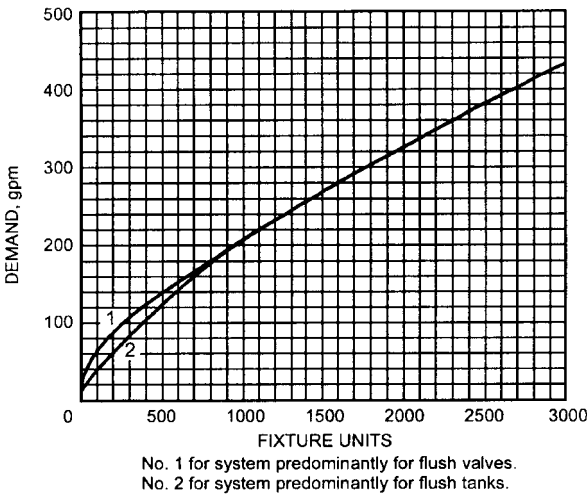
Fig 9-6. Estimate curves for demand load
