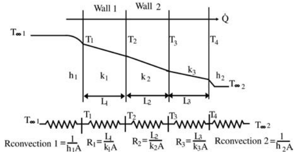
Fig 5-8. Heat transfer resistance
