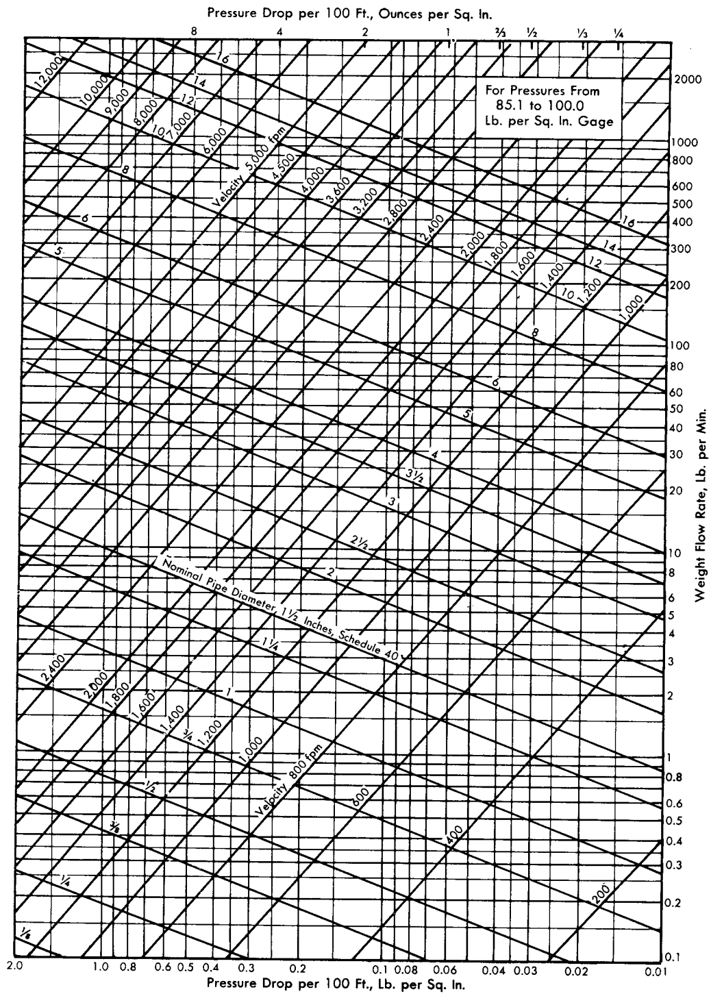
Fig 9-28. For pressure from 85.1 to 100.0 psig
