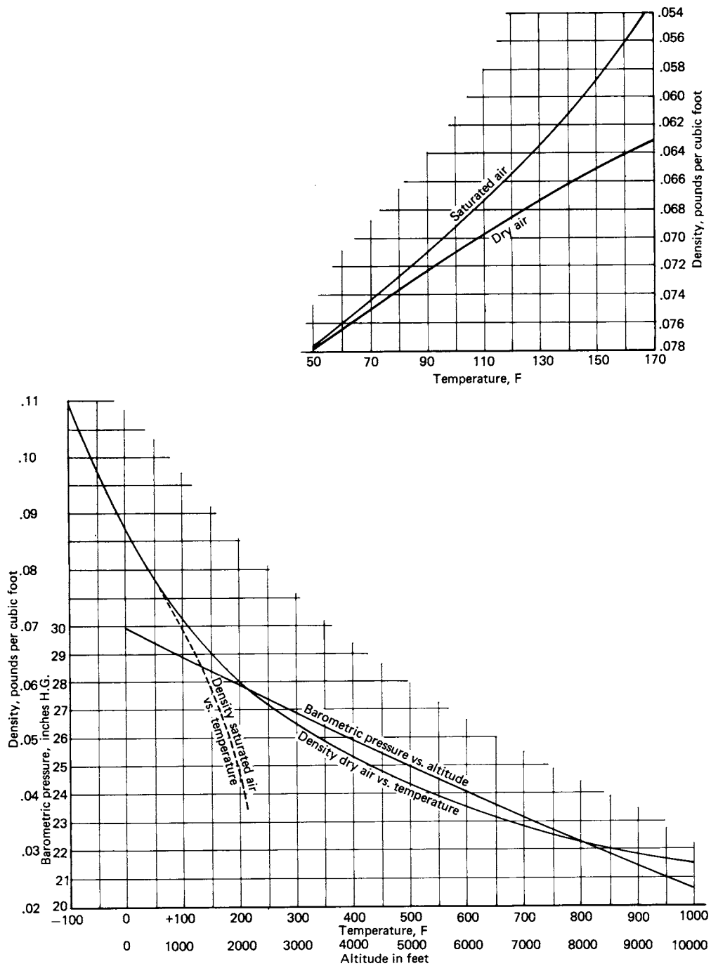
Fig 14-21. Density versus temperature and pressure versus elevation
