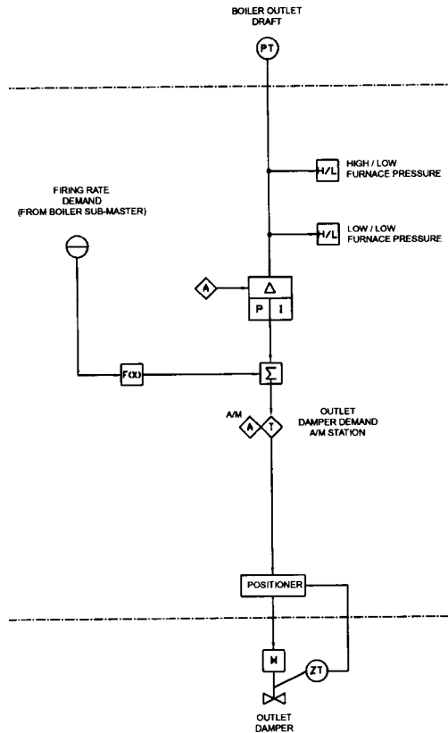
Fig 12-15. Draft system diagram
