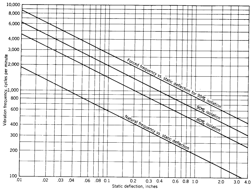
Fig 16-7. Isolation efficiency graph for cork, rubber, or felt mountings
