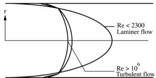
Fig 1-9. Laminar and turbulent velocity profiles in a circular duct
