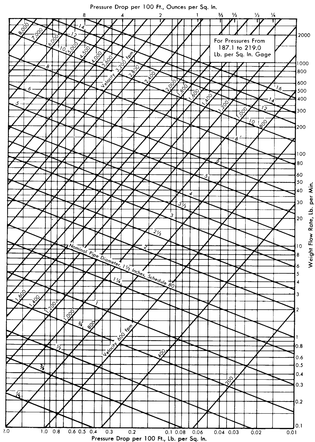
Fig 9-33. For pressure from 187.1 to 219.0 psig
