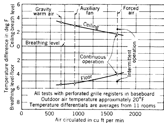
Fig 15-132. Average temperature differentials with gravity, auxiliary fan, and forced air systems
