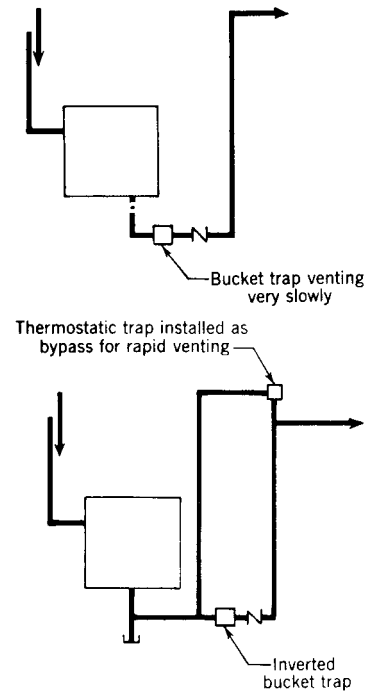
Fig 15-85. Cause and cure of airbinding
