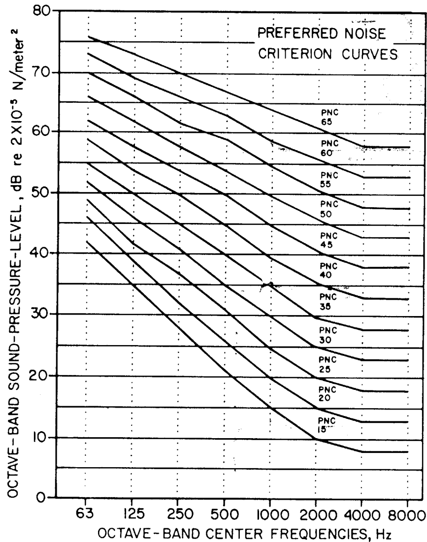
Fig 16-1. Preferred Noise Criteria Curves for determination of Permissible Broad Band background Sound Levels for indoor spaces
