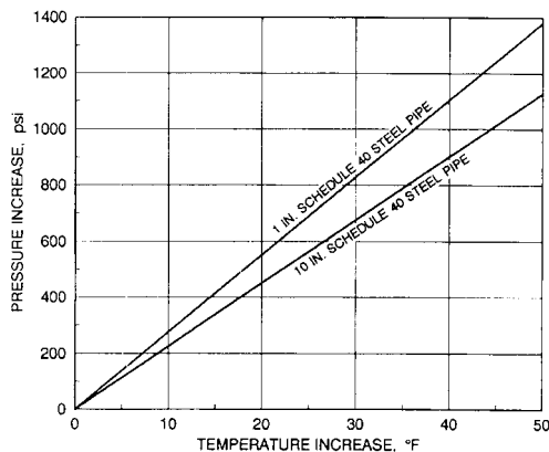
Fig 10-9. Pressure increase resulting from thermal expansion as function of temperature increase
