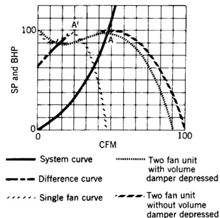
Fig 14-31. Elimination of paralleling
