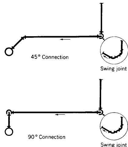
Fig 15-27. Connections to first floor heating units or riser
