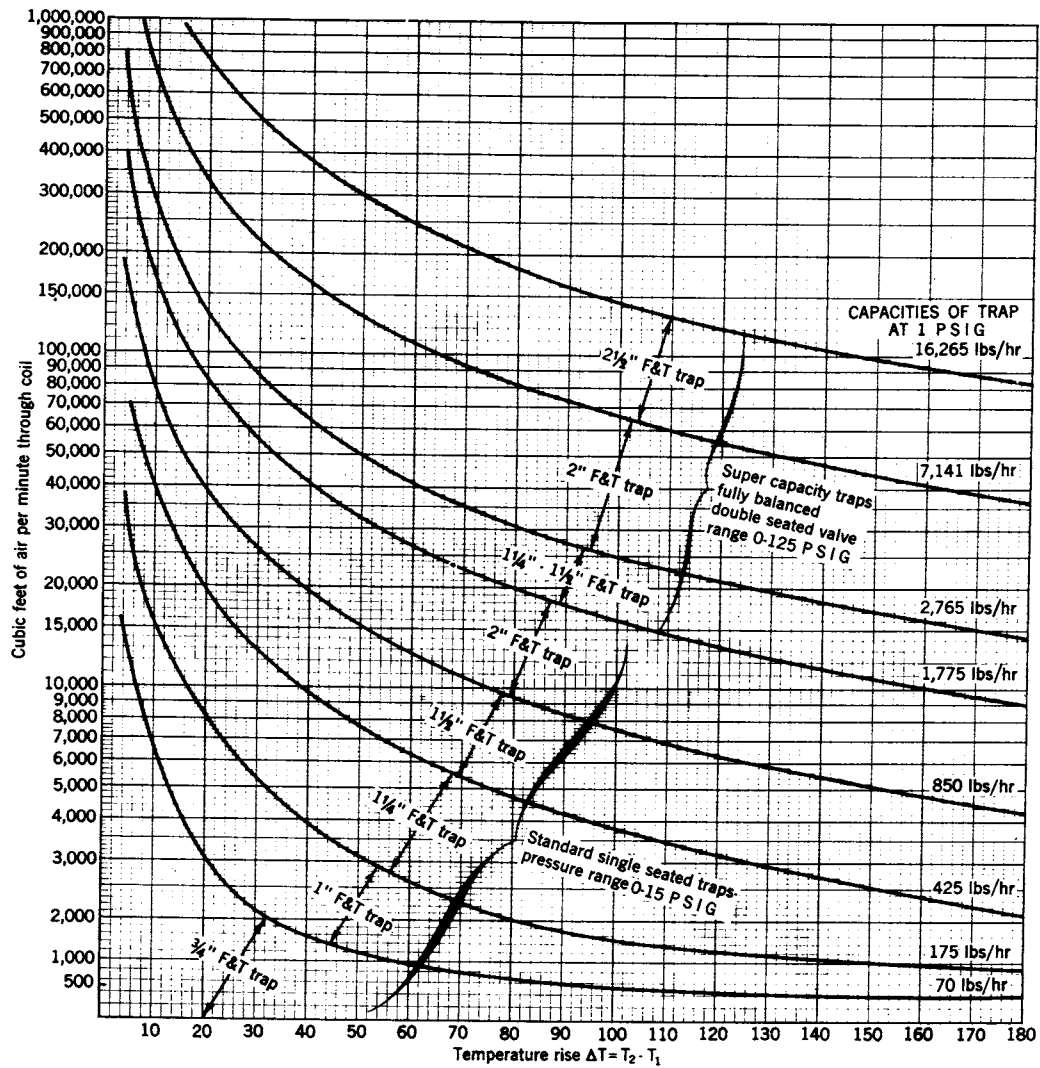
Fig 15-154. Sizing of steam traps
