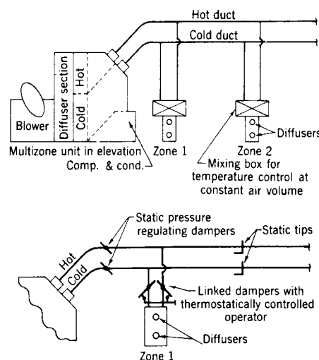
Fig 13-33. Multizone package serves in dual duct system
