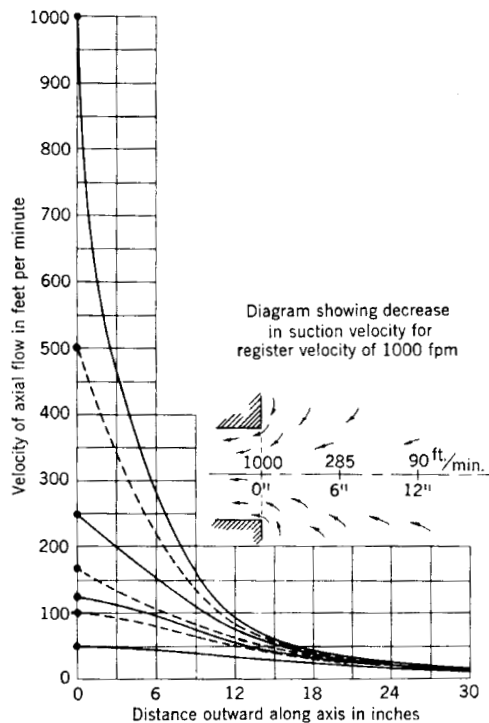
Fig 15-134. Air velocity front of intake
