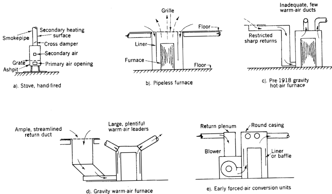
Fig 15-123. Development stages of forced air furnace
