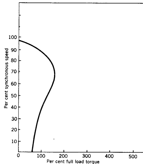
Fig 17-5e. Speed torque curve for a shaded pole motor
