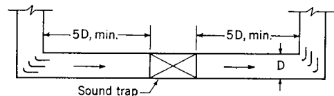
Fig 16-41. Locate sound traps with long straight inlet and discharge duct sections to provide best approach and leaving air pattern to trap
