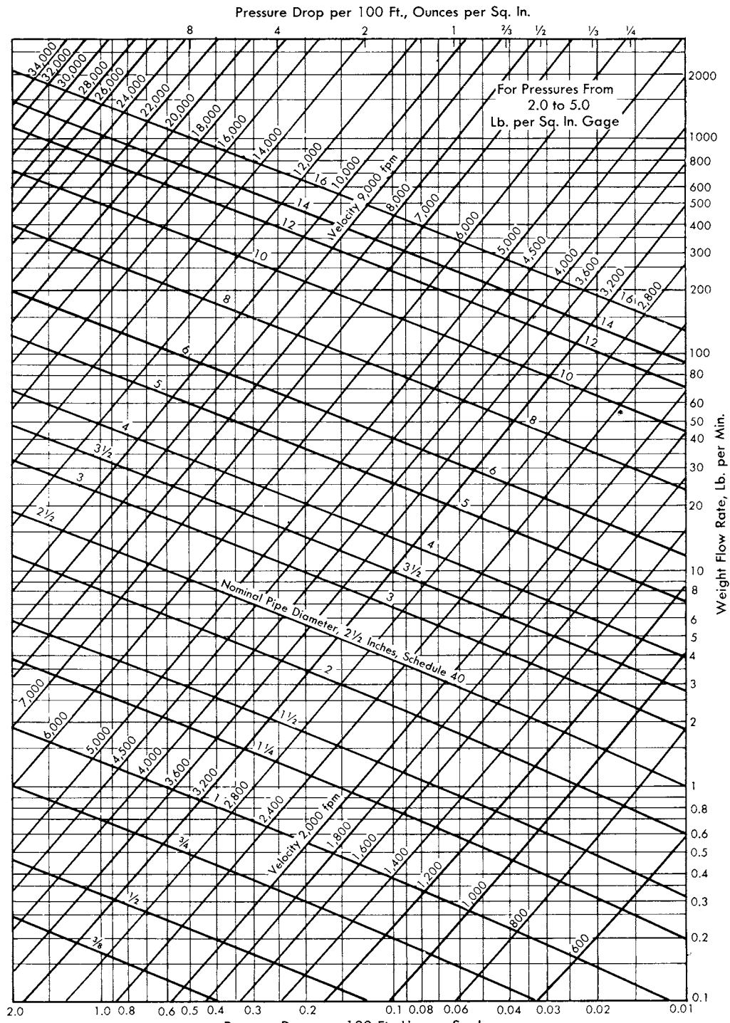
Fig 9-16. For pressure from 2.0 to 5.0 psig
