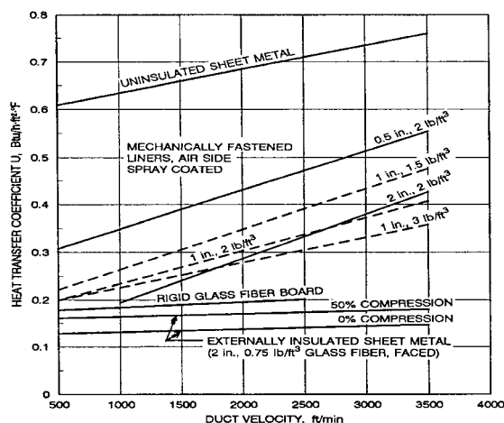
Fig 8-4a. Rigid ducts
