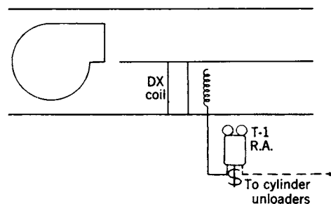
Fig 13-122. Control of cold plenum with cylinder unloader
