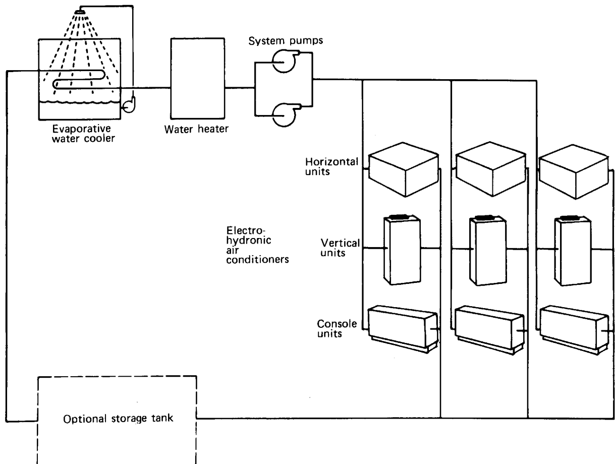
Fig 13-75. System water is cooled by evaporation of spray water, which is recirculated over the outside of the coil
