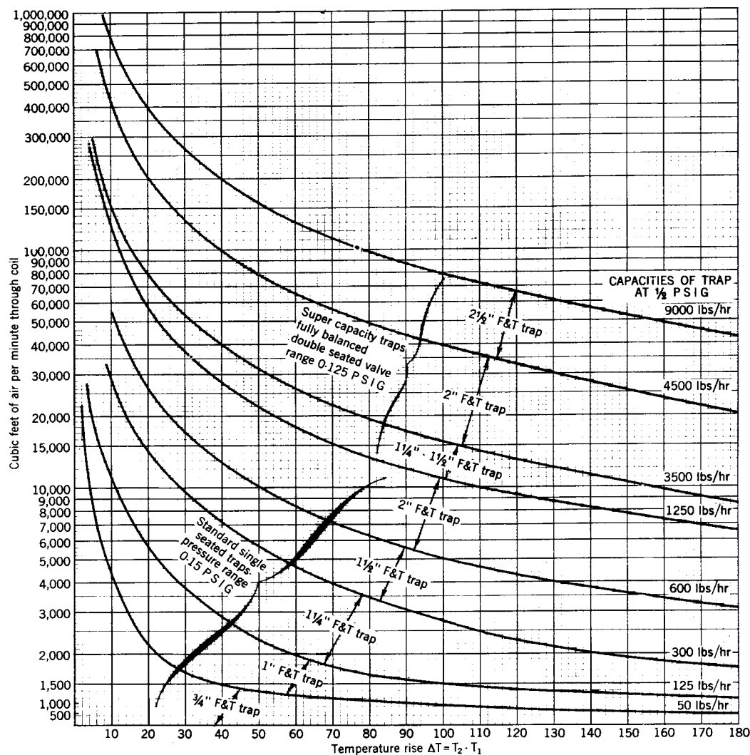
Fig 15-153. Sizing of steam traps
