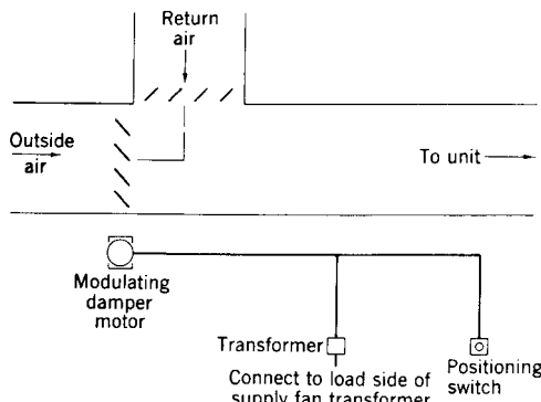
Fig 13-35. Most complex ventilation system with modulating damper motor
