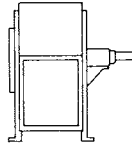
No. 2, SW, SI. For belt drive or direct connection. Wheel overhung. Bearings in bracket supported by fan housing.
