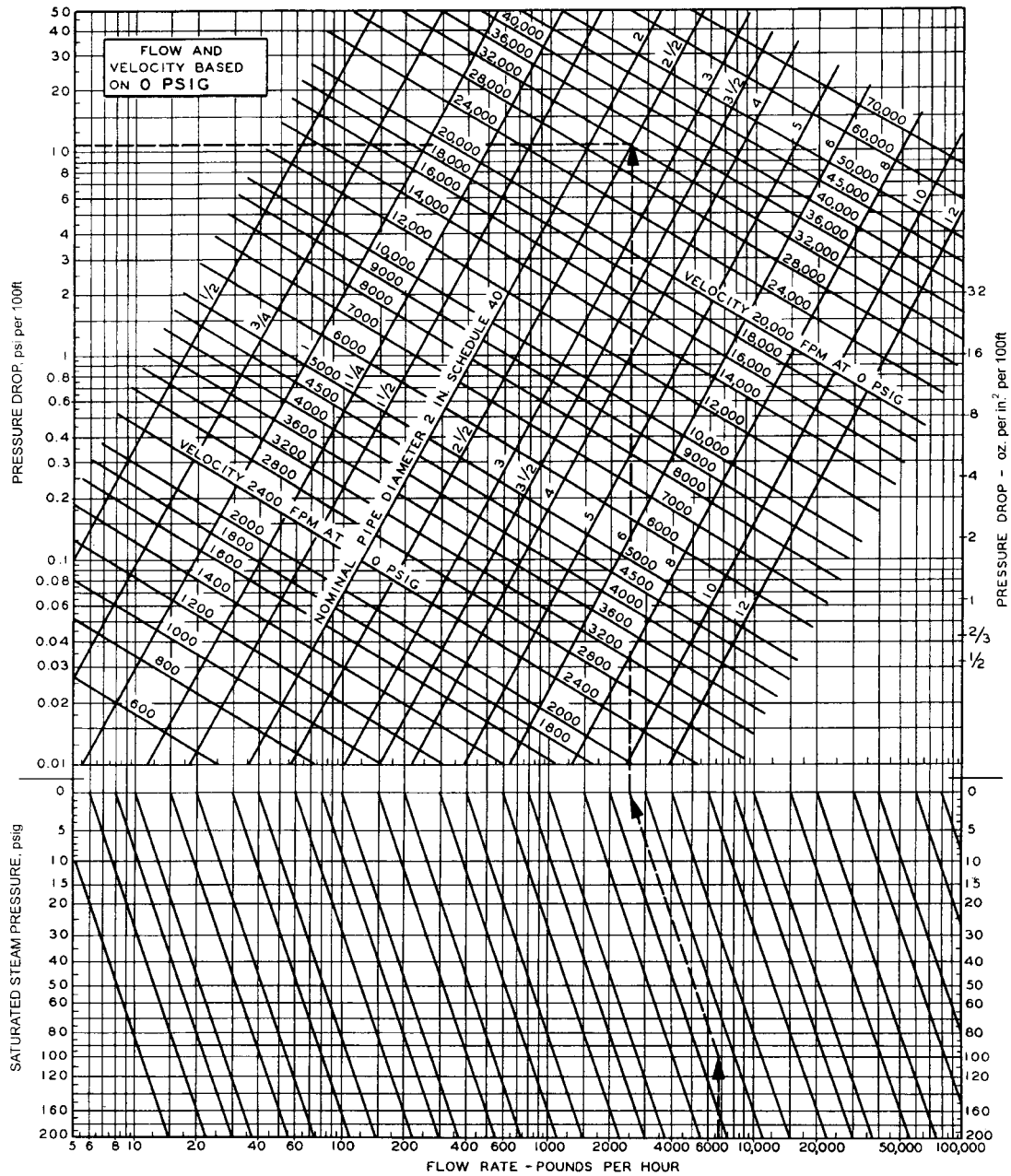
Fig 9-10. Flow rate and velocity of steam in Schedule 40 pipe at saturation pressure of 0 psig
