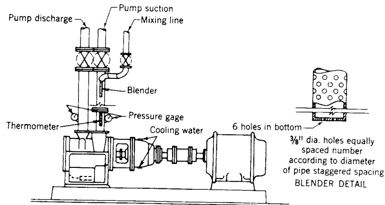
Fig 15-115. Mixing connection for steam pressurized HTW system
