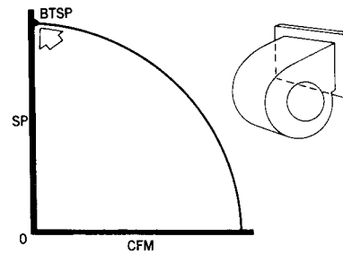
Fig 14-6. Blocked tight static pressure
