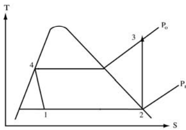
Fig 1-5a. Practical refrigeration cycle in (T,s) coordinates
