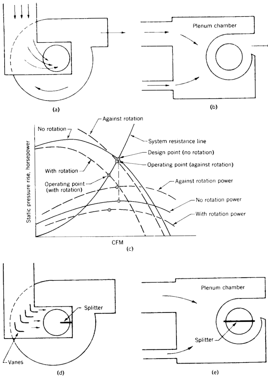
Fig 14-46. Fan inlet swirl (a) inertia of air tends to crowd it to bottom of inlet, setting up swirl. (b) with two unequal sized inlets to plenum chamber, imbalance is set-up, causing swirl at fan inlet. (c) effect of two-inlet swirl on fan performance. (d) vanes and splitter prevent swirl in inlet box. (e) a splitter overcomes the imbalance that is due to unequal inlets.
