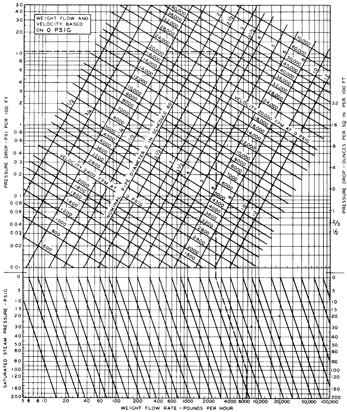
Fig 15-68. Pipe sizing
