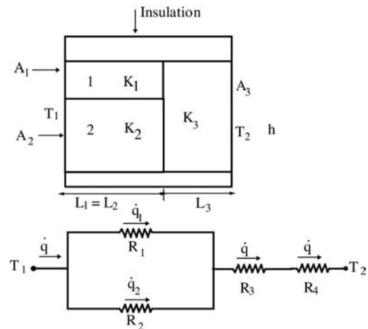
Fig 5-12. Thermal resistance network for combined arrangement
