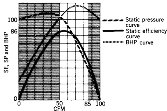
Fig 14-35. Characteristic curve for airfoil fans
