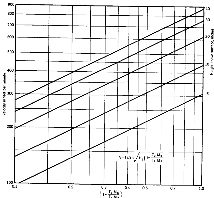
Fig 14-87. Calculation chart for determining theoretical convection velocity
