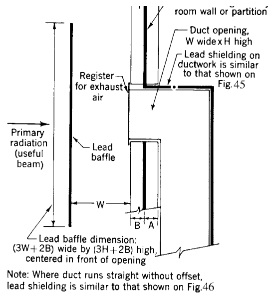
Fig 16-46. Elevation of section through X-ray room
