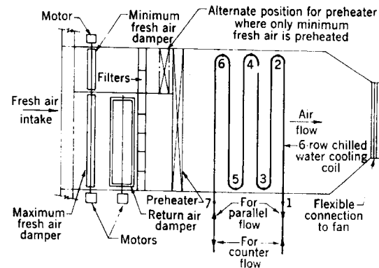
Fig 13-143. Schematic of a large central station air conditioning system
