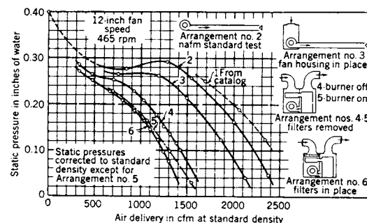
Fig 15-128b. Static pressure characteristics of a blower furnace combination
