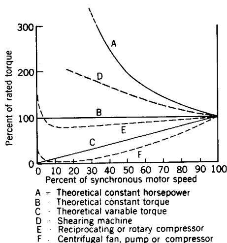
Fig 17-3. Load Torque Relationships for 100 hp, 1800 rpm motor; locked rotor kva/hp=5.52; Code letter F
