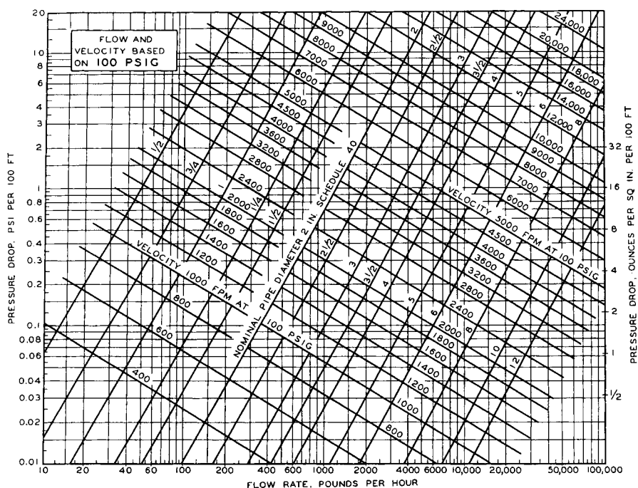
Fig 9-13. Flow rate and velocity of steam in Schedule 40 pipe at saturation pressure of 100 psig
