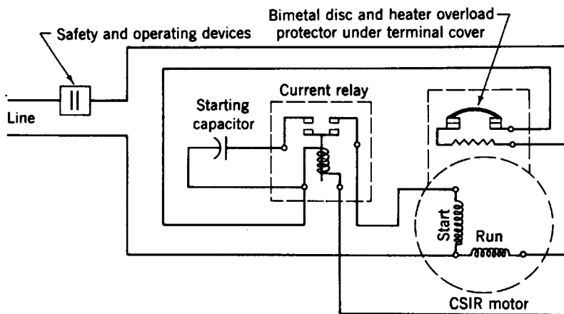
Fig 17-8. Current relay and overload with capacitor start, induction run motor
