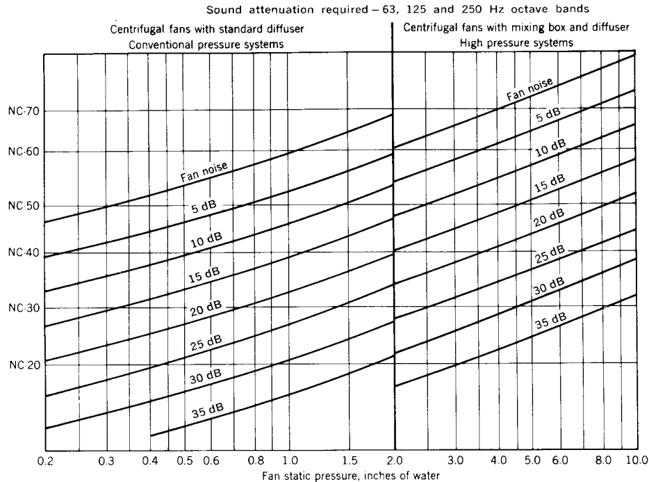
Fig 16-8. Sound Attenuation required 63, 125, and 250 Hz octave length
