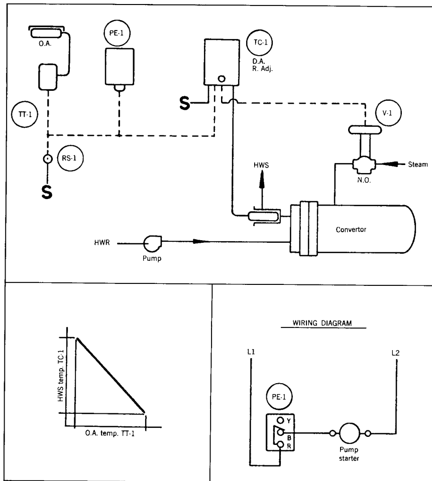
Fig 13-137. Hot water control with reset
