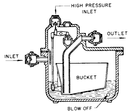
Fig 15-81. Lifting trap
