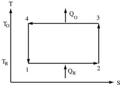
Fig 1-3. Carnot cycle
