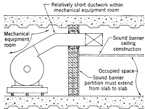
Fig 16-33. Ductwork is short, use special barrier
