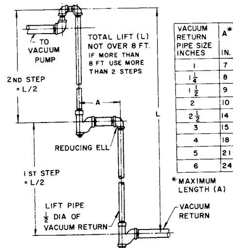
Fig 15-47. Two step condensate lift
