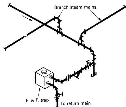
Fig 15-21. Splitting a single steam main into two mains with a drip
