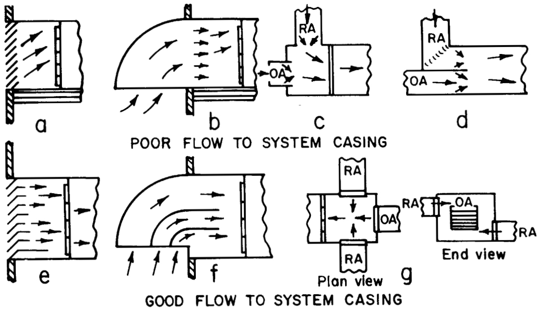
Fig 14-68. Flow to system casing
