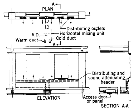
Fig 13-106. Perimeter header feed by horizontal unit
