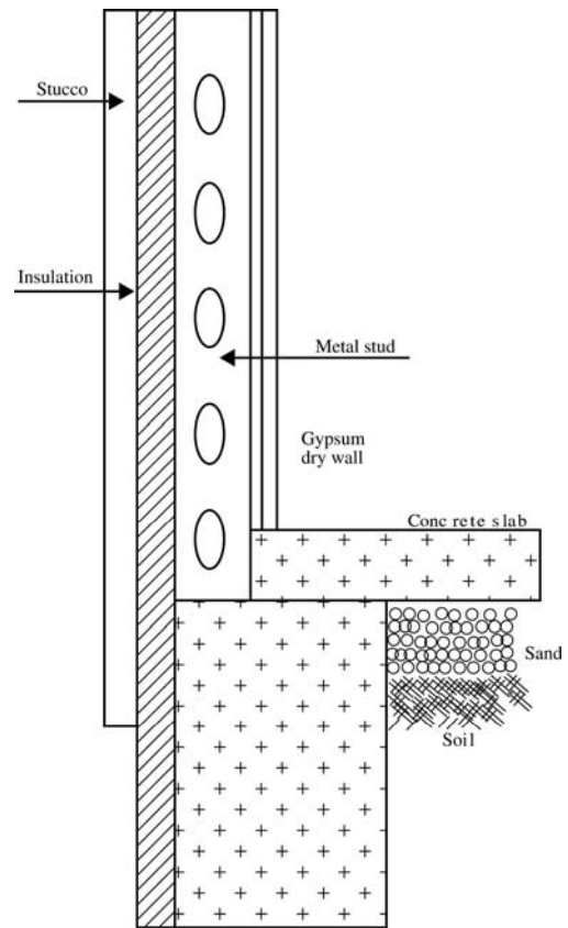
Fig 6-6. 4-inch block wall slab on grade foundation insulation
