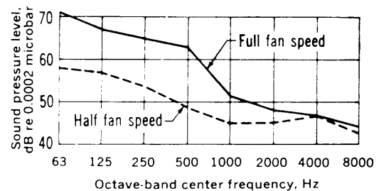
Fig 16-27. Effect of half speed operation
