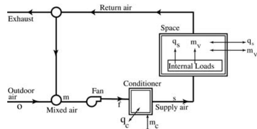
Fig 3-14. Air conditioning system
