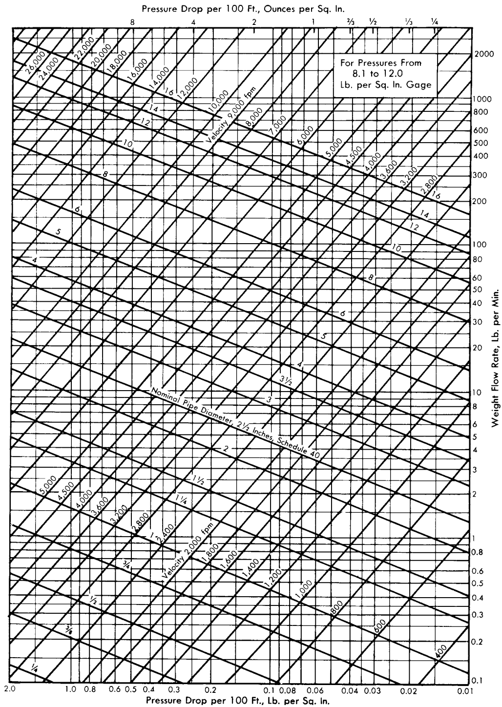
Fig 9-18. For pressure from 8.1 to 12.0 psig
