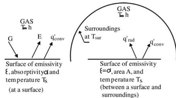
Fig 5-6. Radiation exchange
