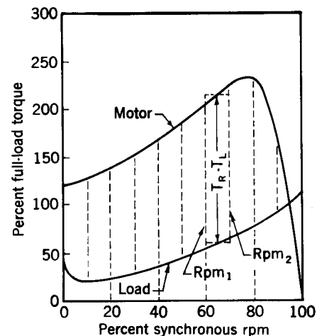
Fig 17-4. Dynamics of motor and load
