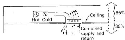
b. Combined fixture for both supply and return (35% energy enters room)
