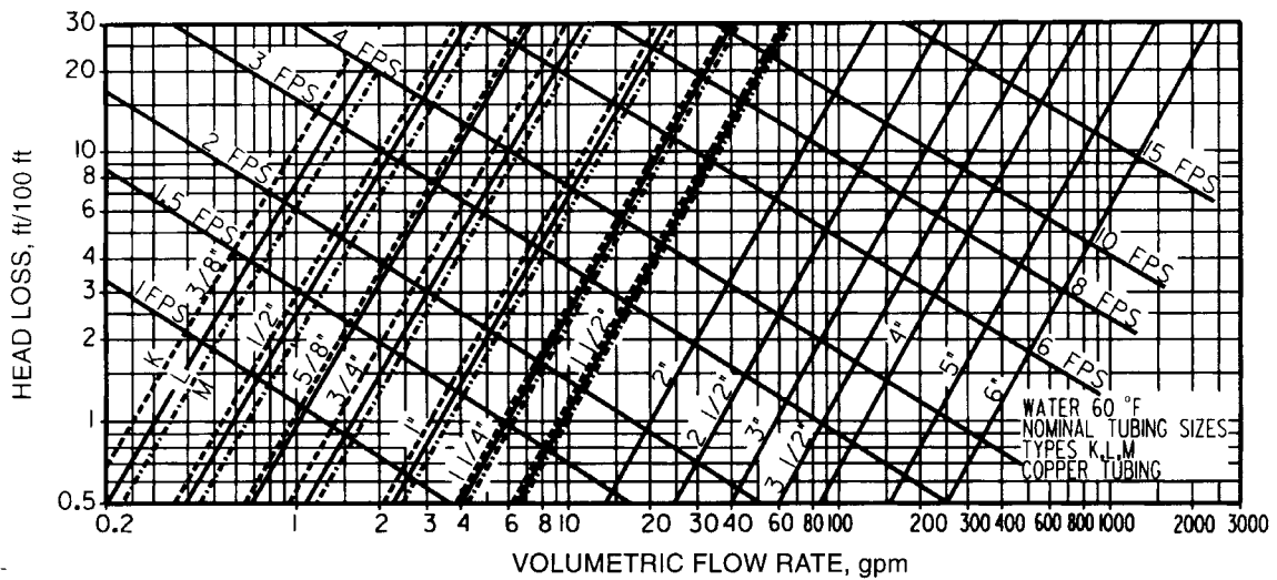
Fig 9-2. Friction loss for water in copper tubing (Types K, L, M)
