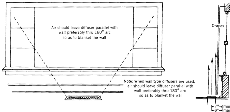
Fig 15-133. Location of floor diffuser below window
