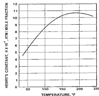
Fig 10-6. Henry's constant versus temperature for air and water
