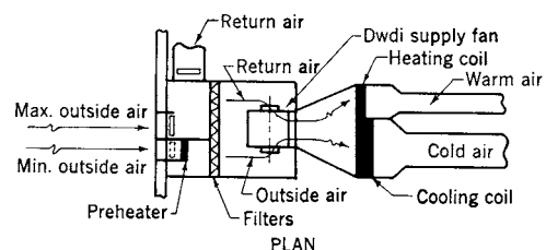
Fig 13-89. Single fan dual duct cycle with stratified air
