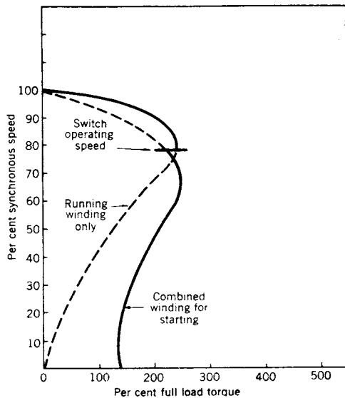
Fig 17-5c. Speed torque curve for a normal purpose split phase motor
