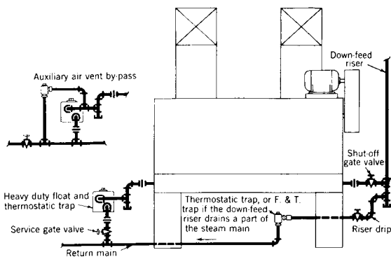
Fig 15-12. Piping connection for industrial type unit heater
