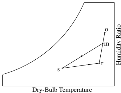
Fig 3-16. Air conditioning cooling system
