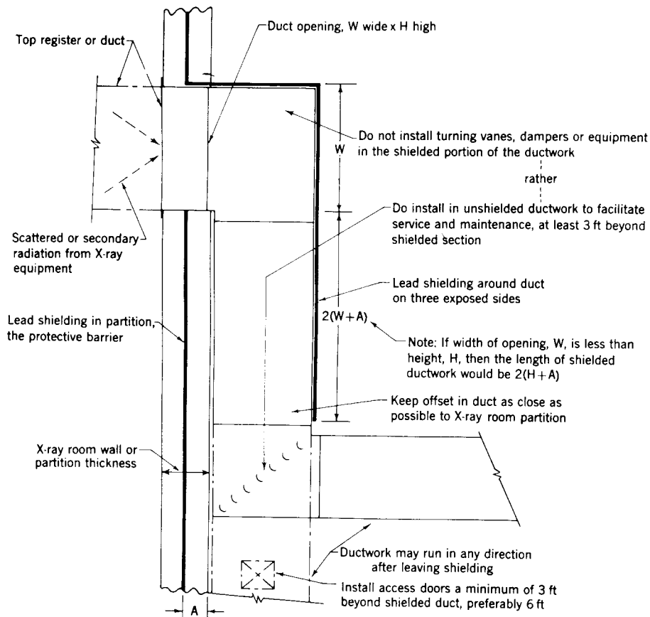
Fig 16-47. Plan view of duct running through partition of X-ray room, exposed to secondary or scattered radiation*
