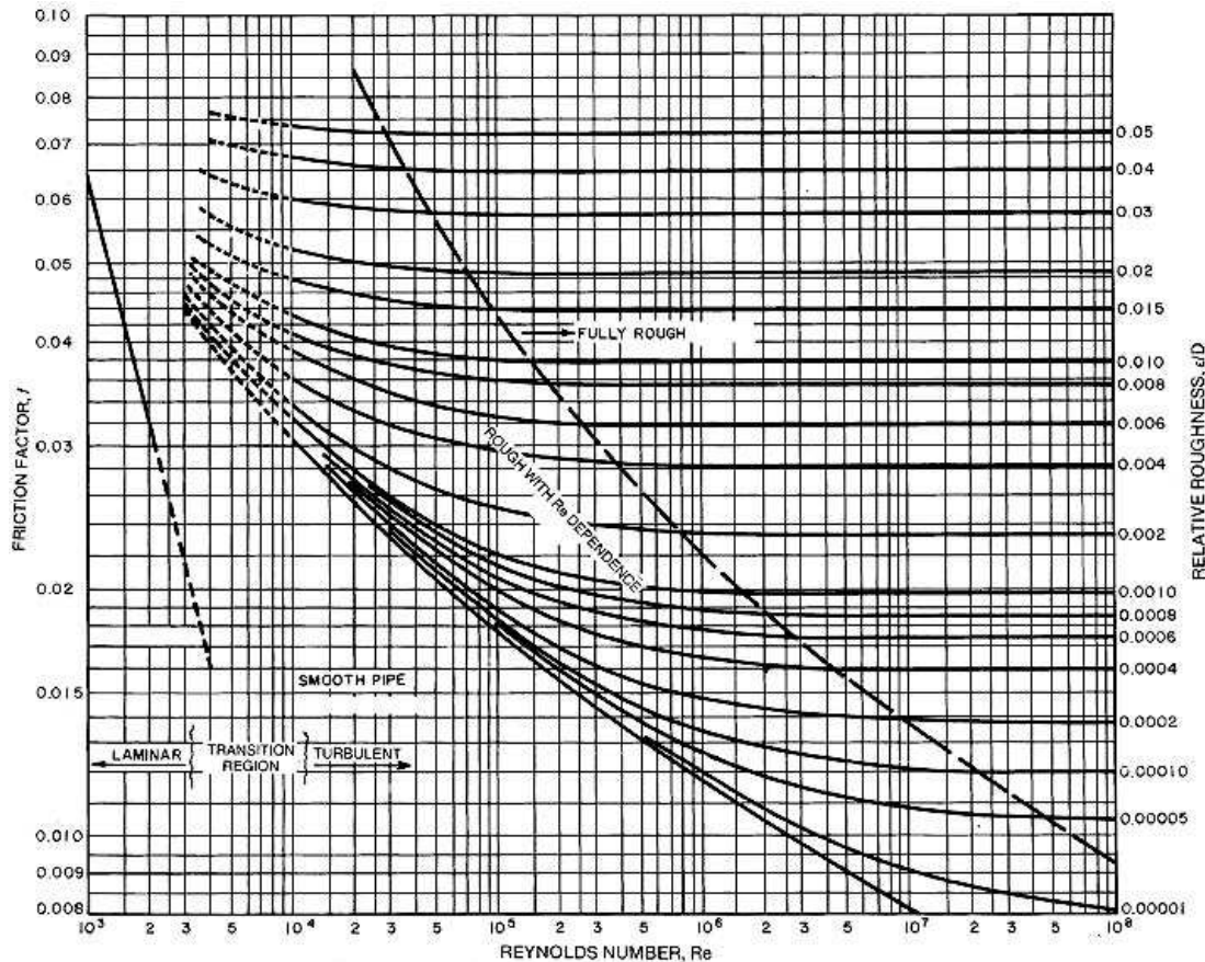
Fig 1-10. Friction factor (Moody's chart)
