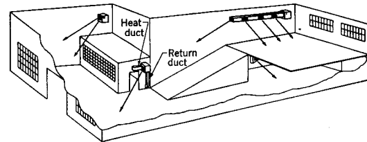
Fig 15-157. The same industrial area could be served by suspended blower type unit heaters shown in this manner. Gas lines and flutes are not shown.
