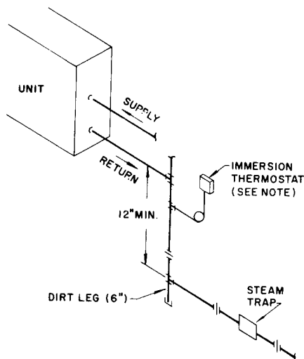
Fig 15-59. Freeze-up protection for high medium, low pressure and vacuum systems
