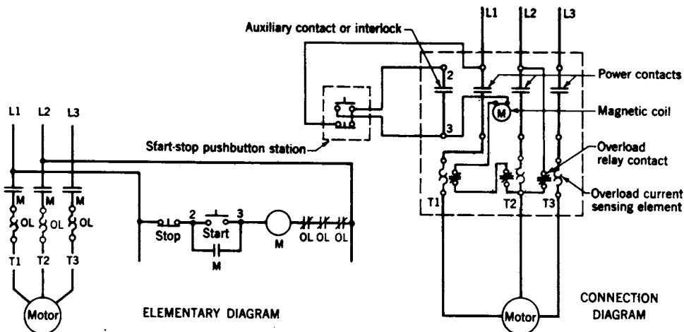
Fig 17-12. Full voltage size 1, 3-phase, magnetic starter; 3-wire control (low voltage protection)
