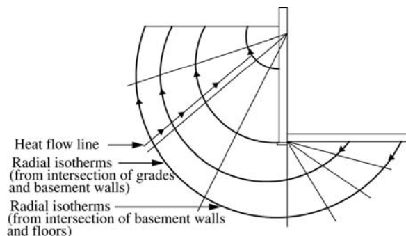
Fig 6-1. Heat flow from basement
