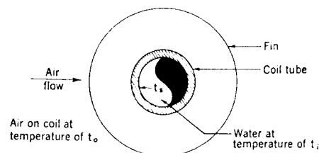
Fig 13-144. Section through a typical chilled water coil tube
