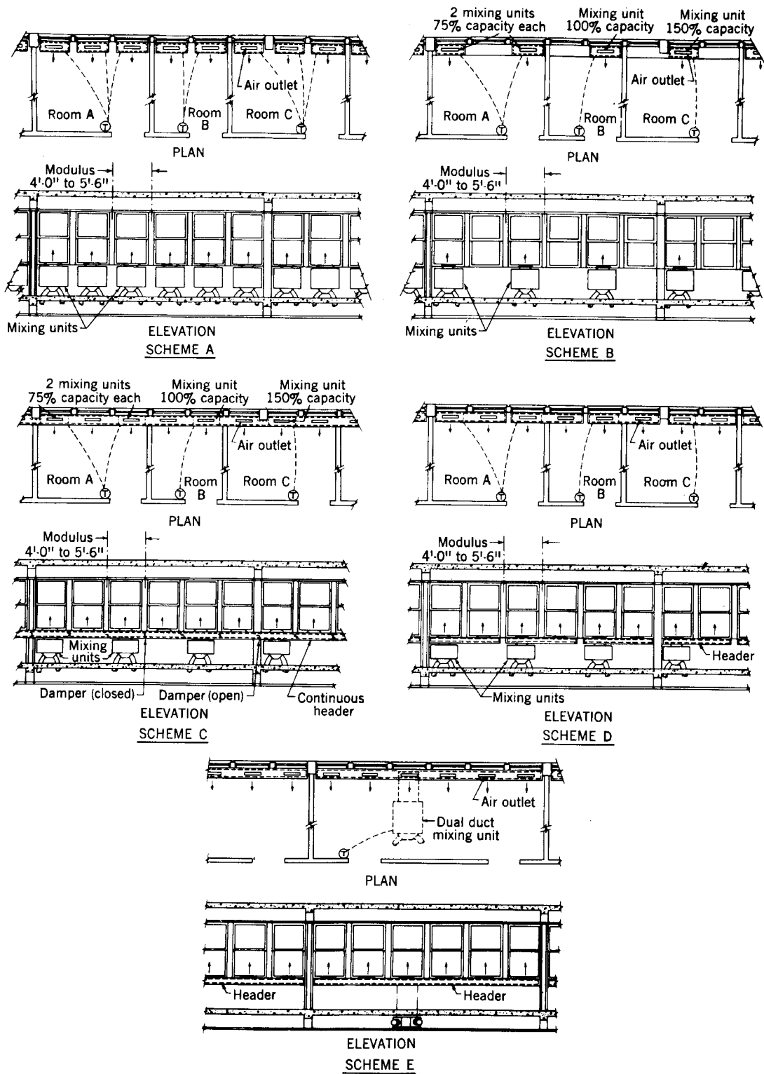
Fig 13-108. Modular arrangement of dual duct mixing units
