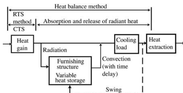
Fig 7-1. The difference between the instantaneous heat gain and instantaneous cooling load due to thermal storage
