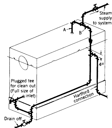
Fig 15-1. Single boiler with Hartford connection
