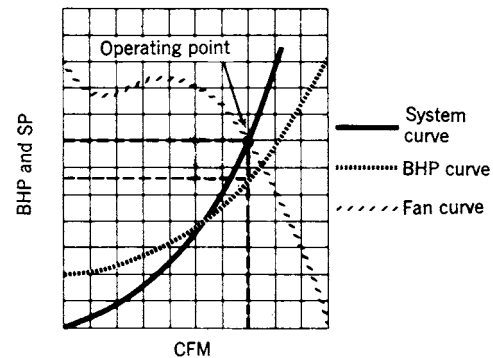
Fig 14-23. Operating point
