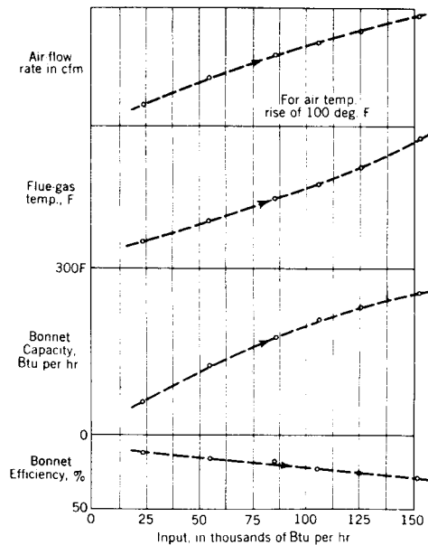
Fig 15-127. Typical trends of furnace performance tests
