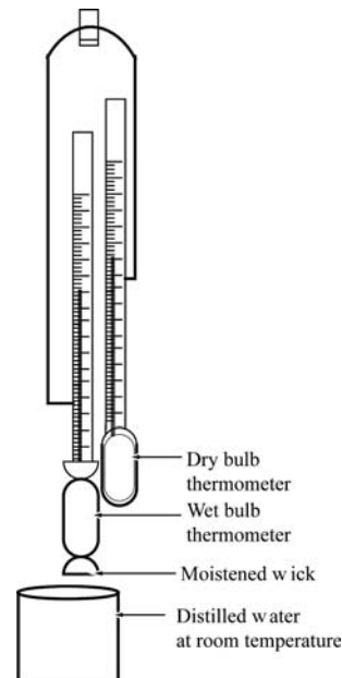
Fig 2-2. Sling psychrometer device for conveniently measuring wet and dry bulb temperatures
