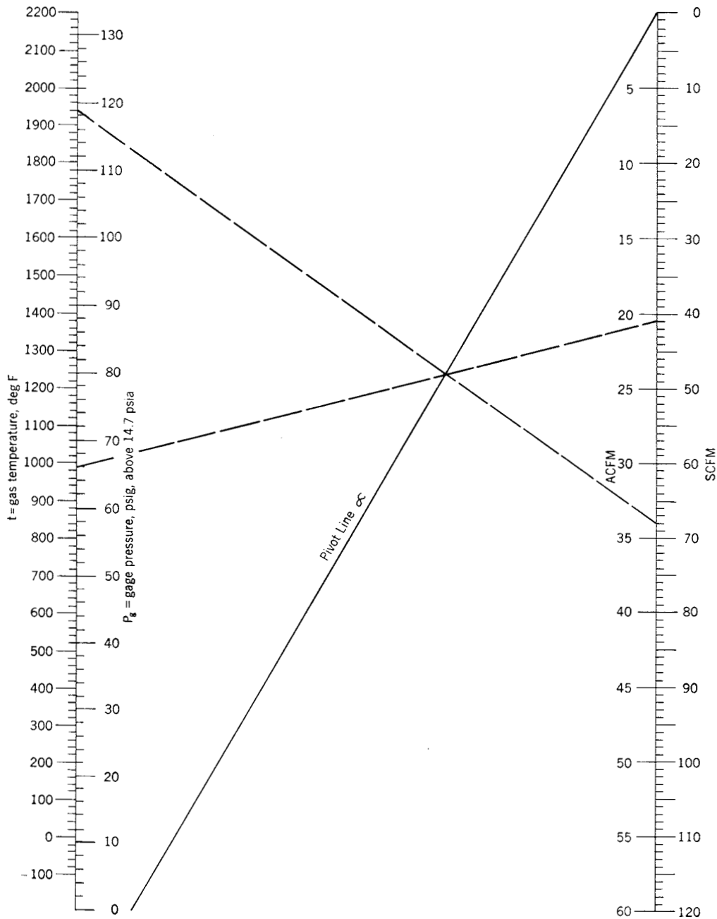
Fig 14-55. Nomograph for pressure and actual capacity in cfm
