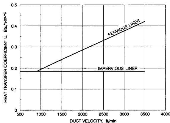
Fig 8-4b. Insulated flexible ducts
