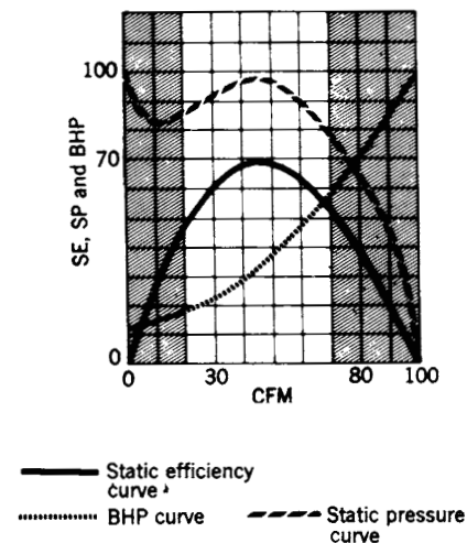
Fig 14-33. Characteristic curve for FC fans
