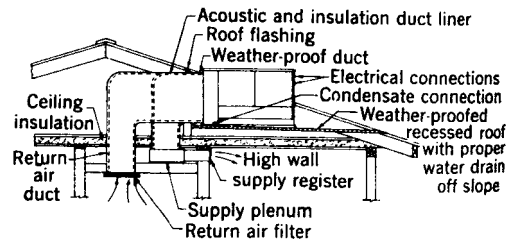
Fig 13-24. Dormer recess installation is less obtrusive
