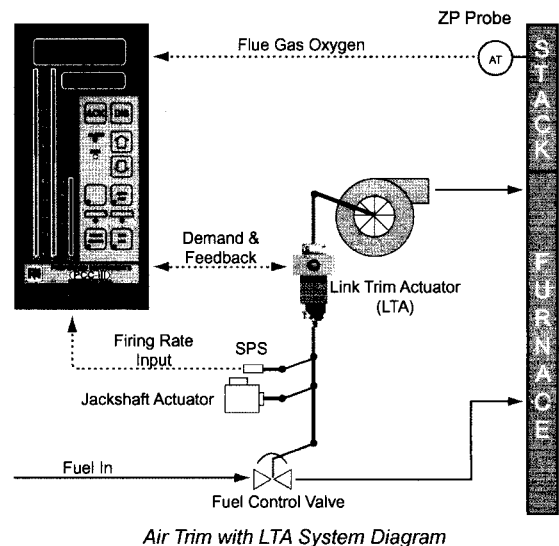
Fig 12-21. Air trim with LTA system diagram
