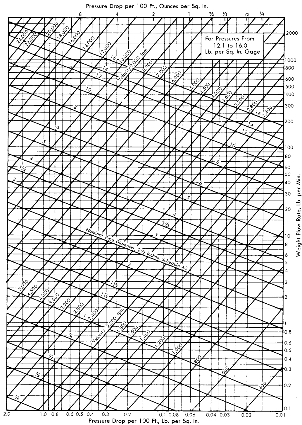
Fig 9-19. For pressure from 12.1 to 16.0 psig
