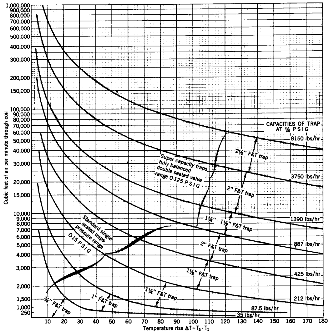
Fig 15-151. Sizing of steam traps
