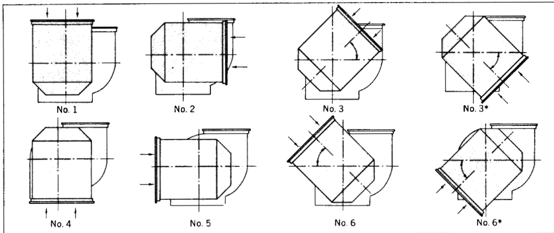
Fig 14-44. Designation of position of inlet boxes
