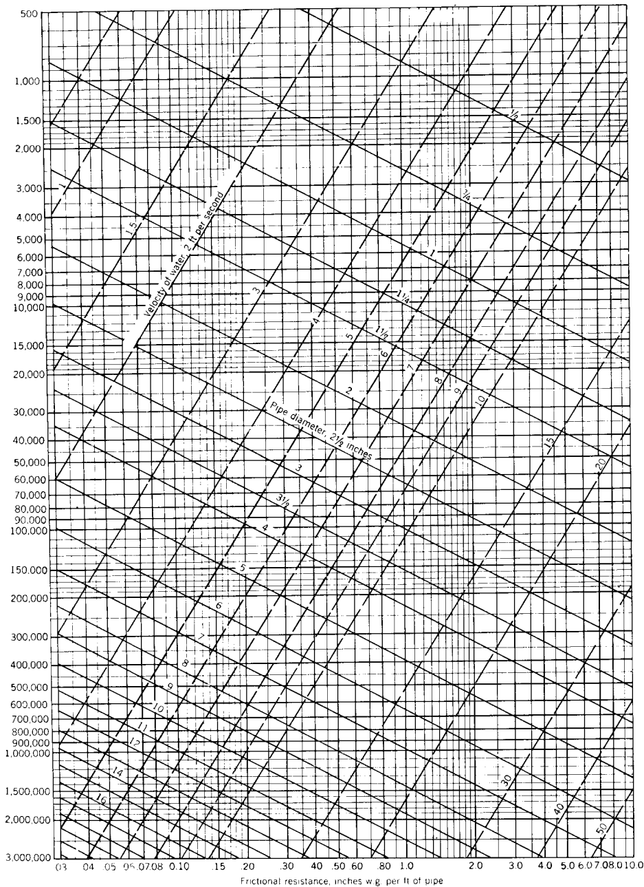
Fig 15-121. Frictional resistance of 300°F water in schedule 40 steel pipe
