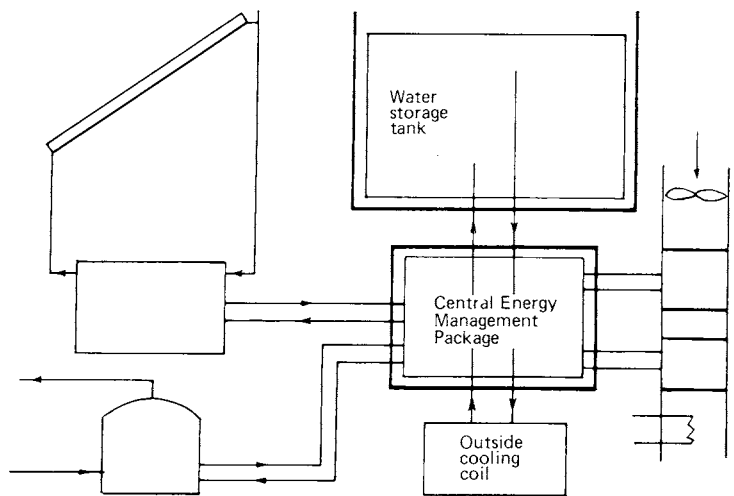
Fig 13-84. Winter to summer tank transition
