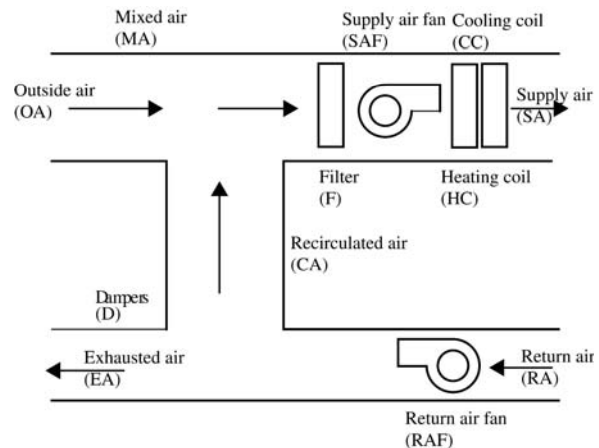
Fig 5-16. Simple all-air-handling unit with associated airflows
