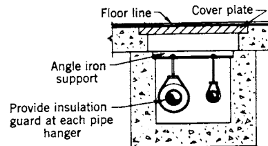
Fig 15-35. Anchoring steam supply piping
