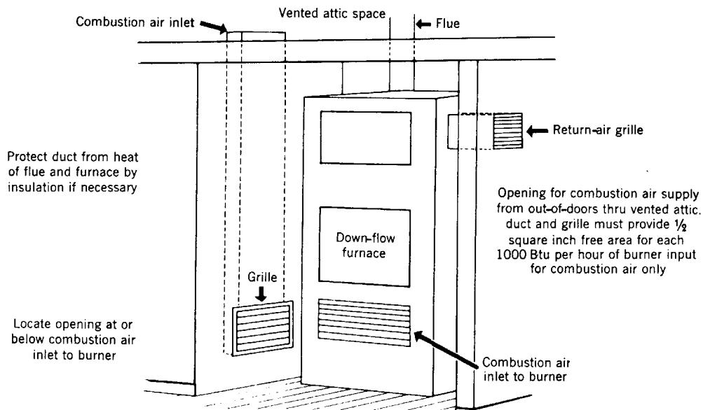
Fig 15-136a. Combustion air supply from attic space
