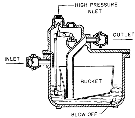
Fig 15-80. Impulse trap
