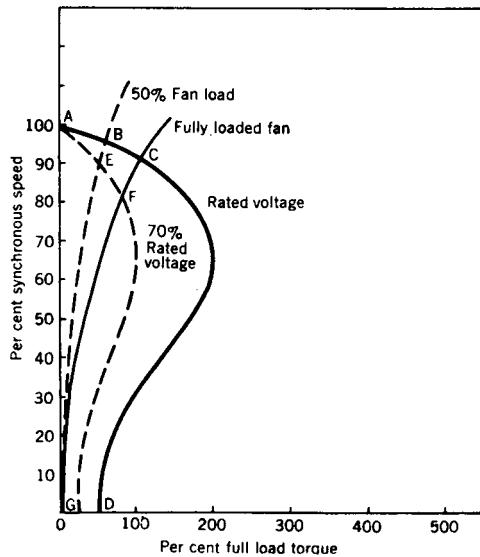
Fig 17-5b. Speed torque curve for a permanent split capacitor start motor
