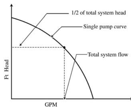
Fig 10-37. Basic series operation single pump curve
