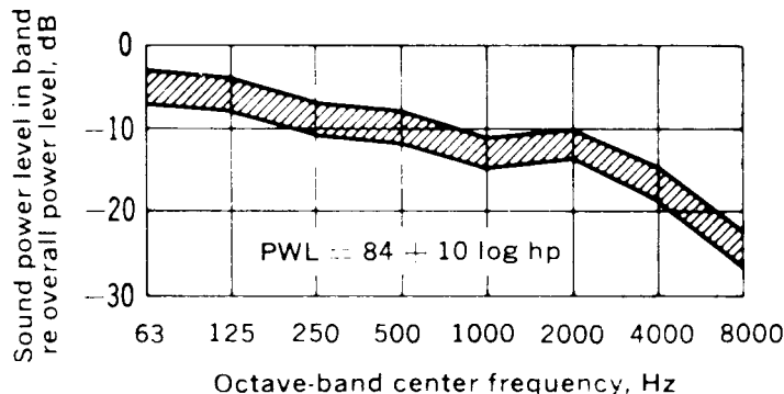
Fig 16-22. Sound spectrum for centrifugal flow tower fans
