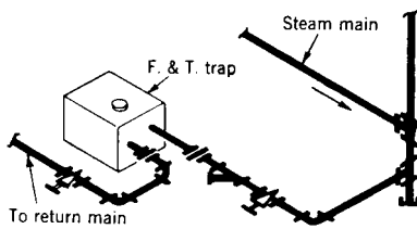
Fig 15-23. Details of main supply riser drip
