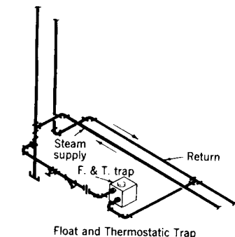
Fig 15-25. Supply riser drip connection
