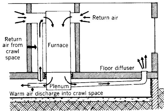
Fig 15-135e. Downflow furnace with crawl space duct system and crawl space plenum system
