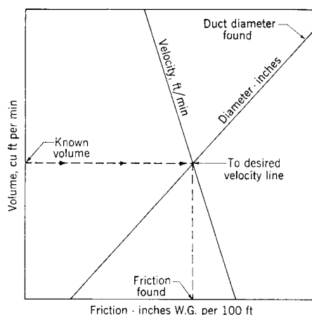
Fig 14-60a. Finding diameter and friction from known volume and velocity
