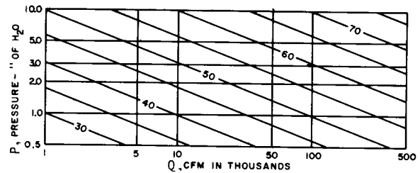
Fig 16-12. Correction factors
