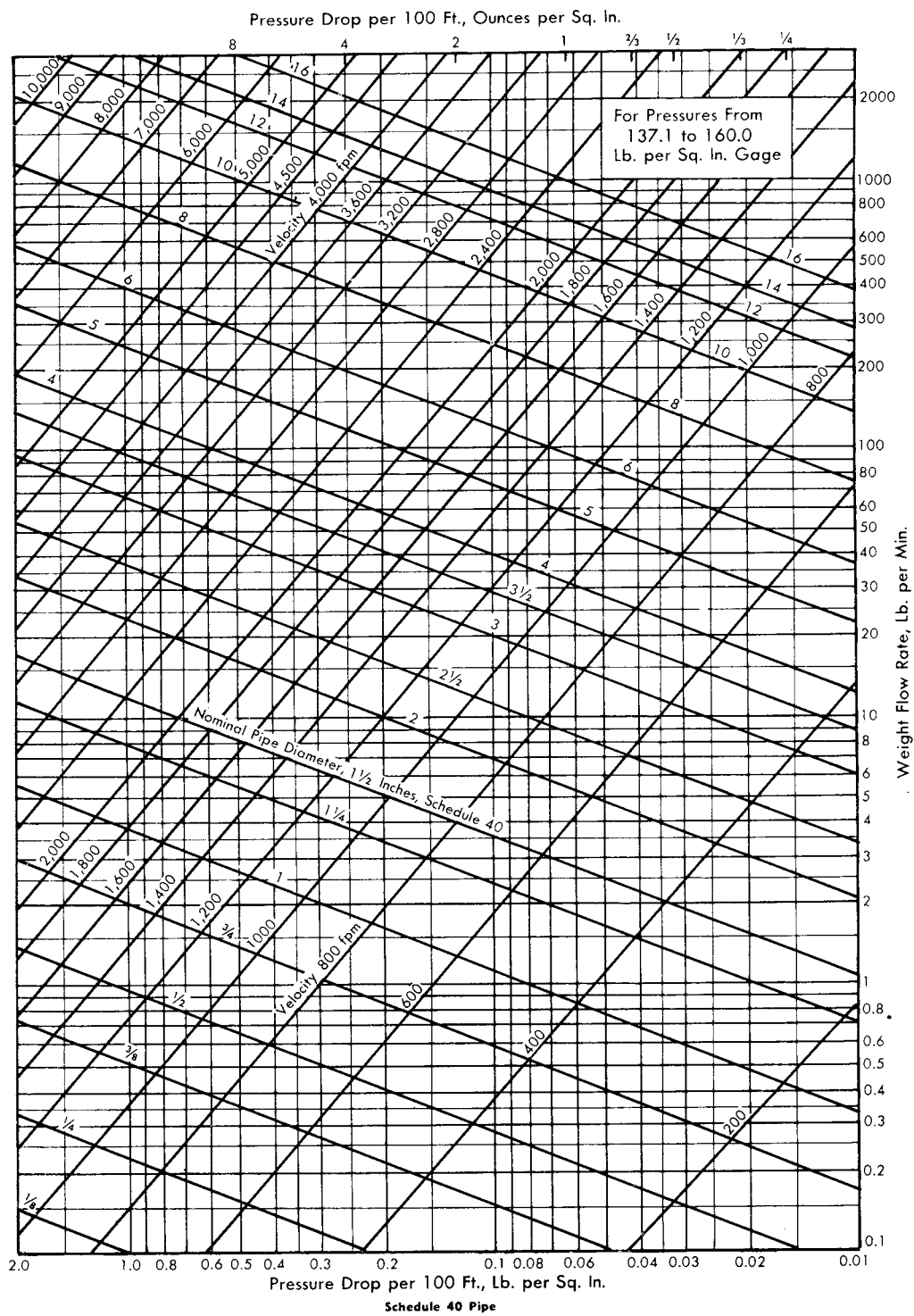
Fig 9-31. For pressure from 137.1 to 160.0 psig
