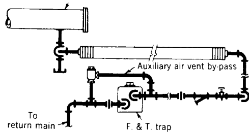
Fig 15-17. Controlled steam header drip
