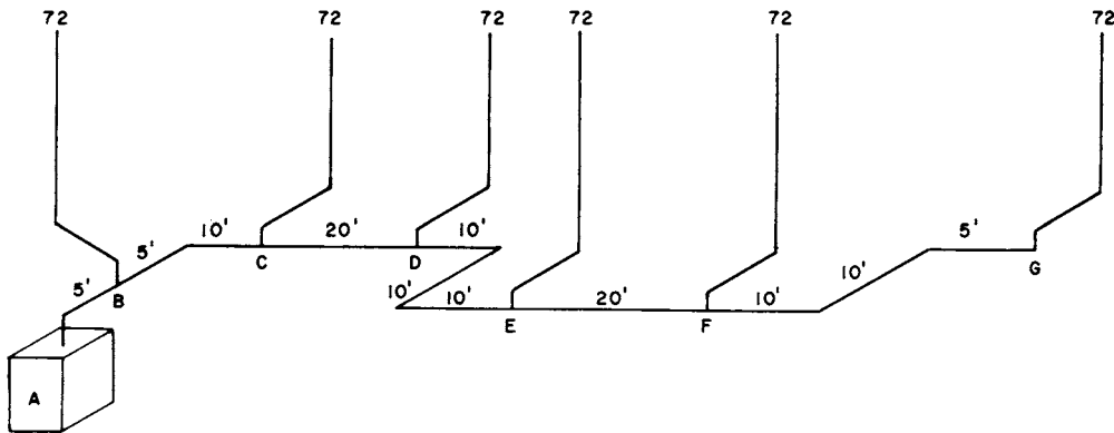
Fig 15-69. Low pressure steam supply main
