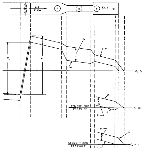
Fig 8-3b. Pressure changes in system
