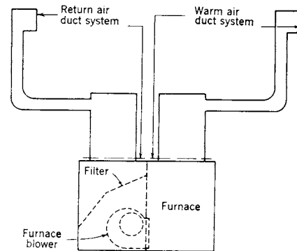
Fig 15-128a. Schematic diagram of a forced air system
