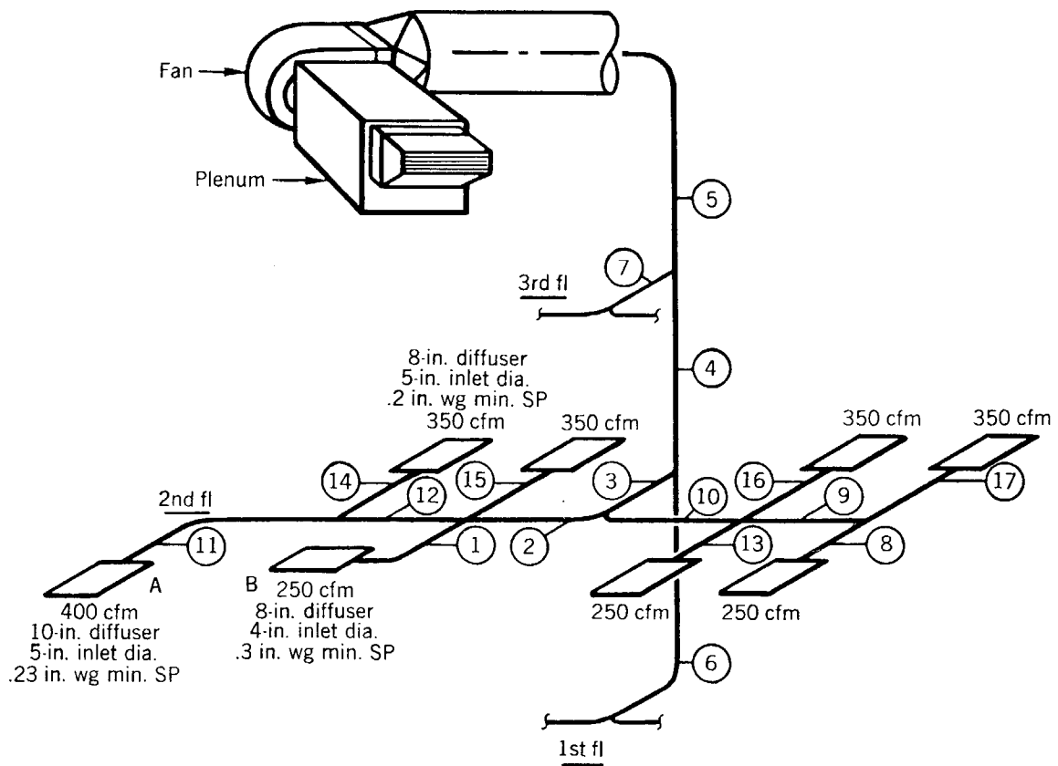
Fig 14-75. Layout and specifications chart for duct system in a 3-story office building
