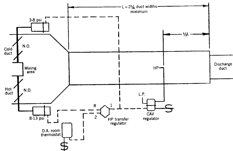
Fig 13-138. Dual duct constant volume mixing box
