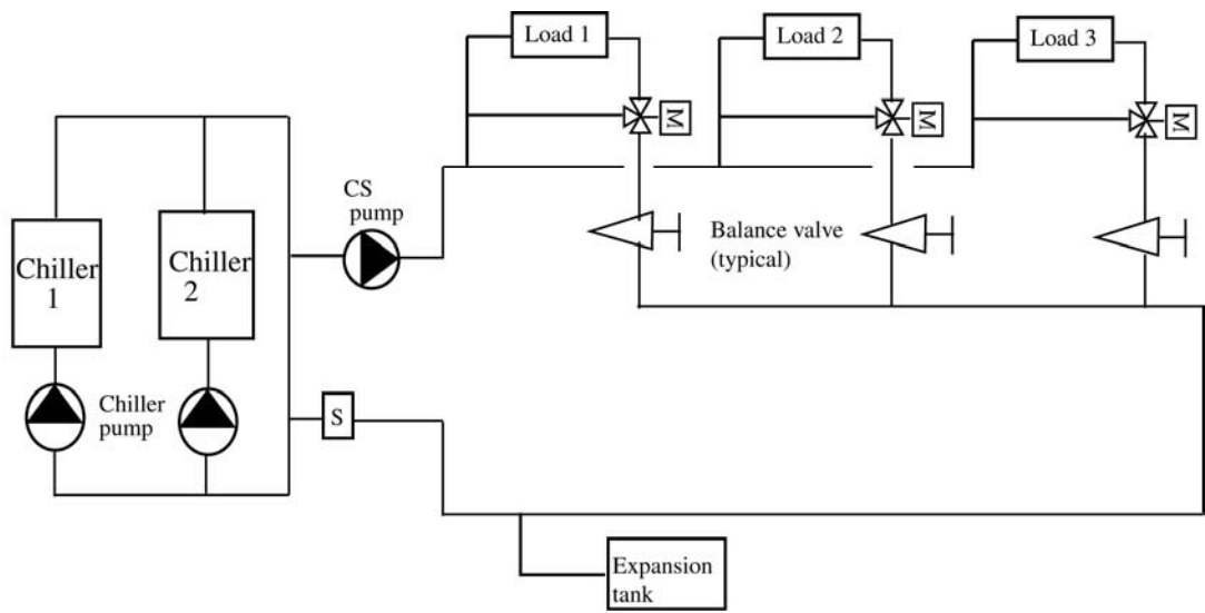
Fig 10-4. Closed chilled water system with constant speed chilled water supply pump and mixing valve
