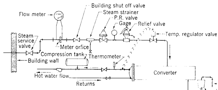
Fig 15-92. Use of district steam as a heat source
