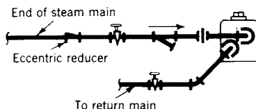
Fig 15-20. End of main drip with minimum elevation between steam main and return main
