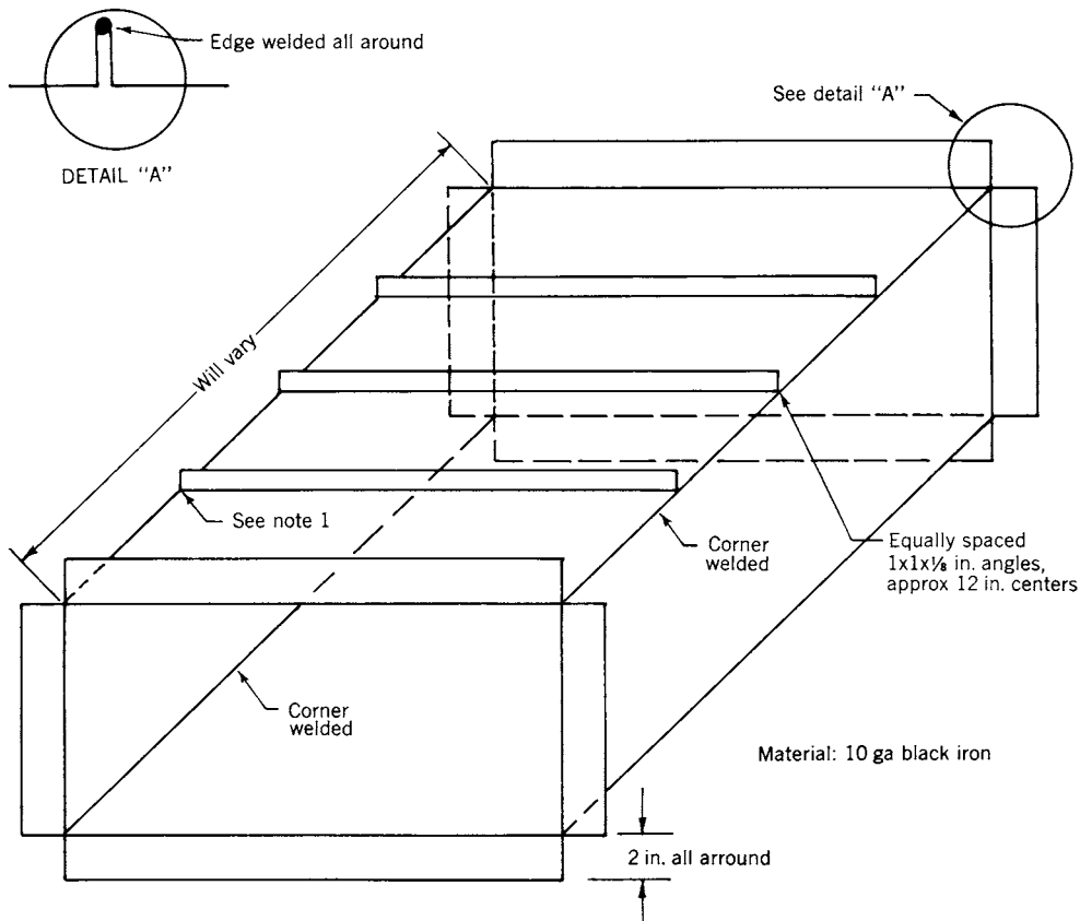
Fig 14-84. Typical rectangular breeching for low pressure
