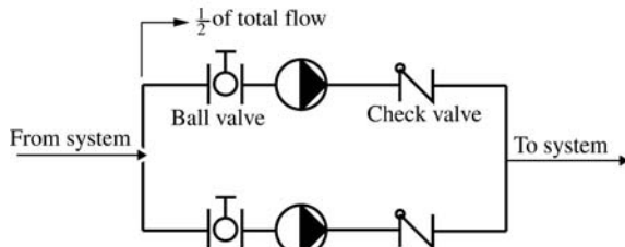
Fig 10-27. Typical installation of two pumps in parallel, with check valve
