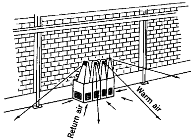
Fig 15-158. Details of gas fired heater installation
