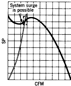
Fig 14-25. System surge
