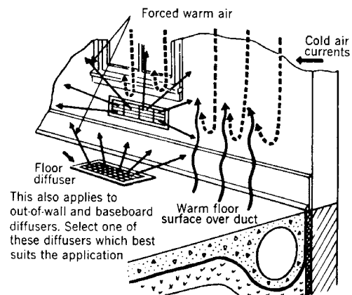
Fig 15-135b. Details of perimeter loop system with floor or baseboard diffuser below window
