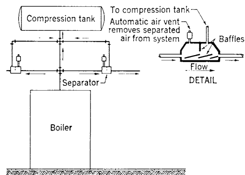
Fig 15-97. Use of air separators for air removal
