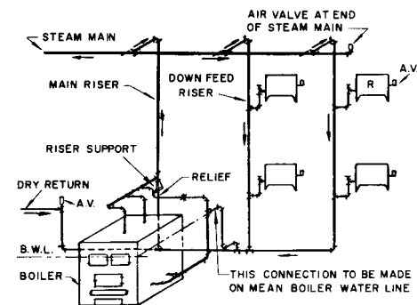
Fig 15-63. One pipe downfeed gravity systems
