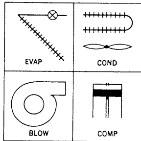
Fig 13-1. Self contained air conditioner
