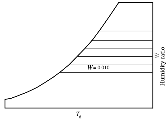
Fig 2-4b. Lines of constant humidity ratio ( W )
