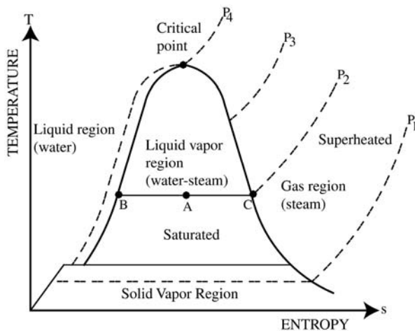
Fig 1-1b. Thermodynamic states of water in T-s coordinates
