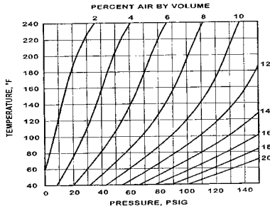
Fig 10-7. Solubility versus temperature and pressure for air/water solution
