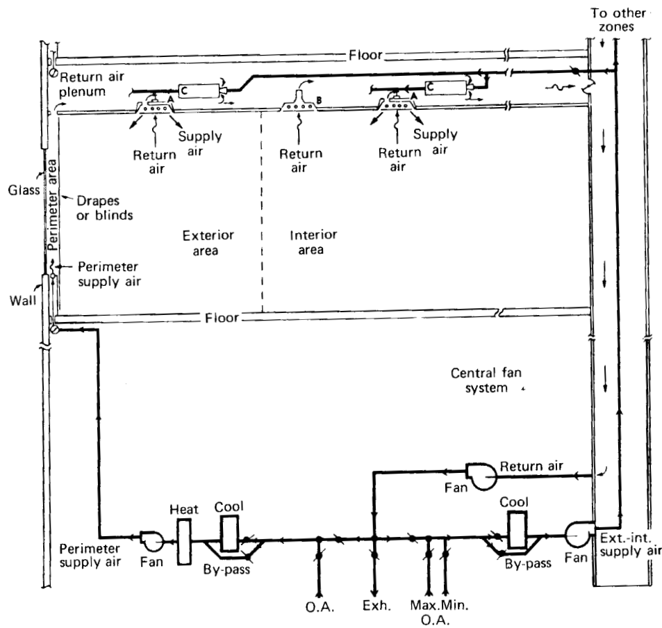
Fig 13-58. Typical air system using induction type mixing units
