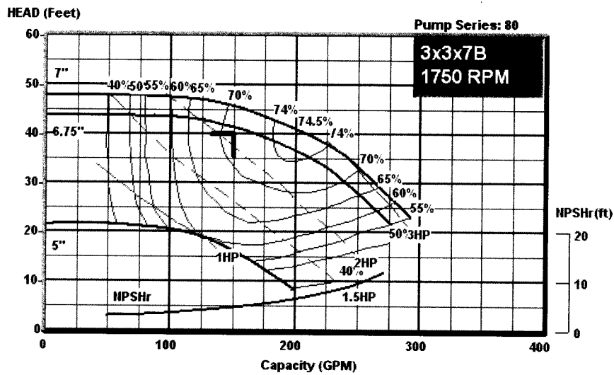
Fig 10-19. Pump curve for Series 80 B&G inline pump
