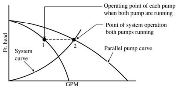
Fig 10-32. System curve plotted over single pump and combined impeller curves
