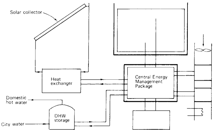
Fig 13-79. Solar heating of domestic hot water
