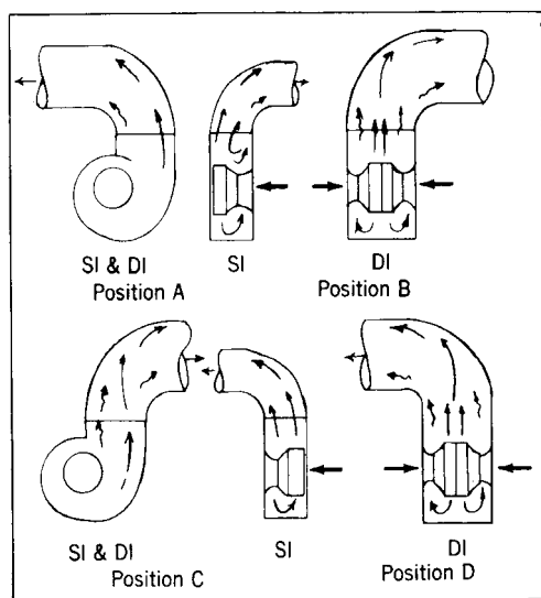
Fig 14-51. Discharge elbow flow patterns
