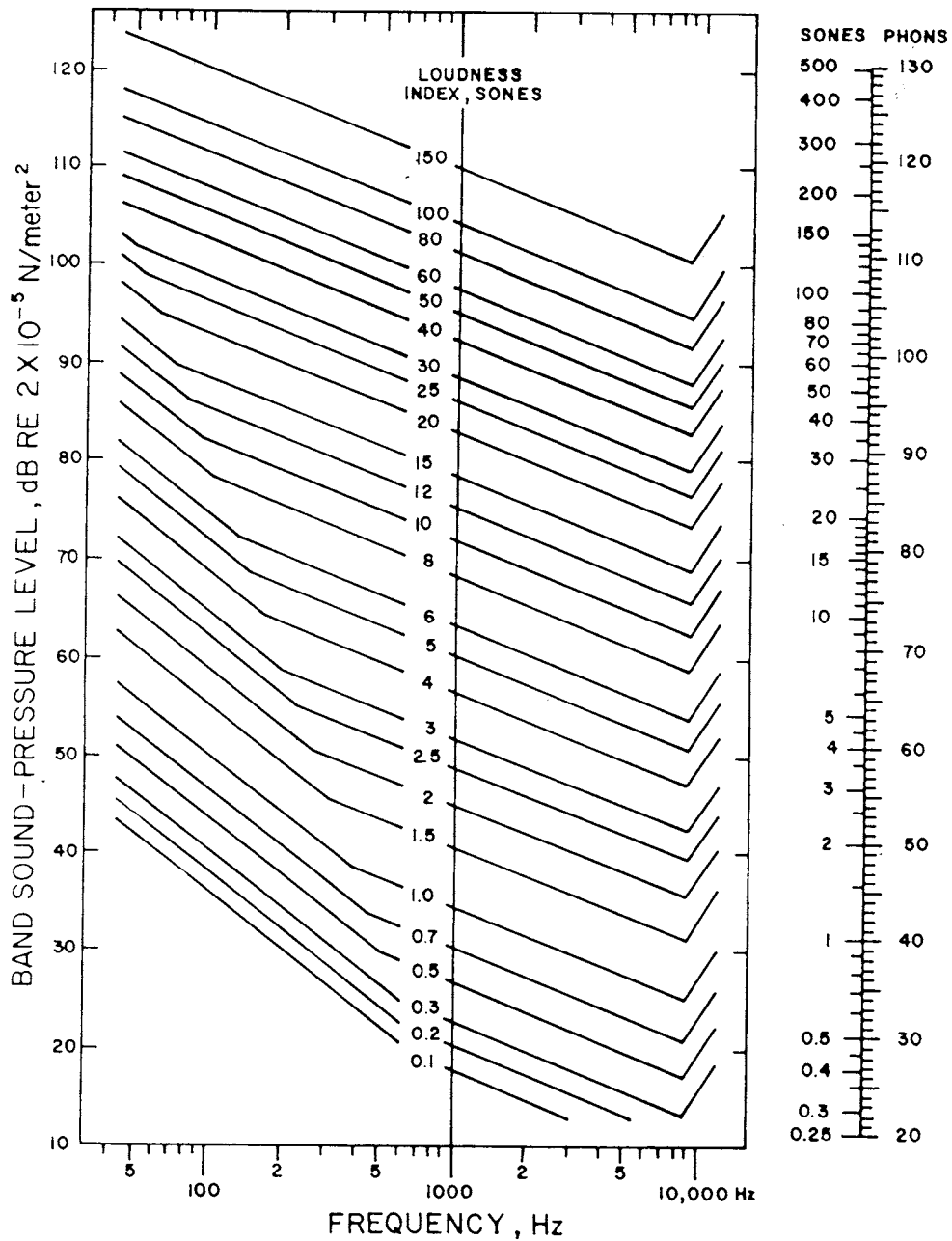
Fig 16-3. Contours of equal loudness index to compare noise source
