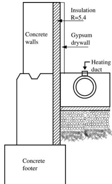
Fig 6-7. Metal stud wall slab on grade foundation insulation
