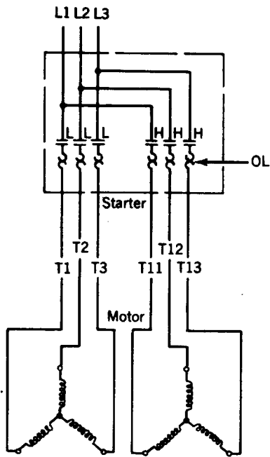
Two speed, two winding (separate winding) constant horsepower, constant torque, or variable torque
