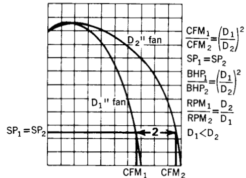
Fig 14-10. Fan law No. 2—change in wheel diameter (constant volume)
