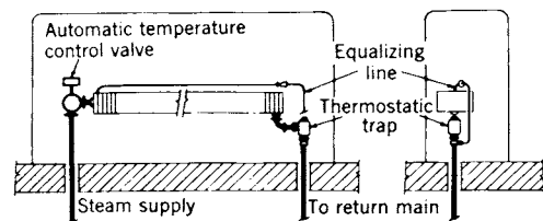
Fig 15-13. Unit ventilator piping details
