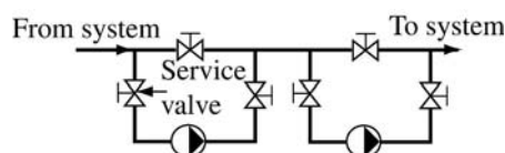
Fig 10-36. Practical series pump installation
