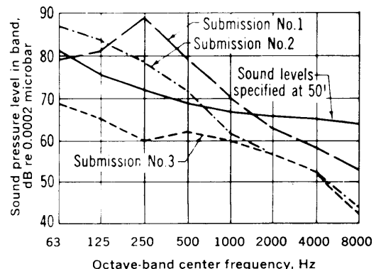
Fig 16-30. Manufacturers cooling tower submissions to meet sound level specifications
