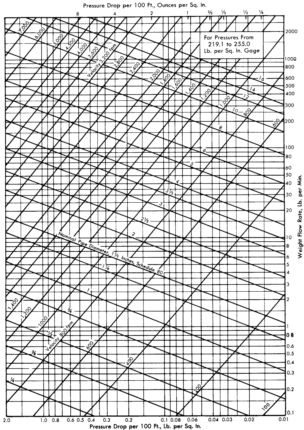
Fig 9-34. For pressure from 219.1 to 255.0 psig
