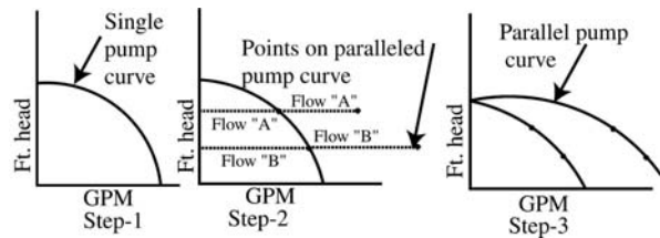
Fig 10-29. Paralleled pump curve construction
