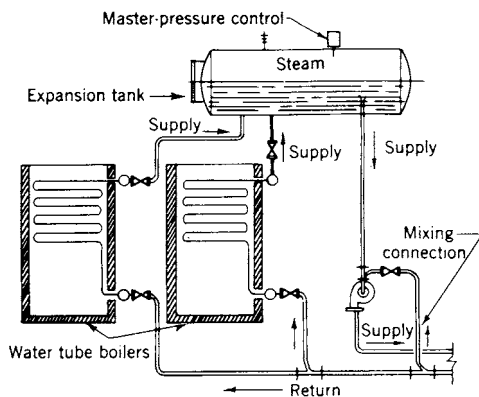
Fig 15-109. HTW system pressurized by steam
