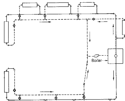
Fig 15-94. Two pipe direct return system
