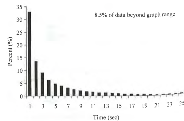
Fig. 8. Distribution of idle periods.
