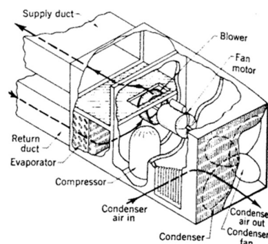
Fig 13-3. Horizontal self contained air conditioned unit
