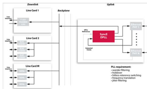
Figure 5. Next-generation digital loop carrier
