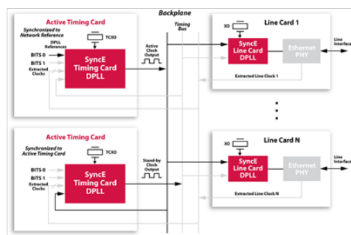
Figure 4: Redundant timing in carrier-grade SyncE
