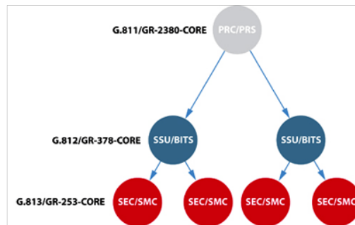
Figure 1: SDH/SONET network synchronization hierarchy
