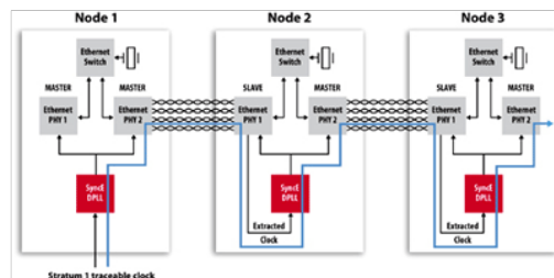
Figure 3: Physical layer timing in synchronized Ethernet
