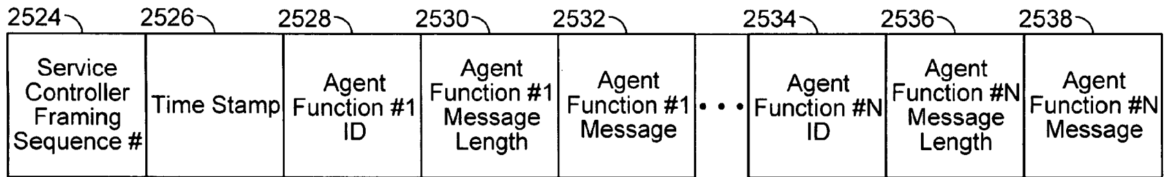
Service Controller Communication Frame
