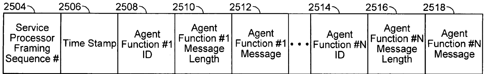
Service Processor Communication Frame
