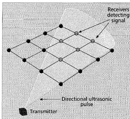
■ Figure 4. Single-transmitter orientation.
