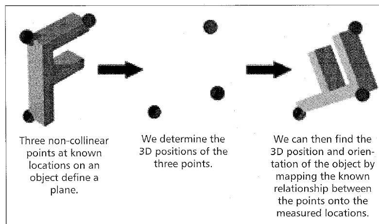
■ Figure 3. Orientation from location information.
