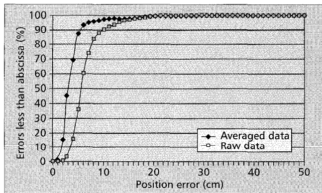
■ Figure 5. Position error cumulative probability distribution for ultrasonic location system.
