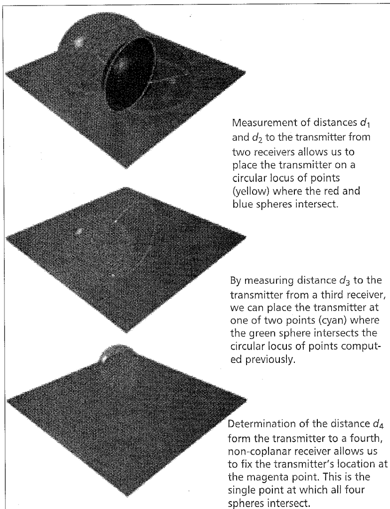
■ Figure 2. Position finding by multilateration.
