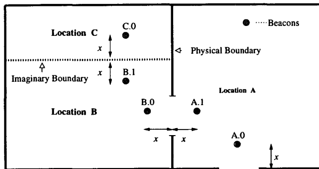
Figure 3: Correct positioning of beacons.
