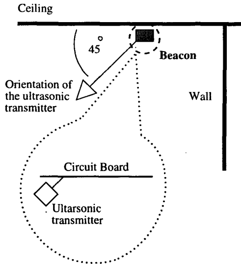
Figure 5: Correct alignment of a Cricket ultrasonic transmitter.
