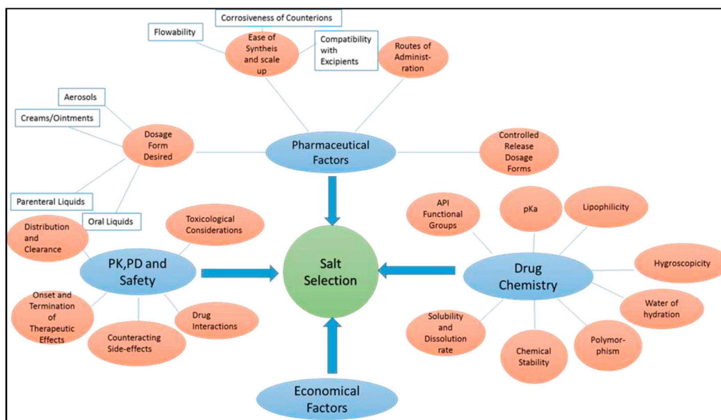
Figure 4. Various factors affecting the salt selection process.
