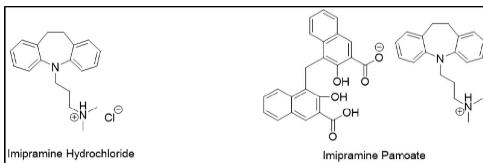
Figure 3. Salts of imipramine.
