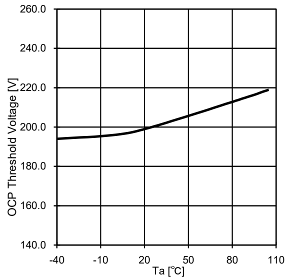
Fig.21 OCP Threshold Voltage-Ta
