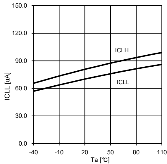
Fig.22 ICLH, ICLL-Ta
