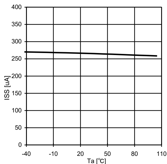
Fig.8 SS Sink Current-Ta ( V_{SS}=1\text{V} , Protection)
