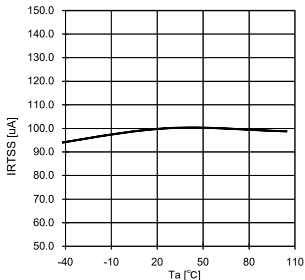
Fig.6 RTSS Pre-charge Current-Ta
