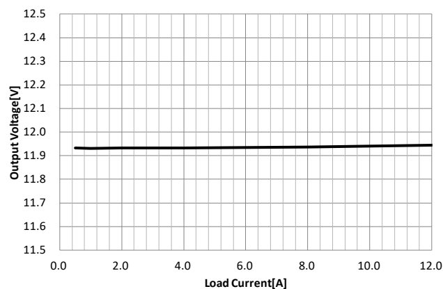
Fig.37 Load Regulation ( V_{CC}=34V )
