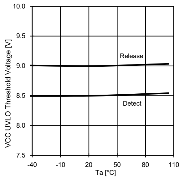
Fig.9 VCC UVLO-Ta
