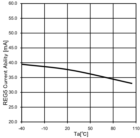
Fig.27 REG5 Current Ability -Ta
