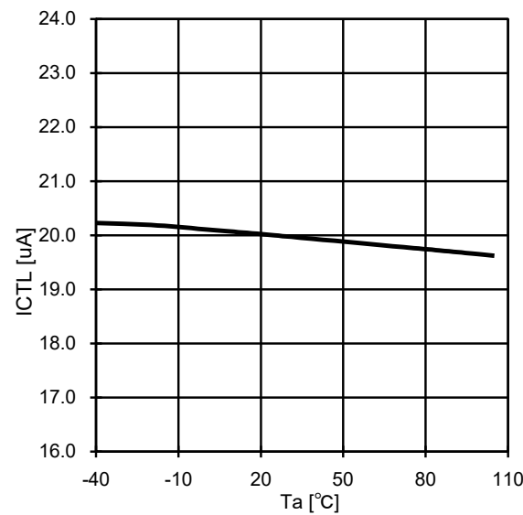
Fig.11 UVLO Hysteresis Current-Ta
