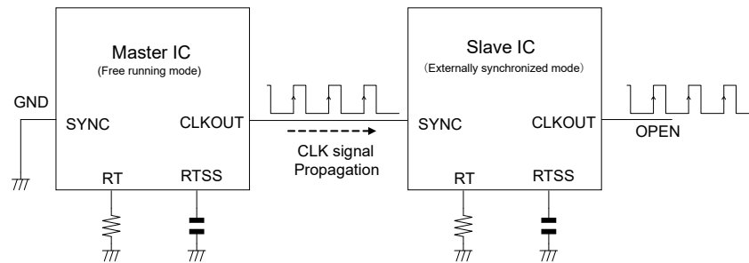
Fig.43 Example of an External Synchronization Circuit
