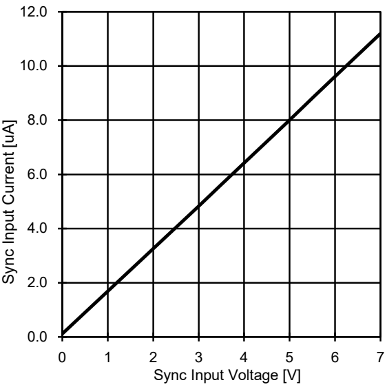
Fig.28 ISYNC-VSYNC
