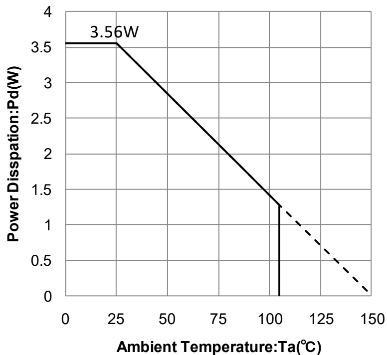
Fig.60 Power Dissipation
