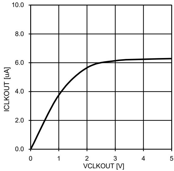
Fig.29 CLKOUT Sink Current - VCLKOUT
