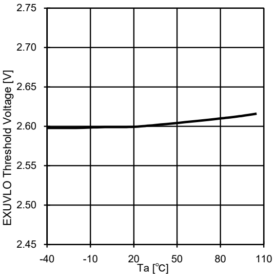
Fig.10 EXUVLO (CTL)-Ta
