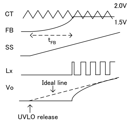
Fig.58 Startup Timing Chart
