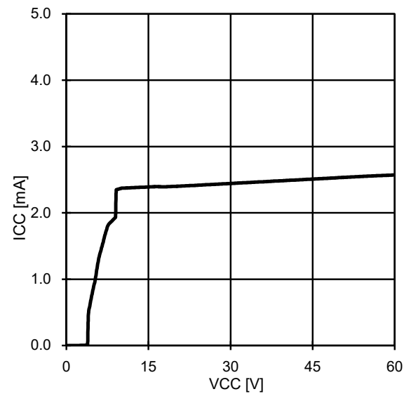
Fig.34 Quiescent Current -VCC
