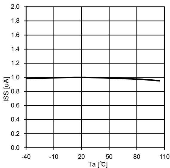
Fig.7 SS Source Current-Ta ( V_{SS}=1\text{V} )
