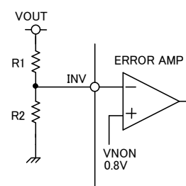
Fig.55 Vout setting
