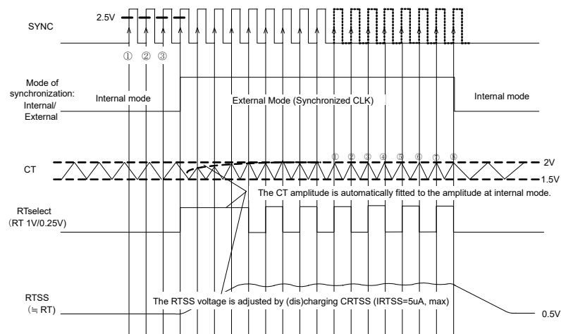
Fig.44 Timing Chart of External Synchronization
