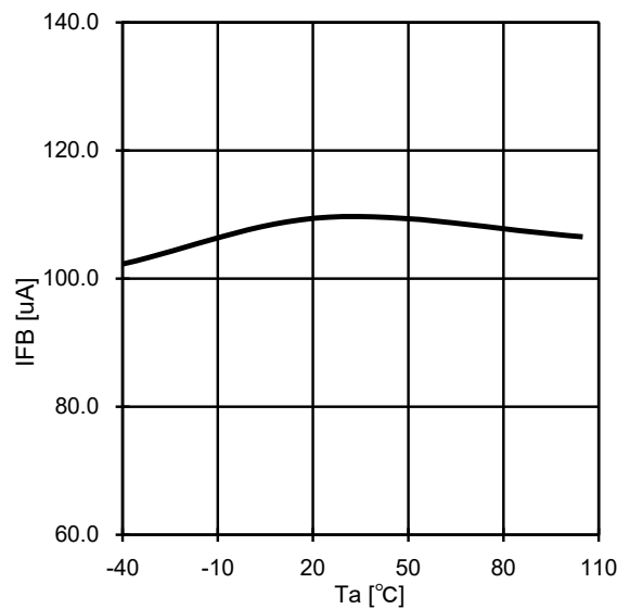
Fig.16 FB Source current-Ta
