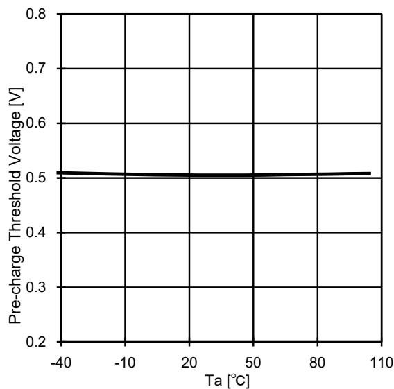
Fig.5 RTSS Pre-charge Threshold-Ta
