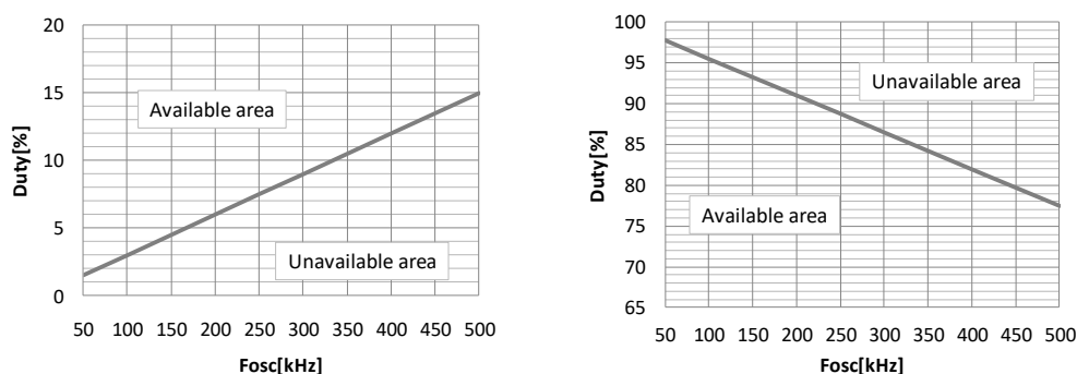
Fig.50 Frequency vs Input-Output Voltage Ratio (Duty)
