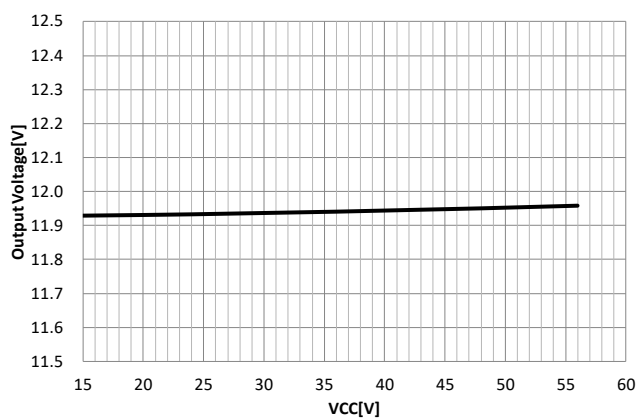
Fig.36 Line Regulation ( I_o=10A )
