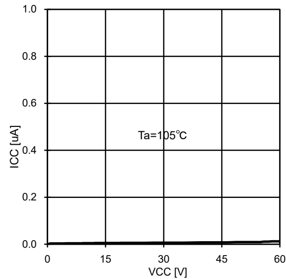
Fig.33 Stand-by Current -VCC
