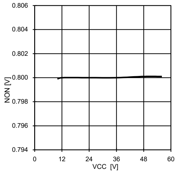
Fig.14 Reference Voltage-VCC
