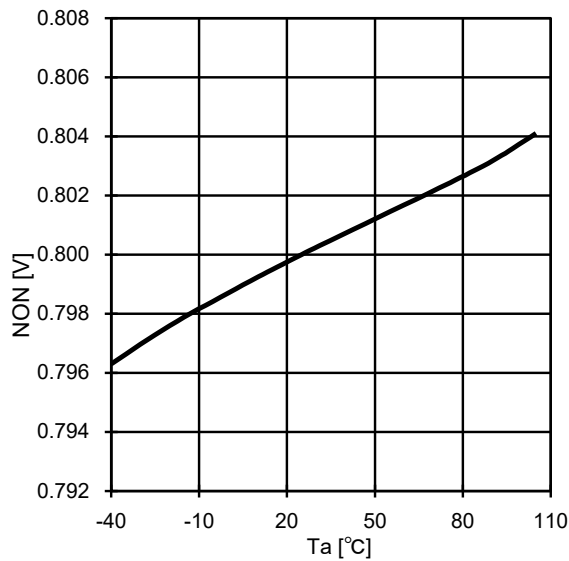
Fig.13 Reference Voltage-Ta
