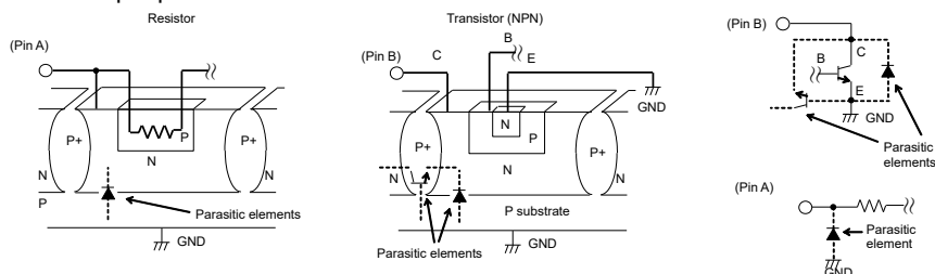
Fig.61 Example of simple structure of Bipolar IC
