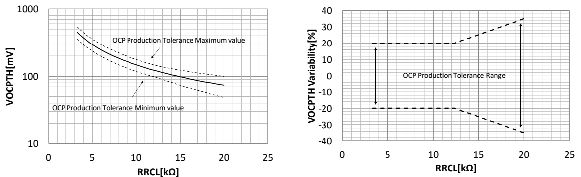
Fig.45 OCP Threshold vs RRCL
