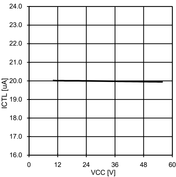
Fig.12 UVLO Hysteresis Current-VCC
