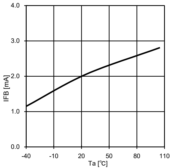
Fig.15 FB Sink current-Ta
