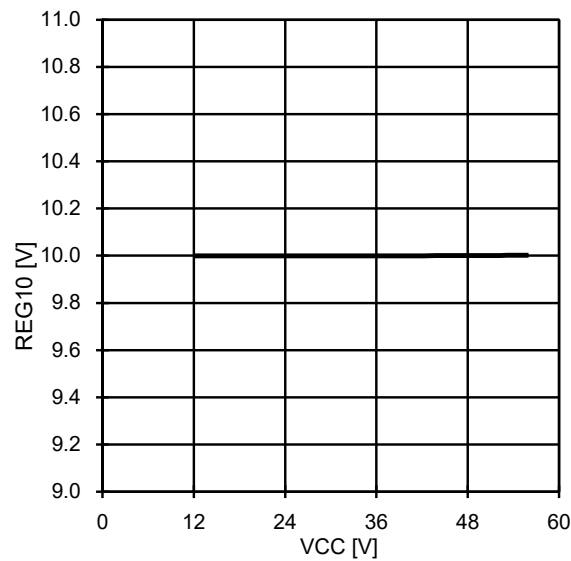
Fig.24 REG10 Line Regulation
