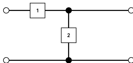
L network
