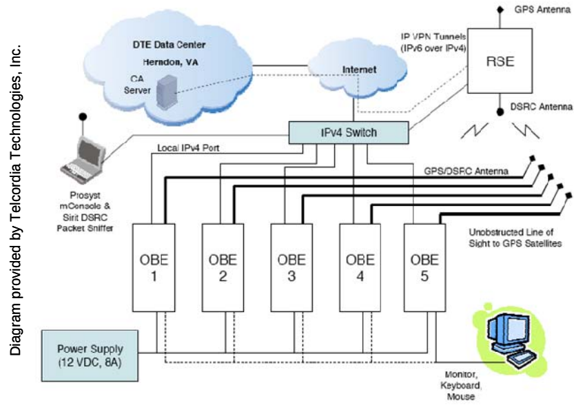
Figure 4-29 Phase 1 Laboratory Security Test Setup
