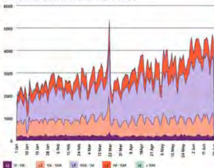
Number of network DDoS attacks (January-June 2024)
