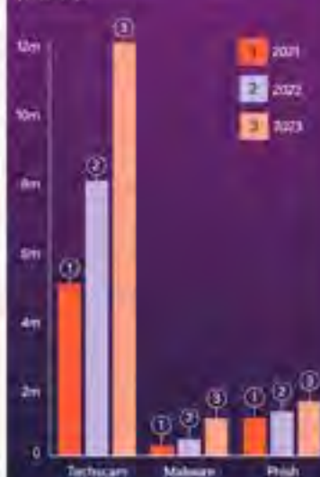
Daily malicious traffic volume (millions)
