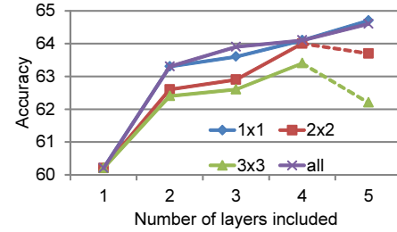
Figure 6. We evaluate spatial pooling strategies to see if retaining spatial information (by pooling over smaller windows) helps multi-scale performance. The answer is essentially ‘no’: global pooling (using a 1 \times 1 window covering the entire layer) does as well as or better than local windows, either of a fixed-size or adaptive-size dynamically selected during the greedy search ( all ). We posit two reasons: (1) finer spatial cues may already be captured by multiscale features extracted from neighboring layers and (2) additional training data might be needed to realize the benefit of local pooling windows since they generate larger descriptors. Dotted line means the layer will not be selected by greedy procedure. For reference, we also experimented with max-pooling strategies, but saw consistently worse results.
