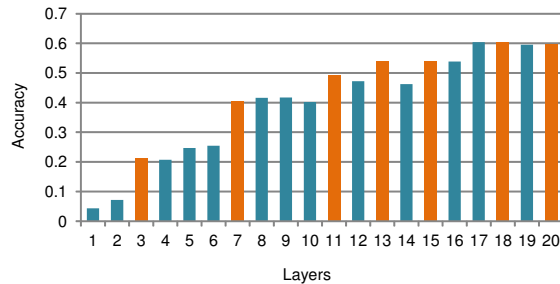
Figure 3. The classification accuracy on MIT67 [26] using activations from each layer. We use an orange color fill representing the output of a ReLU layer, where there are 7 in total for the Caffe model. We tend to see a performance jump at each successive ReLU layer, particularly earlier on in the model.
