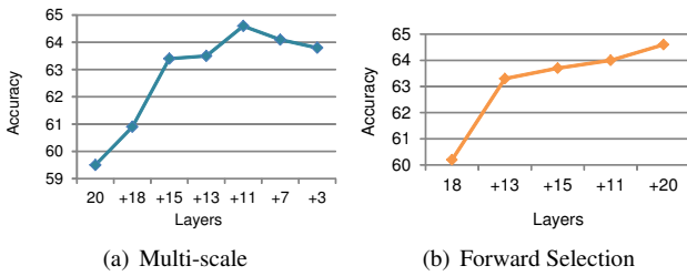
Figure 5. (a) The performance of a multi-scale classifier as we add more layer-specific features. We start with the last ReLU layer, and iteratively add the previous ReLU layer. The “+” sign means the recent-most added layer. Adding additional layers help, but performance saturates and even slightly decreases when adding lower-layer features. This suggests it may be helpful to search for the “optimal” combination of layers. (b) The performance trend when using forward selection to incorporate the ReLU layers. Note that layers are not selected in high-to-low order. Specifically, it begin with the second-to-last ReLU layer, and skip one or more previous layers when adding the next layer. This suggests that layers encode some redundant or correlated information. Overall, we see a significant 6% improvement.
