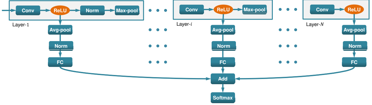
Figure 7. Our multi-scale DAG-CNN architecture is constructed by adding multi-scale output connections to an underlying chain backbone from the original CNN. Specifically, for each scale, we spatially (average) pool activations, normalize them to have unit-norm, compute an inner product with a fully-connected (FC) layer with K outputs, and add the scores across all layers to predictions for K output classes (that are finally soft-maxed together).
