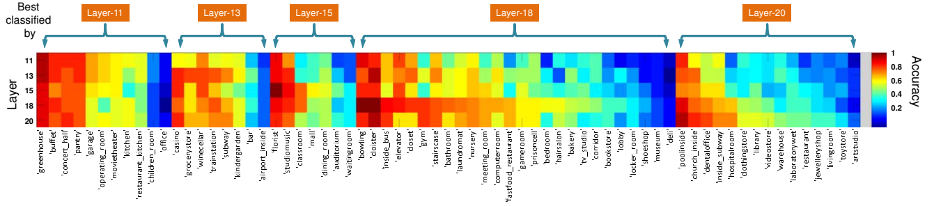
Figure 4. The “per-class” performance using features extracted from particular layers. We group classes with identical best-performing layers. The last layer (20) is optimal for only 15 classes, while the second-to-last layer (18) proves most discriminative for 26 classes. The third-most effective layer (11) captures significantly lower-level level features. These results validate our underlying hypothesis; different classes require different amounts of invariance. This suggests that a feature extractor shared across such classes will be more effective when multi-scale.
