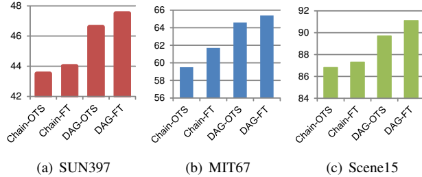
Figure 11. Off-the-shelf vs. Fine-tuning models on both Chain and DAG model for Caffe backbone. Please see the text for a discussion.
