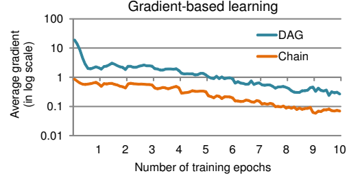
Figure 9. The average gradient from Layer-1 (Conv.) during training, plotted in log-scale. Gradients from the DAG are consistently 10\times larger, implying that they receive a stronger supervised signal from the target label during gradient-based learning.
