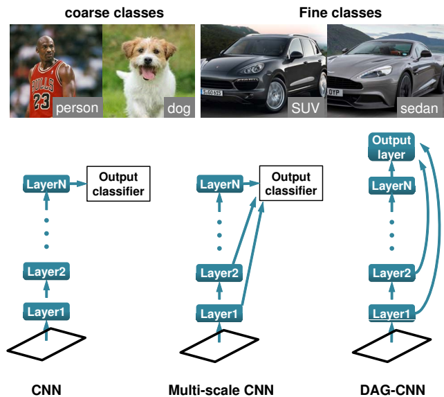
Figure 1. Recognition typically require features at multiple scales. Distinguishing a person versus dog requires highly invariant features robust to the deformation of each category. On the other hand, fine-grained recognition likely requires detailed shape cues to distinguish models of cars ( top ). We use these observations to revisit deep convolutional neural net (CNN) architectures. Typical approaches train a classifier using features from a single output layer ( left ). We extract multi-scale features from multiple layers to simultaneously distinguish coarse and fine classes. Such features come “for free” since they are already computed during the feed-forward pass ( middle ). Interestingly, the entire multi-scale predictor is still a feed-forward architecture that is no longer chain-structured, but a directed-acyclic graph (DAG) ( right ). We show that DAG-CNNs can be discriminatively trained in an end-to-end fashion, yielding state-of-the-art recognition results across various recognition benchmarks.
