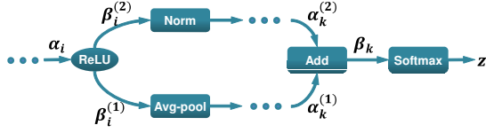
Figure 8. Visualization of the parameter setup at i -th ReLU.
