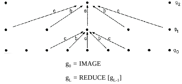
Fig 1. A one-dimensional graphic representation of the process which generates a Gaussian pyramid. Each row of dots represents nodes within a level of the pyramid. The value of each node in the zero level is just the gray level of a corresponding image pixel. The value of each node in a high level is the weighted average of node values in the next lower level. Note that node spacing doubles from level to level, while the same weighting pattern or "generating kernel" is used to generate all levels.
