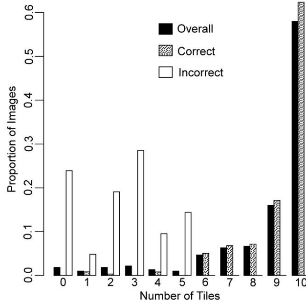
Figure 8: Histogram of the number of tiles correctly classified for the WSI overall, the WSI that were correctly classified, and the WSI that were incorrectly classified. For example, in the data set as a whole, we see that ~58% of the images had all 10 tiles classified correctly, among the WSI that were correctly classified, ~62% had all 10 tiles classified correctly, and
