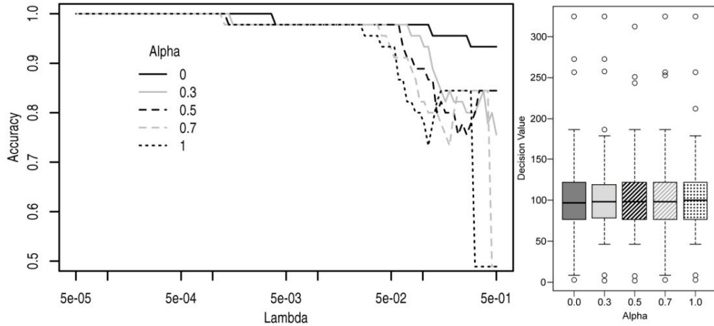
Figure 9: The effect of the Elastic Net model parameters on classification predictions. (a) The impact of lambda and alpha on accuracy over five orders of magnitude for lambda and five different alpha values. (b) Distance distributions of the decision values from the classification threshold for alpha values (0.0, 0.3, 0.5, 0.7, 1.0). Greater values indicate a stronger prediction, positive values indicate an accurate prediction and negative values indicate an inaccurate prediction. There were no inaccurate predictions for any alpha value at lambda min. Accuracy of the model is stable over much of the parameter range, with lower accuracy only occurring where lambda forces few to no features to be included in the model.
