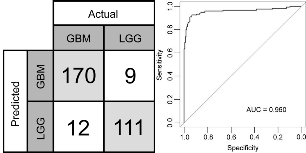
Figure 6: Accuracies LGG/GBM classification in a larger dataset. (a) A confusion matrix summarizing the dataset classification results. (b) ROC curve demonstrating that the values generated by the model match the predicted classes.
