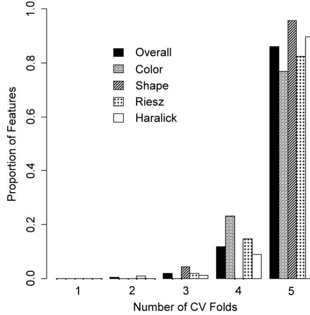
Figure 7: Histogram distribution of features used in Elastic Net models, showing the number of models in which features of a given class appear. The number of features is normalized based on the total number of features represented for each class. Bar patterns represent the feature class. Most features for each class appears in all, or nearly all models, as would be expected if they have diagnostic value.
