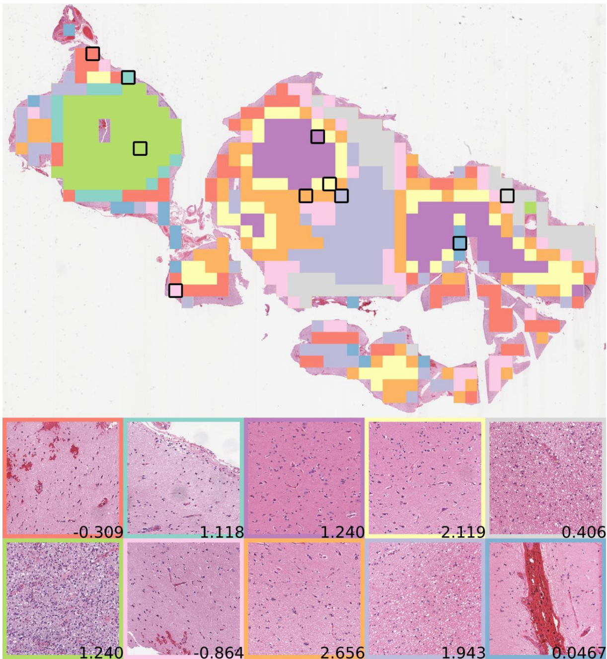
Figure 4: Sample image showing the results of the image processing pipeline. Unique colors represent clusters. Black boxes represent tiles chosen for “fine” profiling. Images at the bottom show the tiles selected from each cluster, with the color on the border of the tiles indicating the cluster from the image. Numbers at the bottom are the decision values the tiles received after machine learning analysis with positive values indicating a correct decision and negative values indicating an incorrect one. The strong positive values from some tiles (e.g., 2.656 in the orange tile) are able to overcome weak incorrect decisions from others (e.g., -0.309 in the red tile). Additionally, the small decision value for the bleeding artifact in the blue tile in the bottom left, demonstrates the pipeline's ability to minimize the impact of artifacts on the final decision.
