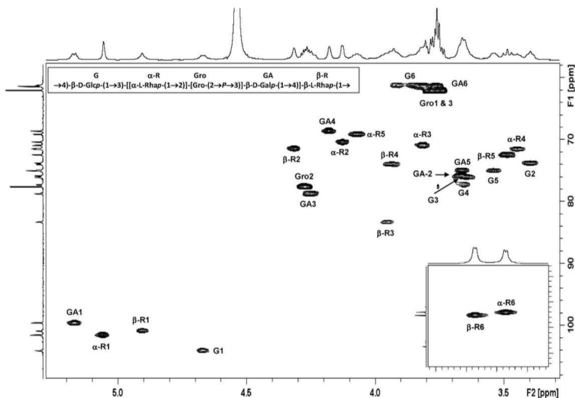
Fig. 5. Expansion of the HSQC spectrum of polysaccharide 23A recorded at 600 MHz, the crosspeaks from the methyl region of the spectrum are shown in the insert. Key tetrasaccharide repeating unit proton/carbon crosspeaks have been labeled according to the carbon atom of the corresponding residue ( \alpha - and \beta -R = \alpha - and \beta -Rha, G = Glc, GA = Gal and Gro = glycerol).
