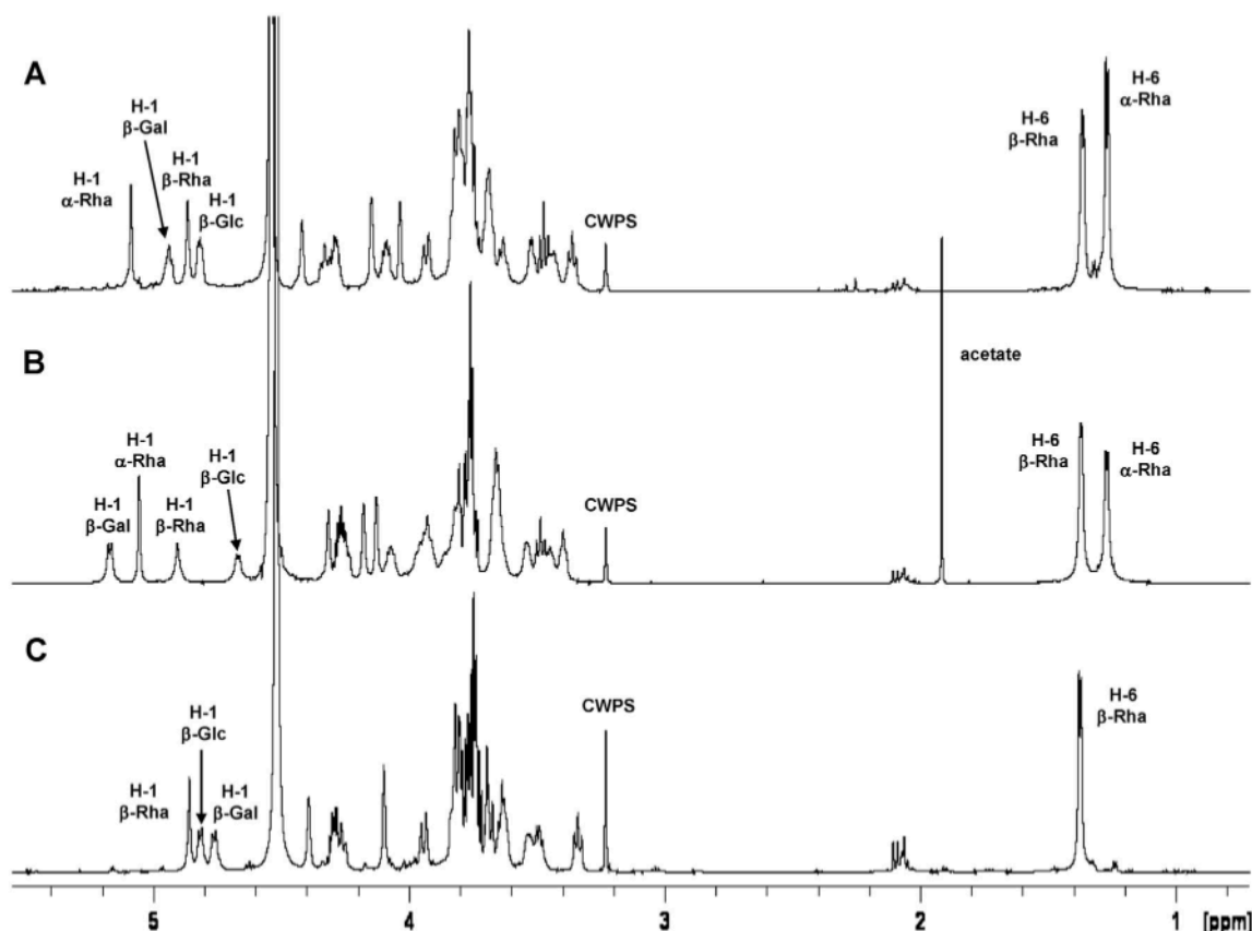
Fig. 2. 1D ^1\text{H} NMR spectra of pneumococcal serotype (A) 23F, (B) 23A and (C) 23B capsular polysaccharides. Some signals including the diagnostic anomeric and methyl protons are labeled.
