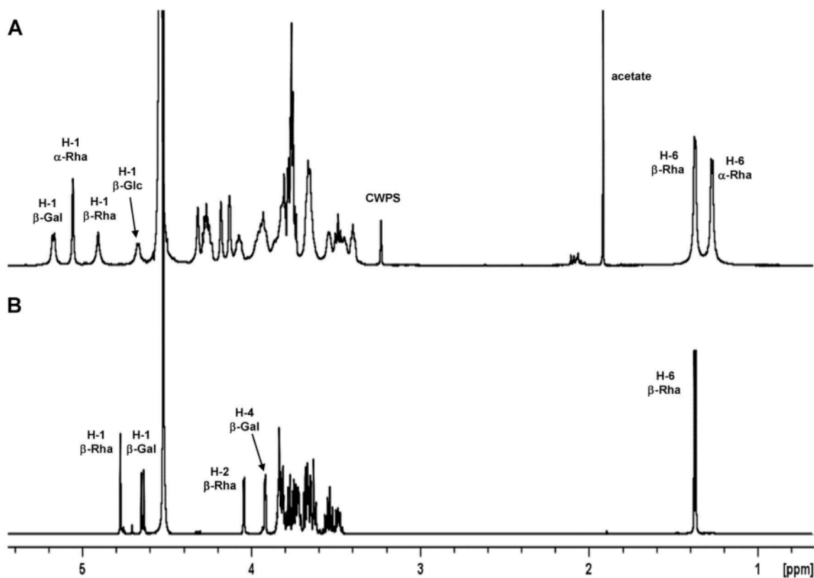
Fig. 6. 1D 1 H NMR spectra of pneumococcal serotype (A) 23A polysaccharide and (B) 23ASD, the oligosaccharide obtained after Smith degradation. Some signals including the diagnostic anomeric and methyl protons are labeled.
