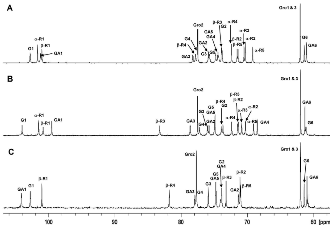
Fig. 4. Expansion of the 1D ^{13}\text{C} NMR spectra of pneumococcal serotype (A) 23F, (B) 23A and (C) 23B capsular polysaccharides showing the anomeric and ring regions. Carbon peaks have been labeled according to the corresponding residue ( \alpha - and \beta -R = \alpha - and \beta -Rha, G = Glc, GA = Gal and Gro = glycerol).
