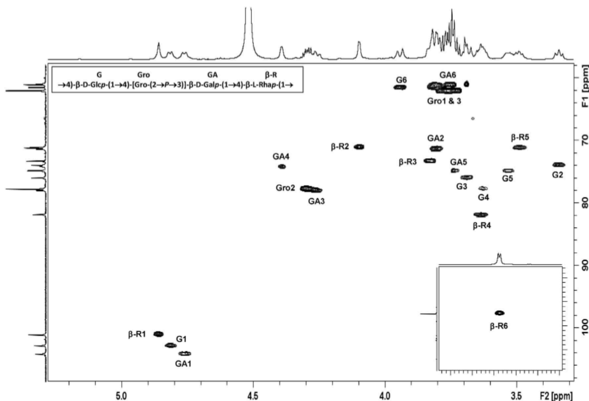
Fig. 7. Expansion of the HSQC spectrum of polysaccharide 23B recorded at 600 MHz, the crosspeaks from the methyl region of the spectrum are shown in the insert. Key trisaccharide repeating unit proton/carbon crosspeaks have been labeled according to the carbon atom of the corresponding residue (β-R = β-Rha, G = Glc, GA = Gal and Gro = glycerol).
