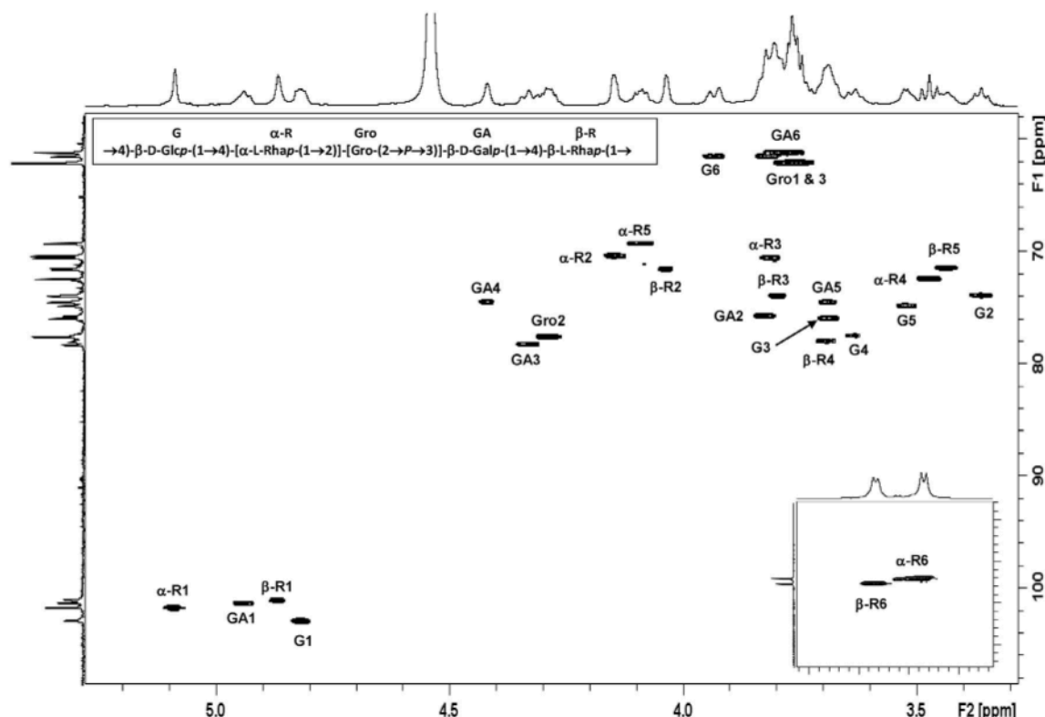
Fig. 3. Expansion of the HSQC spectrum of polysaccharide 23F recorded at 600 MHz, the crosspeaks from the methyl region of the spectrum are shown in the insert. Key tetrasaccharide repeating unit proton/carbon crosspeaks have been labeled according to the carbon atom of the corresponding residue ( \alpha - and \beta -R = \alpha - and \beta -Rha, G = Glc, GA = Gal and Gro = glycerol).
