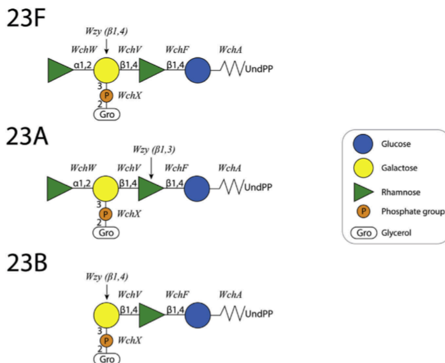
Fig. 9. Proposed glycosyltransferase and polymerase activity in serogroup 23 polysaccharides. Glycosyltransferases responsible for each elongation step are listed above the respective glycosidic linkage in italics. The polymerization site is marked by an arrow.
