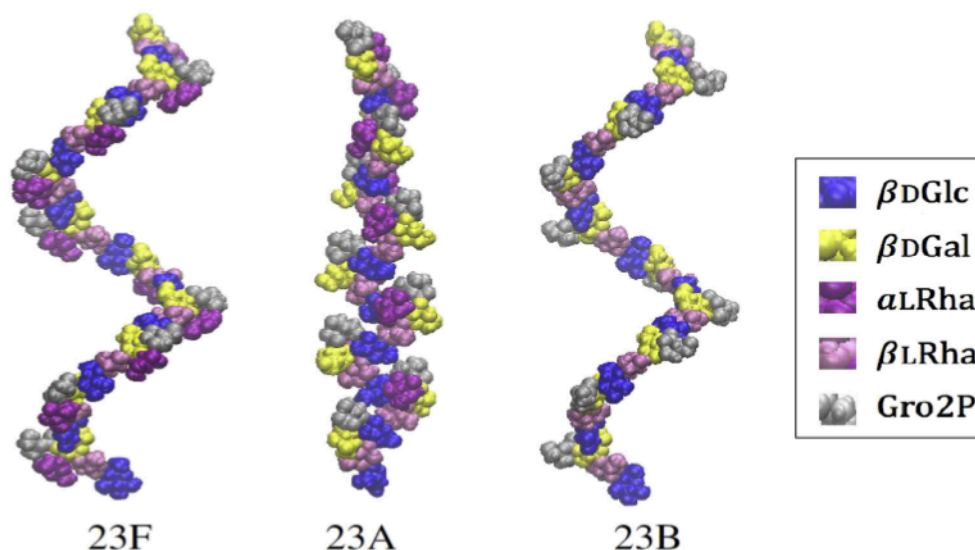
Fig. 8. Minimized molecular models for 10RU of 23F (left) 23A (middle) and 23B (right), shown in space-filling representation and colored according to residue type. The models for 23F and 23B show a similar loose helical conformation, the model for 23A is a slightly twisted flat ribbon, with clear steric crowding at the β-L-Rha branch point. (For interpretation of the references to colour in this figure legend, the reader is referred to the web version of this article.)
