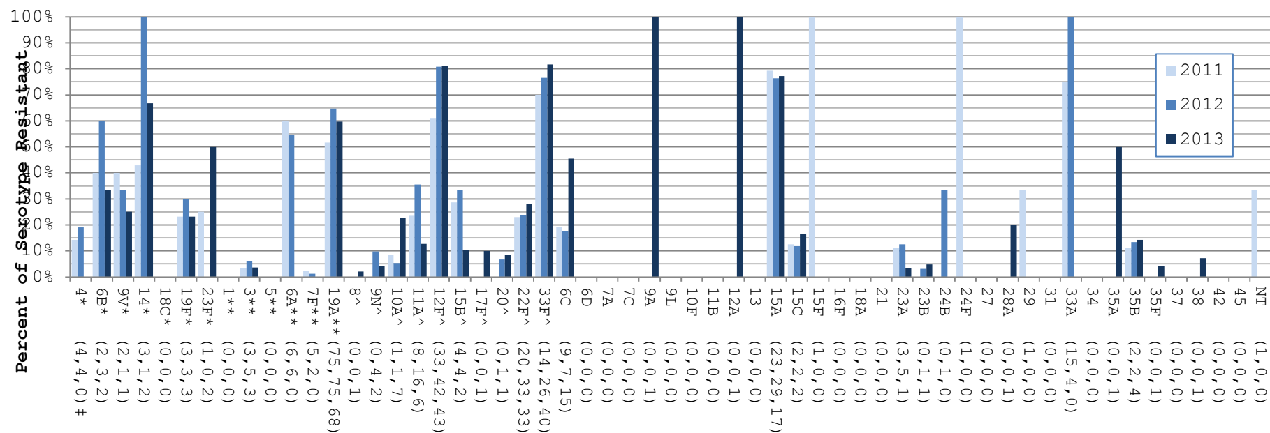
Figure 41. Cefuroxime (parenteral) resistance of S. pneumoniae serotypes collected 2011 - 2013
