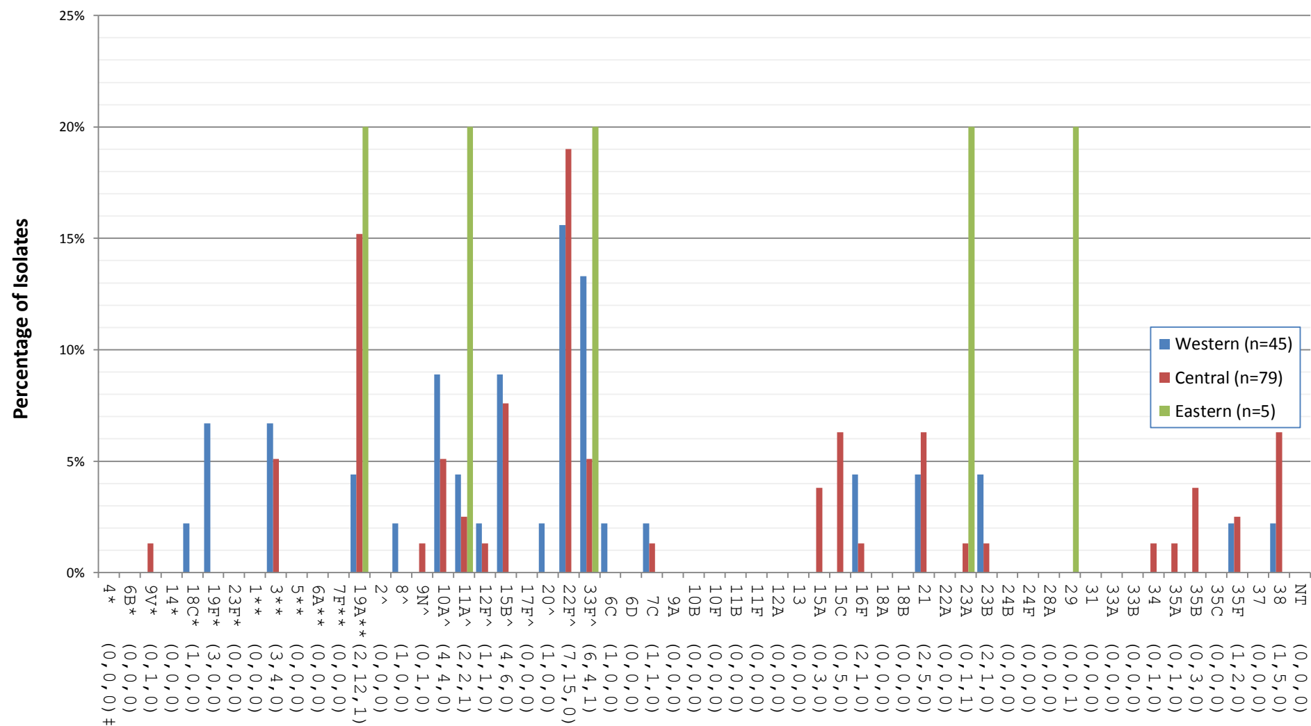
Figure 20. Regional distribution of invasive S. pneumoniae serotypes in <2 year olds, 2013
