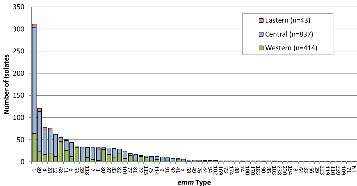
Figure 52. Regional distribution of S. pyogenes emm types
