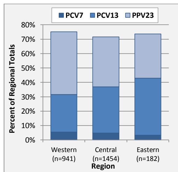
Figure 30. Vaccine serotypes by region, 2013
