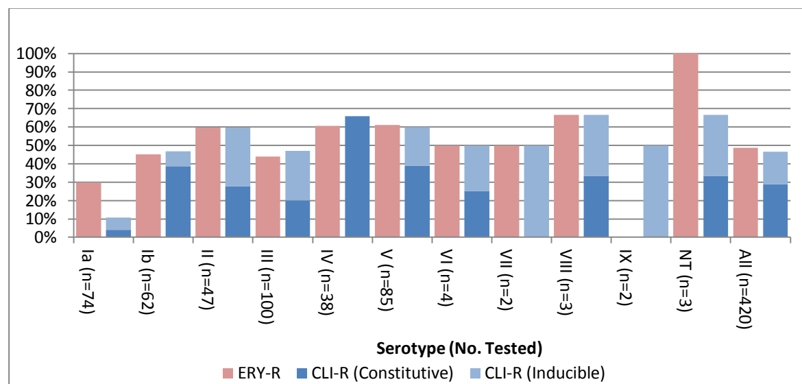
Figure 60. Macrolide resistance of S. agalactiae serotypes, 2013
