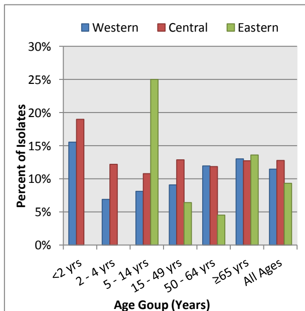
Figure 29. Serotype 22F by region
