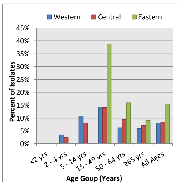
Figure 27. Serotype 7F by region
