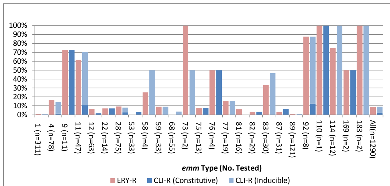
Figure 55. Macrolide resistance of S. pyogenes emm types, 2013
