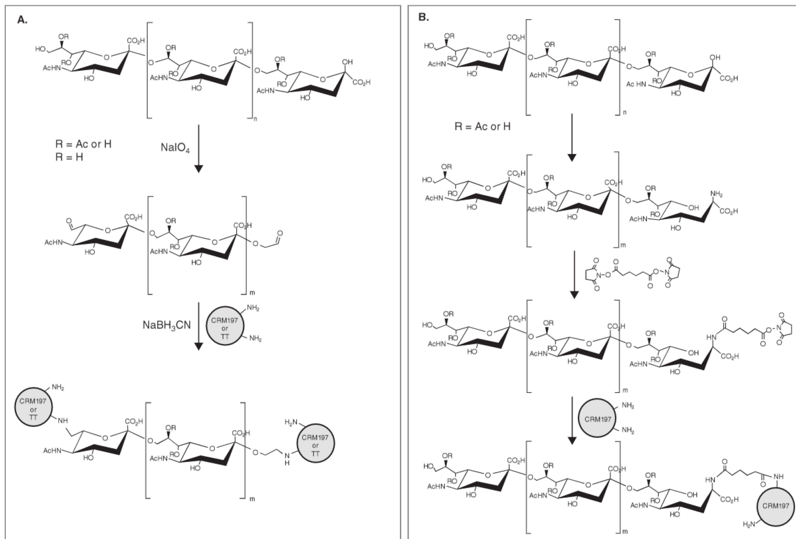
Figure 4. Preparation approaches for licensed meningococcal group C conjugate vaccines of: A) Pfizer (R: Ac or H) and Baxter (R: H) and B) Novartis Vaccines.
