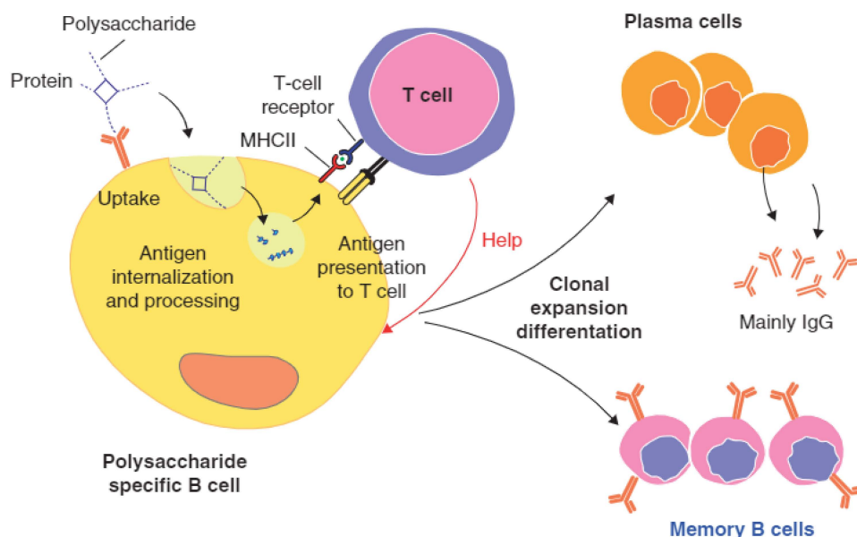
Figure 2. Schematic diagram of mechanism of action for conjugate vaccines.
