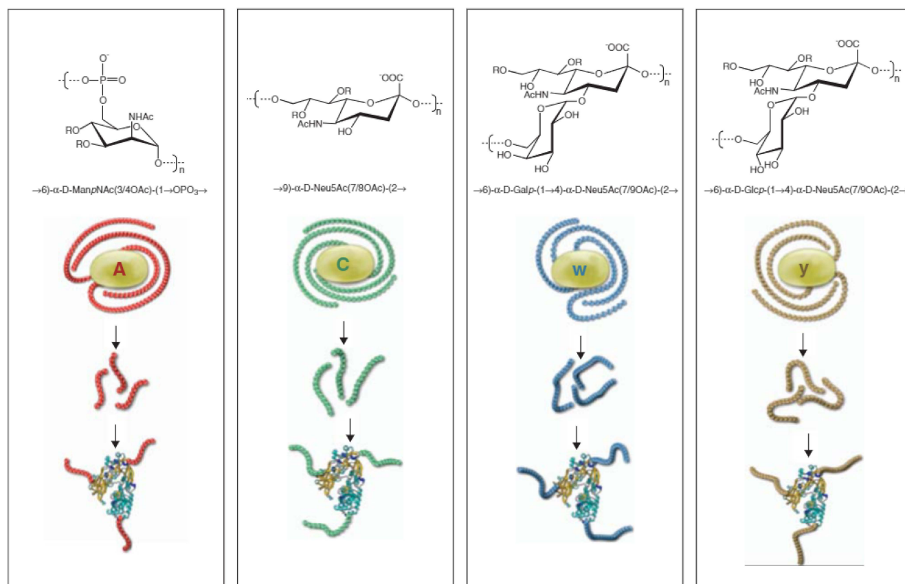
Figure 5. Polysaccharide molecular structures and conjugation technology of licensed meningococcal group A, C, W135, and Y conjugate vaccine produced by Novartis Vaccines.
