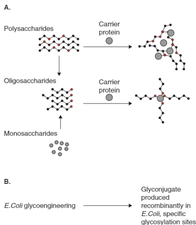
Figure 1. Schematic representation of A) different poly-/oligosaccharide-protein chemical couplings and B) Different way to make glycoconjugate vaccines.
