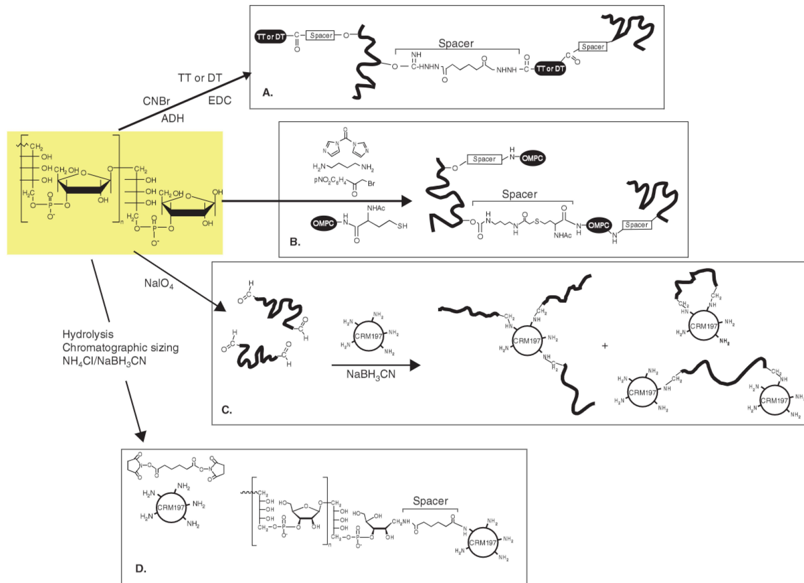
Figure 3. Preparation processes of licensed Hib conjugate vaccines.
