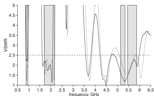
Fig. 2 Measured and simulated VSWR of multiband antenna
