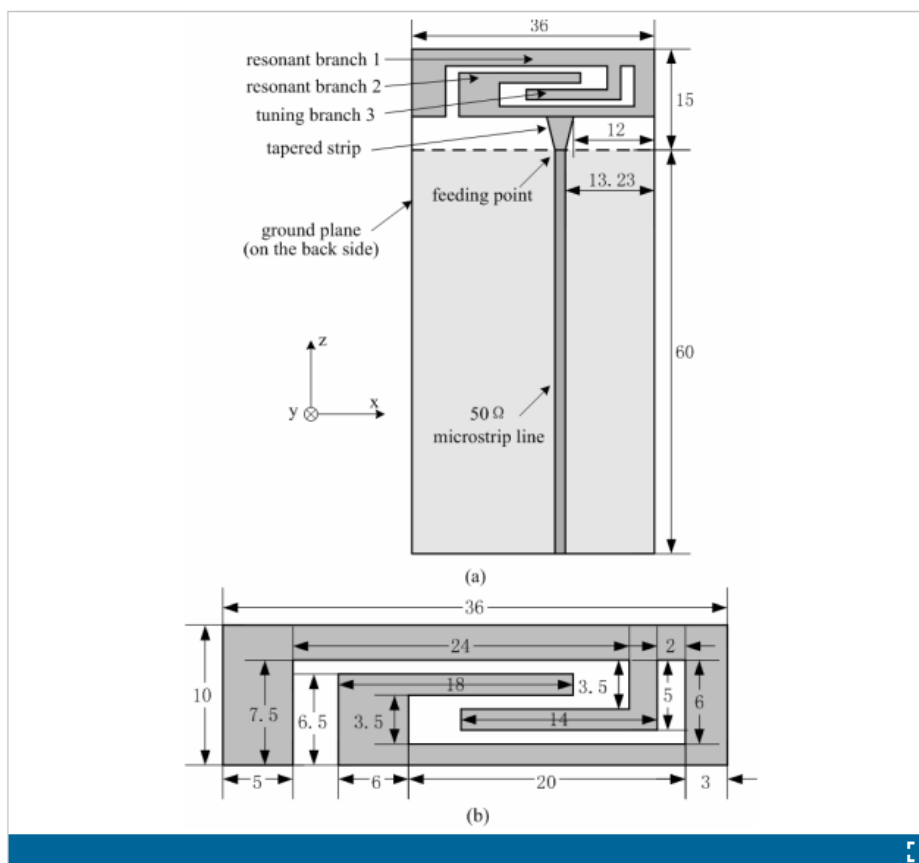
Fig. 1. Configuration of the proposed planar monopole antenna. (a) General view of the antenna. (b) Detailed dimensions of the main radiating element. All dimensions are in millimeter.
