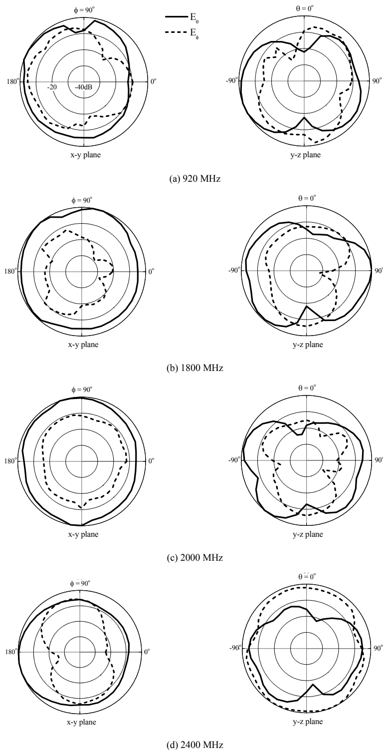
Fig. 4. Measured radiation patterns of the proposed antenna at (a) 920 MHz, (b) 1800 MHz, (c) 2000 MHz and (d) 2400 MHz.
