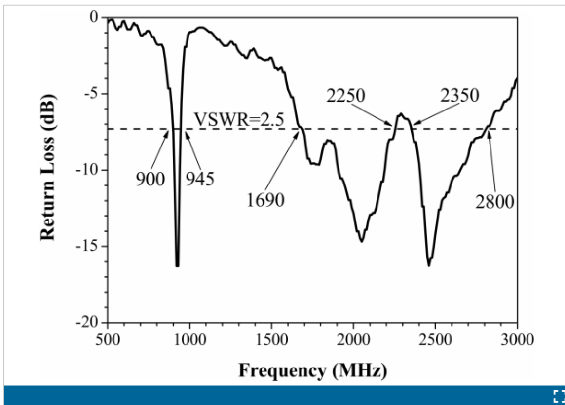
Fig. 3. Measured return loss of the proposed antenna.
