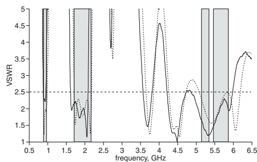
Fig. 2 Measured and simulated VSWR of multiband antenna Standards bandwidth requirement in grey — measurement ——— simulation
