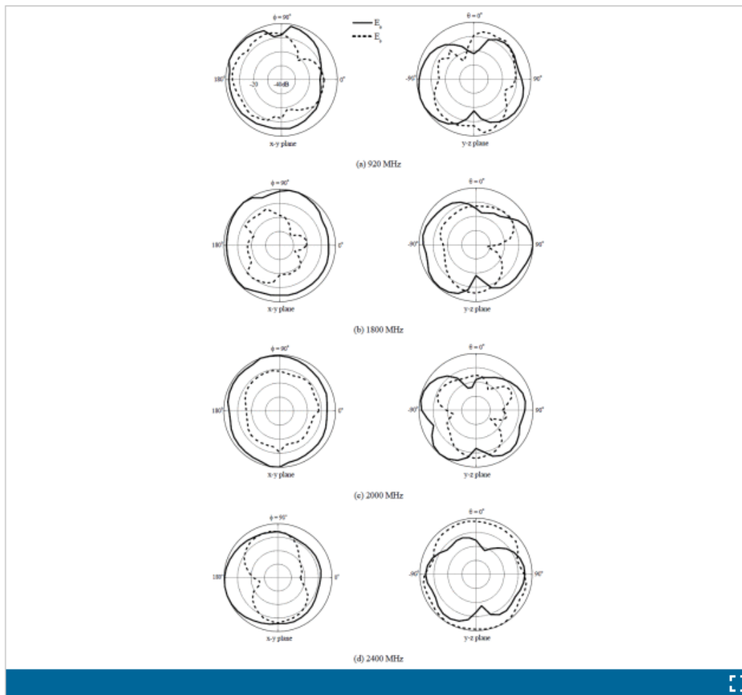
Fig. 4. Measured radiation patterns of the proposed antenna at (a) 920 MHz, (b) 1800 MHz, (c) 2000 MHz and (d) 2400 MHz.
