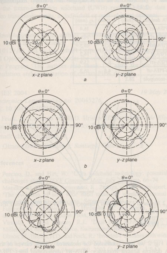
Fig. 3 Measured and simulated radiation gain patterns of multiband antenna
