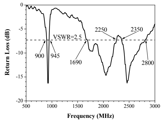
Fig. 3. Measured return loss of the proposed antenna.
