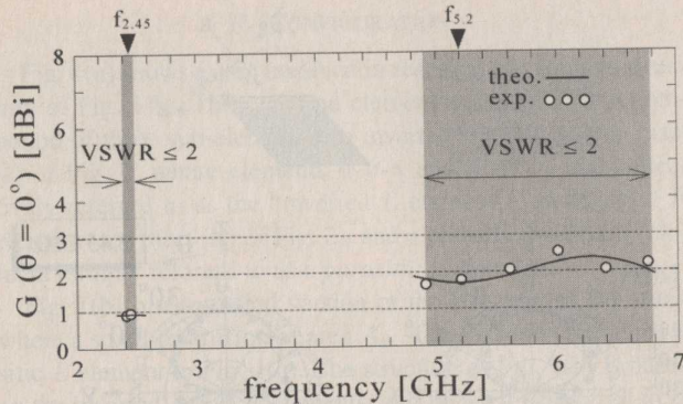
Fig. 6. Gain in the z -direction of an inverted FL antenna. The structural parameters are (H_L, L_L) = (4.5 \text{ mm}, 24.5 \text{ mm}) , (H_F, L_F) = (2.5 \text{ mm}, 10.5 \text{ mm}) , L_{FD} = 7.5 \text{ mm} , (H_P, L_P) = (2.5 \text{ mm}, 9.0 \text{ mm}) , (A_x, A_y) = (4.0 \text{ mm}, 3.0 \text{ mm}) , and (L_x \times L_y) = (30 \text{ mm} \times 25.5 \text{ mm}) .
