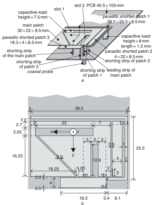
Fig. 1 3D view of multiband antenna
