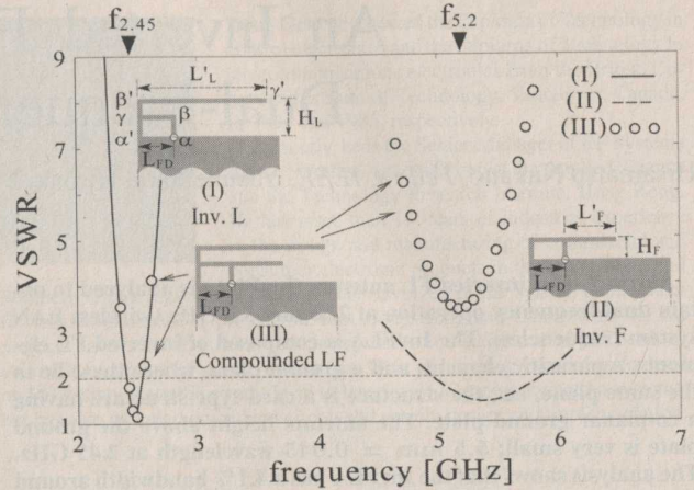
Fig. 2. VSWRs of three structures. The structural parameters for an inverted L element (I) are ( H_L , L'_L ) = (4.5 mm, 27.5 mm) and L_{FD} = 7.5 mm, and those for an inverted F element (II) are ( H_F , L'_F ) = (2.5 mm, 11 mm) and L_{FD} = 7.5 mm. A compounded LF (III) has the same structural parameters used for the sub-elements (I) and (II). The ground plate sizes in structures (I), (II), and (III) are the same: L_x \times L_y = 30 \text{ mm} \times 25.5 \text{ mm} .
