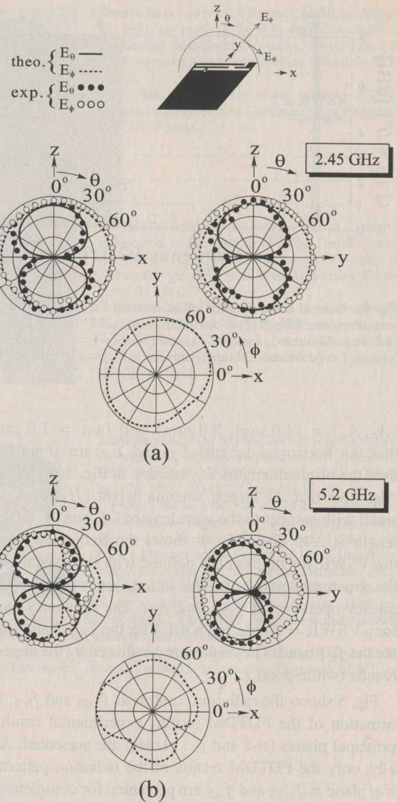
Fig. 5. Radiation patterns of an inverted FL antenna. (a) At 2.45 GHz. (b) At 5.2 GHz. The structural parameters are (H_L, L_L) = (4.5 \text{ mm}, 24.5 \text{ mm}) , (H_F, L_F) = (2.5 \text{ mm}, 10.5 \text{ mm}) , L_{FD} = 7.5 \text{ mm} , (H_P, L_P) = (2.5 \text{ mm}, 9.0 \text{ mm}) , (A_x, A_y) = (4.0 \text{ mm}, 3.0 \text{ mm}) , and (L_x \times L_y) = (30 \text{ mm} \times 25.5 \text{ mm}) .
