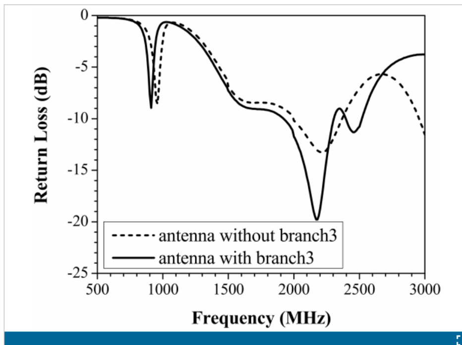
Fig. 2. Simulated return loss of the antennas with and without tuning branch 3.
