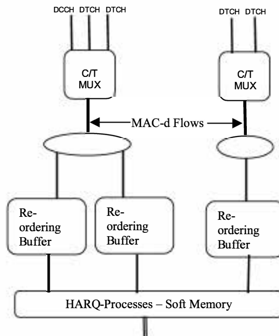
Figure 6.1.2-1: MAC-d architecture
