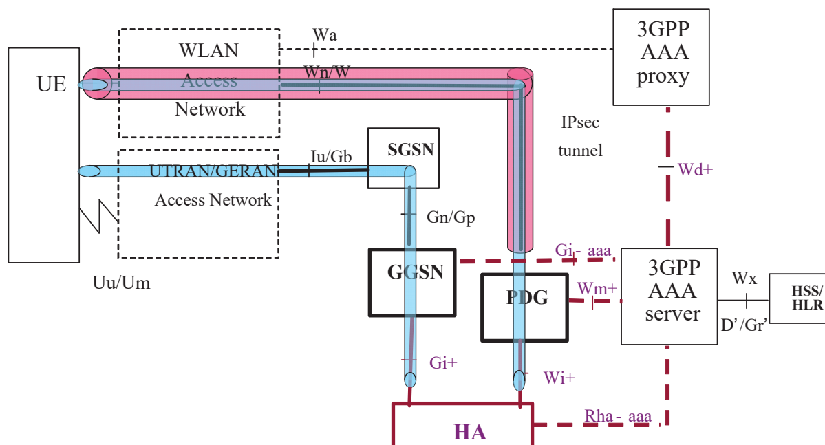
Figure E.5: Use of MIPv6 or MIPv4 with co-CoA for GPRS-WLAN mobility
