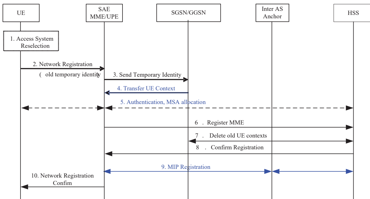
Figure 7.5-7: Information flow for change in idle state from 2G/3G to SAE/LTE
