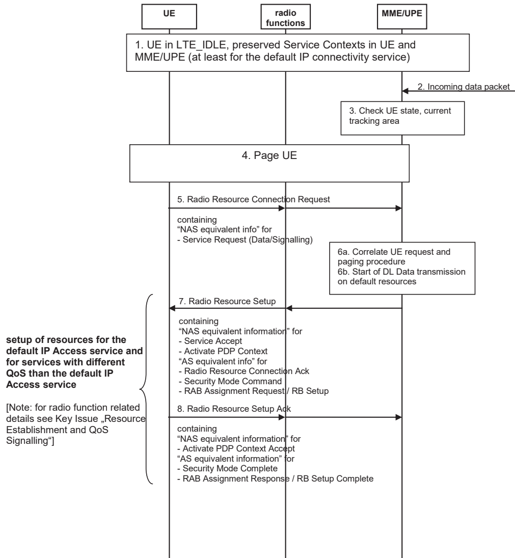
Figure 7.14-1: Information flow for paging and C-plane establishment
