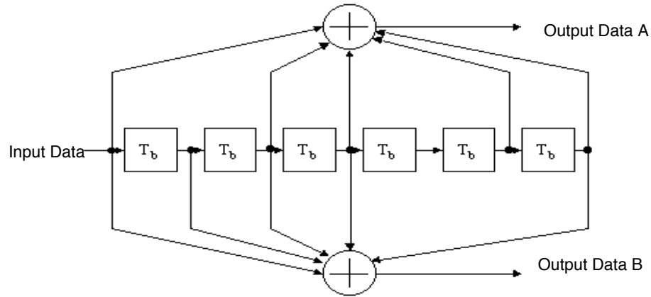
Figure 114—Convolutional encoder ( k = 7 )
