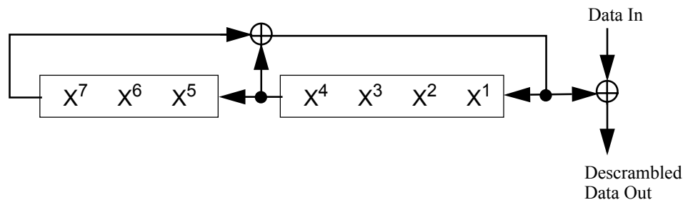
Figure 113—Data scrambler
