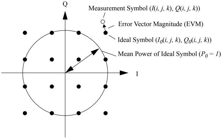
Figure 121—Constellation error
