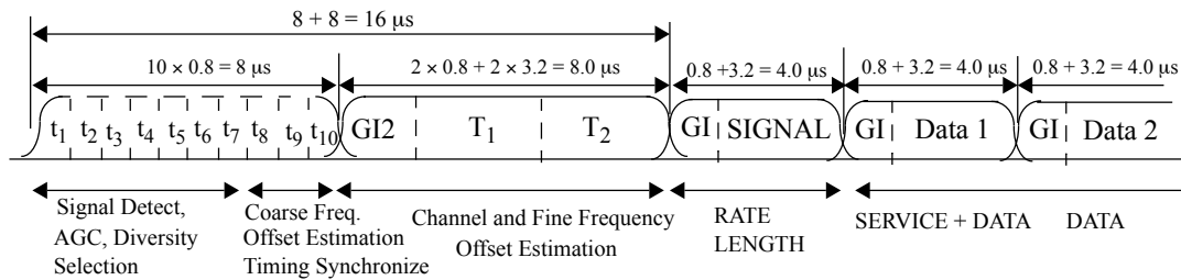
Figure 110—OFDM training structure
