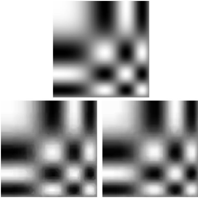
Fig. 8. Subjective comparison: Detail of a chirp image coded with QP = 36 . Top: Original. Left: Encoded without ABT (187 720 bit, 30.25 dB). Right: Encoded with ABT (158 304 bit, 32.53 dB).
