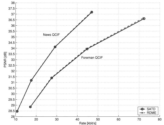
Fig. 2. Comparison of the coding performance for ABT when using the SATD ( \circ ) or the RD cost (RDME, \times ) for motion estimation. Results are presented for the test sequences FOREMAN and NEWS. The sequences were encoded with constant QP in a IPPP structure at 15 Hz using two reference frames and a search range of 32 pixels.
