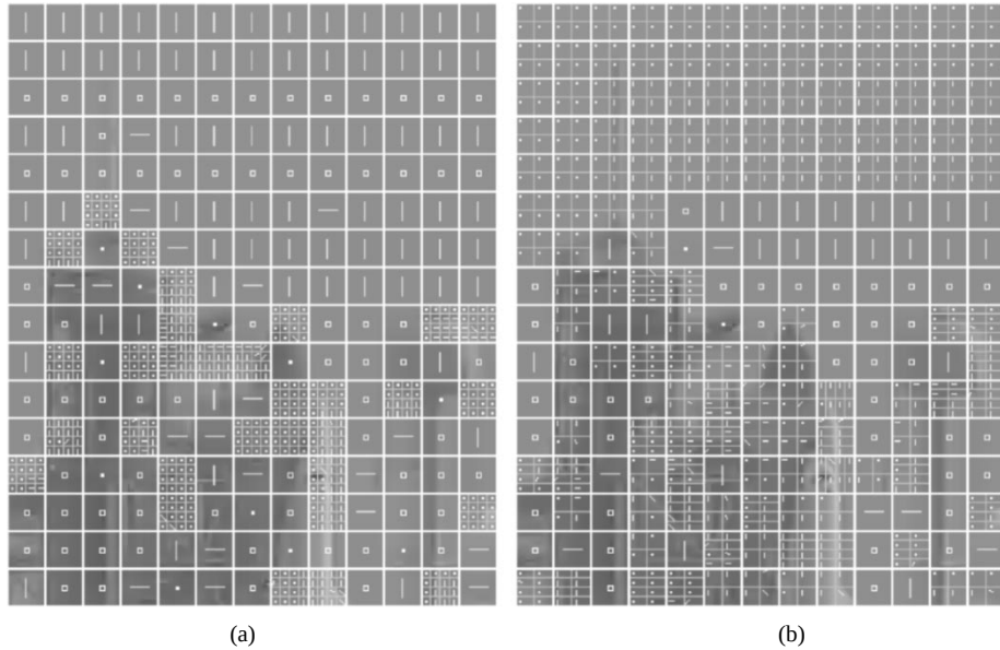
Fig. 11. Intra mode selection for the region shown in Fig. 10. (a) Encoded without ABT. (b) Encoded with ABT. Macroblocks are marked white. Subblocks of 4 \times 4 or ABT intra modes are marked in light gray. The directional modes are indicated by corresponding lines for both intra 16 \times 16 and subblock modes. DC prediction is indicated by a dot ( \bullet ). Intra 16 \times 16 plane prediction is indicated by an empty square ( \square ).
