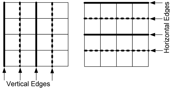
Figure 8-10 – Boundaries in a macroblock to be filtered
