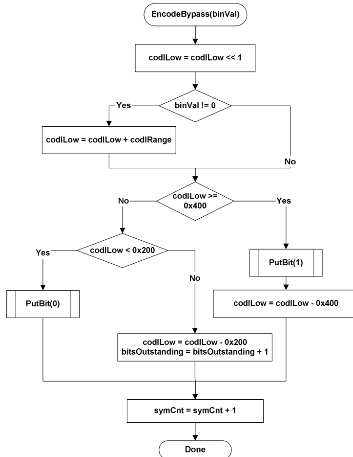
Figure 9-10 – Flowchart of encoding bypass
