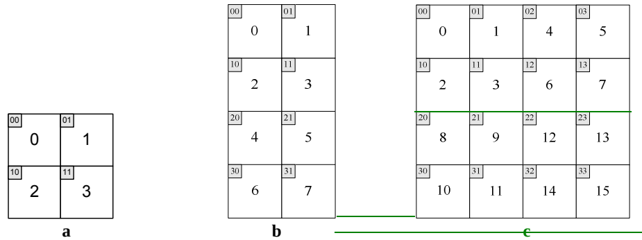
Figure 8-7 – Assignment of the indices of dcC to chroma4x4BlkIdx:
