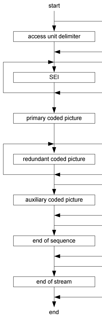
Figure 7-1 – Structure of an access unit not containing any NAL units with nal_unit_type equal to 0, 7, 8, or in the range of 12 to 18, inclusive, or in the range of 20 to 31, inclusive
