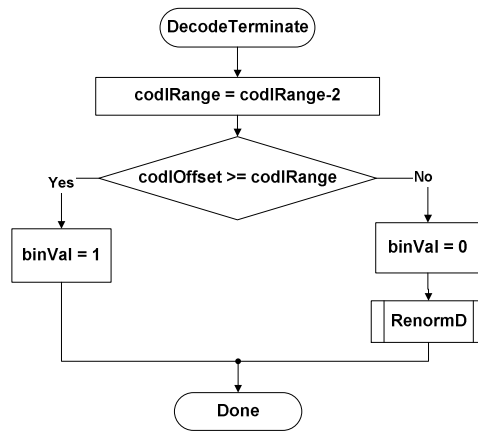
Figure 9-6 – Flowchart of decoding a decision before termination
