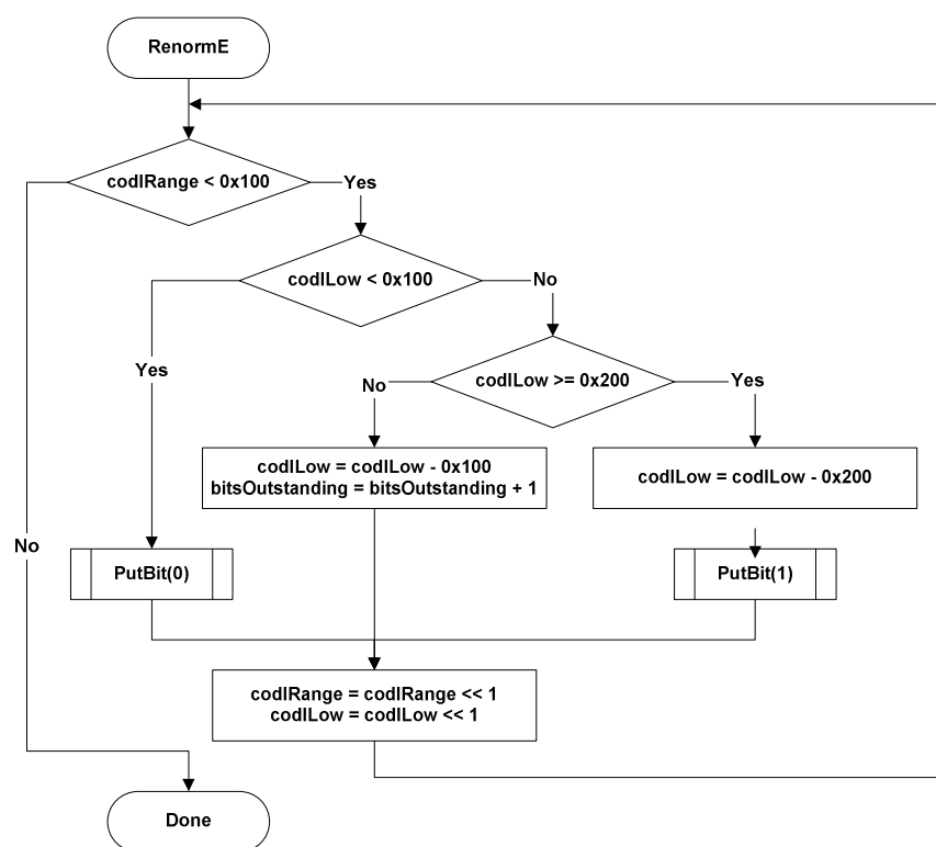
Figure 9-8 – Flowchart of renormalization in the encoder
