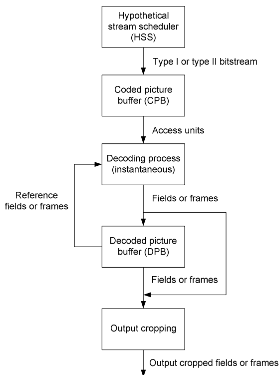
Figure C-2 – HRD buffer model
