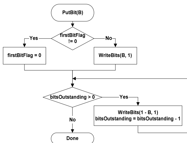
Figure 9-9 – Flowchart of PutBit(B)
