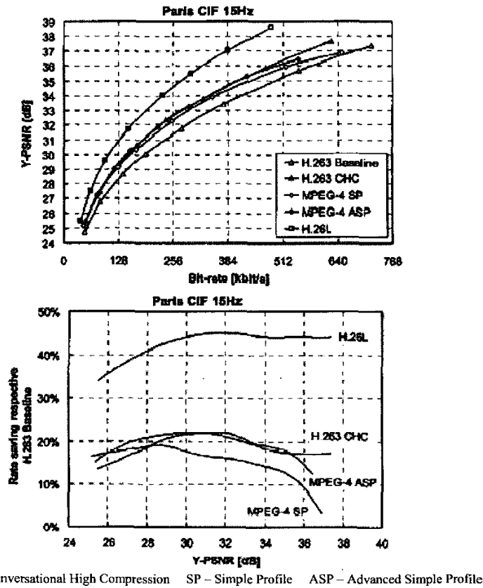
Fig. 53. Rate-distortion and bit-rate saving curves for Paris at 15 Hz in conversational video comparison [8]
