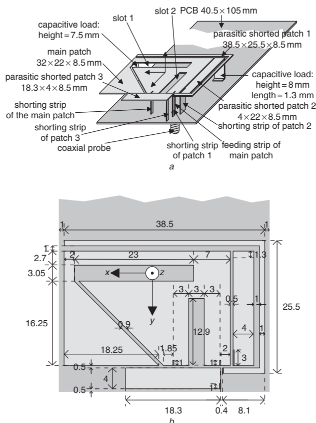
Fig. 1 3D view of multiband antenna a 3D view b Top view (all dimensions in millimetres)
