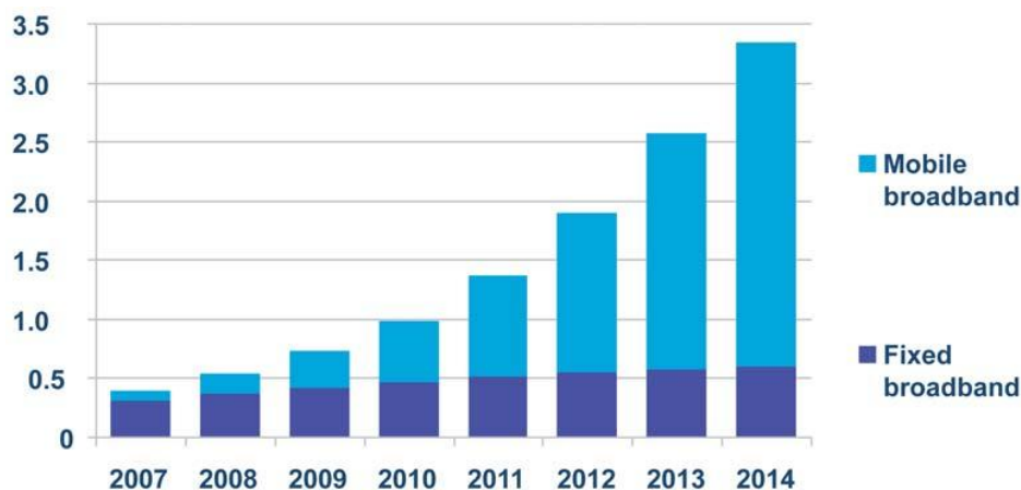
Figure 1: Broadband growth 2007–2014
