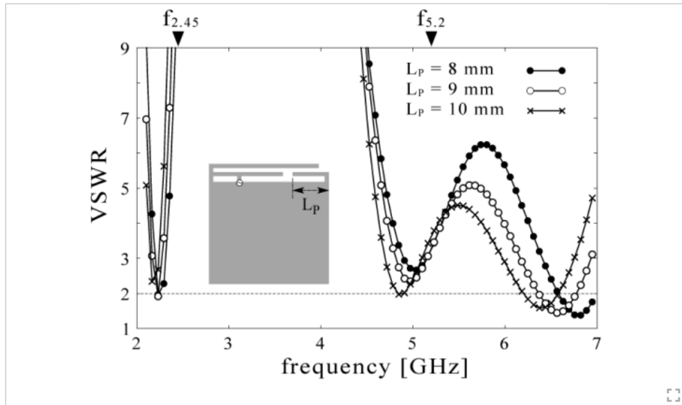
Fig. 3. Effects of the length of a parasitic L element, L_P , on the VSWR, where the structural parameters (H_L, L'_L) = (4.5 \text{ mm}, 27.5 \text{ mm}) , (H_F, L'_F) = (2.5 \text{ mm}, 11 \text{ mm}) , and L_{FD} = 7.5 \text{ mm} are used. The ground plate size is L_x \times L_y = 30 \text{ mm} \times 25.5 \text{ mm} .
