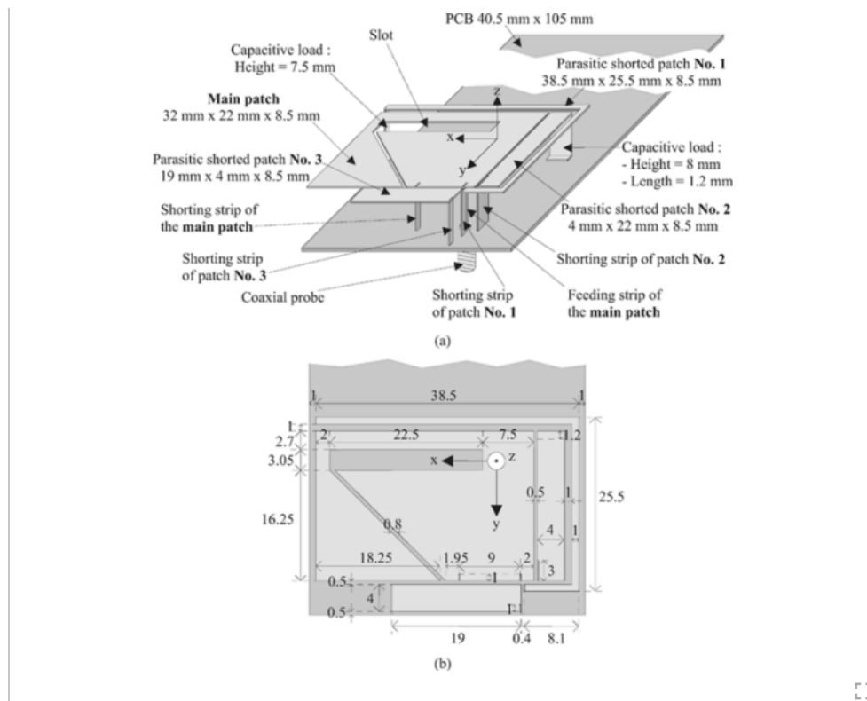
Fig. 1. Configuration of the quad-band antenna. (a) Side view. (b) Top view : all dimensions are in millimeter.
