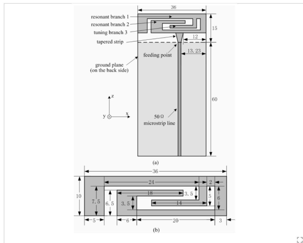
Fig. 1. Configuration of the proposed planar monopole antenna. (a) General view of the antenna. (b) Detailed dimensions of the main radiating element. All dimensions are in millimeter.
