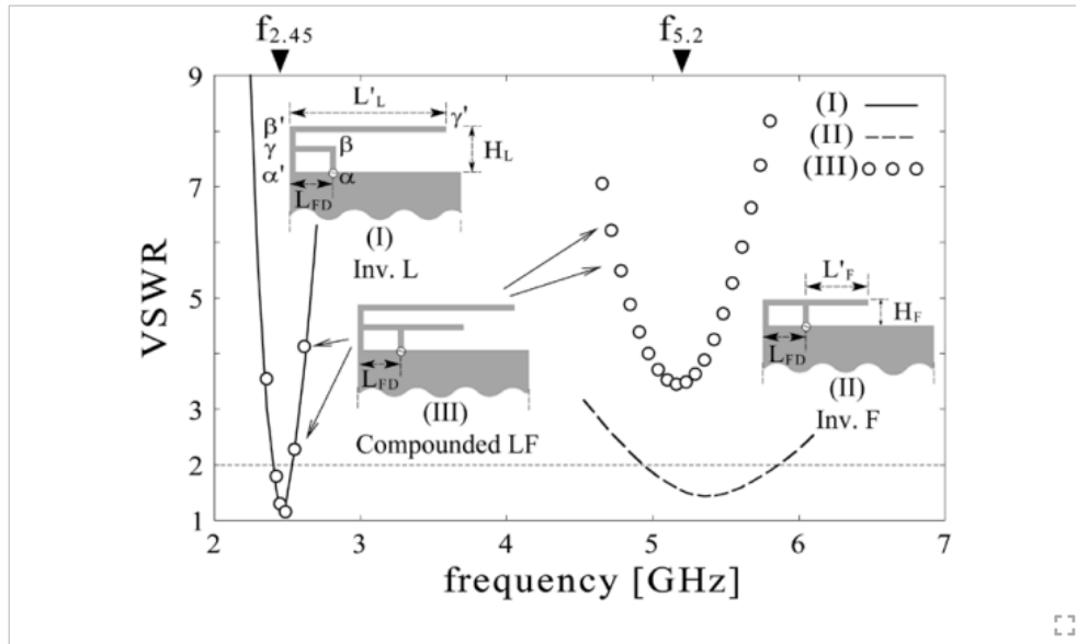
Fig. 2. VSWRs of three structures. The structural parameters for an inverted L element (I) are (H_L, L'_L) = (4.5 \text{ mm}, 27.5 \text{ mm}) and L_{FD} = 7.5 \text{ mm} , and those for an inverted F element (II) are (H_F, L'_F) = (2.5 \text{ mm}, 11 \text{ mm}) and L_{FD} = 7.5 \text{ mm} . A compounded LF (III) has the same structural parameters used for the sub-elements (I) and (II). The ground plate sizes in structures (I), (II), and (III) are the same: L_x \times L_y = 30 \text{ mm} \times 25.5 \text{ mm} .
