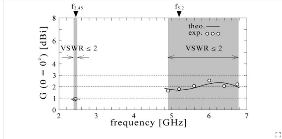
Fig. 6. Gain in the z -direction of an inverted FL antenna. The structural parameters are (H_L, L_L) = (4.5 mm, 24.5 mm), (H_F, L_F) = (2.5 mm, 10.5 mm), L_{FD} = 7.5 mm, (H_P, L_P) = (2.5 mm, 9.0 mm), (A_x, A_y) = (4.0 mm, 3.0 mm), and (L_x \times L_y) = (30 mm \times 25.5 mm).
