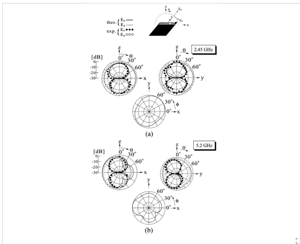
Fig. 5. Radiation patterns of an inverted FL antenna. (a) At 2.45 GHz. (b) At 5.2 GHz. The structural parameters are (H_L, L_L) = (4.5 \text{ mm}, 24.5 \text{ mm}) , (H_F, L_F) = (2.5 \text{ mm}, 10.5 \text{ mm}) ,
