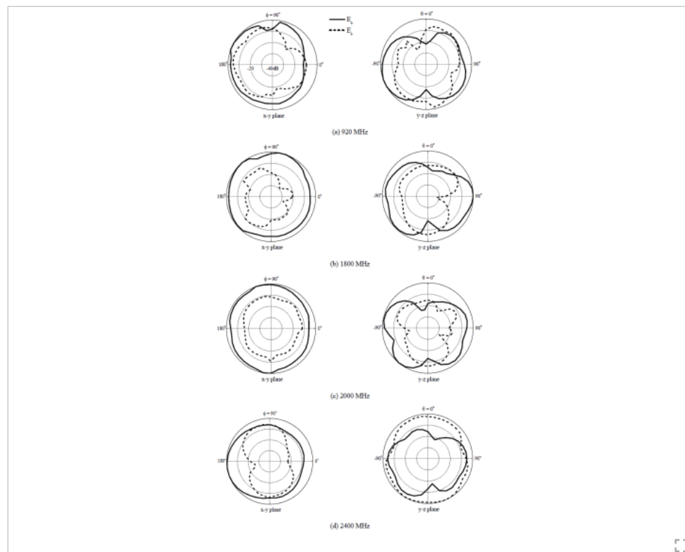
Fig. 4. Measured radiation patterns of the proposed antenna at (a) 920 MHz, (b) 1800 MHz, (c) 2000 MHz and (d) 2400 MHz.
