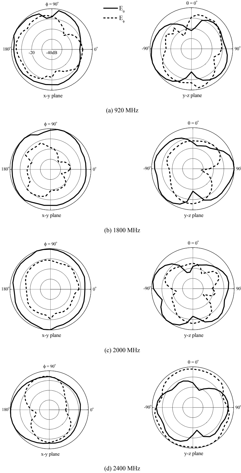
Fig. 4. Measured radiation patterns of the proposed antenna at (a) 920 MHz, (b) 1800 MHz, (c) 2000 MHz and (d) 2400 MHz.
