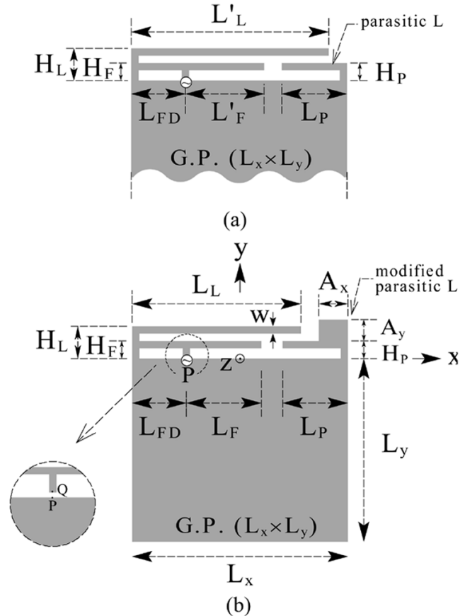
Fig. 1. Antenna structures. (a) A compound of inverted L and F elements (referred to as a compounded LF) with a parasitic L element above a co-planar ground plate (GP). (b) A compounded LF with a modified parasitic L element above a co-planar ground plate, referred to as the inverted FL antenna (InvFLA). The ground plate size in (a) is the same as that in (b): L_x \times L_y = 30 \text{ mm} \times 25.5 \text{ mm} .
