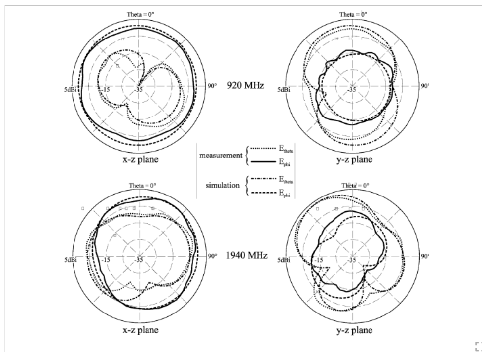
Fig. 4. Measured and simulated radiation gain patterns at 920 MHz and 1940 MHz for the quad-band antenna. Antenna orientation is given in Fig. 1.
