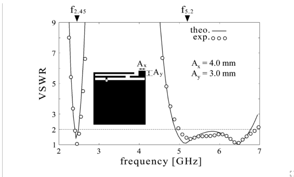
Fig. 4. VSWR for an inverted FL antenna. The structural parameters are (H_L, L_L) = (4.5 \text{ mm}, 24.5 \text{ mm}) , (H_F, L_F) = (2.5 \text{ mm}, 10.5 \text{ mm}) , L_{FD} = 7.5 \text{ mm} , (H_P, L_P) = (2.5 \text{ mm}, 9.0 \text{ mm}) , (A_x, A_y) = (4.0 \text{ mm}, 3.0 \text{ mm}) , and (L_x \times L_y) = (30 \text{ mm} \times 25.5 \text{ mm}) .
