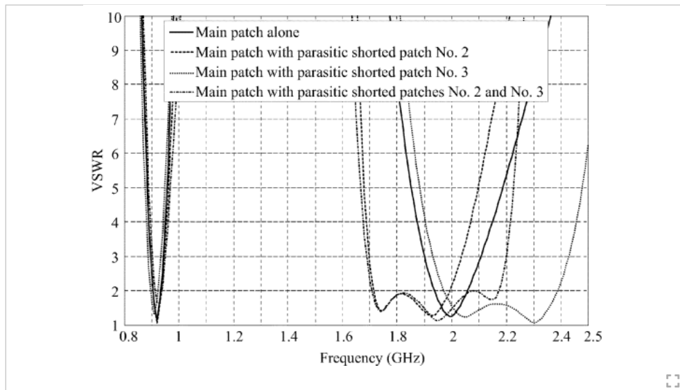
Fig. 2. Simulated VSWR of the main patch with and without parasitic shorted patches no. 2 and no. 3.
