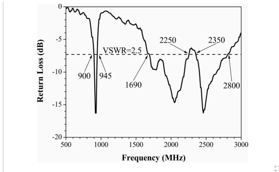
Fig. 3. Measured return loss of the proposed antenna.
