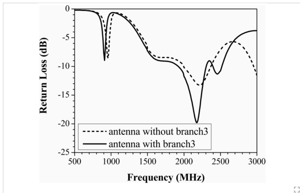
Fig. 2. Simulated return loss of the antennas with and without tuning branch 3.
