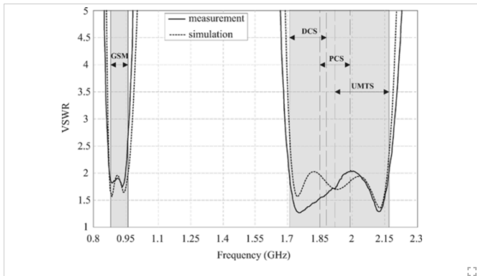
Fig. 3. Measured and simulated VSWR of the quad-band antenna.
