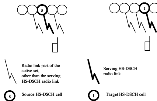
Figure 9-1: Serving HS-DSCH cell change
