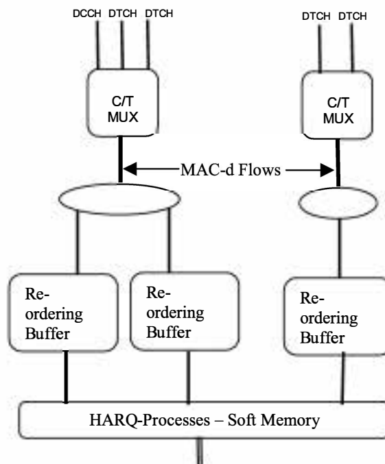
Figure 6.1.2-1: MAC-d architecture
