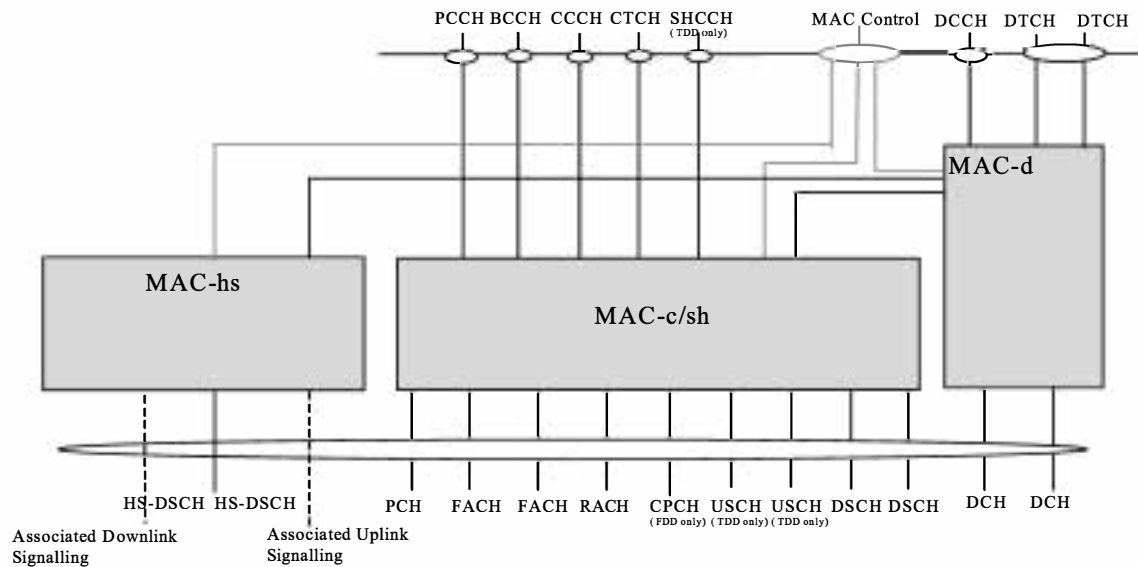
Figure 6.1.1-1: UE side MAC architecture with HS-DSCH
