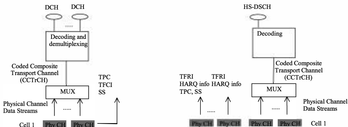
DCH model with HS-DSCH(s)
