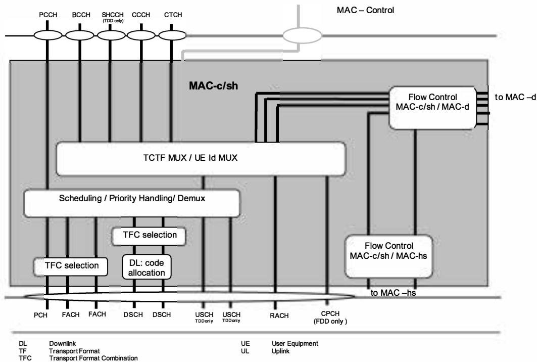
Figure 6.2.2-1: UTRAN side MAC architecture/MAC-c/sh details
