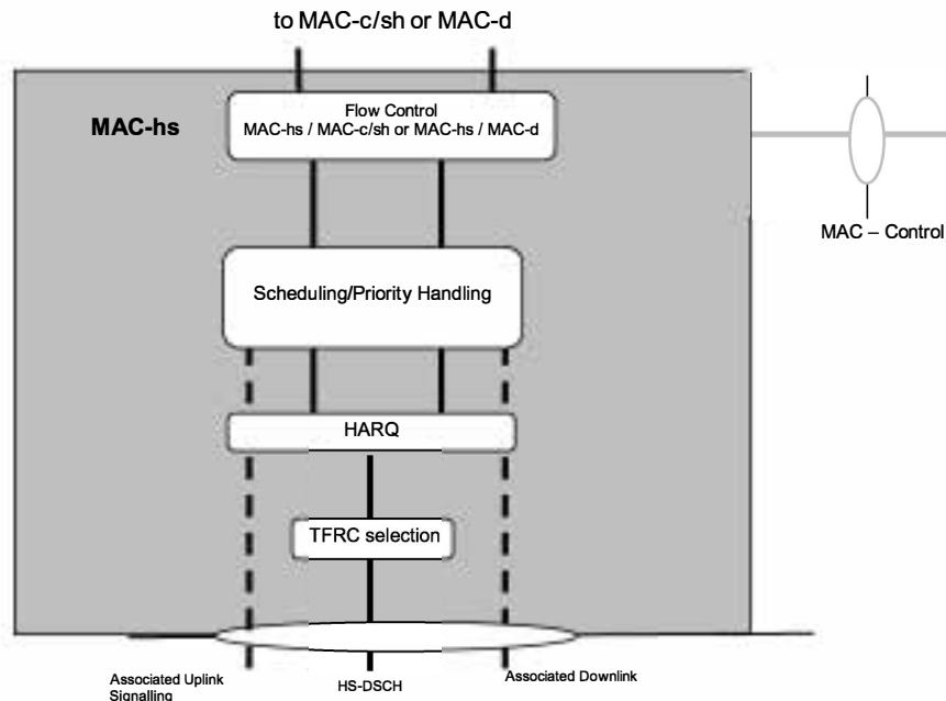
Figure 6.2.3-1: UTRAN side MAC architecture/MAC-hs details
