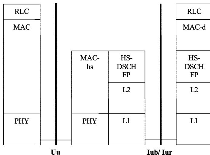
Figure 5.1-2: Protocol Architecture of HS-DSCH, Configuration without MAC-c/sh
