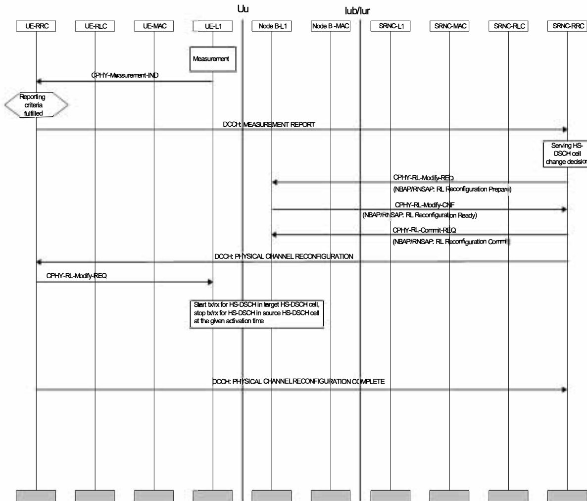
Figure 9.3-1: Intra-Node B synchronised serving HS-DSCH cell change
