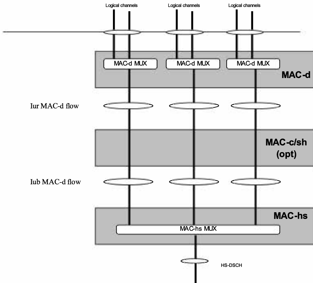
Figure 6.2.1-2: UTRAN side of MAC multiplexing
