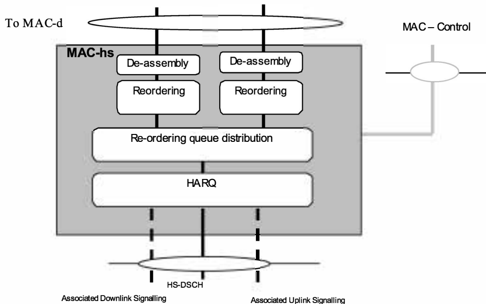
Figure 6.1.4-1: UE side MAC architecture/MAC-hs details
