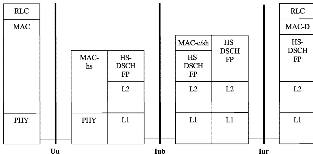
Figure 5.1-1: Protocol Architecture of HS-DSCH, Configuration with MAC-c/sh
