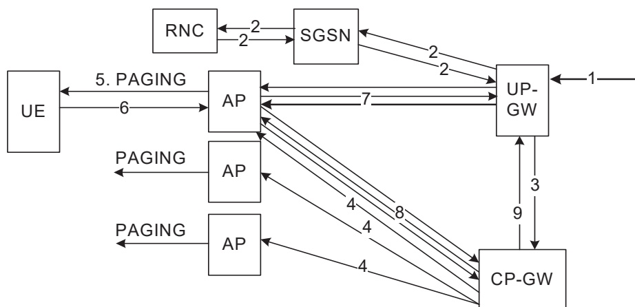
Figure D.3: Transfer from Idle to Active states for Ues caused by downlink Traffic whilst in EUTRA coverage
