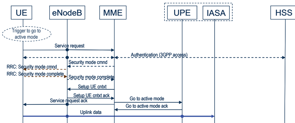
Figure H.6.2-1: Alternative B, service request
