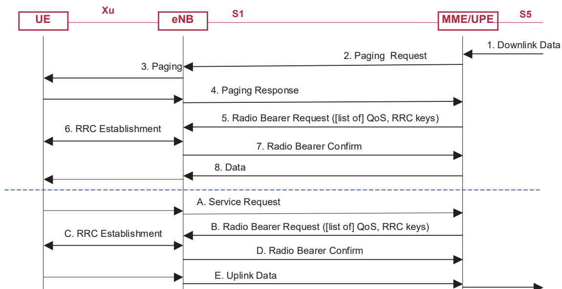
Figure H.6.1: Alternative A
