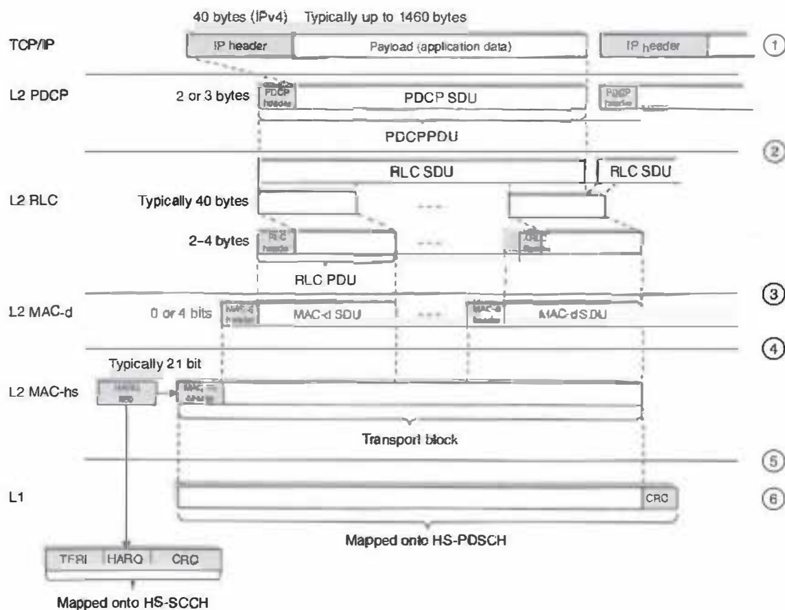
Figure 9.12 Data flow at UTRAN side.
