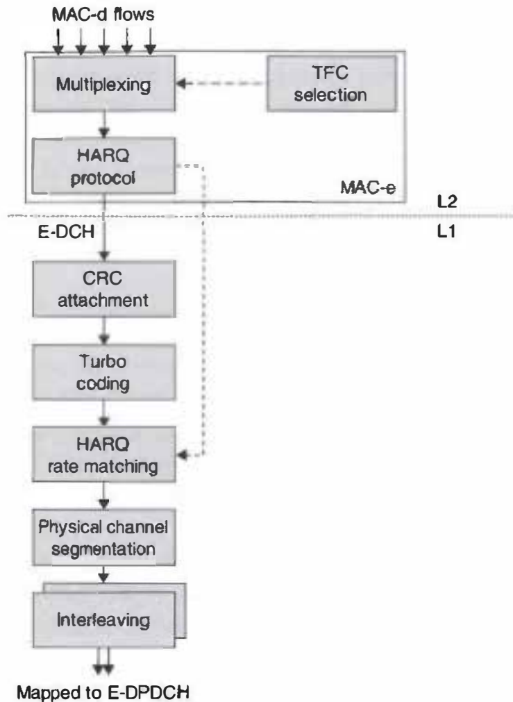
Figure 10.5 MAC-e and physical-layer processing.
