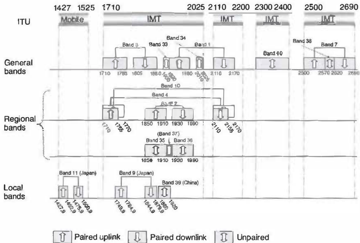
Figure 20.1 Operating bands specified in 3GPP above 1 GHz and the corresponding ITU allocation.
