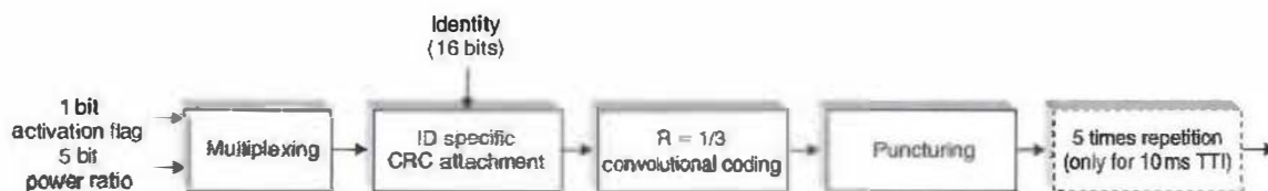
Figure 10.30 E-AGCH coding structure.
