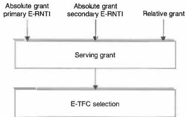
Figure 10.16 The relation between absolute grant, relative grant and serving grant.
