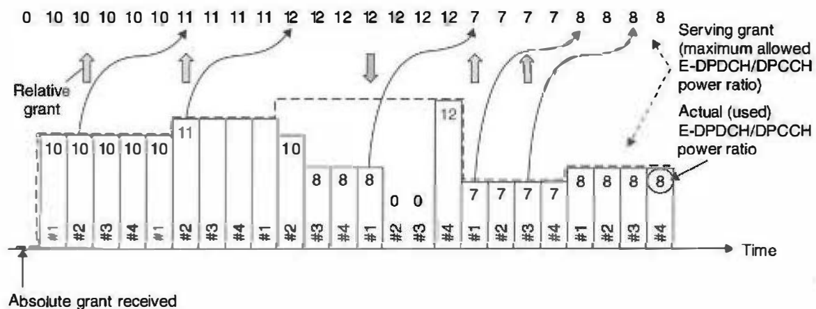
Figure 10.8 Illustration of relative grant usage.
