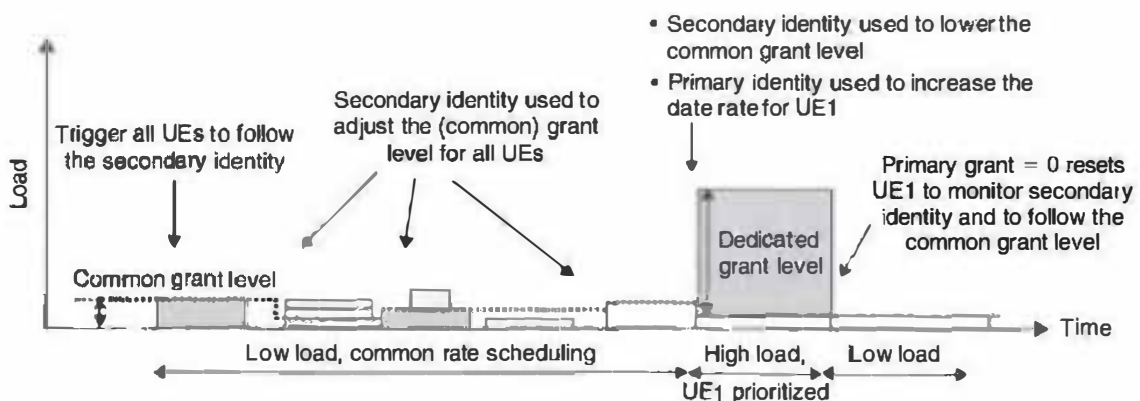
Figure 10.18 Example of common and dedicated scheduling.
