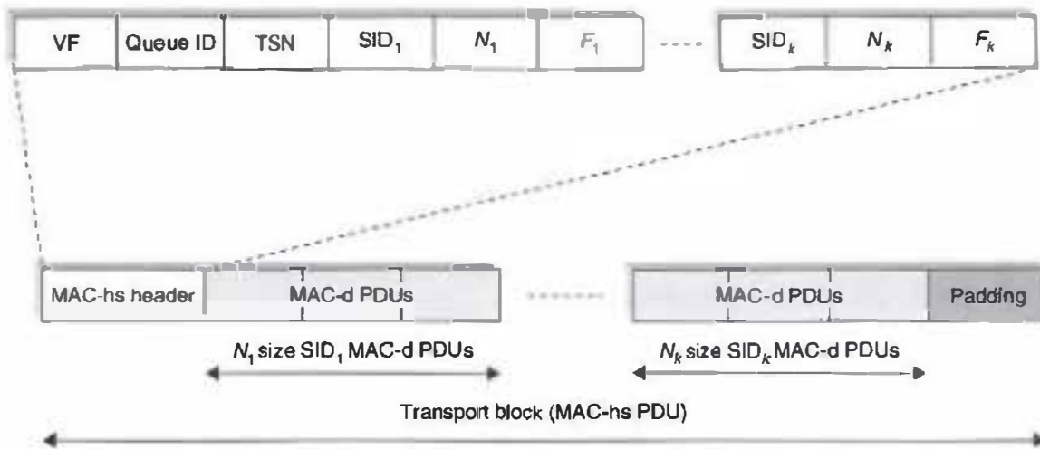
Figure 9.20 The structure of the MAC-hs header.
