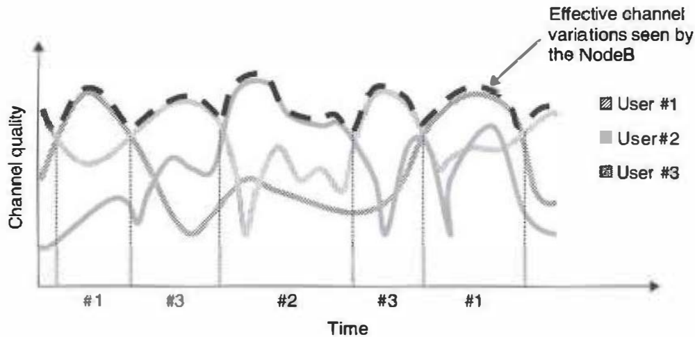
Figure 9.2 Channel-dependent scheduling for HSDPA.
