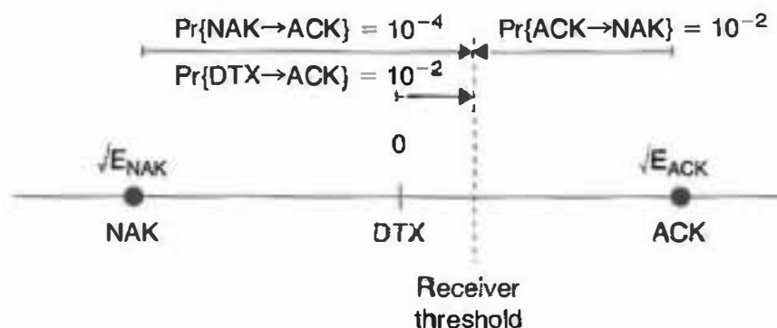
Figure 9.25 Detection threshold for the ACK/NAK field of HS-DPCCH.
