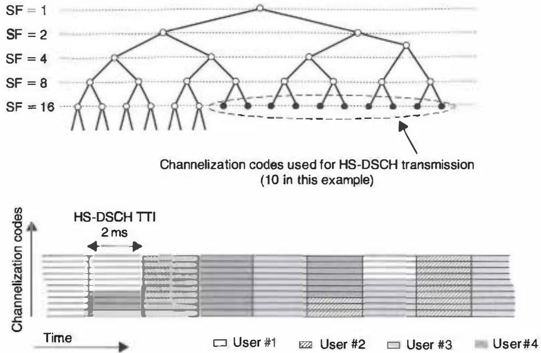
Figure 9.1 Time- and code-domain structure for HS-DSCH.
