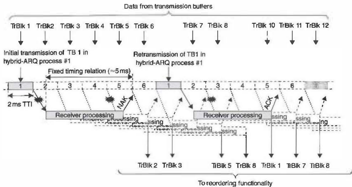
Figure 9.10 Multiple hybrid-ARQ process (six in this example).
