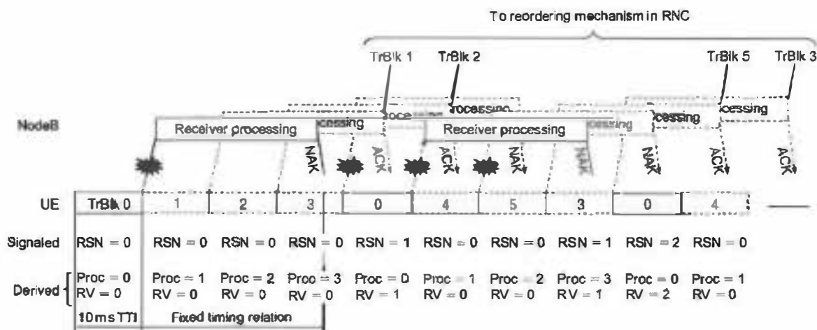
Figure 10.11 Multiple hybrid ARQ processes for Enhanced Uplink.
