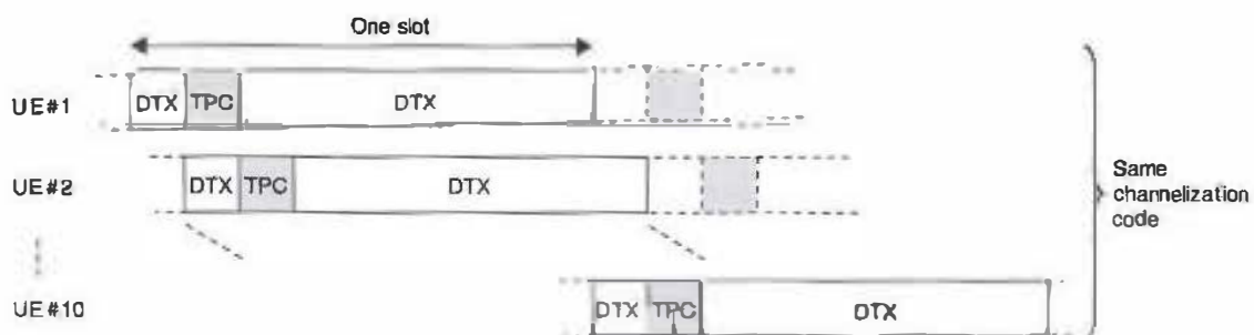
Figure 9.23 Fractional DPCH (F-DPCH), introduced in Release 6.
