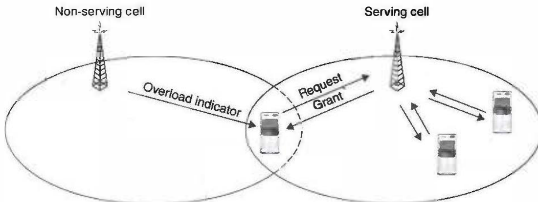
Figure 10.1 Enhanced Uplink scheduling framework.
