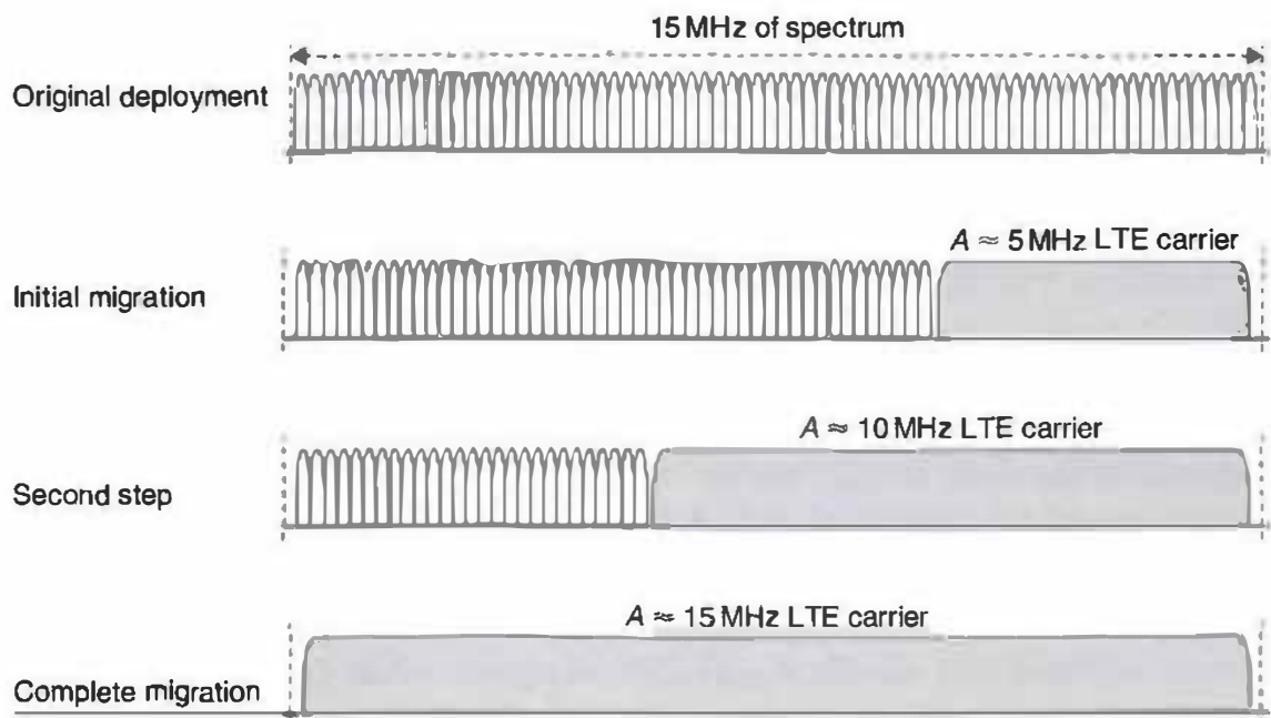
Figure 20.3 Example of how LTE can be migrated step-by-step into a spectrum allocation with an original GSM deployment.
