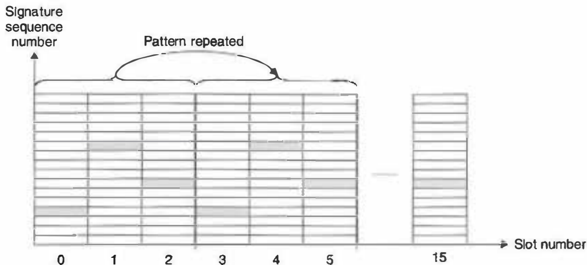
Figure 10.29 Illustration of signature sequence hopping.
