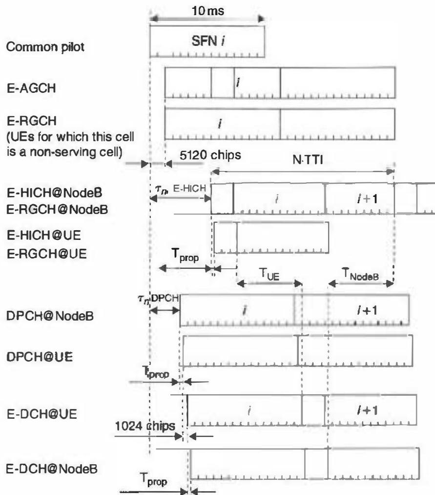
Figure 10.32 Timing relation for downlink control channels, 2 ms TTI.
