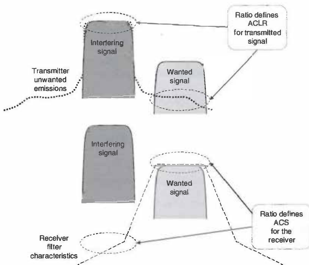
Figure 20.6 Definitions of ACLR and ACS, using example characteristics of an 'aggressor' interfering and a 'victim' wanted signal.
