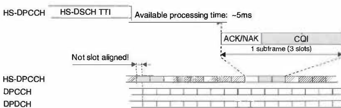
Figure 9.24 Basic structure of uplink signaling with IQ/code-multiplexed HS-DPCCH.
