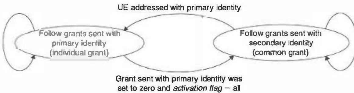
Figure 10.17 Illustration of UE monitoring of the two identities.
