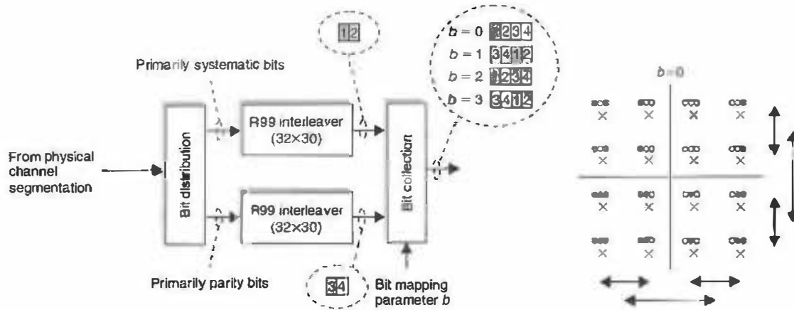
Figure 9.17 The channel interleaver for the HS-DSCH. The shaded parts are only used for 16QAM. Colors illustrate the mapping order for a sequence of 4 bits, where a bar on top of the figure denotes bit inversion.
