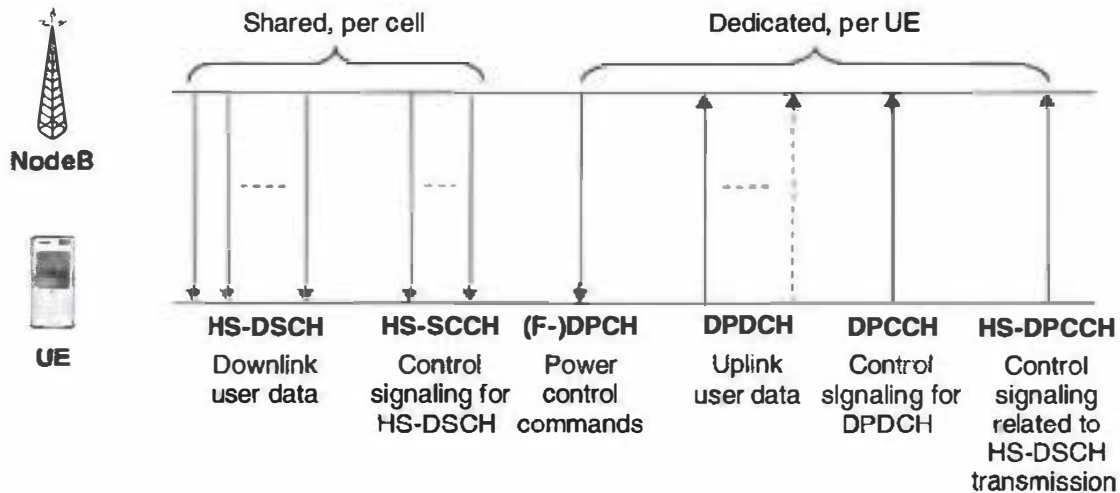
Figure 9.5 Channel structure with HSDPA.
