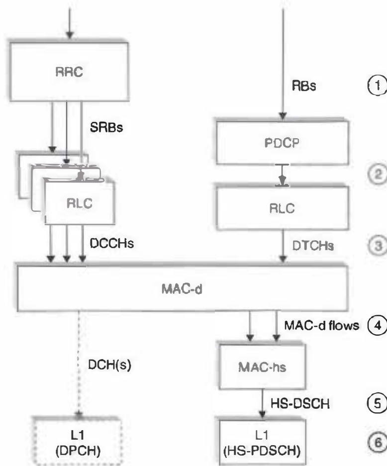
Figure 9.11 Protocol configuration when HS-DSCH is assigned. The numbers in the rightmost part of the figure corresponds to the numbers to the right in Figure 9.12.
