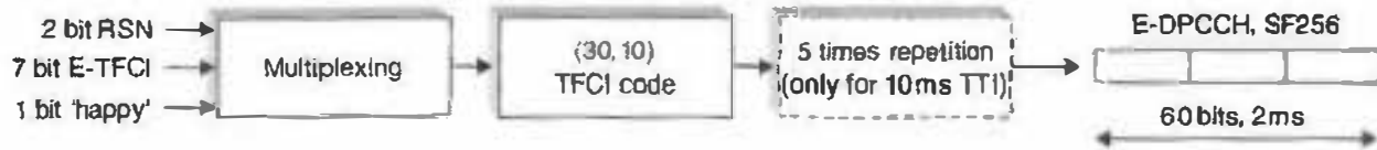
Figure 10.33 E-DPCCH coding.
