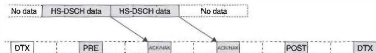
Figure 9.26 Enhanced ACK/NAK using PRE and POST.
