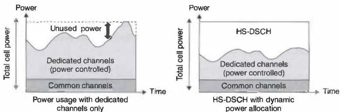
Figure 9.4 Dynamic power usage with HS-DSCH.
