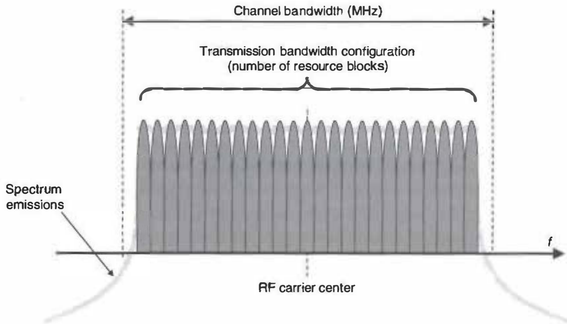
Figure 20.4 The channel bandwidth for one RF carrier and the corresponding transmission bandwidth configuration.
