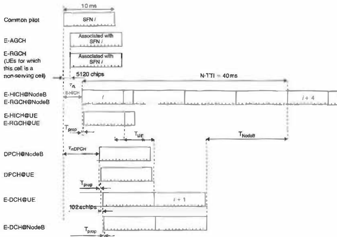
Figure 10.31 Timing relation for downlink control channels, 10ms TTI.
