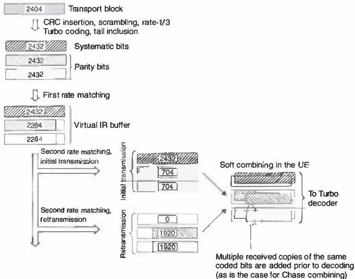
Figure 9.16 An example of the generation of different redundancy versions in the case of IR. The numbers indicate the number of bits after the different stages using the example case in the text.
