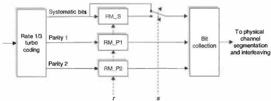
Figure 10.22 E-DCH rate matching and the r and s parameters. The bit collection procedure is identical to the QPSK bit collection for HS-DSCH.
