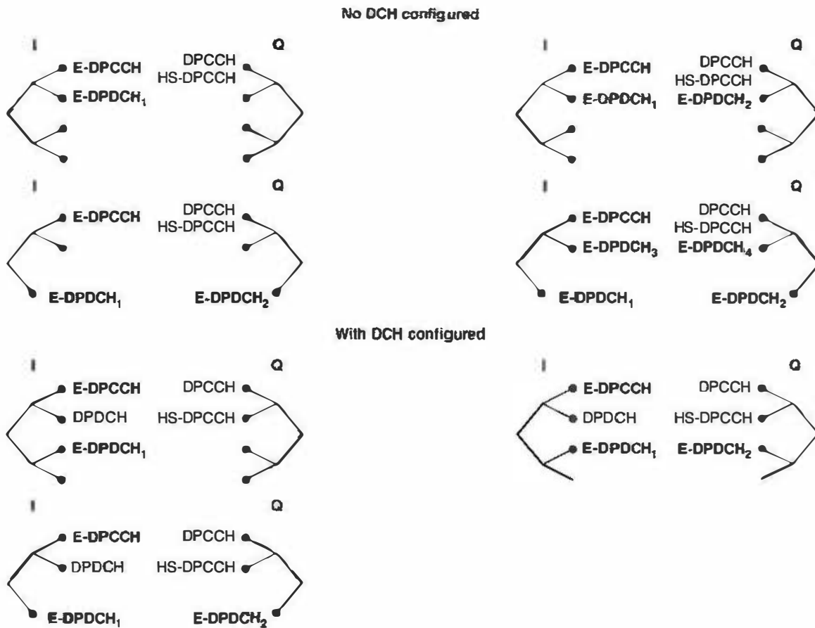
Figure 10.13 Code allocation in case of simultaneous E-DCH and HS-DSCH operation (note that the code allocation is slightly different when no HS-DPCCH is configured). Channels with SF > 4 are shown on the corresponding SF4 branch for illustrative purposes.
