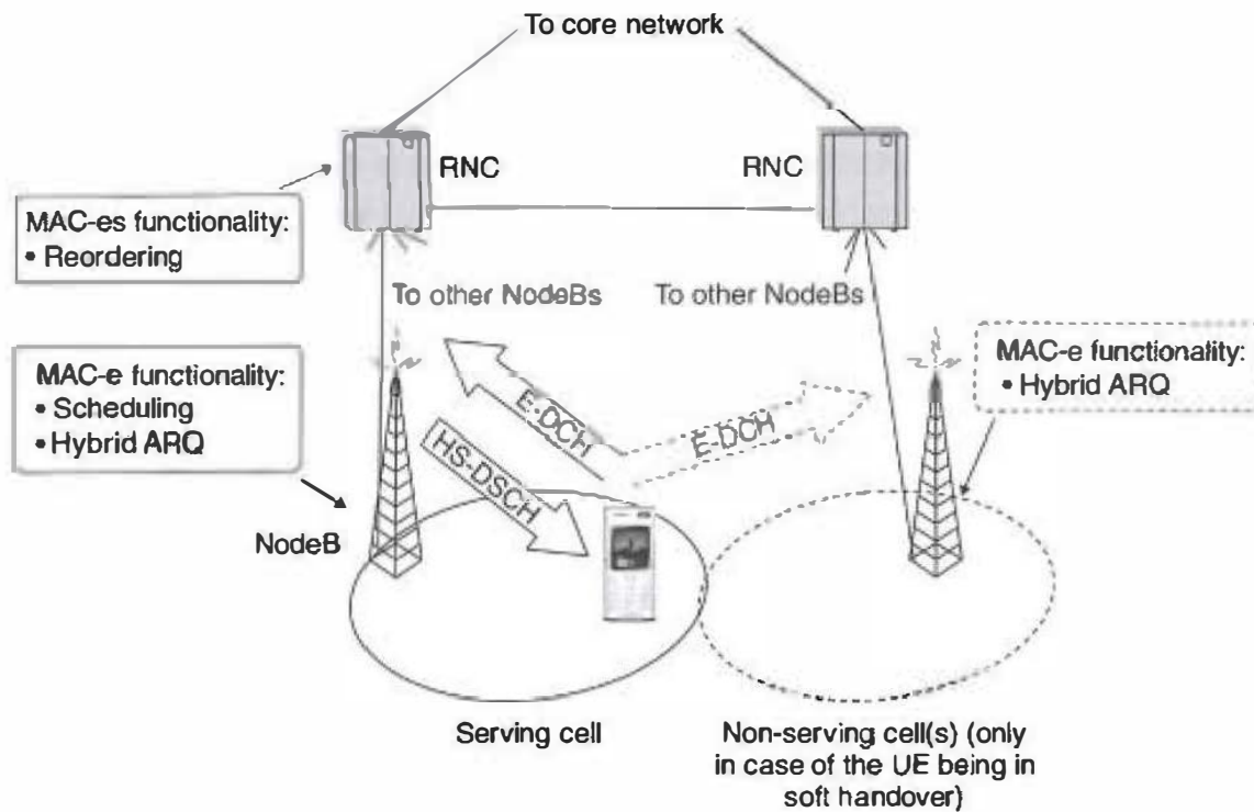
Figure 10.2 The architecture with E-DCH (and HS-DSCH) configured.
