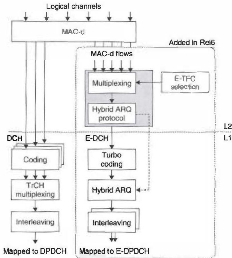
Figure 10.3 Separate processing of E-DCH and DCH.
