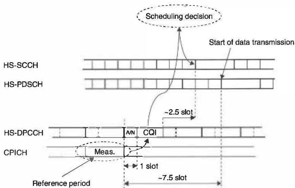
Figure 9.21 Timing relation for the CQI reports.
