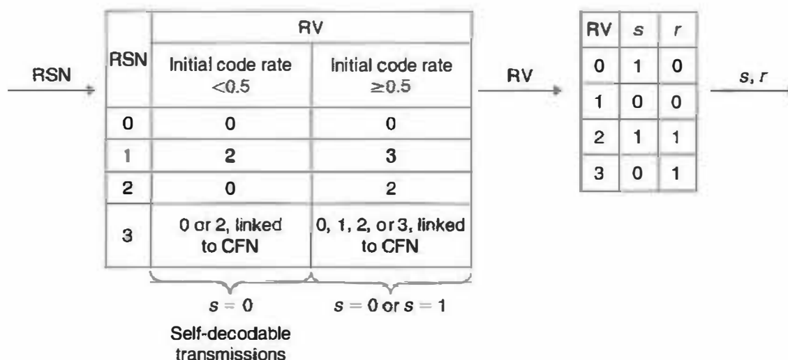
Figure 10.24 Mapping from RSN via RV to s and r .
