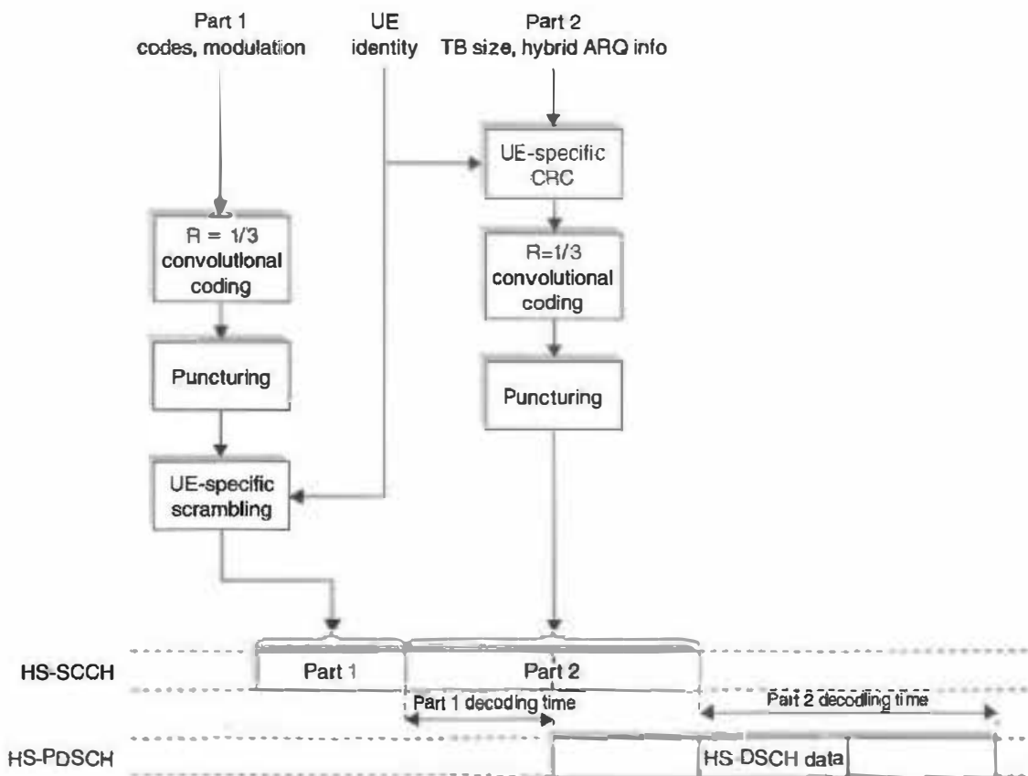
Figure 9.22 HS-SCCH channel coding.
