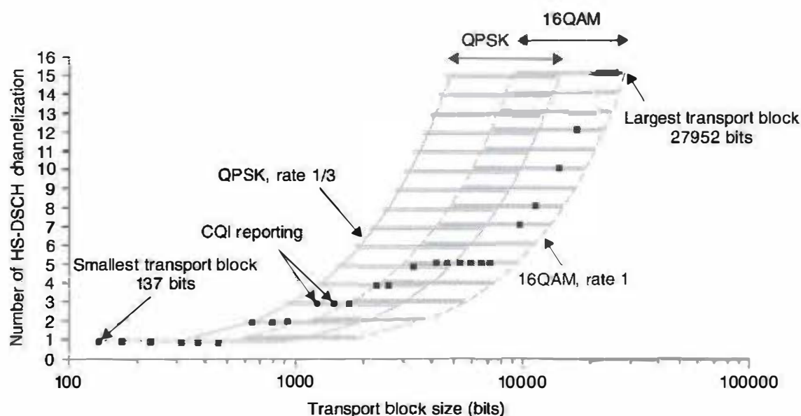
Figure 9.8 Transport-block sizes vs. the number of channelization codes for QPSK and 16QAM modulation. The transport-block sizes used for CQI reporting are also illustrated.
