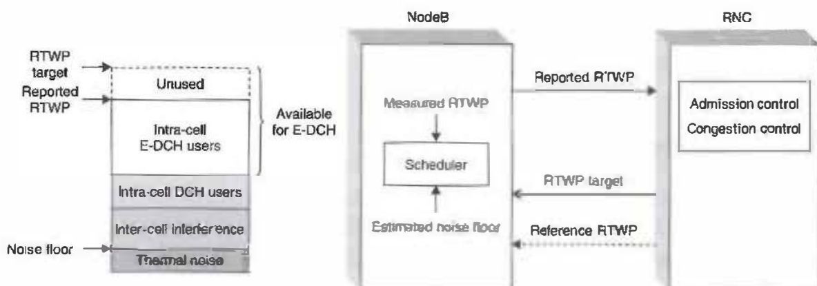
Figure 10.15 Illustration of the resource sharing between E-DCH and DCH channels.
