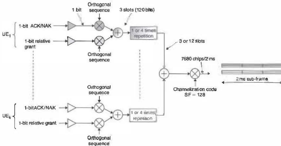
Figure 10.28 E-HICH and E-RGCH structures (from the serving cell).
