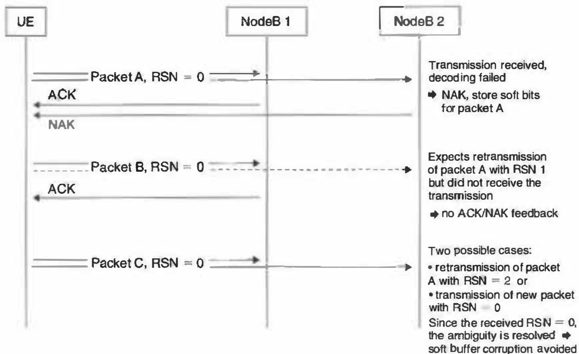
Figure 10.12 Retransmissions in soft handover.
