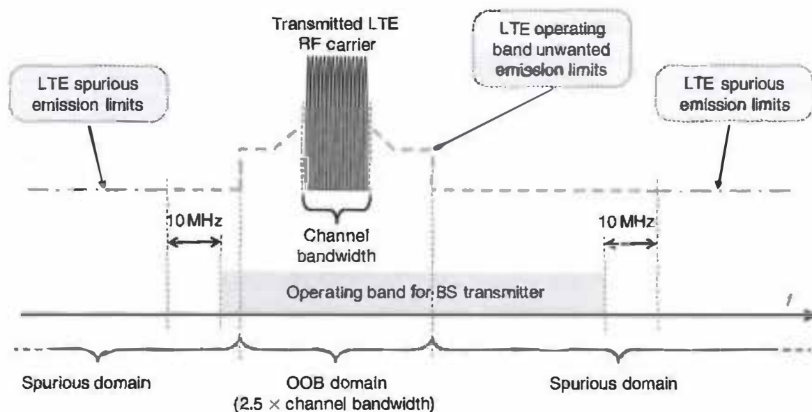
Figure 20.5 Defined frequency ranges for spurious emissions and operating band unwanted emissions.
