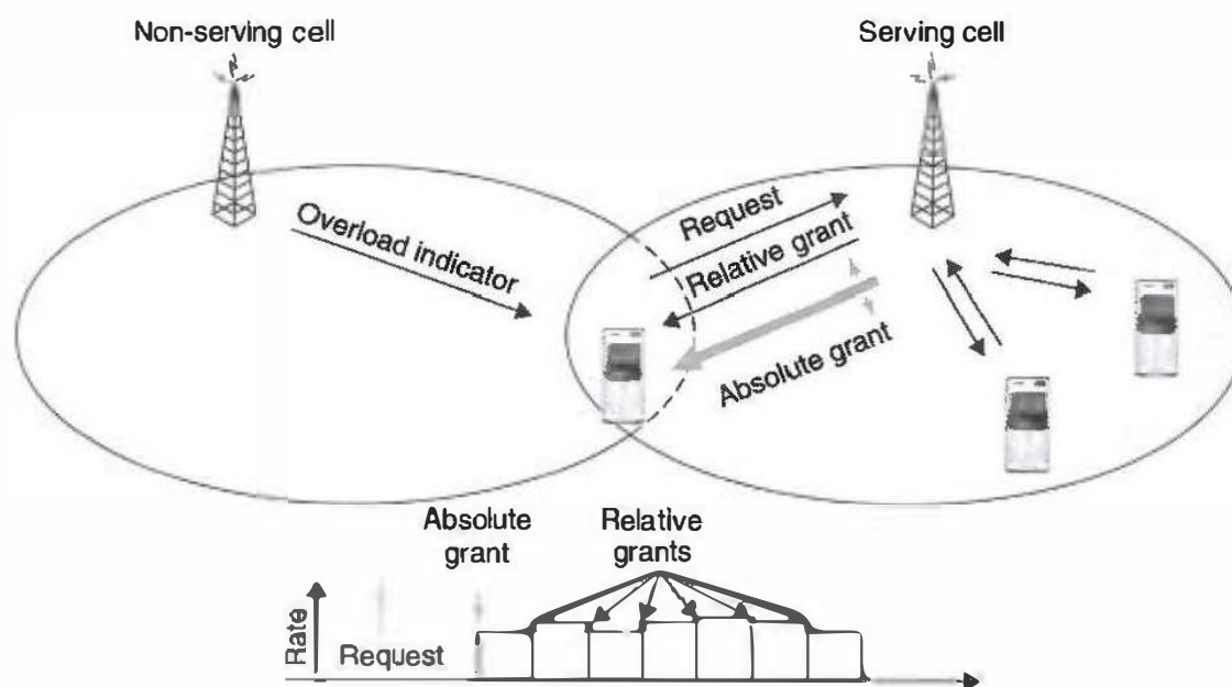
Figure 10.6 Overview of the scheduling operation.
