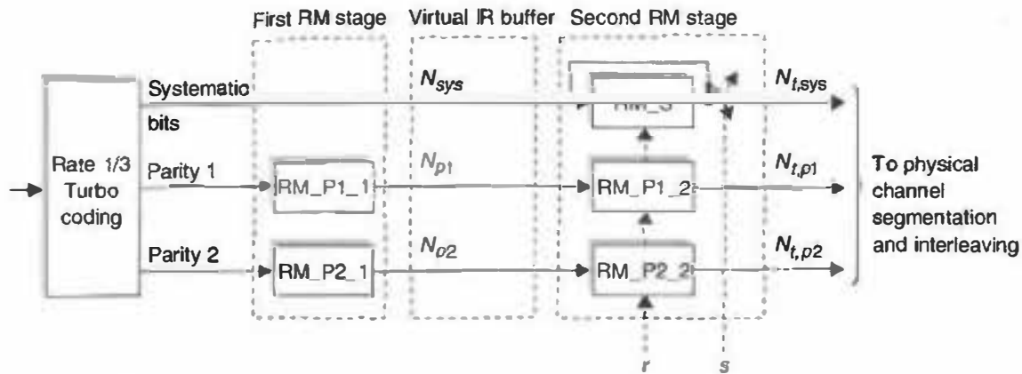
Figure 9.15 The principle of two-stage rate matching.
