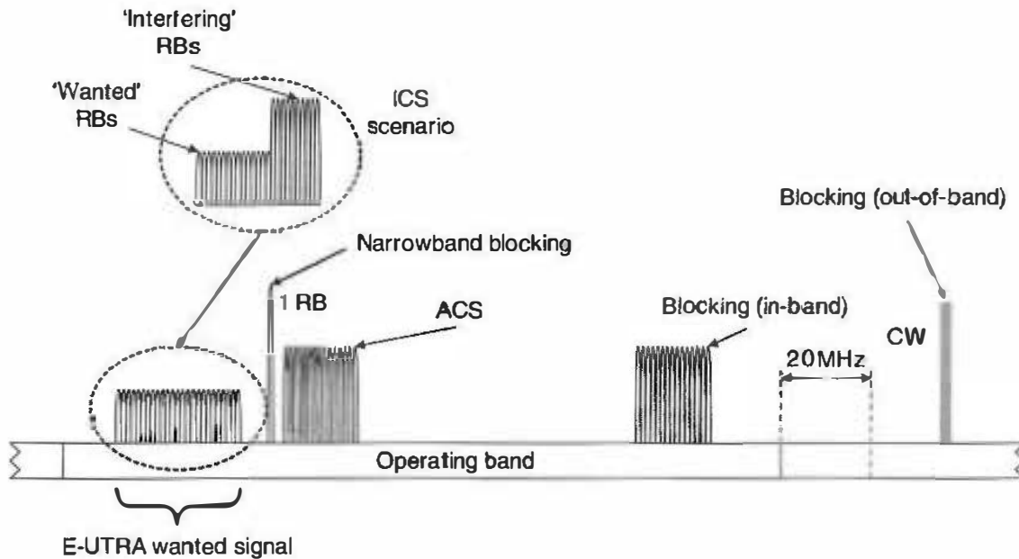
Figure 20.7 Requirements for receiver susceptibility to interfering signals in terms of blocking, ACS, narrowband blocking, and in-channel selectivity (ICS).
