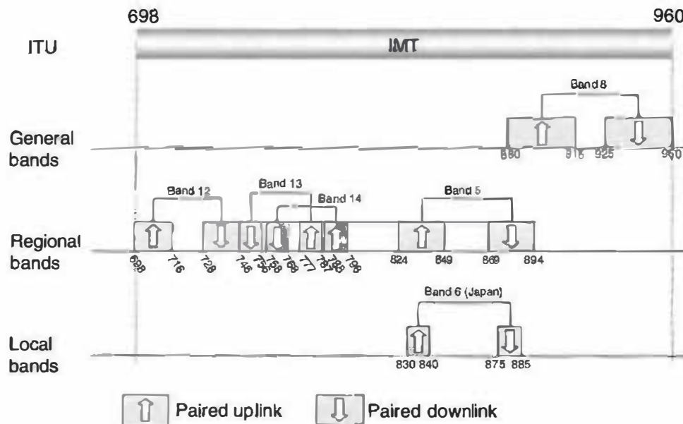
Figure 20.2 Operating bands specified in 3GPP below 1 GHz and the corresponding ITU allocation.
