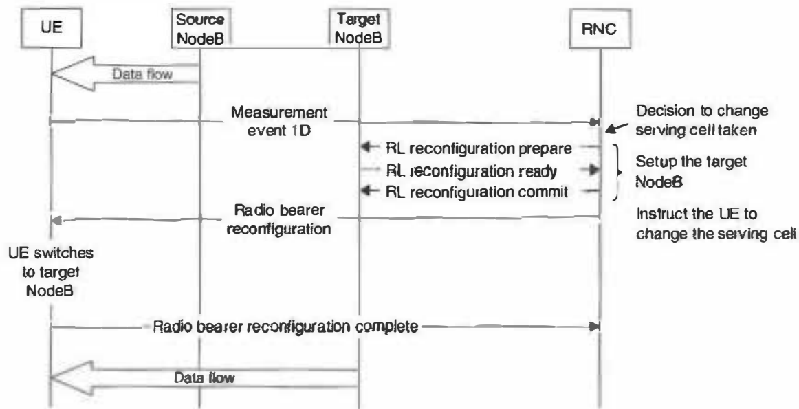
Figure 9.14 Change of serving cell for HSPA. It is assumed that both the source and target NodeB are part of the active set.
