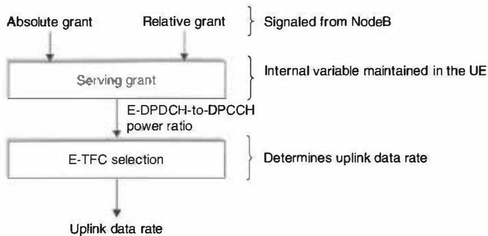
Figure 10.7 The relation between absolute grant, relative grant and serving grant.
