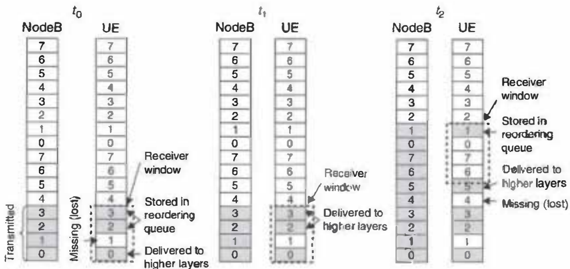
Figure 9.19 Illustration of the principles behind reordering queues.
