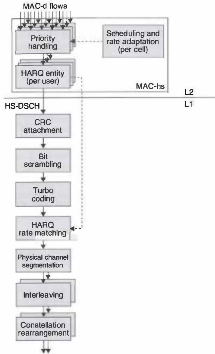
Figure 9.6 MAC-hs and physical-layer processing.
