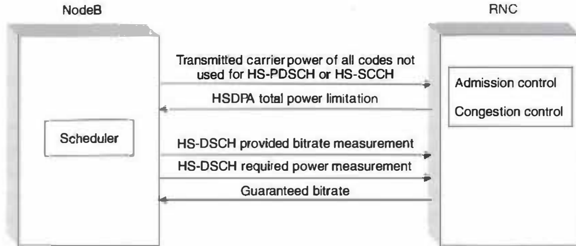
Figure 9.13 Measurements and resource limitations for HSDPA.
