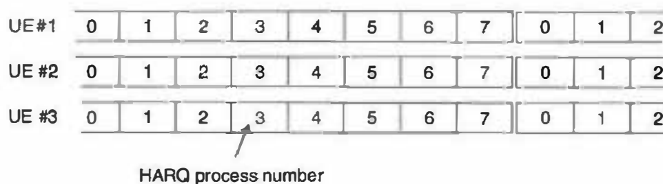
Figure 10.20 Example of activation of individual hybrid ARQ processes.
