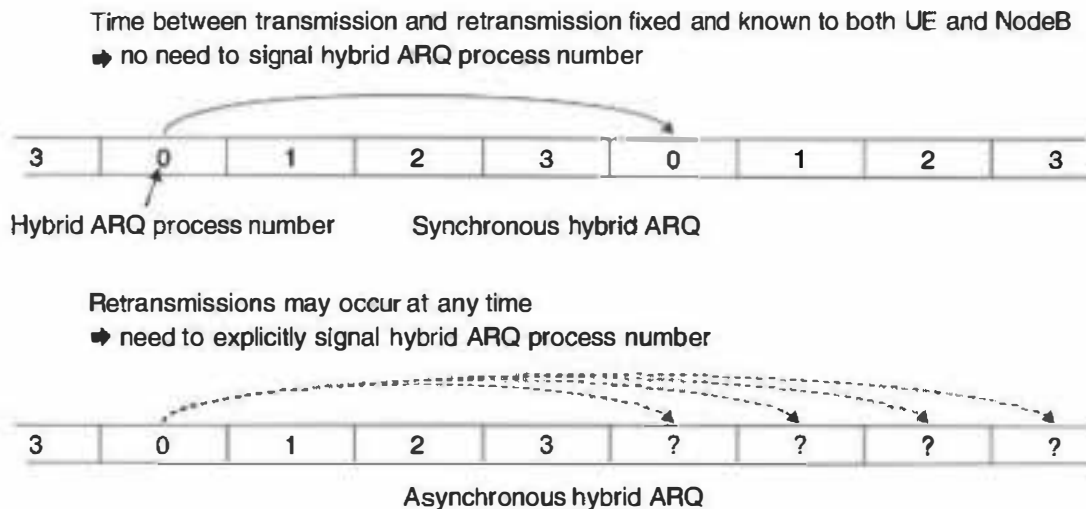
Figure 10.10 Synchronous vs. asynchronous hybrid ARQ.
