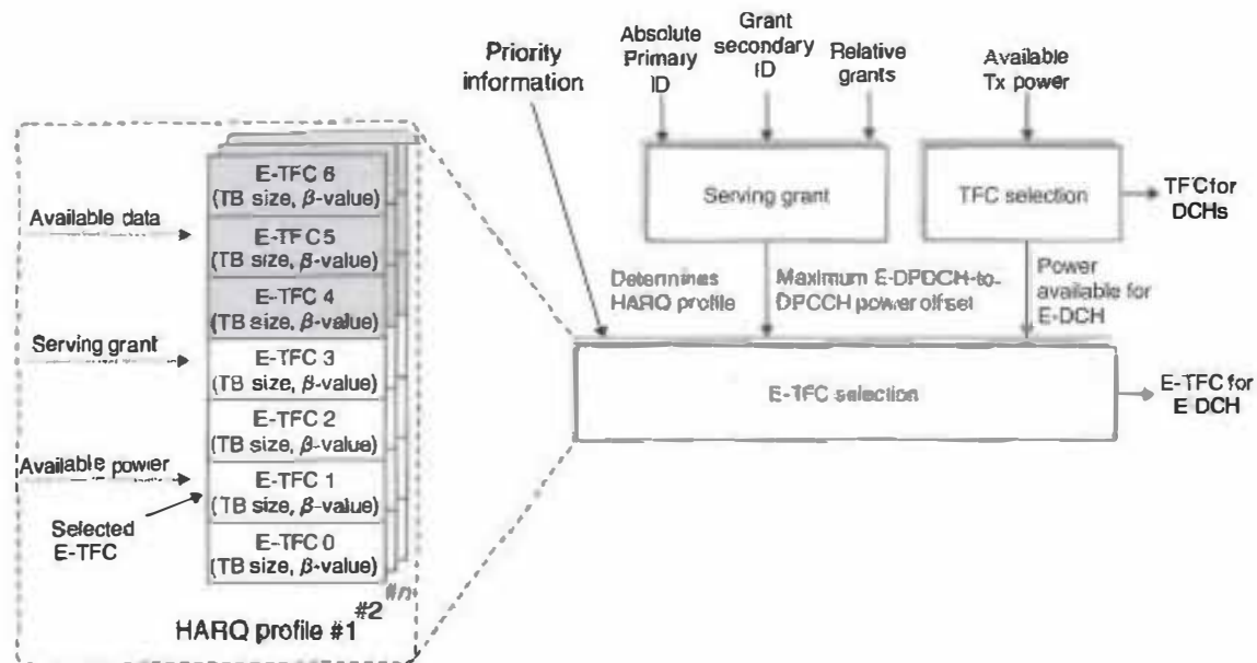
Figure 10.21 E-TFC selection and hybrid ARQ profiles.
