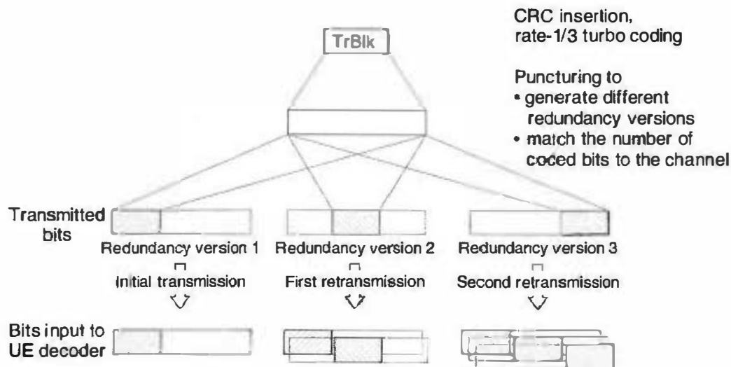
Figure 9.9 Generation of redundancy versions.
