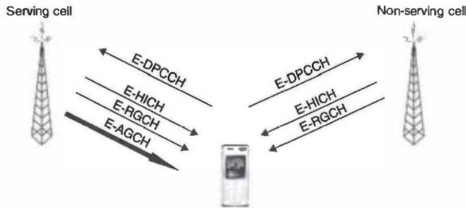
Figure 10.27 E-DCH-related out-band control signaling.
