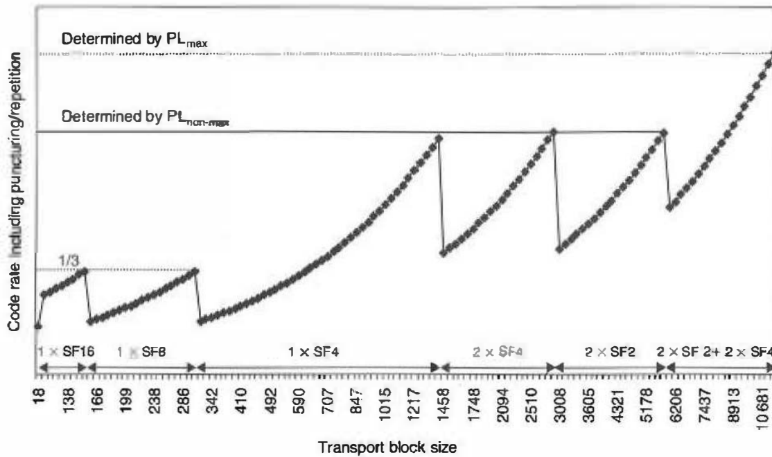
Figure 10.23 Amount of puncturing as a function of the transport block size.
