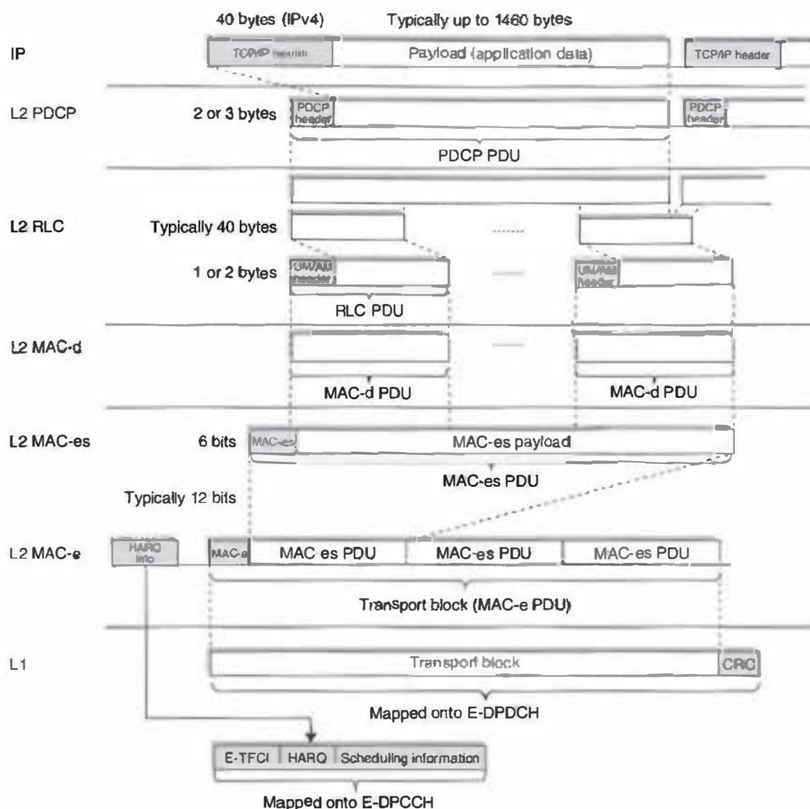
Figure 10.14 Data flow.
