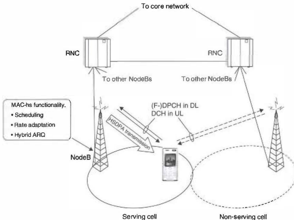
Figure 9.3 Illustration of the HSDPA architecture.
