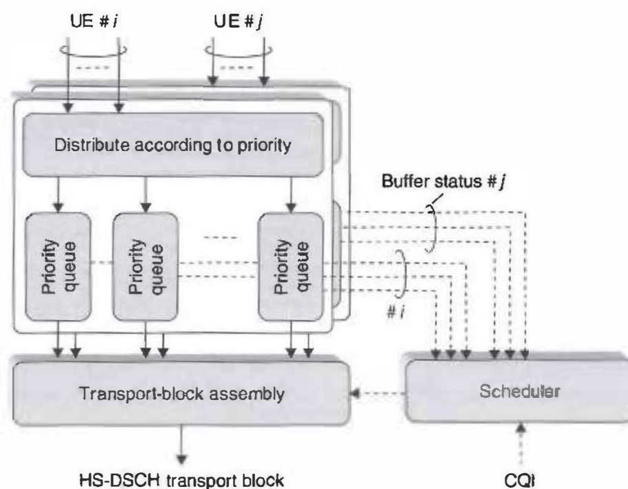
Figure 9.7 Priority handling in the scheduler.
