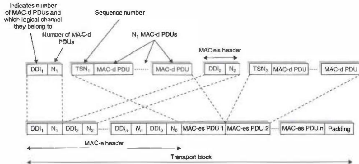
Figure 10.26 Structure and format of the MAC-e/es PDU.
