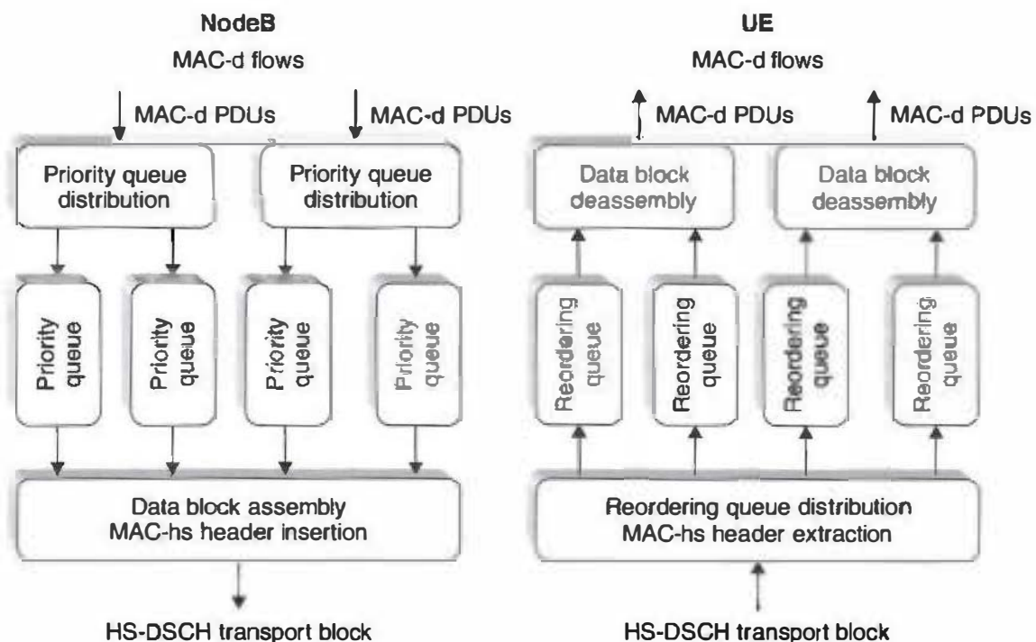
Figure 9.18 The priority queues in the NodeB MAC-hs (left) and the reordering queues in the UE MAC-hs (right).
