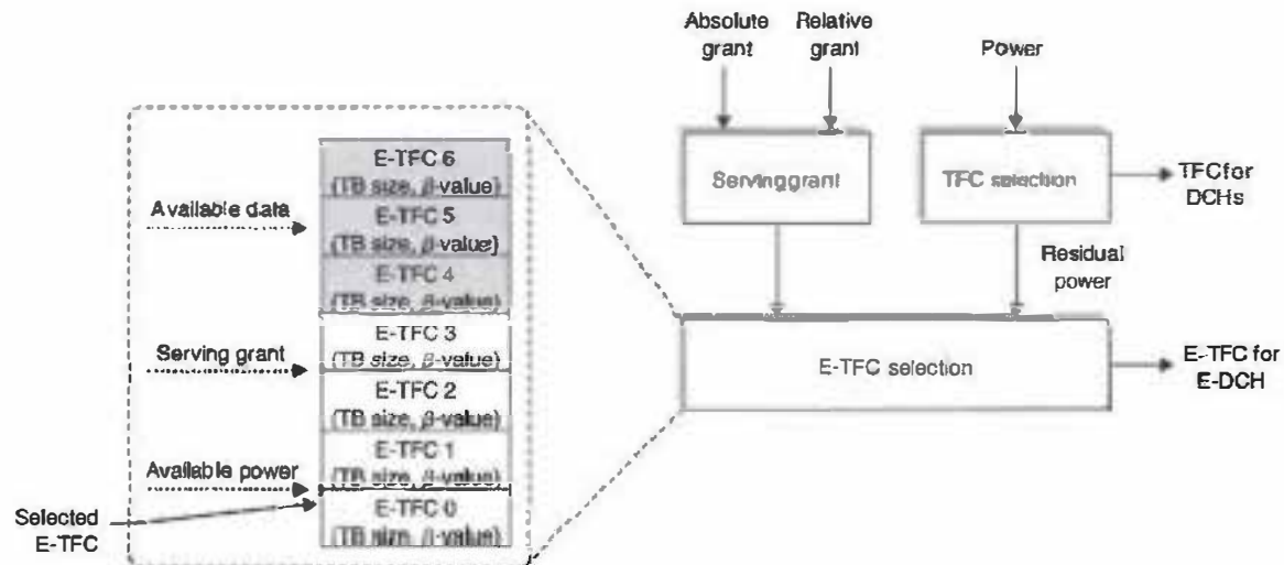
Figure 10.9 Illustration of the E-TFC selection process.
