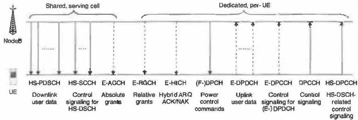
Figure 10.4 Overall channel structure with HSDPA and Enhanced Uplink. The new channels introduced as part of Enhanced Uplink are shown with dashed lines.
