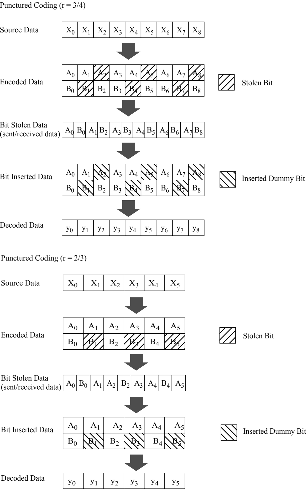
Figure 115—An example of the bit-stealing and bit-insertion procedure ( r = 3/4, 2/3 )
