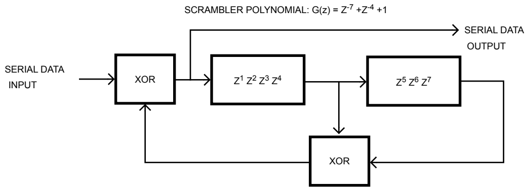
Figure 131—Data scrambler
