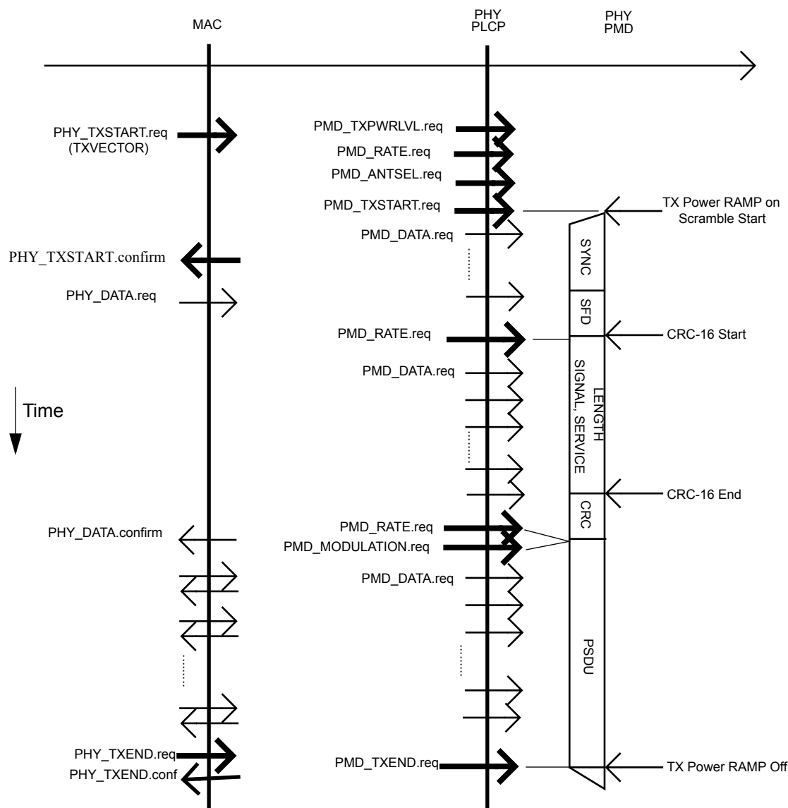
Figure 133—PLCP transmit procedure
