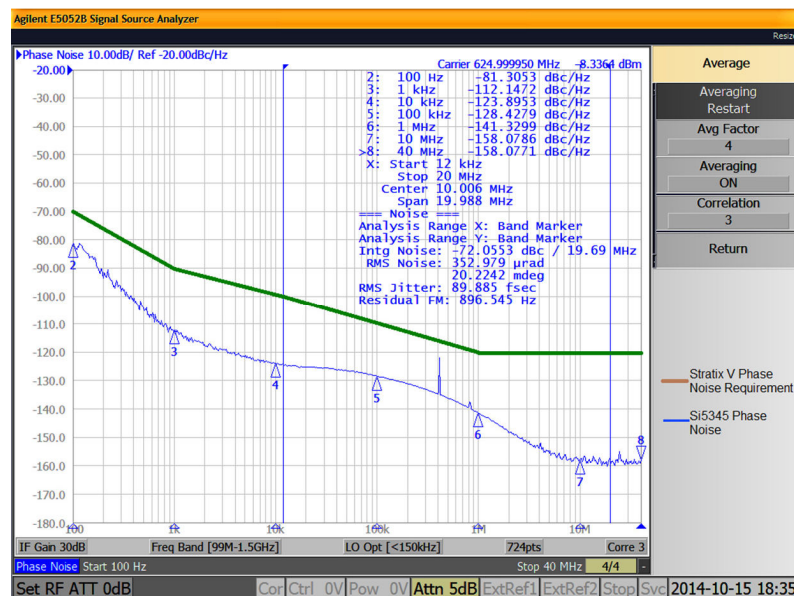
Figure 2. Si5345 Phase Noise vs. Stratix V FPGA Requirements for 10G Ethernet
