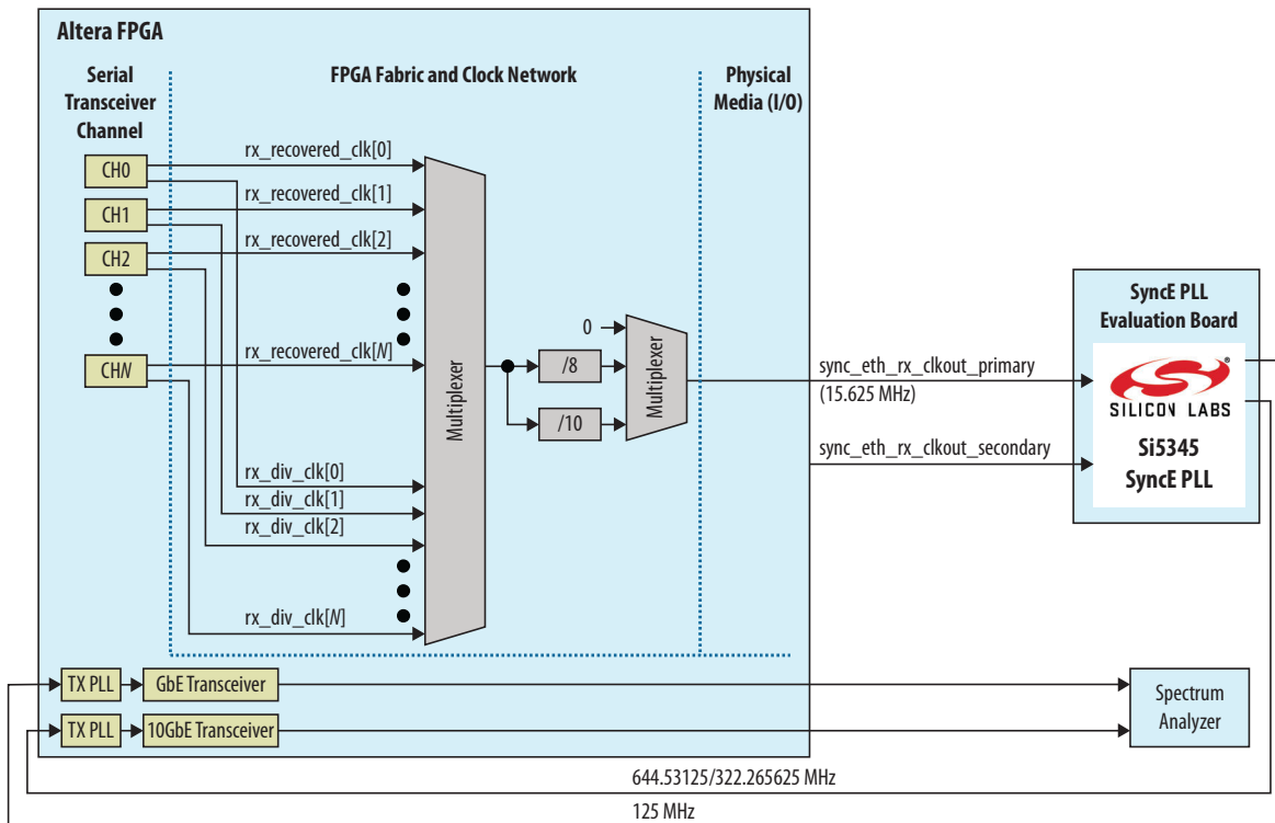
Figure 3. Altera and Silicon Labs SyncE Jitter Test Setup
