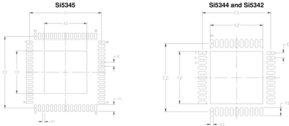
Figure 30. PCB Land Pattern
