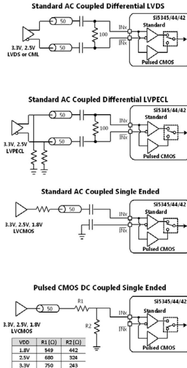
Figure 14. Termination of Differential and LVCMOS Input Signals
