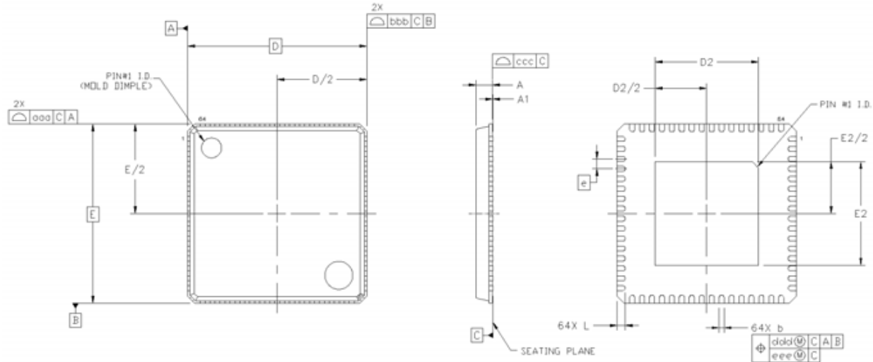
Figure 28. 64-Pin Quad Flat No-Lead (QFN)
