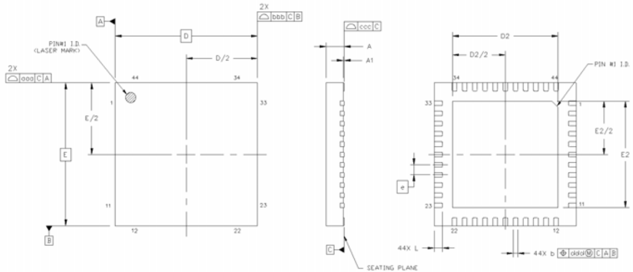
Figure 29. 44-Pin Quad Flat No-Lead (QFN)
