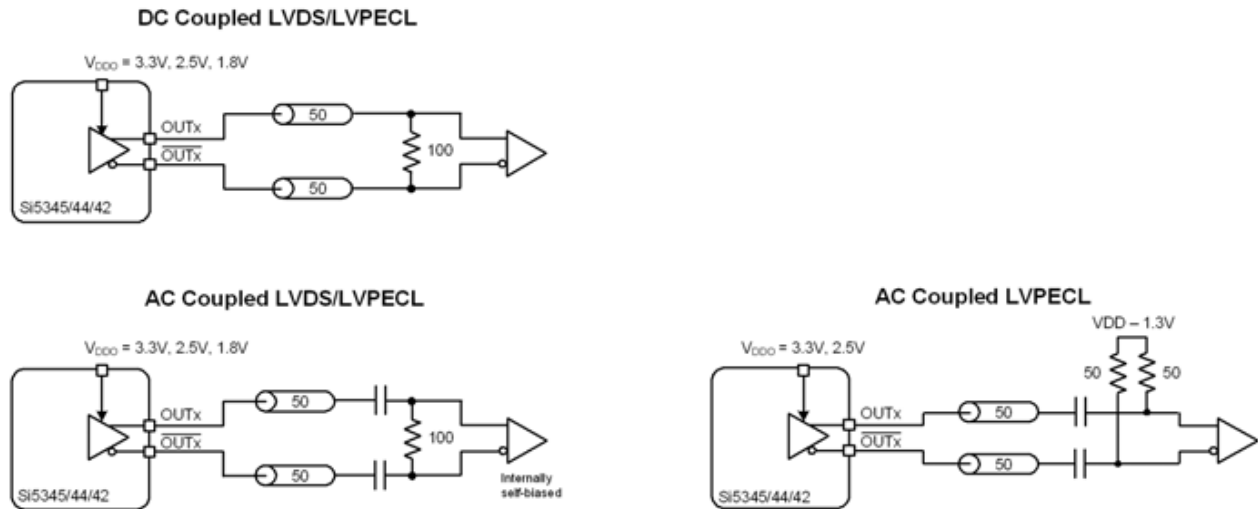
Figure 23. Supported Differential Output Terminations
