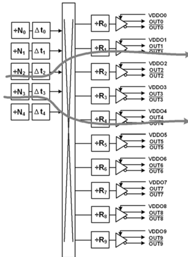
Figure 25. Example of Independently Configurable Path Delays
