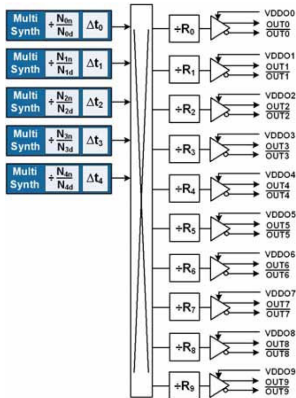
Figure 22. MultiSynth to Output Driver Crosspoint
