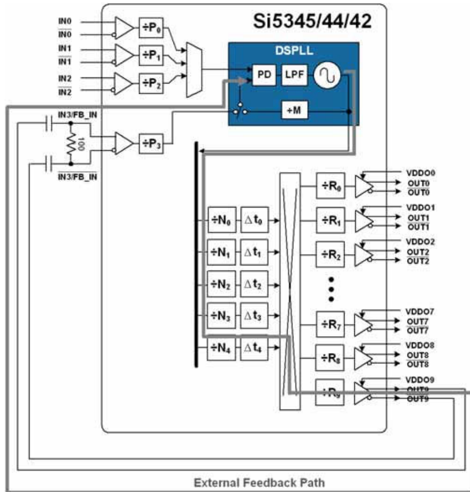
Figure 26. Si5345 Zero Delay Mode Setup
