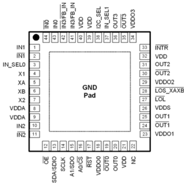
Si5344 44QFN Top View
