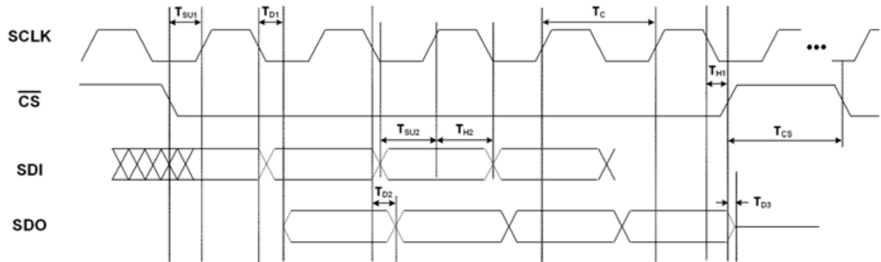
Figure 3. 4-Wire SPI Serial Interface Timing
