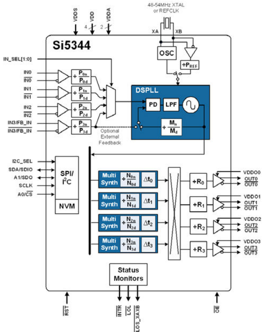
Figure 9. Si5344 Block Diagram
