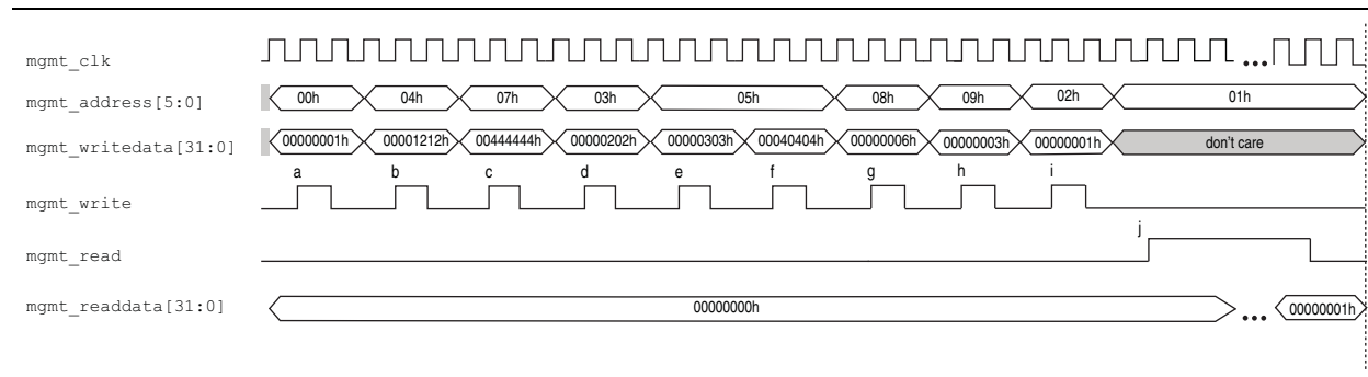
Figure 2. Waveform Example for Performing Dynamic Reconfiguration in Reconfiguring M , M_{\text{FRAC}} , N and C counters
