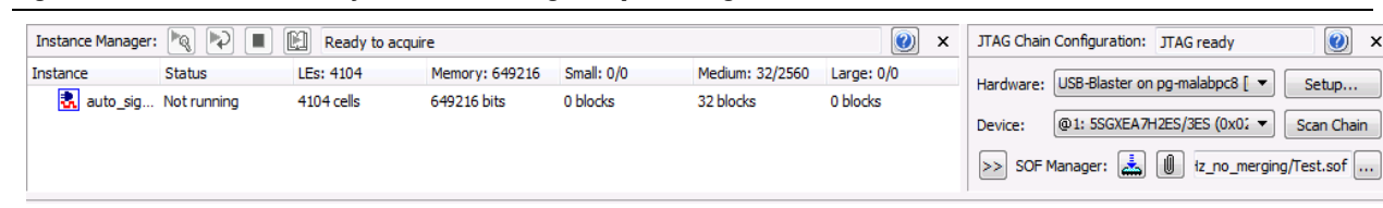
Figure 8. Install the SRAM Object File in the SignalTap II Dialog Box
