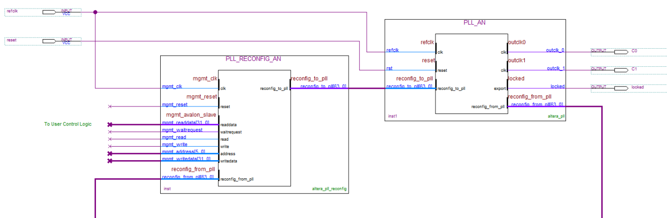
Figure 1. Altera PLL Reconfig and Altera PLL Megafunctions in the Quartus II Software
