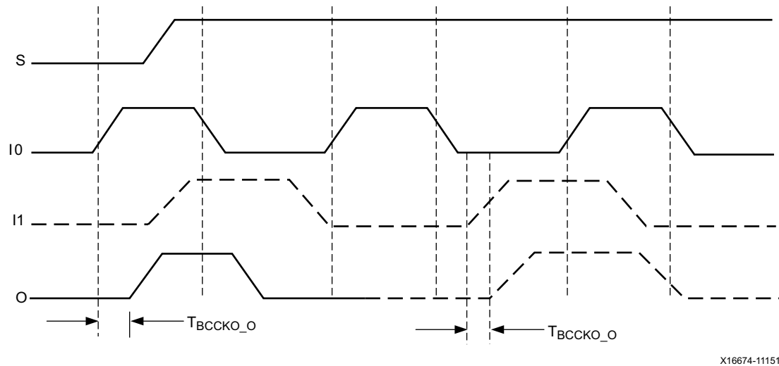
Figure 2-13: BUFGMUX_CTRL Timing Diagram
