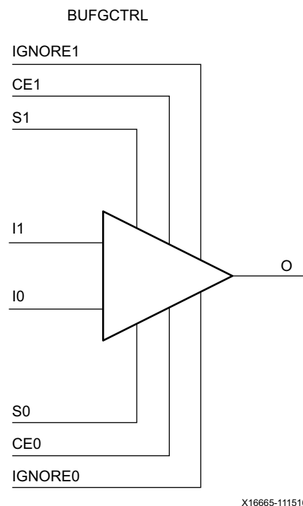
Figure 2-5: BUFCTRL Primitive
