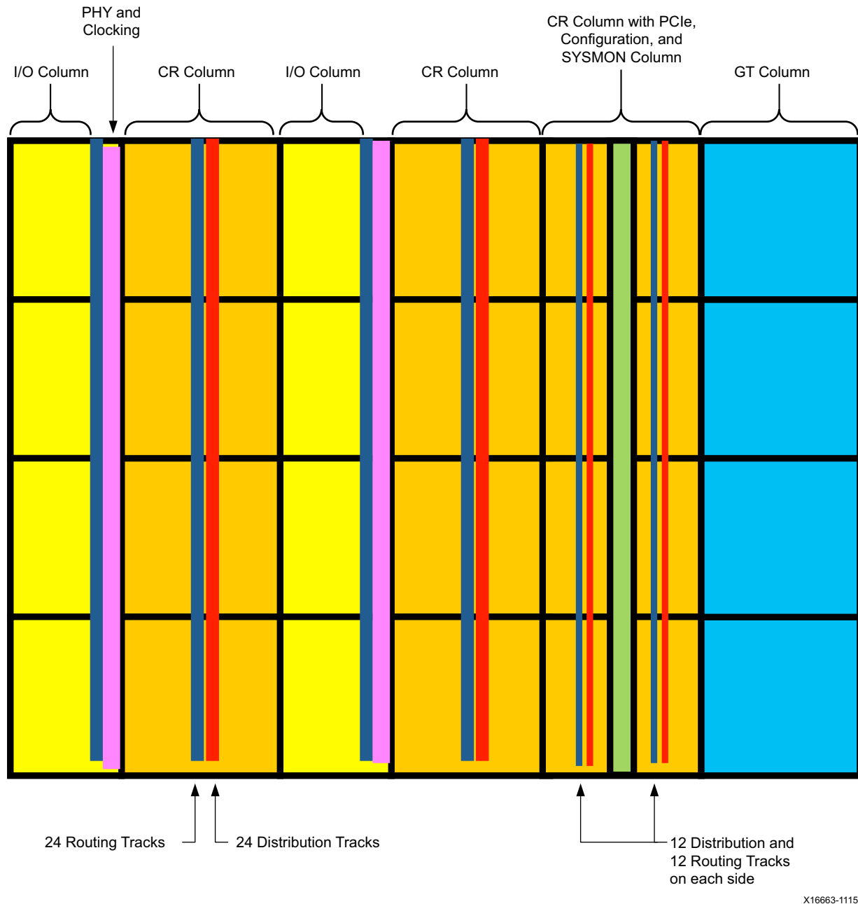
Figure 2-2: Vertical Clocking
