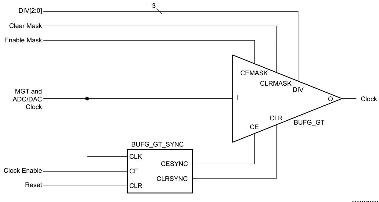
Figure 2-21: BUFG_GT Primitive
