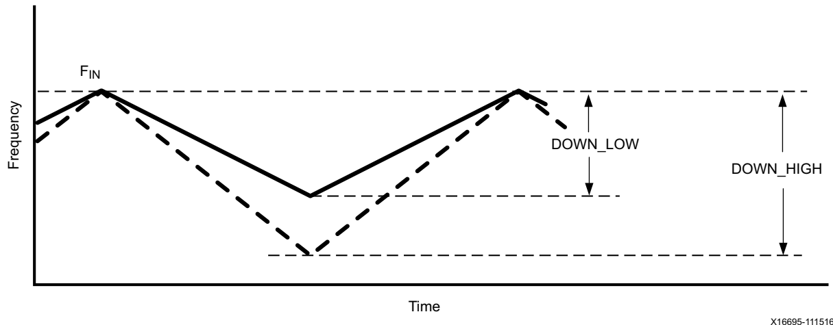
Figure 3-14: Down-Spread Modulation
