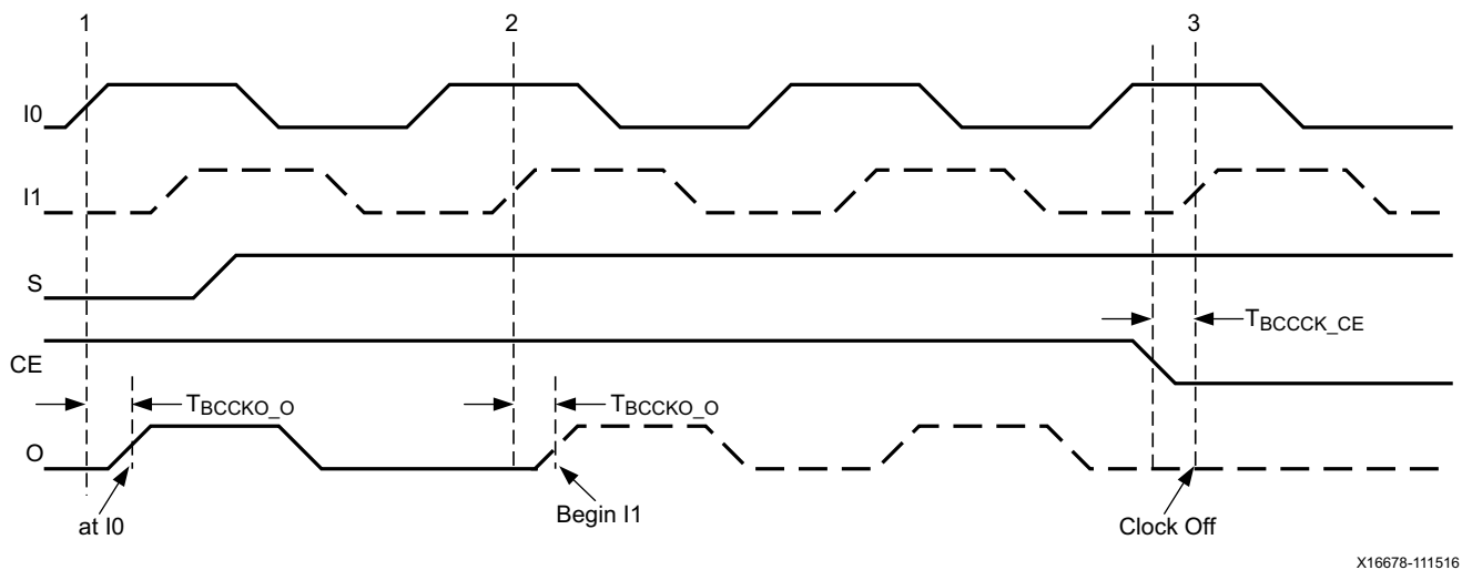
Figure 2-17: BUFGMUX_CTRL with a CE Timing Diagram
