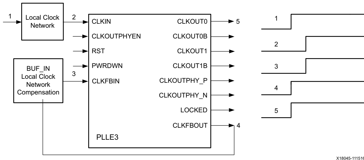
Figure 3-17: Clock Deskew Using BUF_IN Compensation Mode
