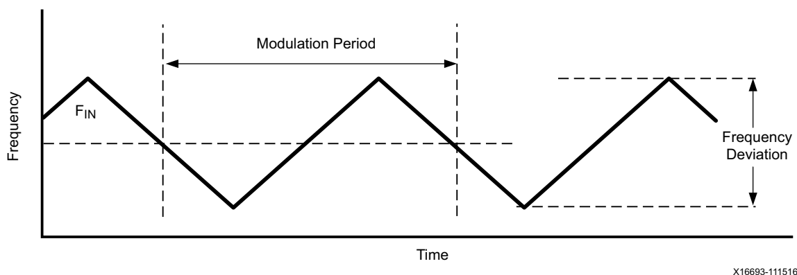
Figure 3-12: Center-Spread Modulation
