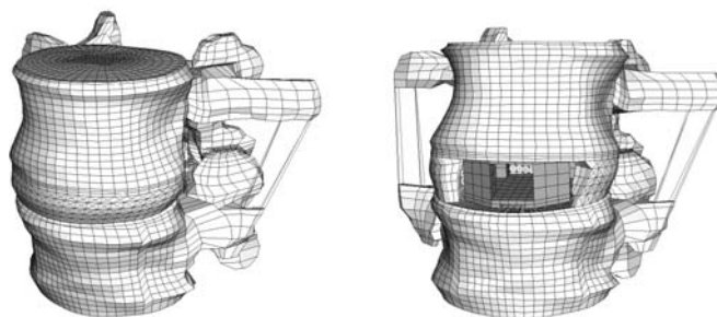
Fig. 1 The intact finite-element model ( left ) and the model with cage ( right )
