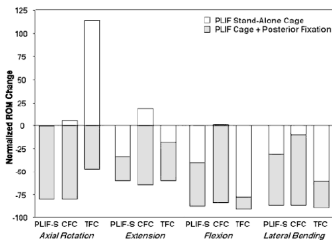
Fig. 3 Normalized to intact percentage changes in the range of motion (ROM) of three different cage constructs (PLIF-Spacer, Contact Fusion Cage and Ray TFC), used as stand-alone (white bars) and supplemented with pedicle screw fixation (gray bars)
