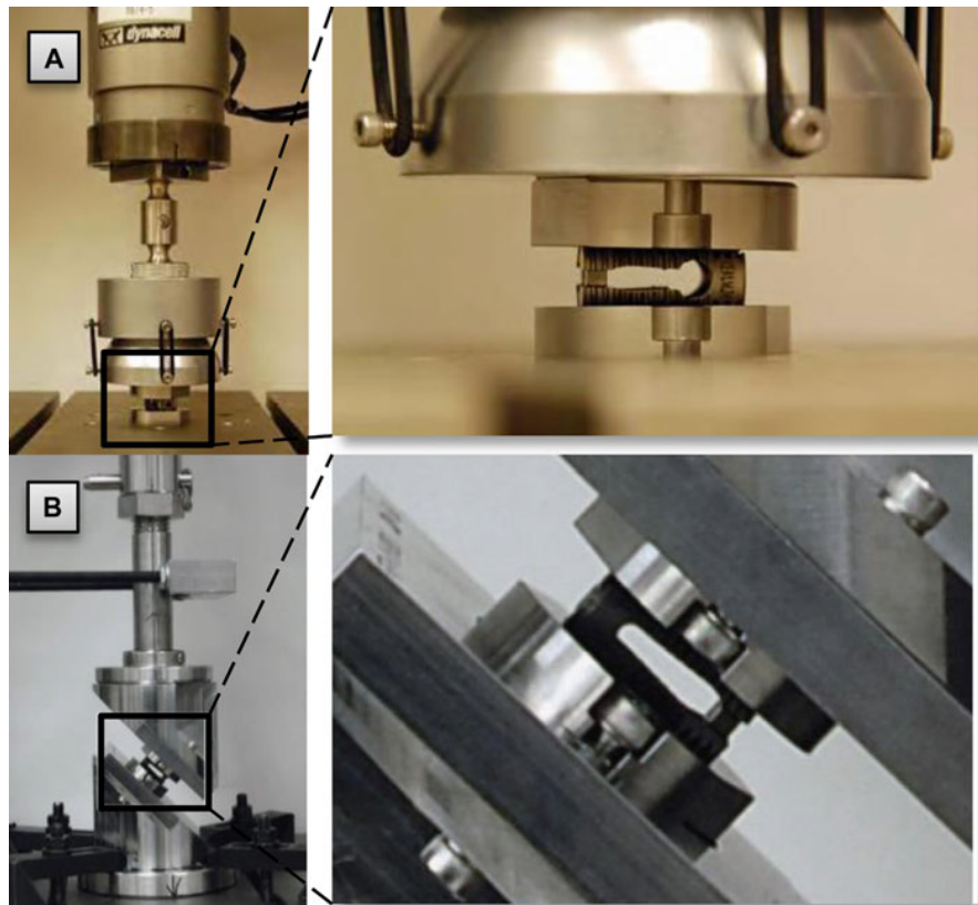
Figure 5 Mechanical test setups for (A) static and dynamic axial compression testing and (B) compressive shear testing.
