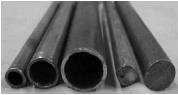
Figure 3. Indenters used in compression testing. Hollow indenters of 9.53, 12.70, and 19.10 mm diameter and solid indenters of 9.53 and 12.70 mm diameters are shown.
