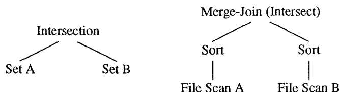
Figure 3. Logical and physical algebra expressions.
