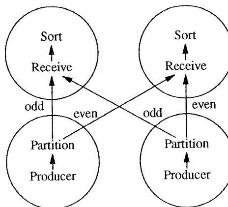
Figure 31. Deadlock-free scenario.
