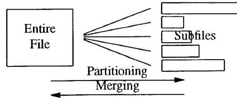
Figure 18. Partitioning skew.
