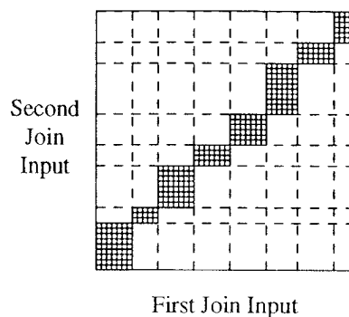
Figure 13. Effect of partitioning for join operations.
