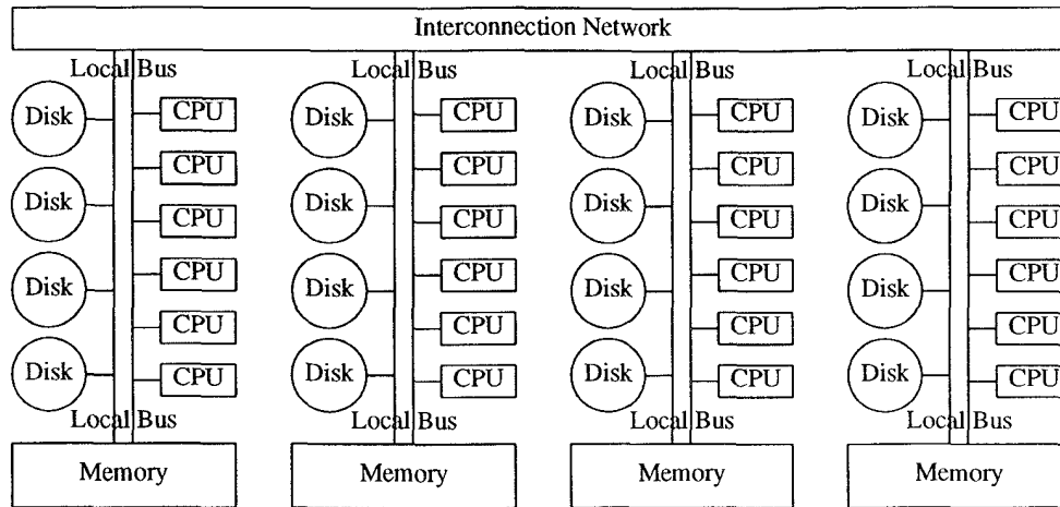
Figure 29. A hierarchical-memory architecture.
