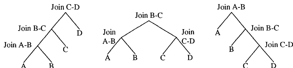
Figure 4. Left-deep, bushy, and right-deep plans.
