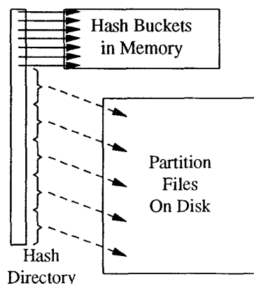
Figure 8. Hybrid hashing.
