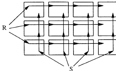
Figure 34. Symmetric fragment-and-replicate join.
