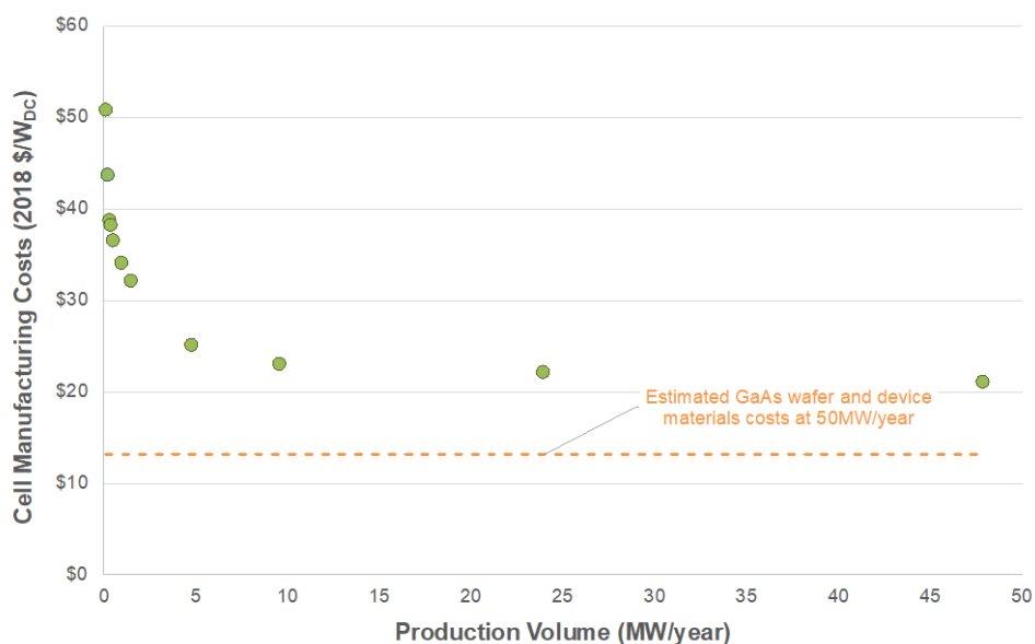
Figure 11. Estimated impact of increased production volume on 2J GaInP/GaAs solar cell costs fabricated with MOCVD
