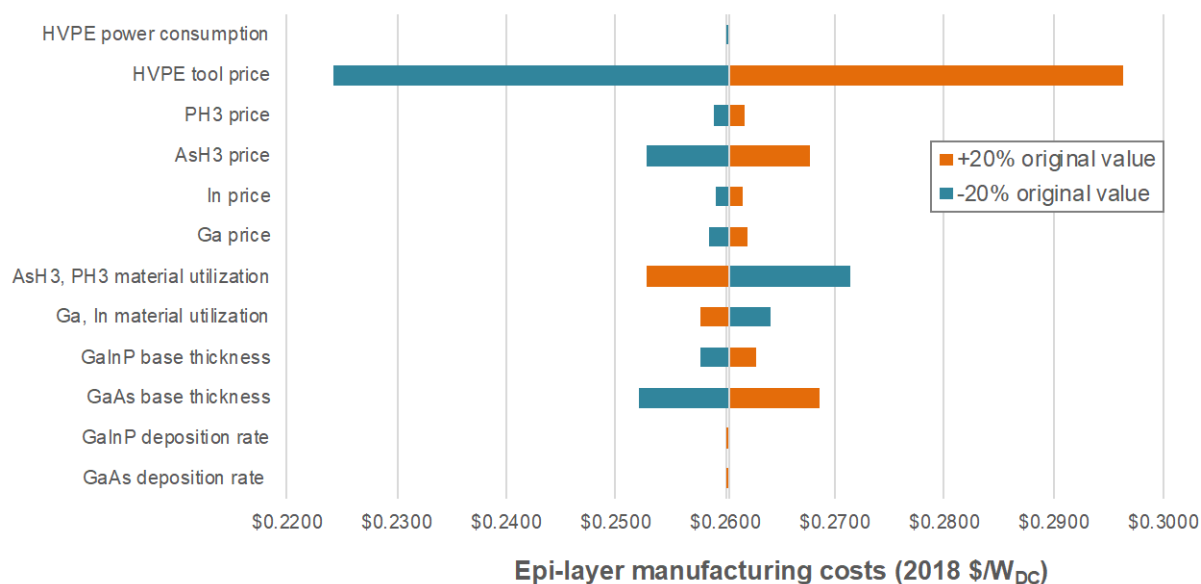
Figure 15. Sensitivity of epi-layer costs for a 2J GaInP/GaAs cell grown via D-HVPE to key input parameters
