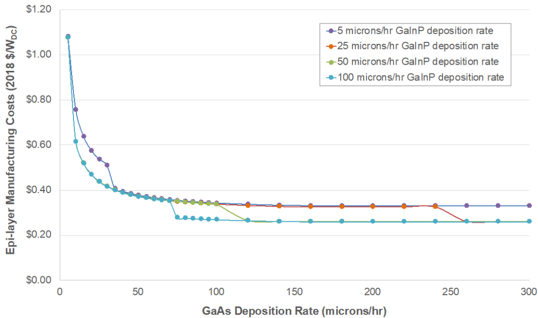
Figure 16. Sensitivity of epi-layer costs for a 2J GaInP/GaAs solar cell grown using D-HVPE to GaAs and GaInP deposition rates
