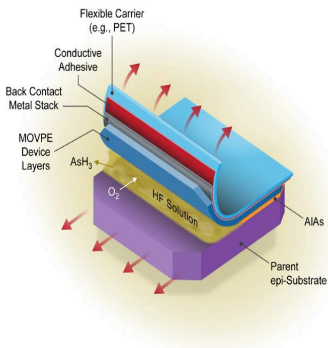
Figure 6. Illustration of the ELO process
