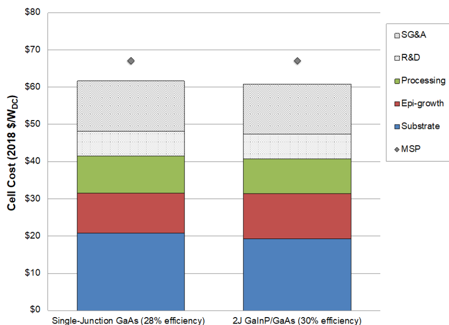
Figure 8. Comparison of cell cost breakdown for single- and dual-junction III-V solar cells grown via MOCVD
