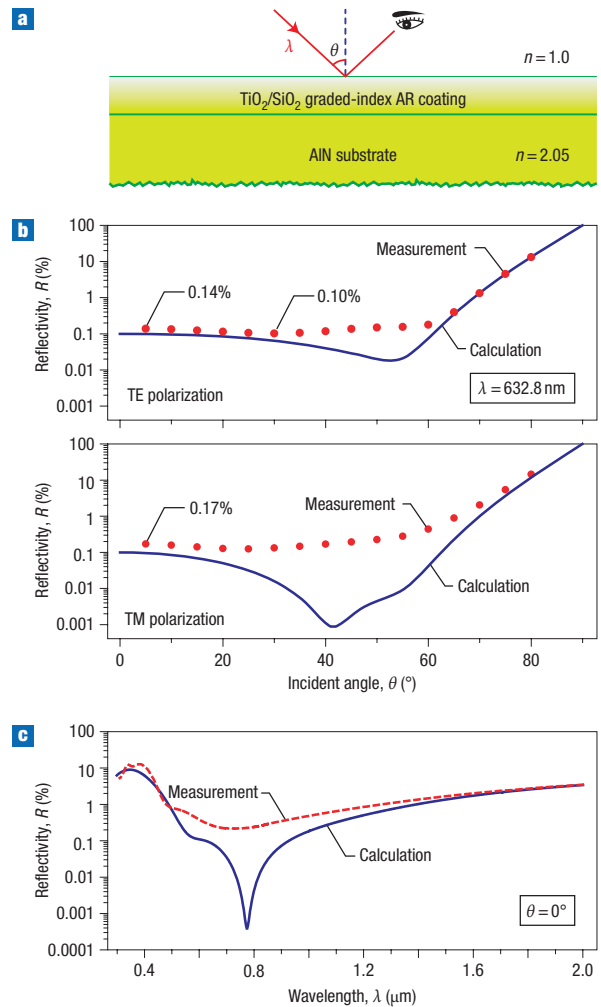
Figure 4 Reflectivity of graded-index coating. a , Schematic of reflectivity measurement. b , Theoretical (solid line) and measured (dotted line) reflectivity versus incident angle of graded-index coating at wavelength \lambda = 632.8 nm. c , Wavelength dependence of theoretical (solid line) and measured (dashed line) reflectivity of graded-index coating at normal incidence.
