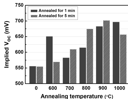
Figure 1. The implied V_{oc} of double side TOPCon electron contacts measured by quasi-stead-state photoconductance annealing at various temperatures and times.
