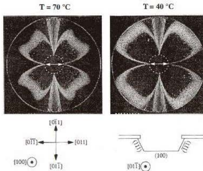
Fig. 5. Appearance of wagon-wheel mask patterns after etching in 35% KOH. The etch depths (i.e., in the [100] direction, into the plane of the paper) are 155\ \mu\text{m} for the sample on the left (etched at 70.3^\circ\text{C} ) and 227\ \mu\text{m} for the sample on the right (etched at 40.2^\circ\text{C} ). The diagrams illustrate the four \langle 110 \rangle directions in the (100) plane; V-grooves aligned along these directions have sides defined by \{111\} planes. The length of the radius from the center to the pattern cusp along these directions is proportional to the \{111\} etch rate.
